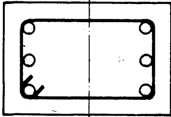
Rectangular Tied Column with Bars on y - faces
