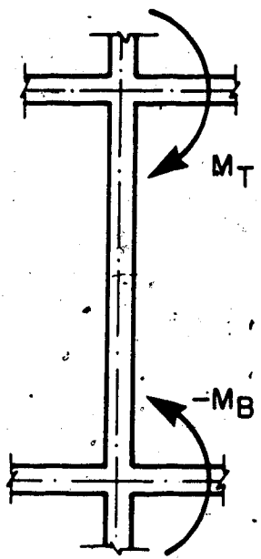
(a) Input Moments from Analysis Clockwise Positive (b) Deflected Shape and Design Moments used by Program
