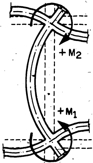
(a) Input Moments from Analysis Clockwise Positive (b) Deflected Shape and Design Moments used by Program
