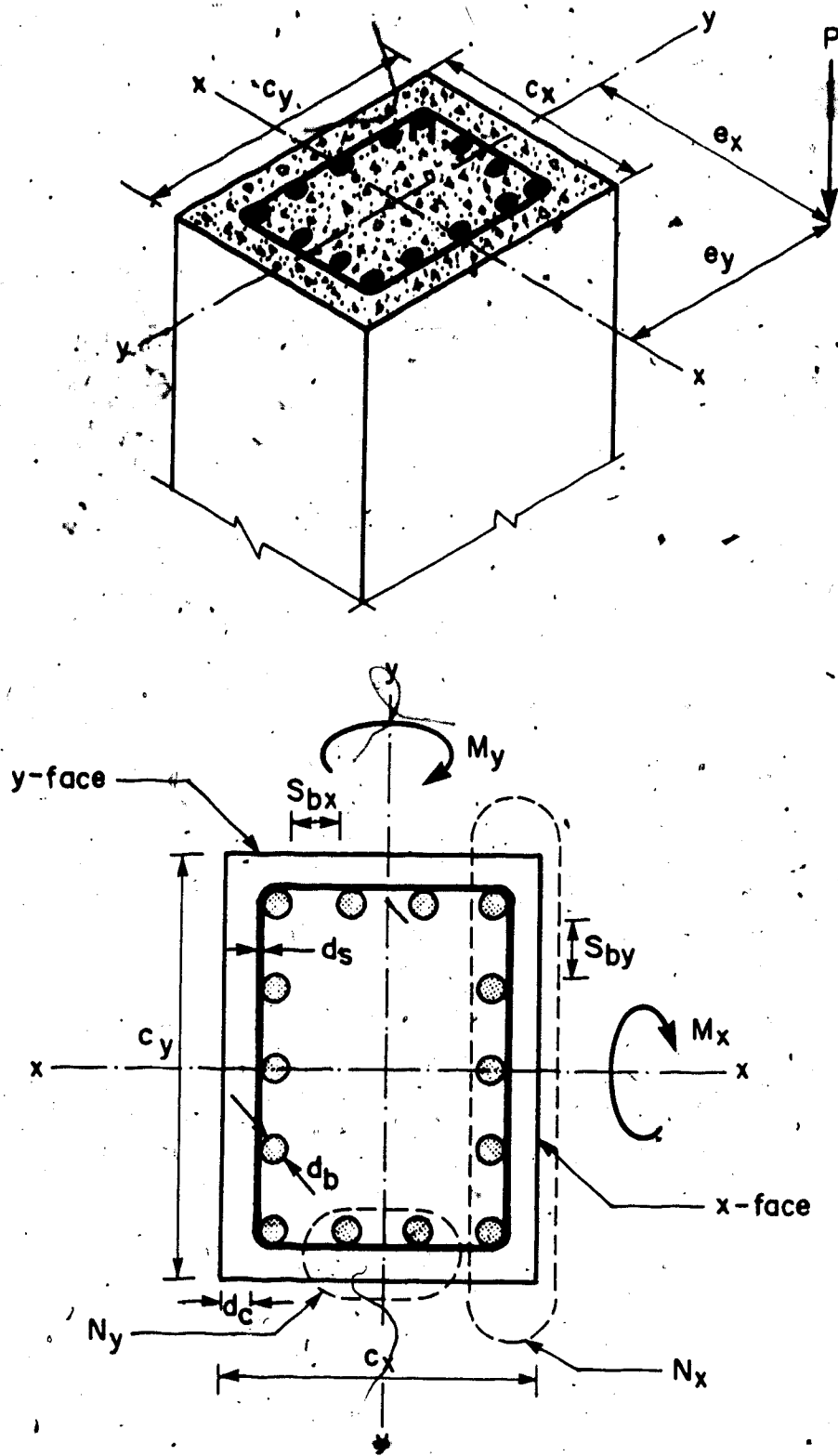
Figure A.2 Sign Convention and Nomenclature
