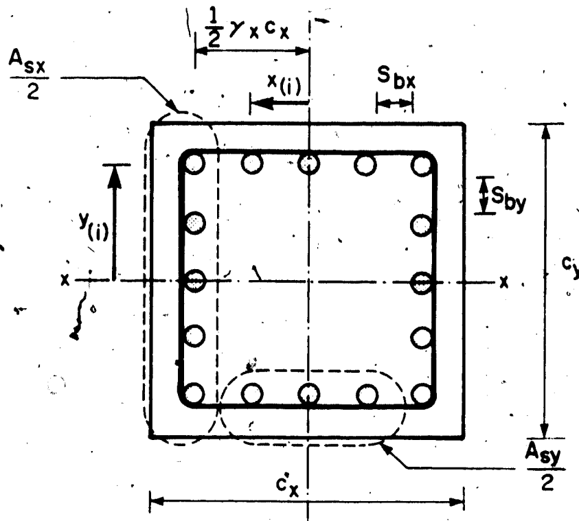
Figure A.3 Reinforcement in a Rectangular Array
