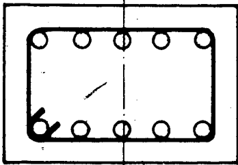
Rectangular Tied Column with Bars on x - faces
