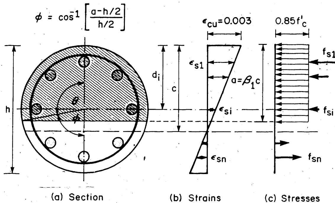
Figure 4.8 Compression Zone for Circular Section ( a > h/2 )
