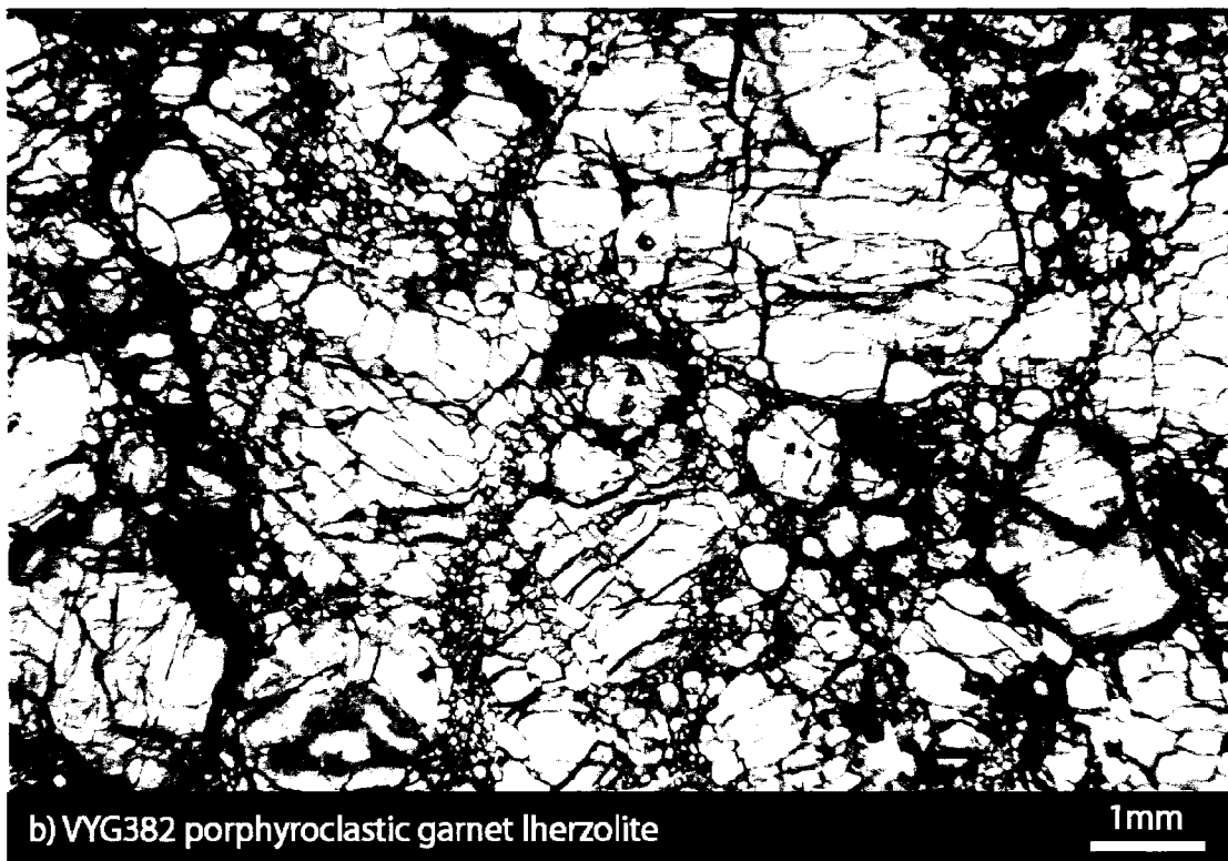
Fig. 3.2.2 Thin section images of garnet lherzolites from the Voyager kimberlite pipe
