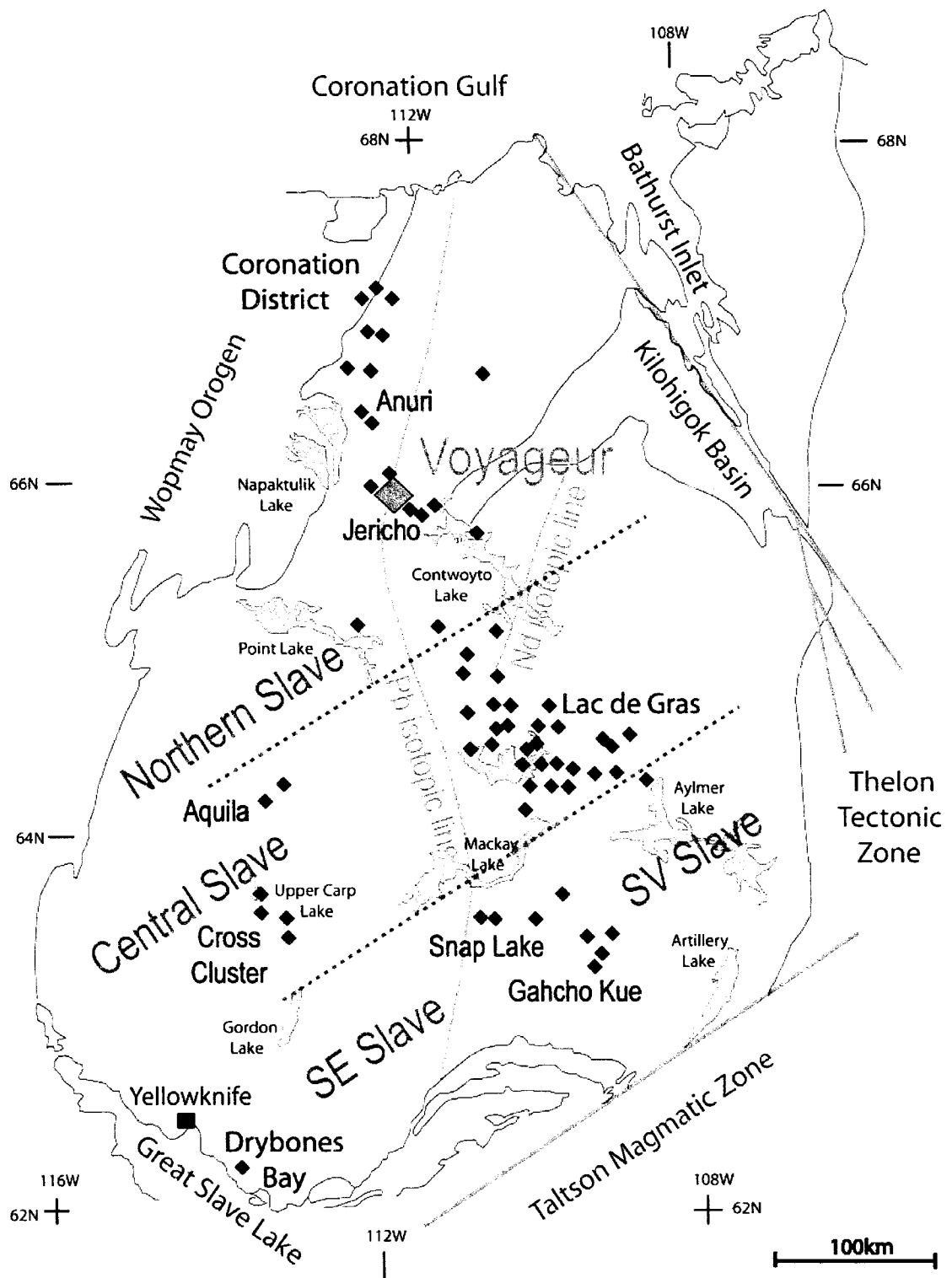
Fig. 2.3.1 Distribution of kimberlites in the Slave Province. Pb isotopic line from Thorpe et al., 1992. Nd isotopic line from Davis and Hegner, 1992. Geochemical boundaries from Grutter et al., 1999.
