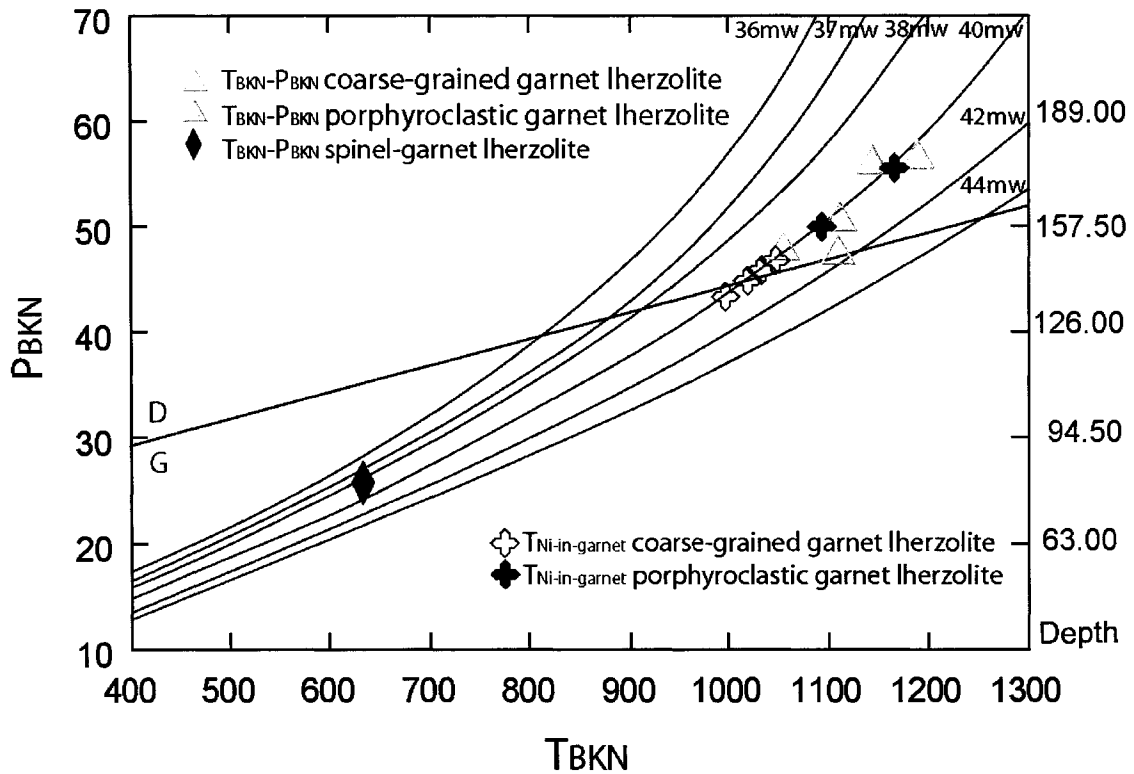
Fig. 4.4 Comparison of garnet equilibration temperatures calculated using T_{\text{Ni-in-garnet}} (version of Canil, 1999) and T_{\text{BKN}}\text{-}P_{\text{BKN}} geothermometers
