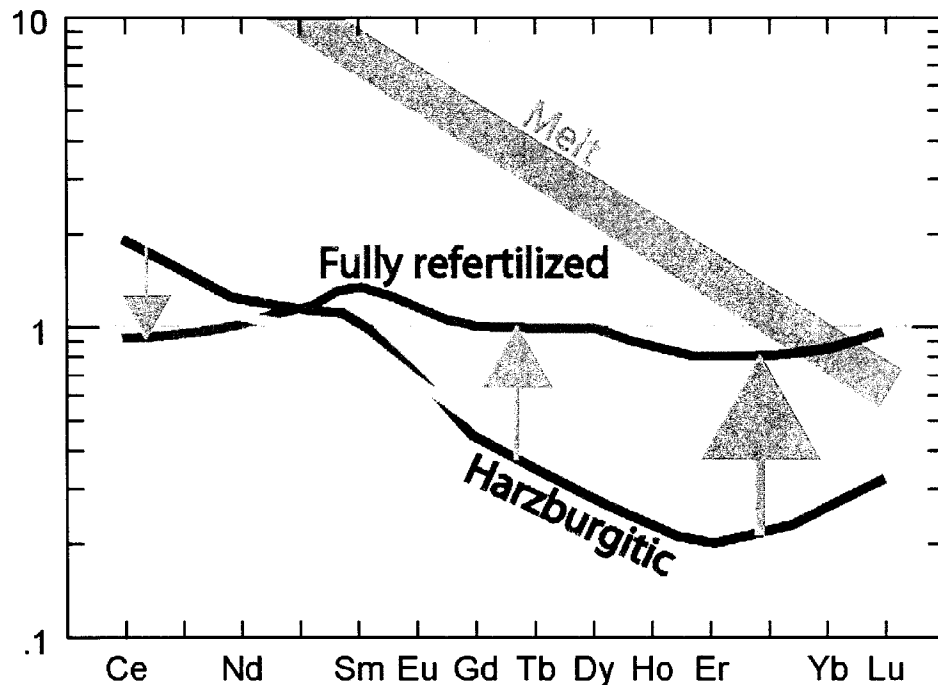
Fig. 3.4.4 Origin of lherzolitic garnets through metasomatic enrichment of former harzburgites. Modified after Stachel et al. (2004).
