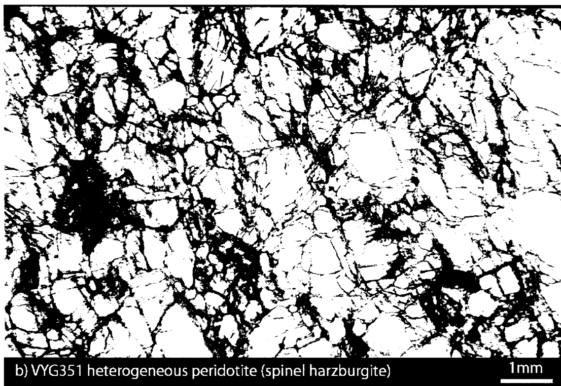
Fig. 3.2.7 Thin section images of heterogeneous samples from the Voyager kimberlite pipe
