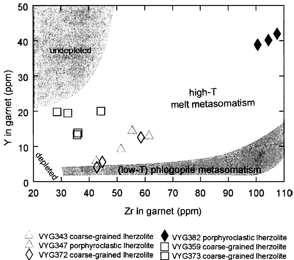
Fig. 3.4.6 Zr (ppm) Vs Y (ppm) concentrations in lherzolitic garnets from the Voyager peridotite xenoliths. Metasomatic fields after Griffin & Ryan (1995).
