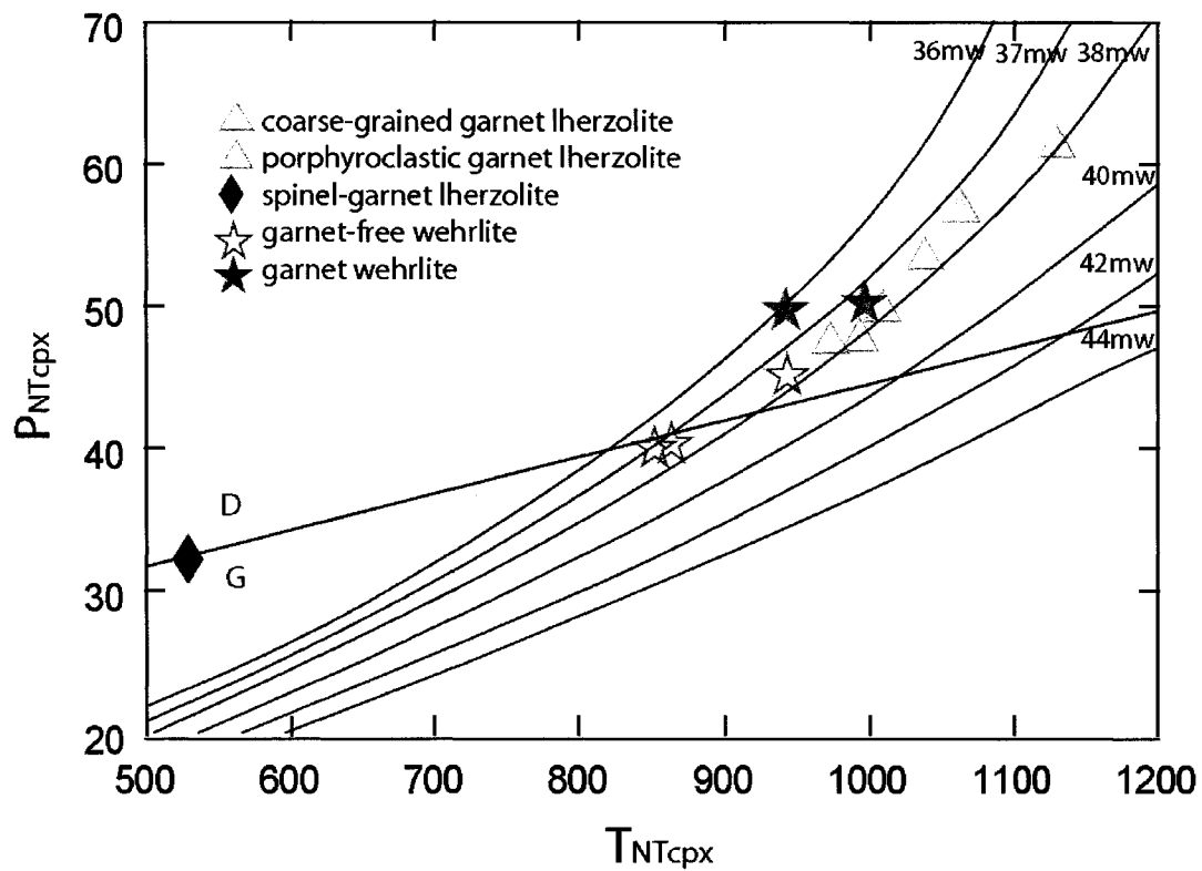
Fig. 4.3 Averaged P-T estimates of peridotite xenoliths from Voyageur kimberlite calculated iteratively using T_{NTcpx} - P_{NTcpx} . Geotherms from Pollack & Chapman (1977)
