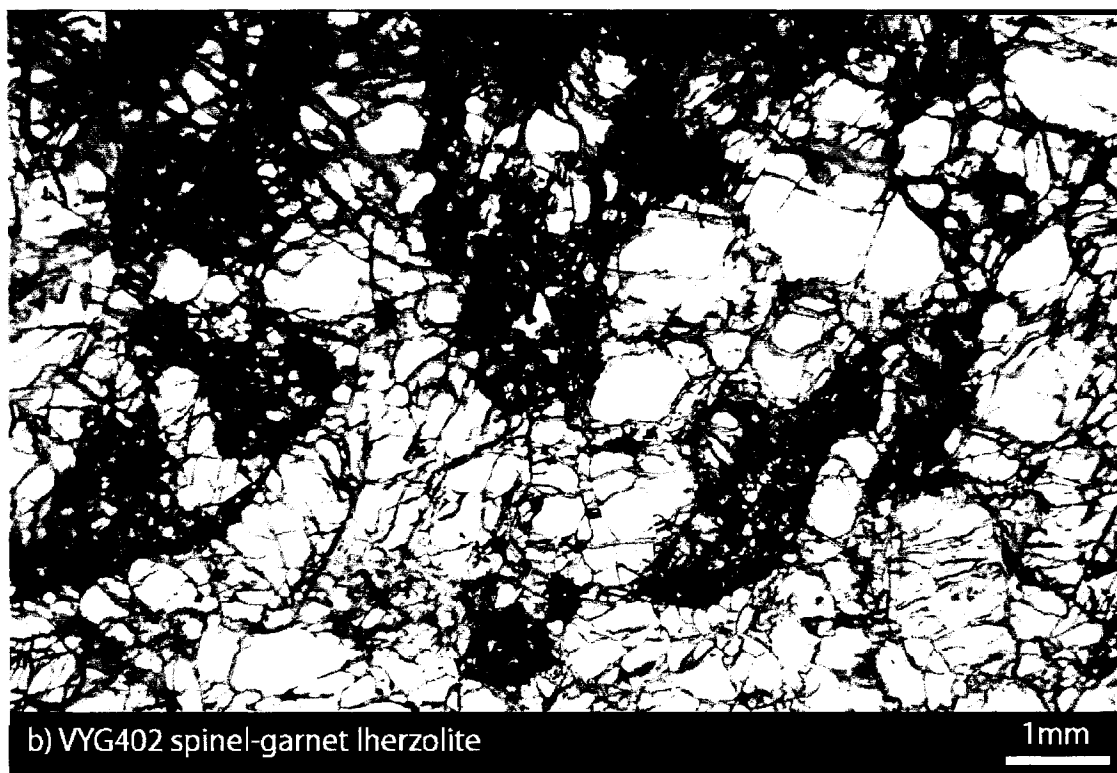
Fig. 3.2.6 Thin section images of spinel-garnet lherzolites from the Voyager kimberlite pipe
