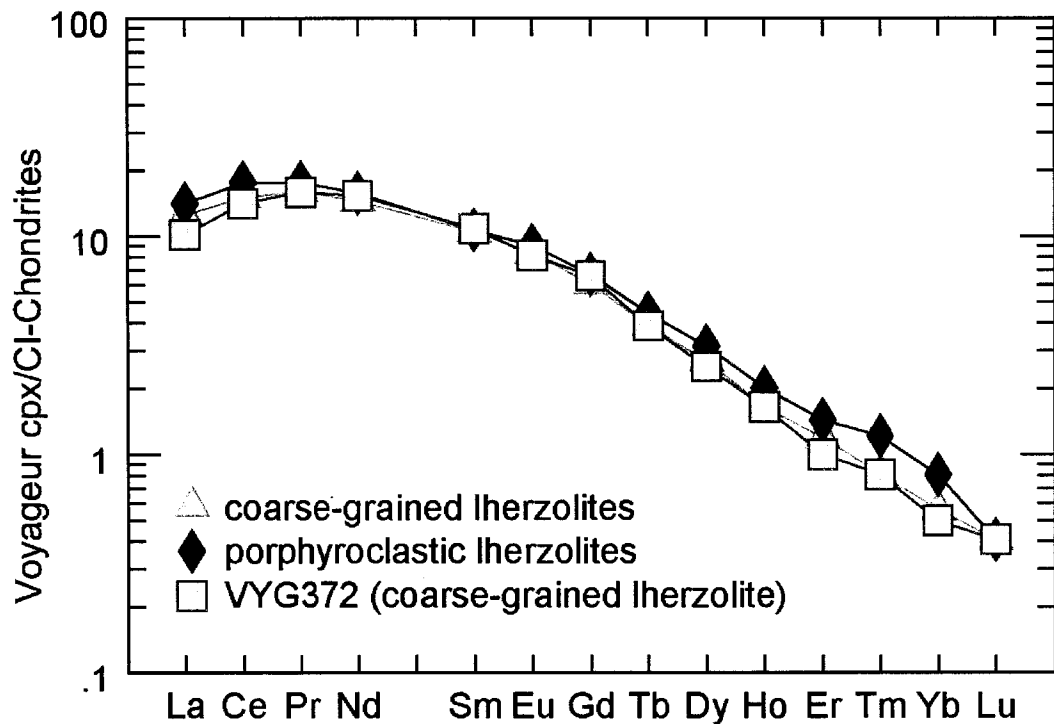
Fig. 3.4.2 Averaged REE abundances in lherzolitic clinopyroxenes from Voyageur peridotite xenoliths normalized to the C1 chondrite (McDonough & Sun, 1996)
