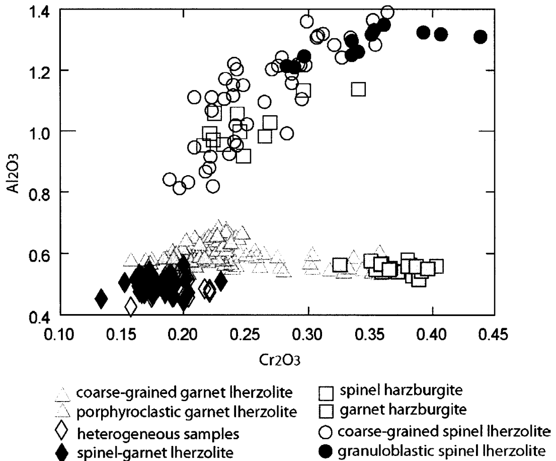
Fig. 3.3.2 Composition of orthopyroxenes from the Voyageur peridotite xenoliths
