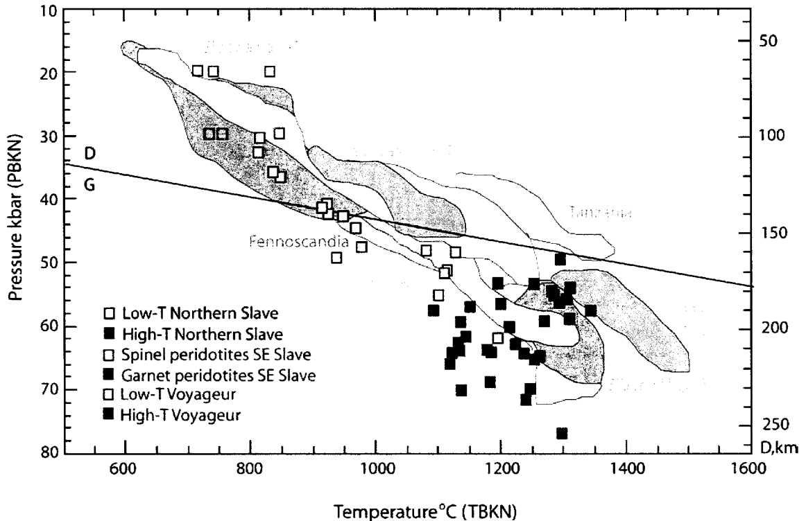
Fig. 5.3 Equilibrium pressure and temperature estimates calculated using the TBKN-PBKN geothermobarometer for Voyager garnet peridotite xenoliths in comparison with data from cratonic mantle worldwide. Data points are from Kopylova et al., 1999 (Northern Slave) and Kopylova & Caro, 2004 (Southeastern Slave). P-T fields are based on data from Boyd, 1990 (unpublished, as cited in Kopylova and Caro, 2004) for the Kaapvaal craton; from Boyd et al., 1997 (Udachnaya) and Roden et al., 1999 (Mir) for the Siberian craton; from Kukkonen & Peltonen, 1999; Lehtonen et al., 2003 for the Fennoscandian craton; from Lee & Rudnick, 1999 for the Tanzanian craton; from Meyer et al., 1994 for the Superior craton; from Kjarsgaard & Peterson, 1992 and Schmidberger & Francis, 1999 for the Canadian Shield (Somerset Island). Modified from Kopylova & Caro, 2004
