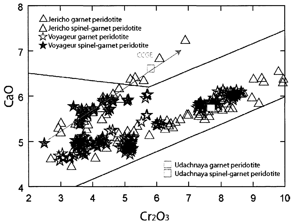
Fig. 5.2 Comparison of the CCGE trend in garnets from Voyageur and Jericho
