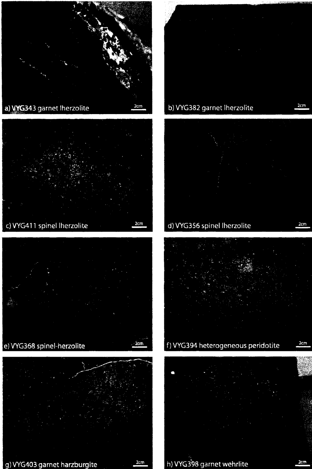
Fig. 3.2.1 Core samples from the Voyageur kimberlite pipe
