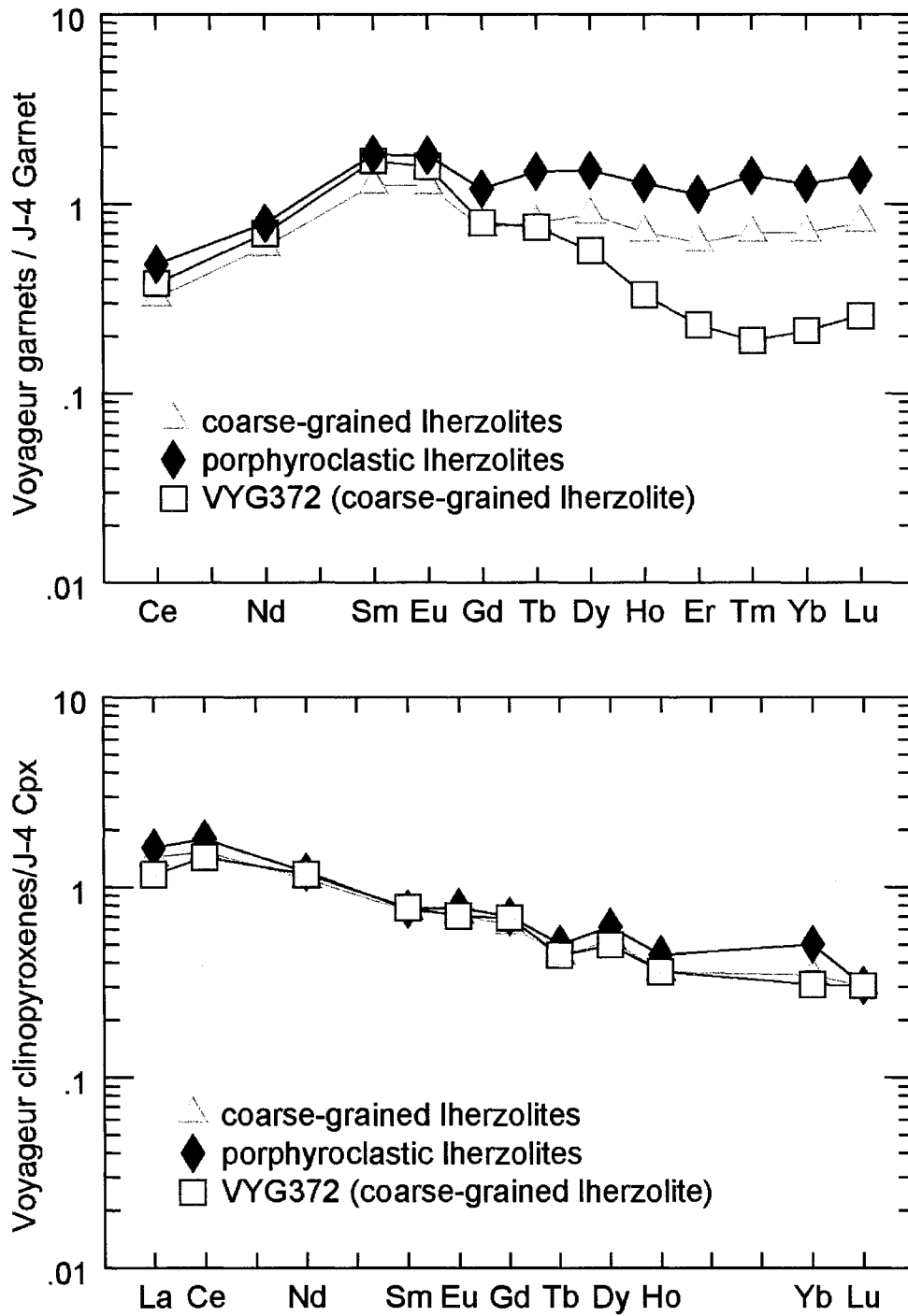
Fig. 3.4.3 Averaged REE abundances in lherzolitic garnets (a) and clinopyroxenes (b) from Voyager peridotite xenoliths normalized to the composition of a primitive lherzolitic garnet/clinopyroxene (J4 of Jagoutz & Spettel).
