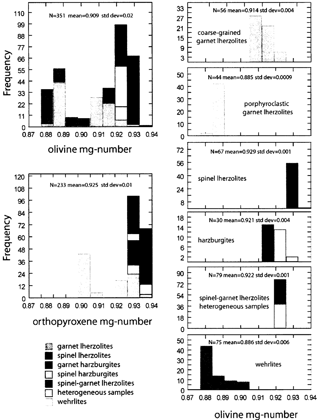
Fig. 3.3.1 Mg number of olivines and orthopyroxenes from the Voyageur peridotite xenoliths:
