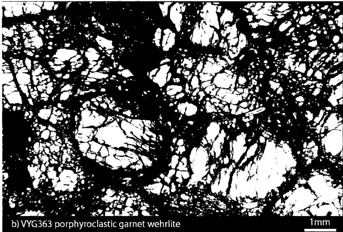
Fig. 3.2.5 Thin section images of wehrlites from the Voyager kimberlite pipe
