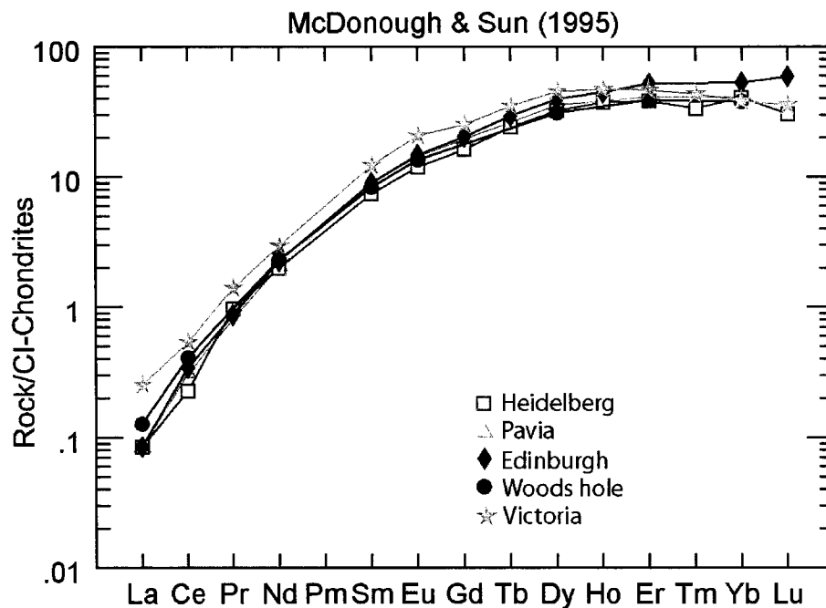
Fig. 3.1.1 Comparison of LA-ICPMS measurements on mantle garnet PN2 obtained at University of Victoria with SIMS measurements on the same garnet obtained at University of Edinburgh (Stachel), University of Heidelberg (Tappert), University of Pavia (Ottoloni) and Woods Hole Oceanographic Institution (Banas) laboratories.
