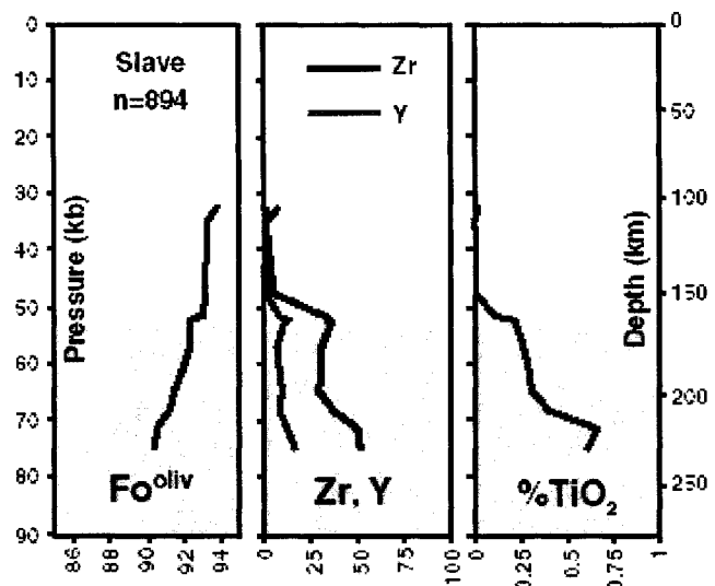
Fig. 2.3.2 The layered structure of the Slave lithospheric mantle shown by key geochemical indicators
