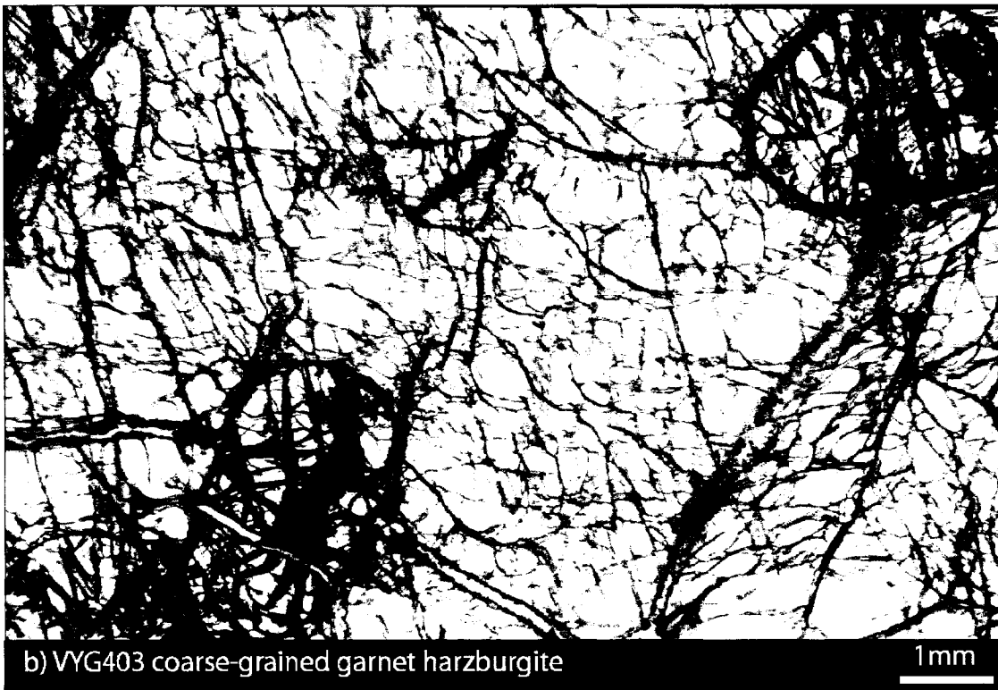
Fig. 3.2.4 Thin section images of harzburgites from the Voyager kimberlite pipe
