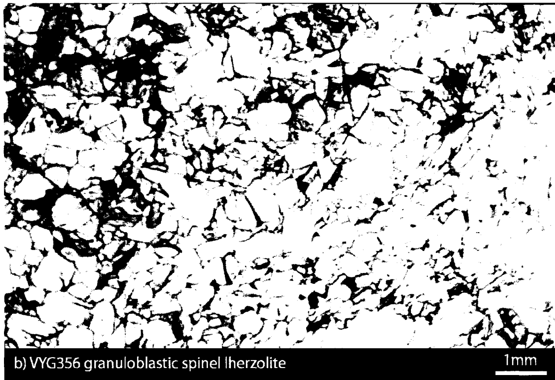
Fig. 3.2.3 Thin section images of spinel lherzolites from the Voyageur kimberlite pipe
