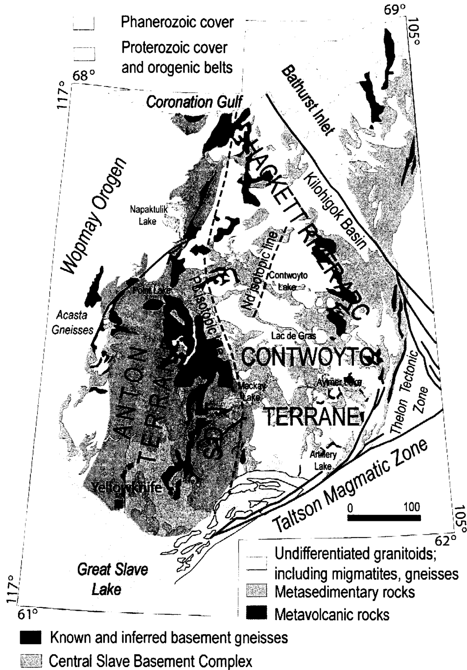
Fig. 2.1.1 Geological map of the Slave Province, Canada (modified after Davis & Bleeker, 1999). Lithotectonic terrains after Kusky (1990). Pb isotopic line from Thorpe et al. (1992), Nd isotopic line from Davis and Hegner (1992).
