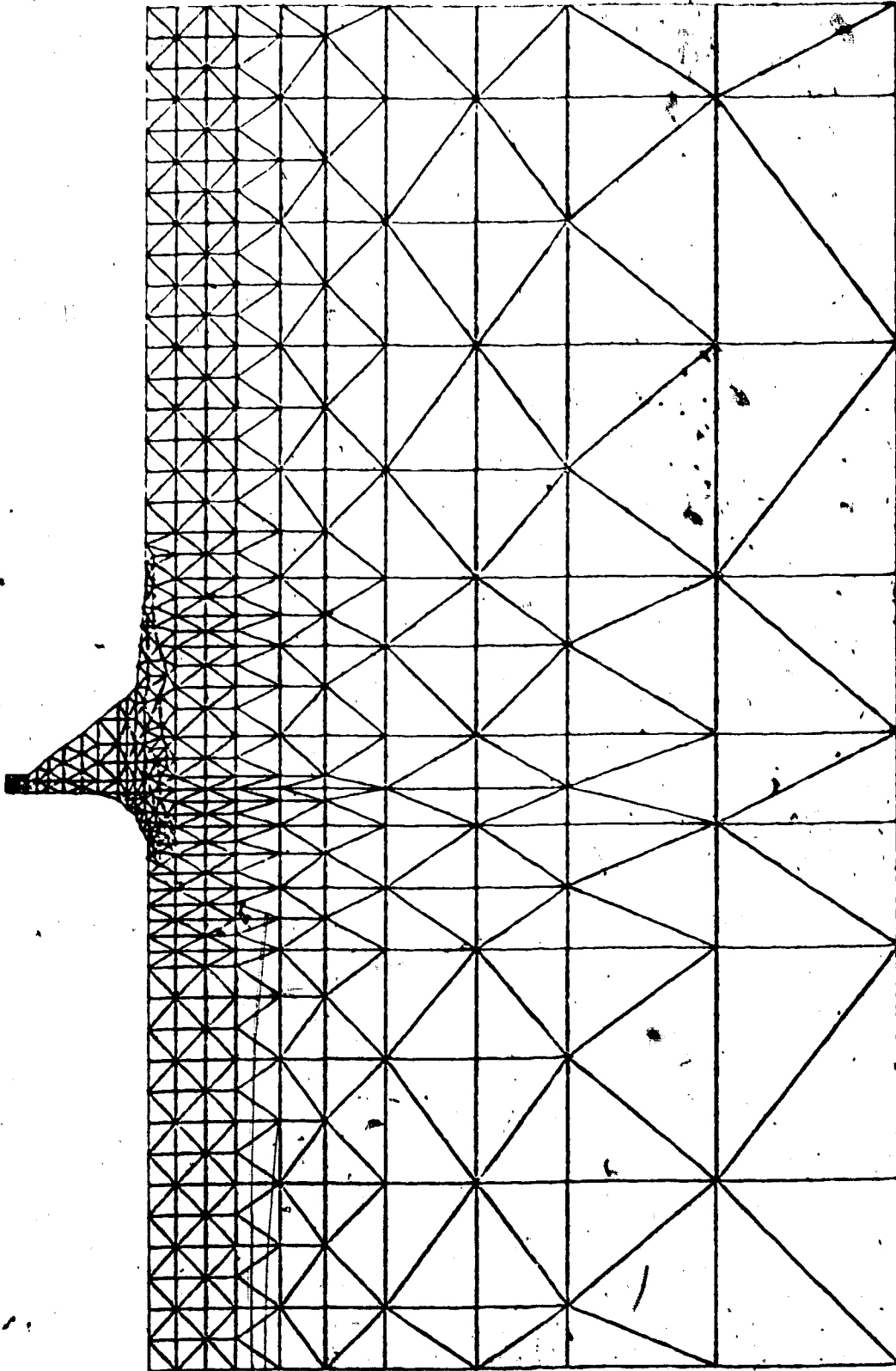
FIG. 3.5.3 FINITE ELEMENT MESH USED IN THE STUDY OF BHAKRA DAM
