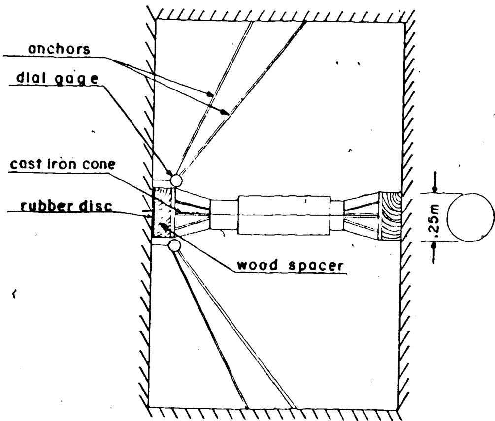
FIG. 3.4.2 JACKING TEST SET-UP
