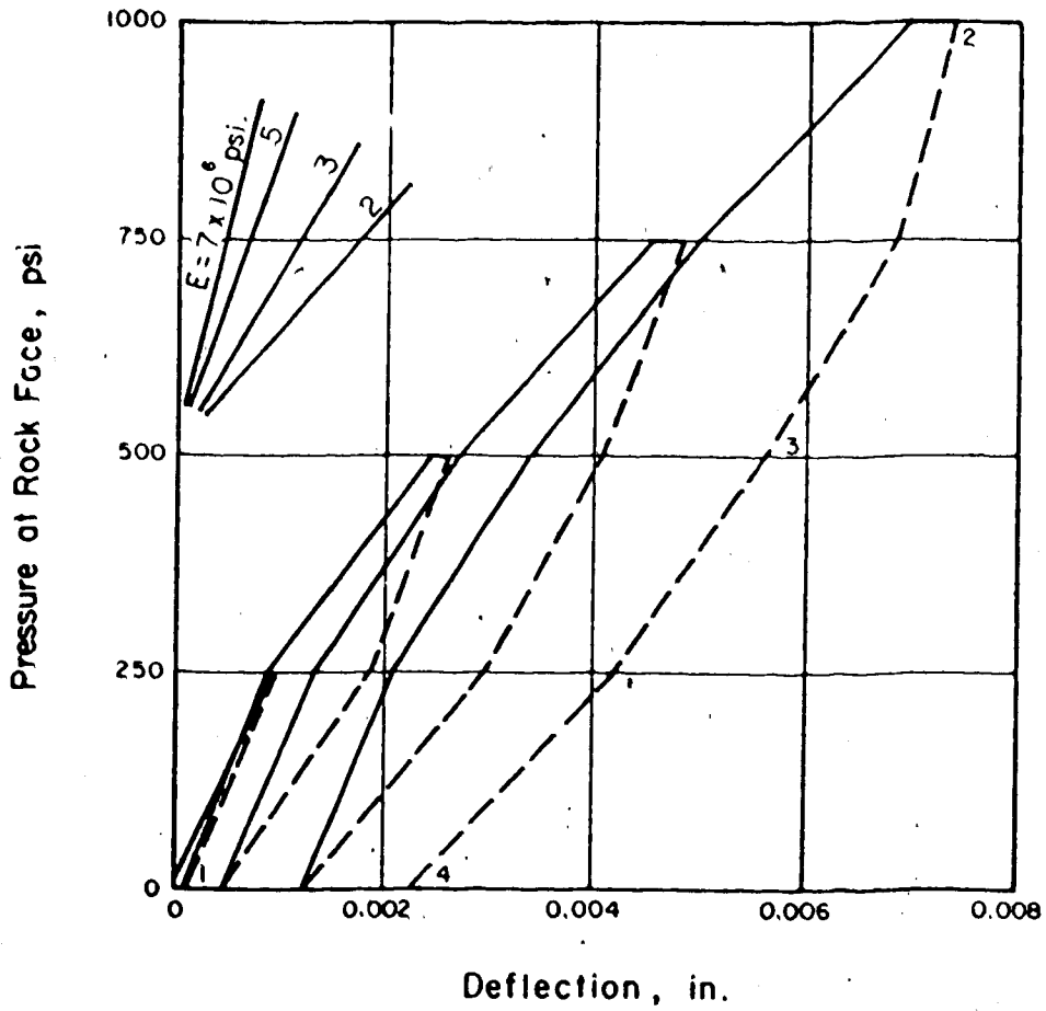
FIG. 2.1.1 REPRESENTATION OF MODULI OF DEFORMATION AND ELASTICITY. (FROM DEERE ET AL., 1969)
