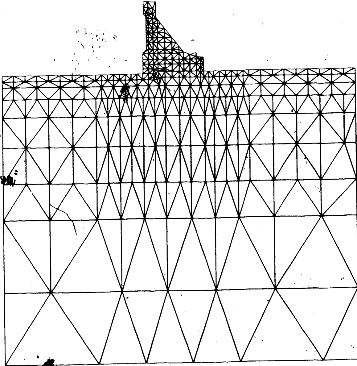
FIG. 3.3.1 FINITE ELEMENT MESH USED IN THE STUDY OF KRASNOYARSK DAM
