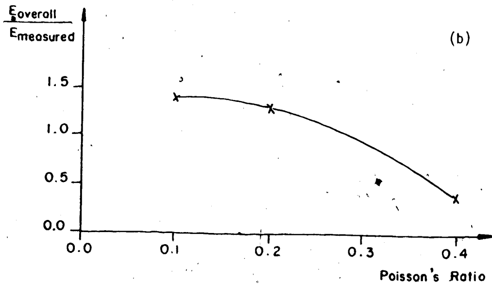
FIG. 3.5.10 INFLUENCE OF POISSON'S RATIO (a) ON THE OVERALL MODULUS OF DEFORMATION (b) ON THE \frac{E_{overall}}{E_{measured}} RATIO
