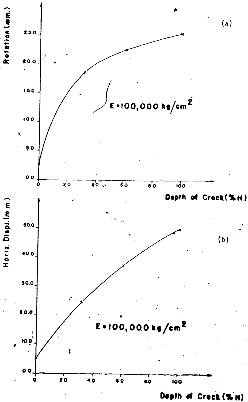
FIG. 3.4.8 (a) ROTATION OF THE FOUNDATION (VS) DEPTH OF CRACKING (b) HORIZONTAL DISPLACEMENT OF POINT 3c (VS) DEPTH OF CRACKING
