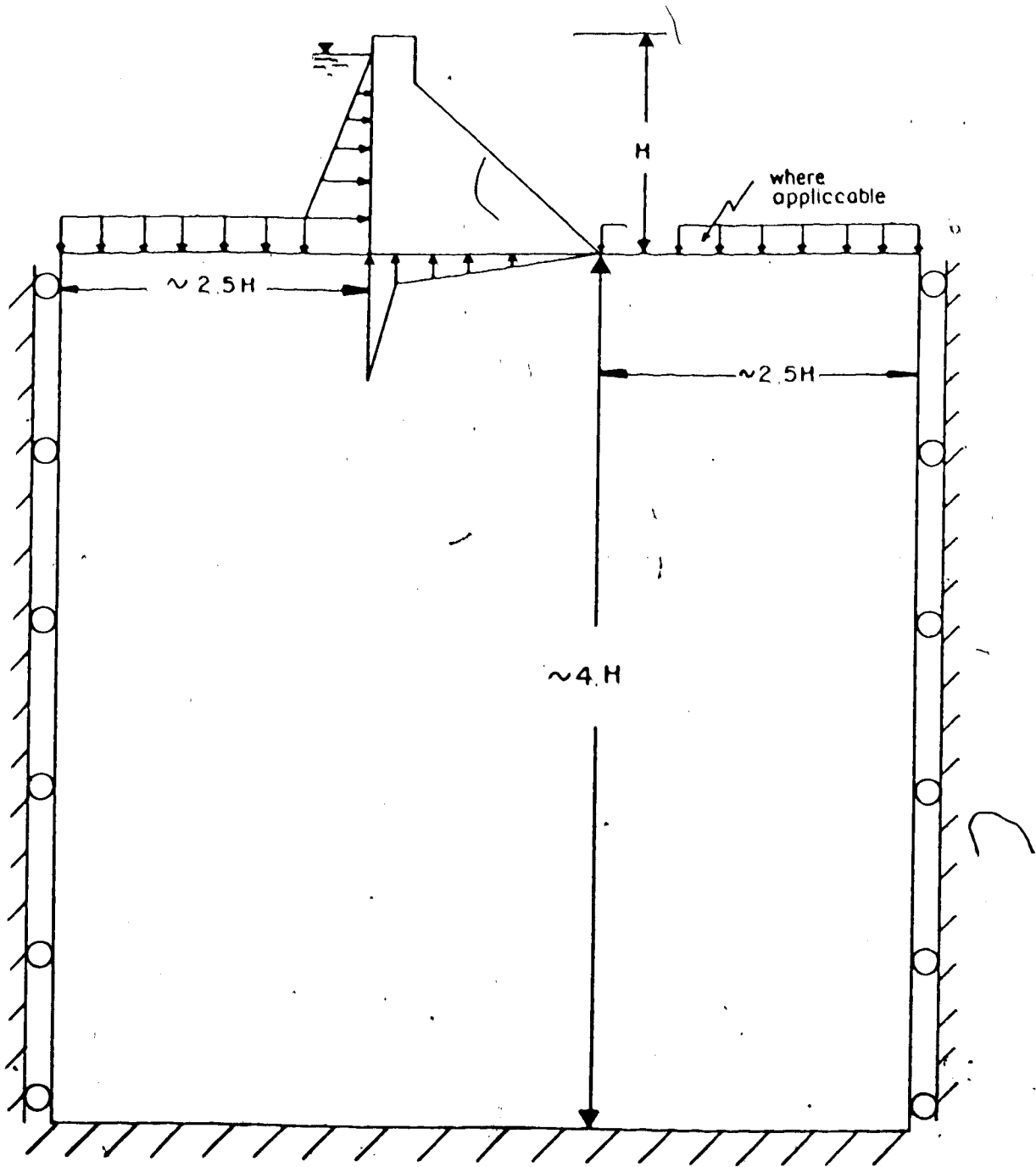
FIG. 3.2.1 BOUNDARY CONDITIONS USED IN THE ANALYSIS OF A DAM.
