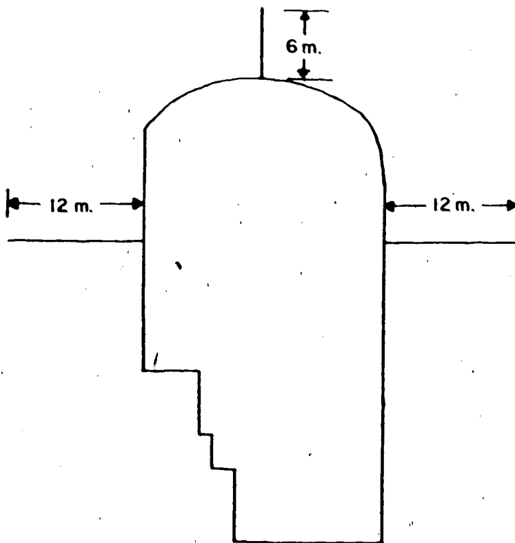
FIG. 3.7.2 RELATIVE POSITION OF EXTENSOMETERS FOR WHICH DISPLACEMENTS ARE QUOTED.
