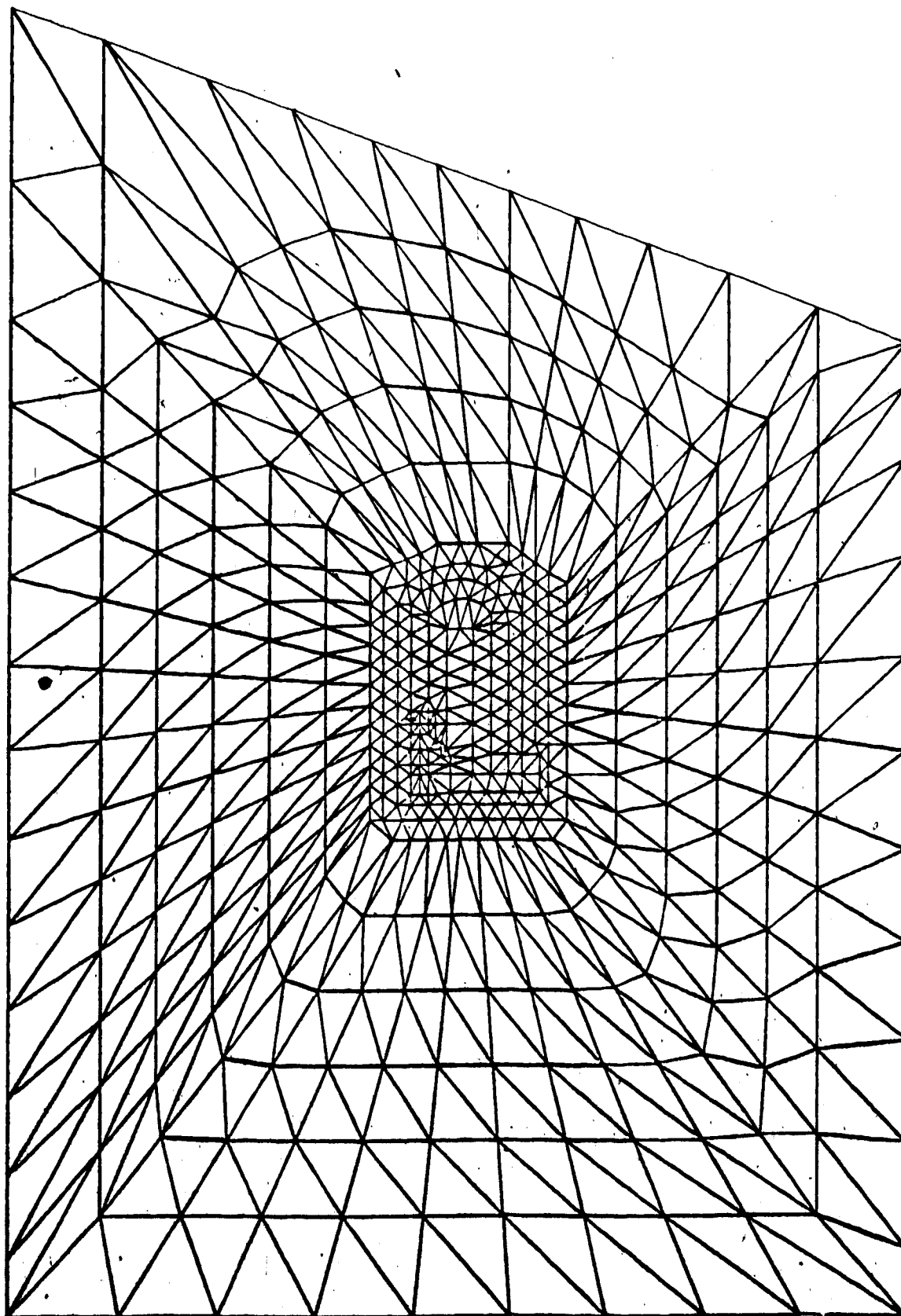
FIG. 3.7.1 FINITE ELEMENT MESH USED IN THE STUDY OF OROVILLE UNDERGROUND POWERPLANT.
