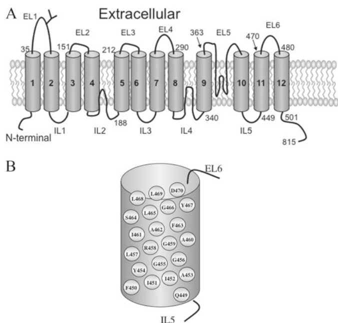
FIGURE 1. Models of the \text{Na}^+/\text{H}^+ exchanger. A, simplified topological model of the transmembrane domain of the NHE1 isoform of the \text{Na}^+/\text{H}^+ exchanger as described earlier (11). EL, extracellular loop; IL, intracellular loop. B, model of amino acids present in TM XI.
