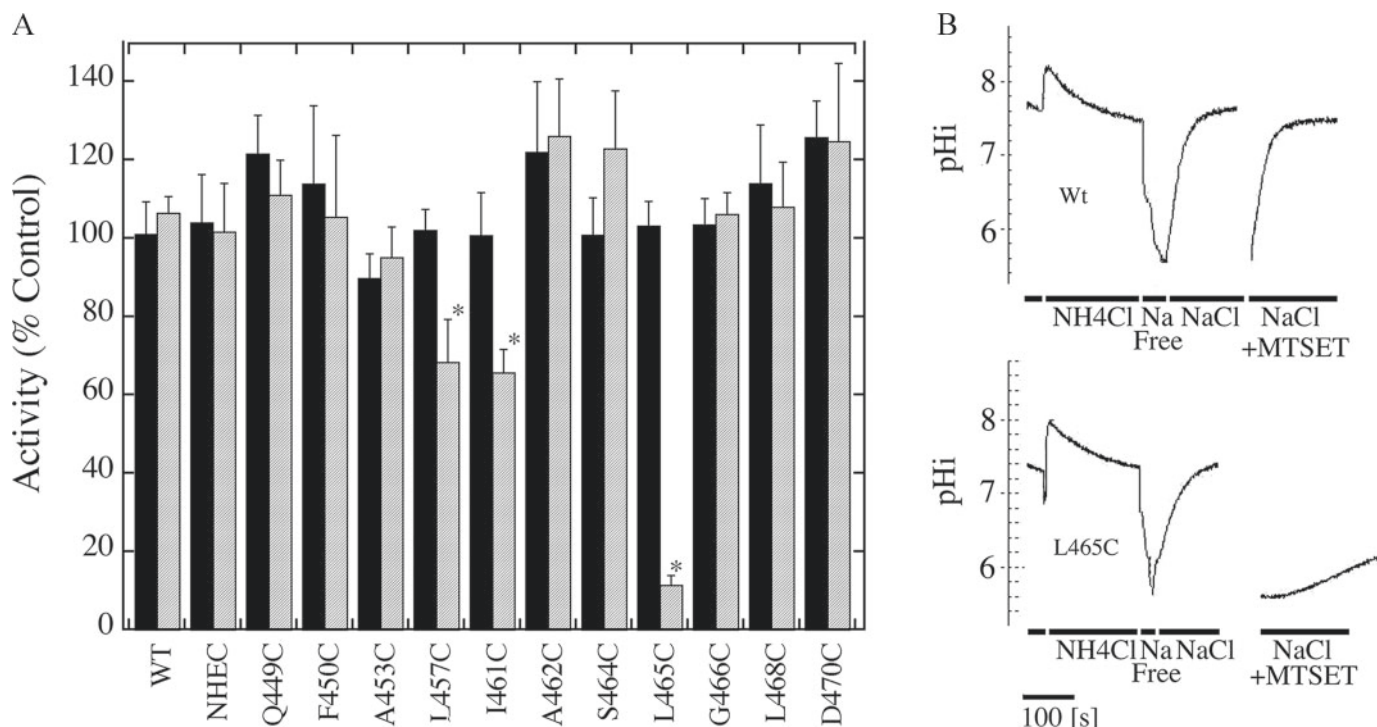
FIGURE 3. Effect of MTSET and MTSES on activity of cNHE1 and single cysteine TM XI mutant NHE1 containing cell lines. A, summary of results of \text{Na}^+/\text{H}^+ exchanger assays of active TM XI mutants. Activity was measured after two pulses of transient induction of an acid load as described under "Experimental Procedures." The first activity was in the absence of MTSES or MTSET, the second was when cells were treated with 10 mM reagent before transient acidification. Results illustrated represent the % of activity of the second acid load, in comparison to the first. * indicates that the second recovery from acid load was significantly lower than the first at p < 0.01 , Mann-Whitney U test. Solid filled bars represent MTSES treatments and hatched bars represent MTSET treatments. B, example of results of effect of MTSET on activity of wild type and L465C mutant. Wild type (Wt) and L465C NHE1 protein activity was assayed in stably transfected AP-1 cells as described under "Experimental Procedures." Activity was measured after two acid pulses as described in A. The first pulse in the absence of MTSET is shown. For ease of viewing, only the recovery from acidosis is shown for the second pulse, in which cells were treated with MTSET. NH 4 Cl, treatment with ammonium chloride; sodium free, treatment with Na + free buffer to induce acidosis; NaCl, recovery from acidosis in NaCl containing buffer, for the second pulse this contained MTSET and cells were pretreated with MTSET for 10 min prior to NH 4 Cl-induced acid load.
