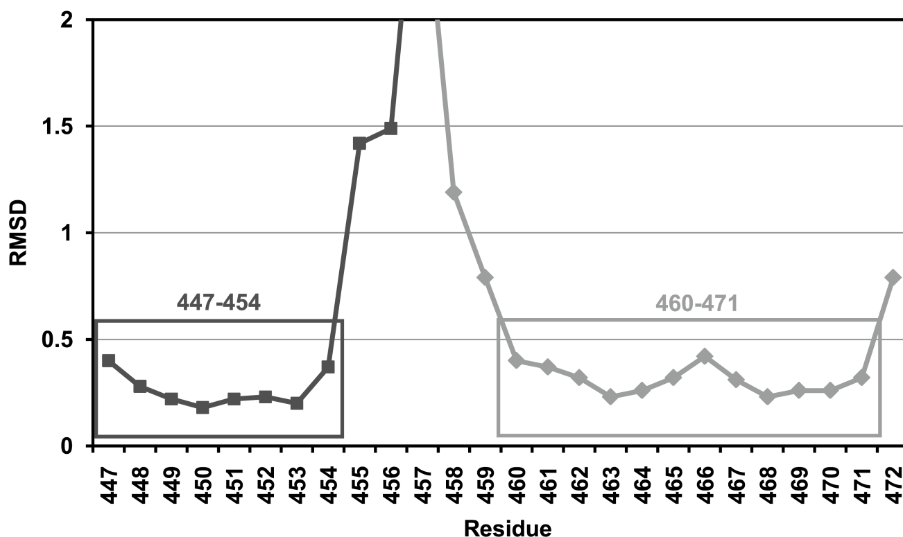
Fig. S3. Per-residue RMSD values for the optimal superimpositions of the N and C terminal helices. Superposition and RMSD calculations were performed with the LSQKAB from the CCP4 suite, and with custom scripts. Regions of the calculated ensemble of the peptide were iteratively superimposed, and resulting segments with RMSD less than 1.0 were further sorted by size and RMSD over the segment to find the optimal regions for superimposition. Per-residue RMSDs are shown for the superimpositions of the backbone atoms of Lys447-Gly454 (squares) and Gly460-Lys471 (diamonds).
