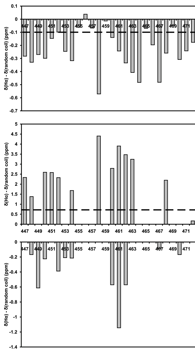
Fig. S1. Chemical shift index prediction of secondary structure. Difference between observed and random coil chemical shifts (1) for each residue in the TM XI peptide for H \alpha (top) C \alpha (center) C \beta (bottom) chemical shifts. Contiguous segments showing upfield shifts for H \alpha (greater than 0.1 ppm, dotted line) and C \beta atoms and downfield shifts for C \alpha atoms (more than 0.7 ppm) from random coil values indicate helical character. Unassigned C \alpha and C \beta atoms are given a value of zero in the figure.
