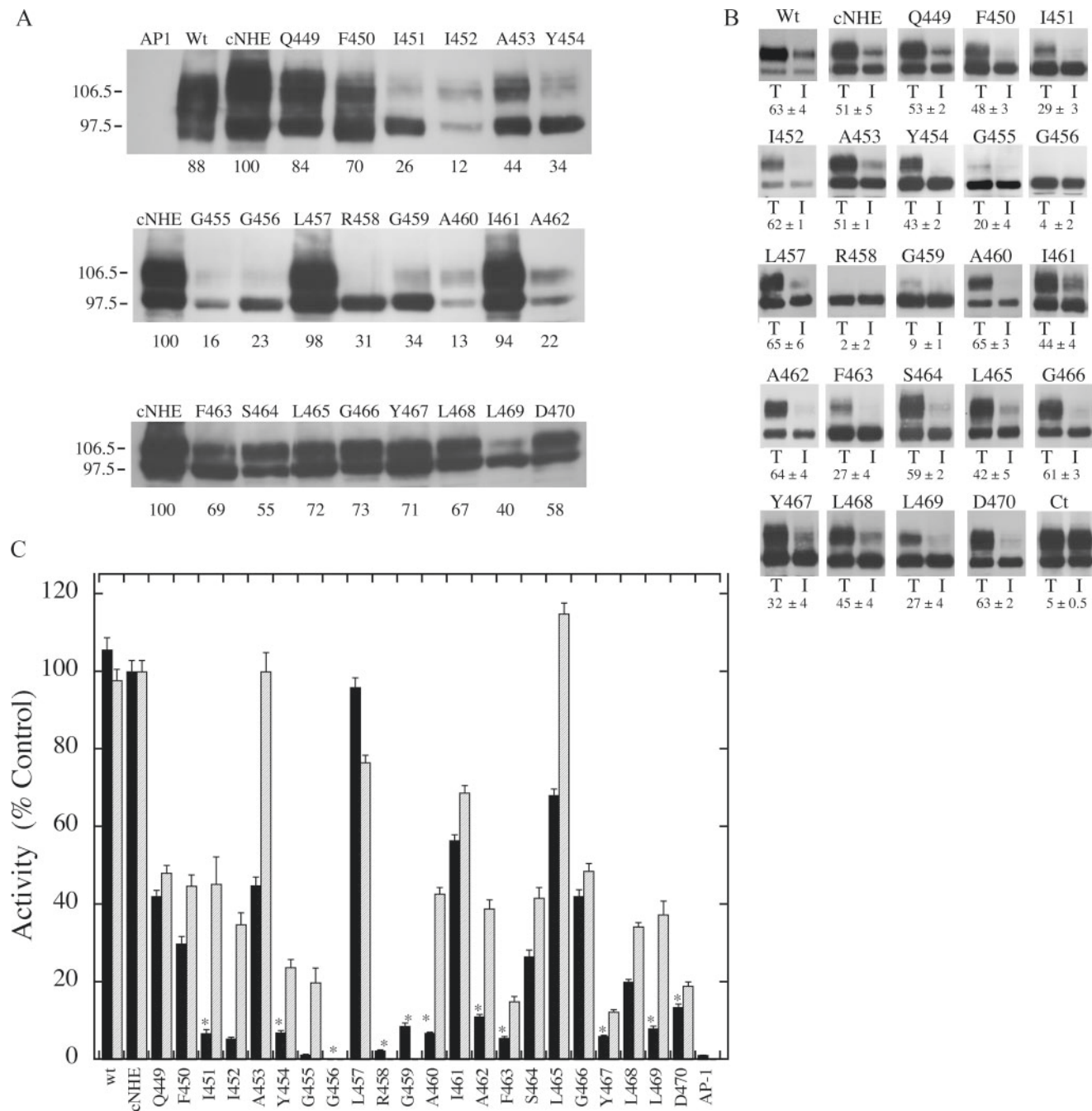
FIGURE 2. Analysis of wild type and mutant NHE1 proteins. A , Western blot of cell extracts of AP-1 cells containing stably transfected \text{Na}^+/\text{H}^+ exchanger mutants or control. In all mutations the amino acid indicated was changed to cysteine. 100 \mu\text{g} of total protein was loaded in each lane. Numbers below the lanes indicate the values obtained from densitometric scans of both the 110- and 95-kDa bands relative to wild type NHE. Results are typical of three to five measurements. AP1 refers to mock transfected AP-1 cells. Wt, refers to cells stably transfected with wild type \text{Na}^+/\text{H}^+ exchanger protein. B , subcellular localization of control and TM XI mutants in AP-1 cells. Sulfo-NHS-SS-biotin-treated cells were lysed and streptavidin-agarose beads were used to bind labeled proteins as described under "Experimental Procedures." Equal amounts of total cell lysate (T) and unbound intracellular lysate (I) were run on SDS-PAGE and Western blotting with anti-HA antibody identified NHE1 protein. Wt, refers to cells stably transfected with wild type \text{Na}^+/\text{H}^+ exchanger protein. Ct refers to a control experiment in which nonspecific binding to streptavidin-agarose beads was carried out following the standard procedure but without labeling cells with biotin. The percent of the total NHE1 protein found within the plasma membrane is indicated for each mutant. For Ct the numbers indicate the amount of nonspecific binding to streptavidin-agarose beads. Results are the mean \pm S.E. of at least three determinations. C , rate of recovery from an acid load by AP-1 cells stably transfected with cNHE, and TM XI \text{Na}^+/\text{H}^+ exchanger mutants. \text{Na}^+/\text{H}^+ exchanger activity was measured after transient induction of an acid load as described under "Experimental Procedures." The activity of cNHE1 stably transfected with NHE1 was 0.036 \Delta pH/s, and this value was set to 100%. All mutations to cysteine were done in the background of the cysteine-less NHE1 and activities are percent of those of cNHE. Mutations were in the cNHE1 and results are expressed as mean \pm S.E. of 8–16 determinations. Results are shown for mean activity of both uncorrected (black) and normalized for surface processing and expression levels (hatched). * indicates mutants with uncorrected activity that is less than 20% of cNHE1.
