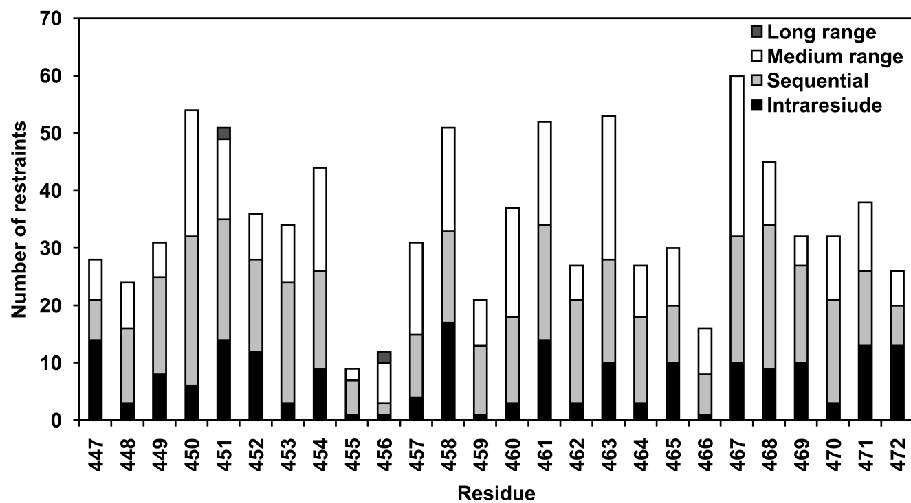
Fig. S2. (B) Summary of the number of NOE restraints per residue classified as intraresidue, sequential, medium range ( i+2 to i+4 ), and long range ( >i+4 ).
