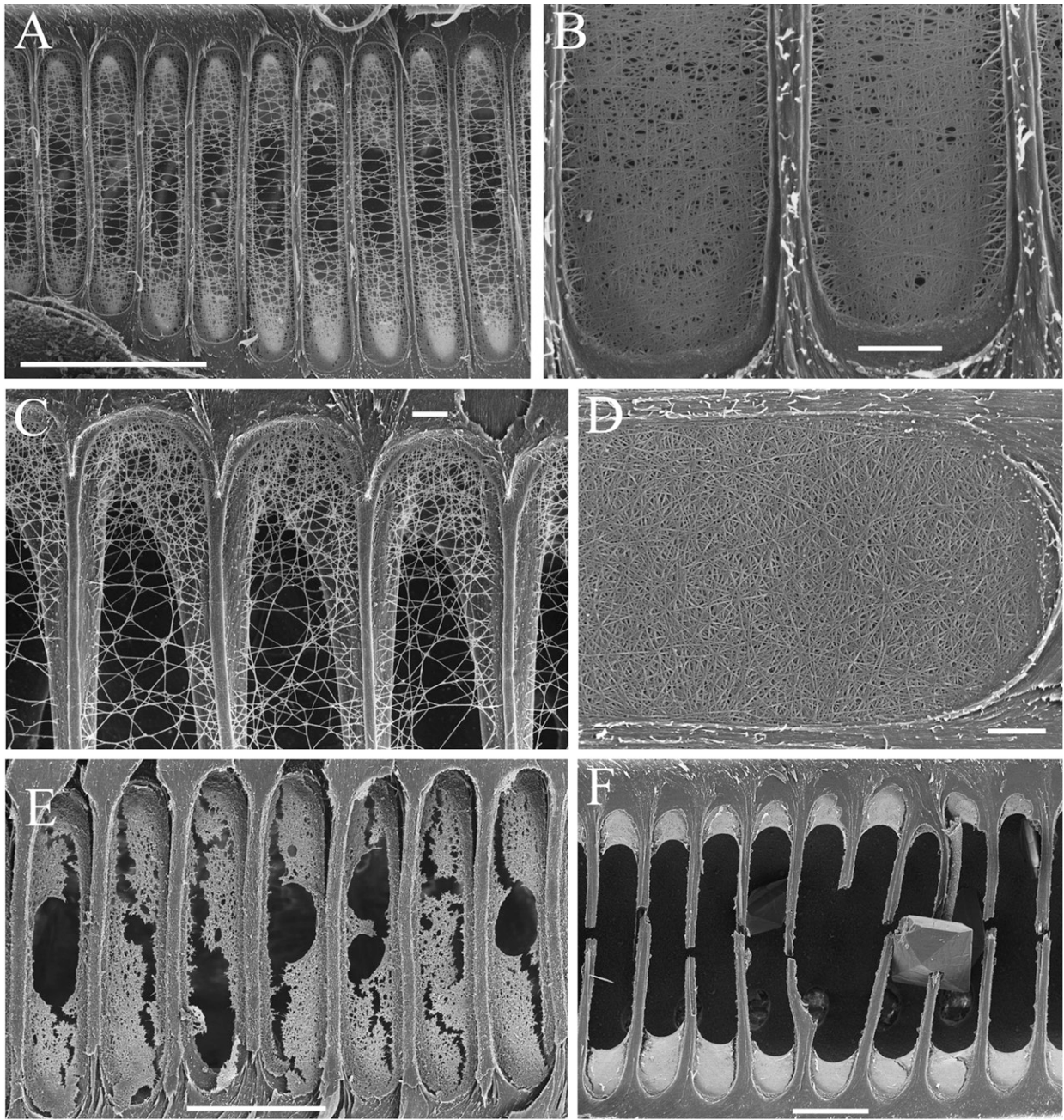
Fig. 6 SEM taken between 1600 ( F ) and 17,000 ( B ) magnification showing scalariform perforation plates ( A , C , E , F ) and inter vessel pits ( B , D ). A , Scalariform perforation plate of Illicium anisatum showing extensive pit membrane remnants. Scale bar = 10 \mu\text{m} . B , Porous inter vessel pit membrane of I. anisatum . Scale bar = 1 \mu\text{m} . C , Scalariform perforation plate of Ascarina rubricaulis laced with pit membrane remnants. Scale bar = 1 \mu\text{m} . D , Inter vessel pit of A. rubricaulis showing much less porosity than in I. anisatum above. Scale bar = 1 \mu\text{m} . E , Perforation plate of Hedyosmum goudotianum with extensive pit membrane remnants (cracked) and also with large elliptical openings. Scale bar = 10 \mu\text{m} . F , Perforation plate of Trimenia neocaledonica with pit membrane remnants confined to the edges, suggesting large elliptical openings. Note crystal surrounding one bar. Scale bar = 10 \mu\text{m} .
