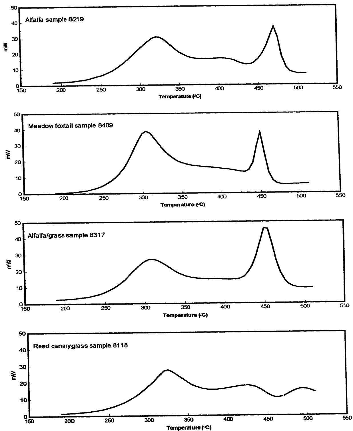
Figure 3.3. Four example DSC curves of hay samples (5.0 mg sample weight; 90.8- 92.0% DM).
