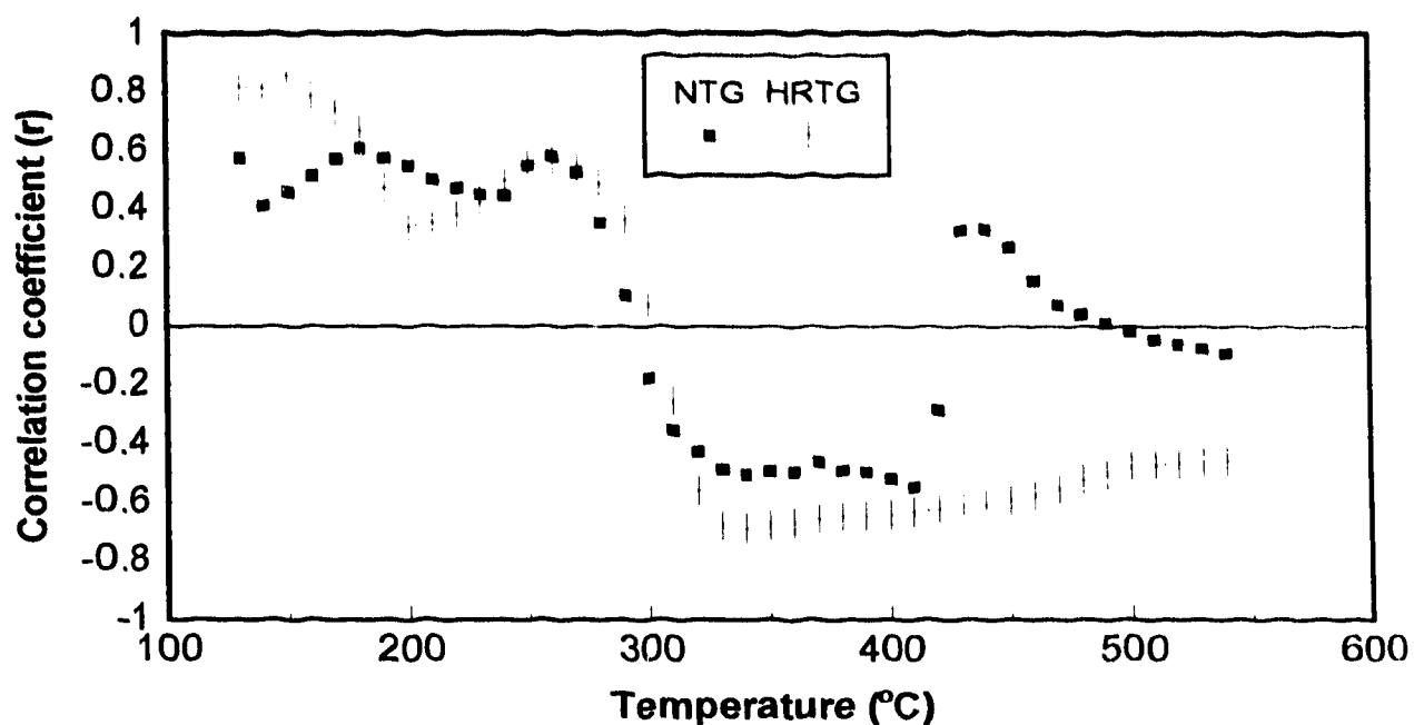
Figure 7.1. Correlation between neutral detergent fibre and normal and high resolution TG residual weights at each temperature for all 18 hay samples.
