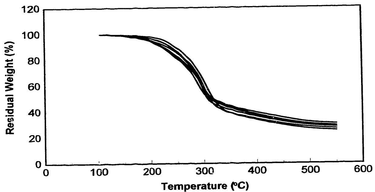
Figure 4.1. High resolution TG curves of seven alfalfa samples.
