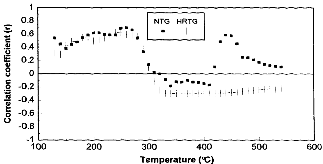
Figure 7.2. Correlation between acid detergent fibre and normal and high resolution TG residual weights at each temperature for all 18 hay samples.
