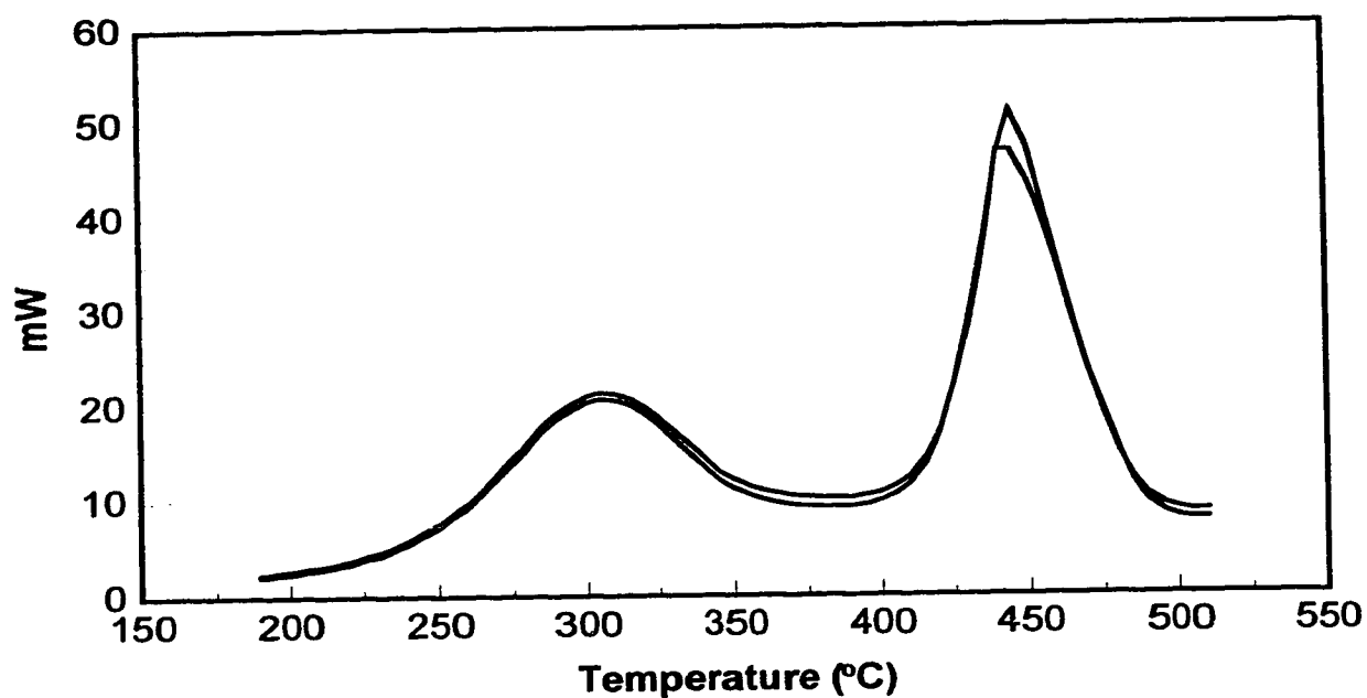
Figure 3.1. Duplicate DSC curves of alfalfa sample 8507 (5.0 mg; 90.3% DM).
