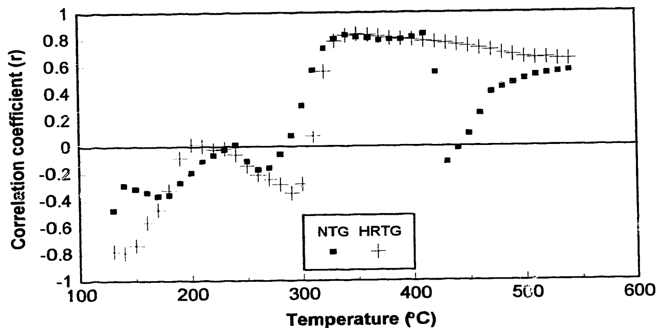
Figure 4.5. Correlation between ash and normal and high resolution TG residual weights at each temperature for all 18 hay samples.
