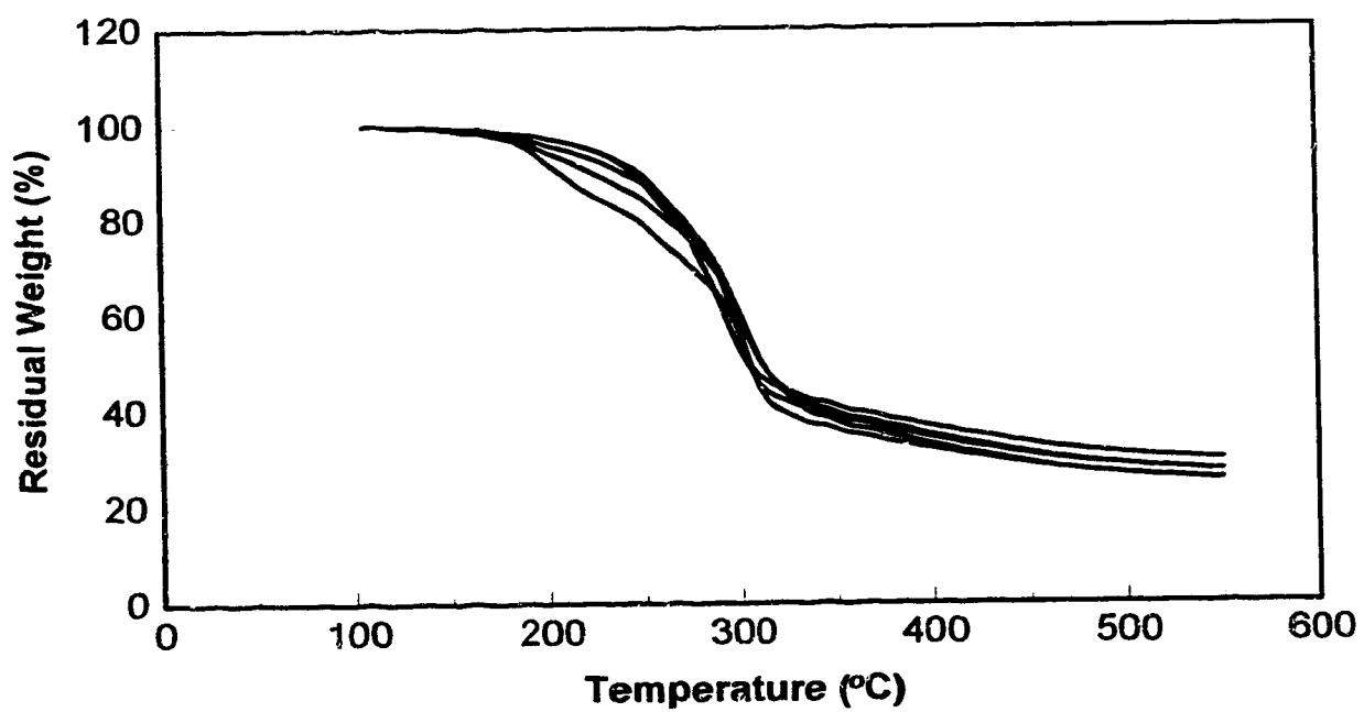
Figure 4.2. High resolution TG curves of five bromegrass samples.
