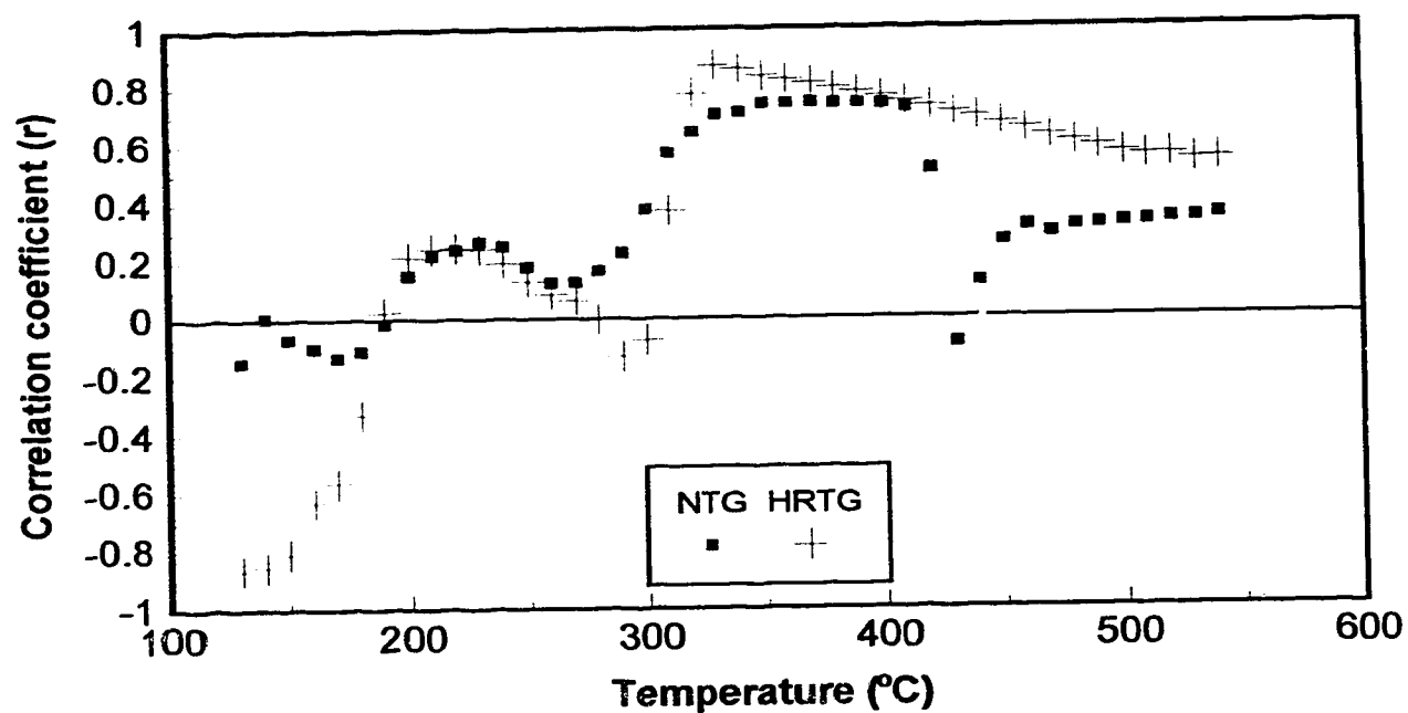
Figure 4.4. Correlation between crude protein and normal and high resolution TG residual weights at each temperature for all 18 hay samples.
