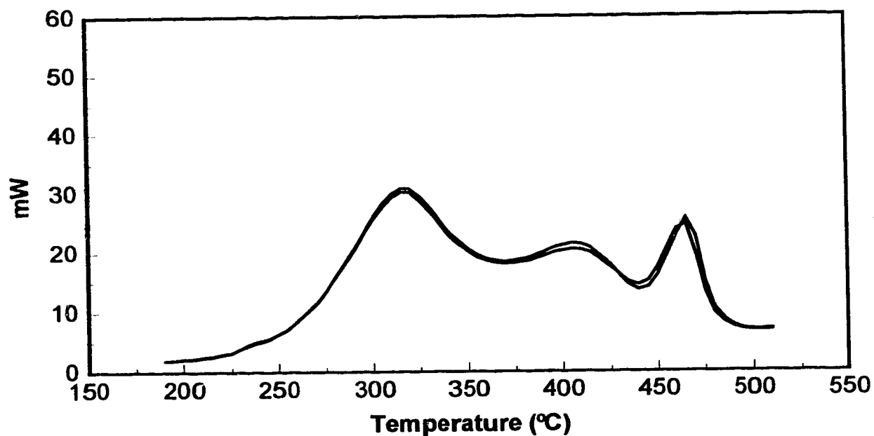
Figure 3.2. Duplicate DSC curves of timothy sample 8226 (5.0 mg; 91.9% DM).
