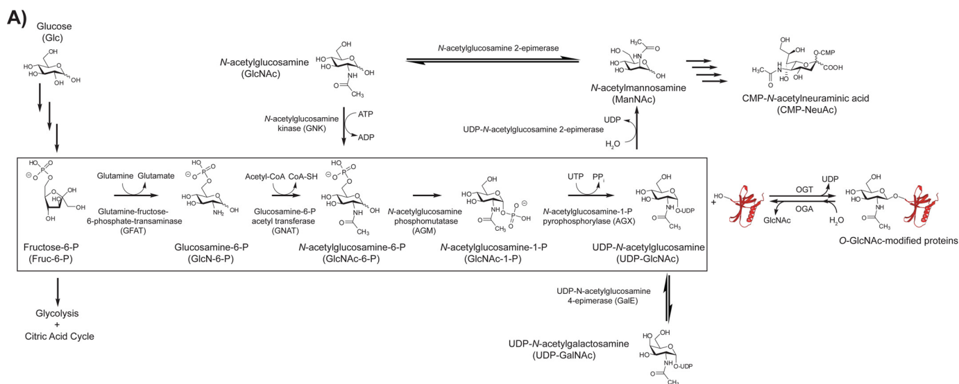
FIGURE 1. The Hexosamine biosynthetic pathway leads to the formation of UDP-GlcNAc, which is the donor substrate used by OGT to form the O-GlcNAc modification, which is in turn processed within the conserved active site pocket found in human OGA and homologs. A , O-GlcNAc consists of serine and threonine residues modified with a single \beta -O-linked N -acetylglucosamine (GlcNAc) residue. Installation of O-GlcNAc is catalyzed by OGT, which uses UDP-GlcNAc as a substrate. Removal of O-GlcNAc from modified proteins is catalyzed by OGA. UDP-GlcNAc is made from the hexosamine biosynthetic pathway (box). GlcNAc can be salvaged by phosphorylation to generate the HBSF intermediate GlcNAc-6-P. UDP-GlcNAc is also used for the biosynthesis of CMP-Neu5Ac and UDP-GalNAc. B and C , a conserved active site pocket is present around the 2-acetamido substituent in all GH84 family members. B , structure of BtGH84 with NAG-thiazoline bound in its active site (Protein Data Bank code 2CHN). Highlighted are residues that line the active site including the pocket formed beneath the 2'-methyl group of NAG-thiazoline. C , sequence alignment of several GH84 family members. Residues in boldface are those that line the active site pocket. Note that Asp-242, Phe-240, Thr-310, and Val-314 are not noted in B because they are either out of plane (into the page) or obscured.
