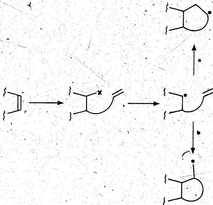
Scheme 7
