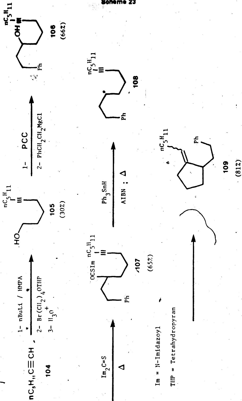
Scheme 23
