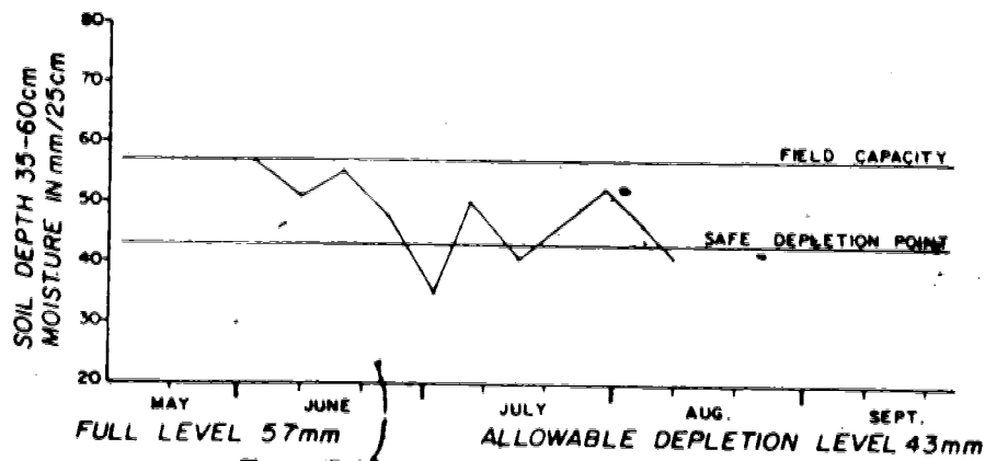
Figure 13(b) Soil moisture change in the 35-60cm zone
