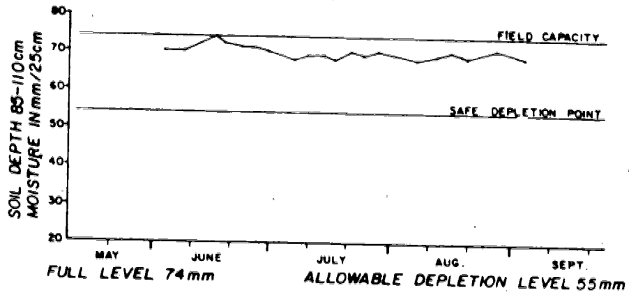
Figure II(d) Soil moisture change in the 85-110cm zone
