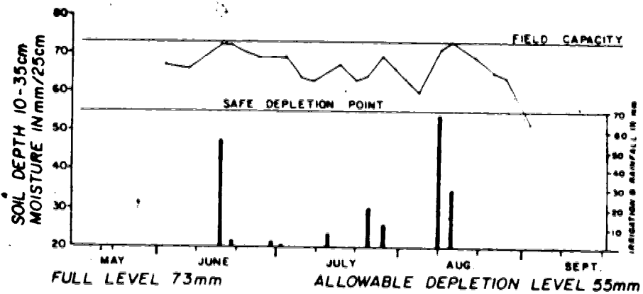
Figure 10(a) Soil moisture change in the 10-35cm zone
