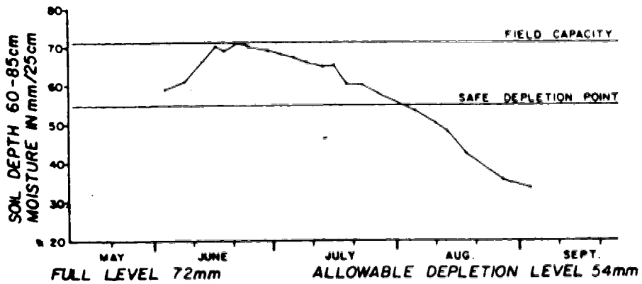
Figure 9(c) Soil moisture change in the 60-85cm zone
