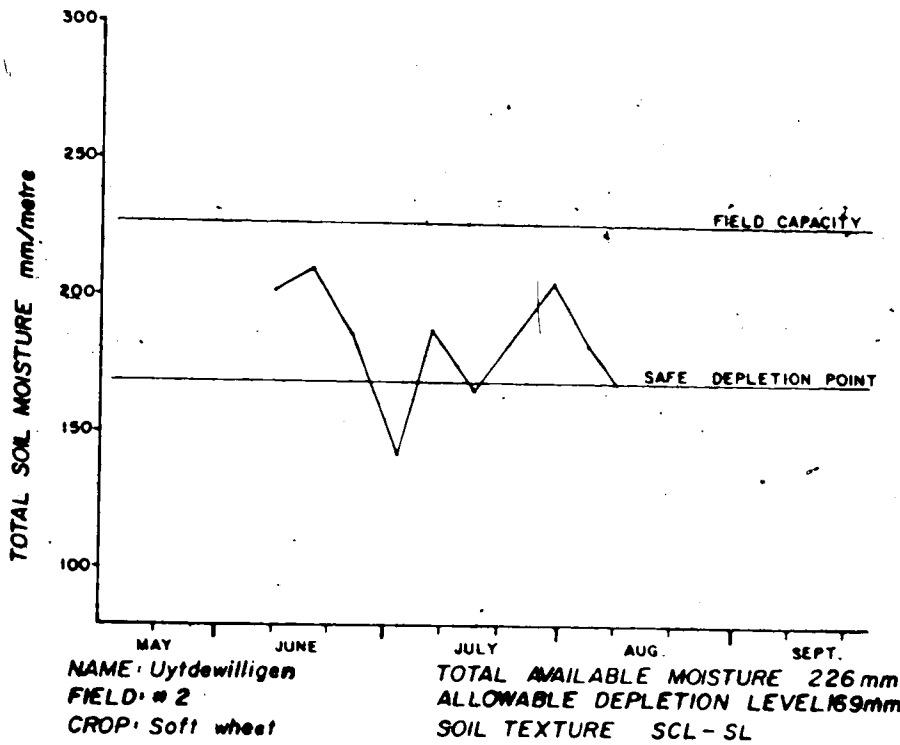
Figure 13(e) Soil moisture change in the total soil profile
