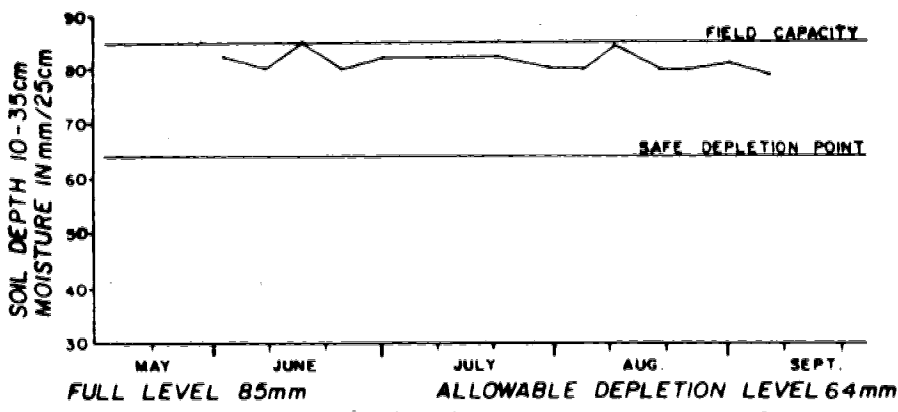
Figure 15(a) Soil moisture change in the 10-35cm zone
