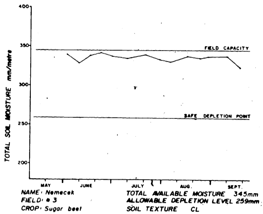
Figure 15(a) Soil moisture change in the total soil profile. Figure 15 Soil moisture change in a sugar beet field irrigated with a pivot system.
