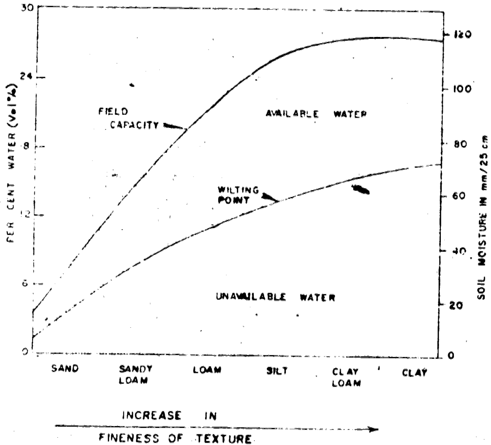
FIGURE 1 RELATIONSHIP BETWEEN SOIL MOISTURE AND SOIL TEXTURE SOURCE: BUCKMAN AND BRADY, 1972
