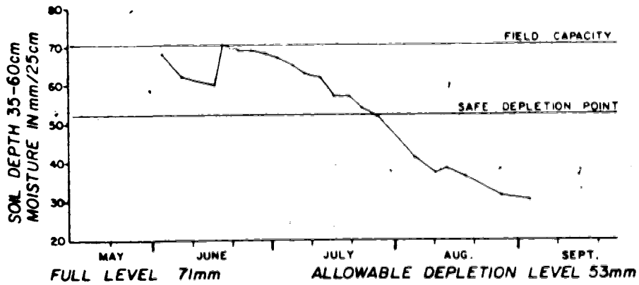
Figure 9(b) Soil moisture change in the 35-60cm zone
