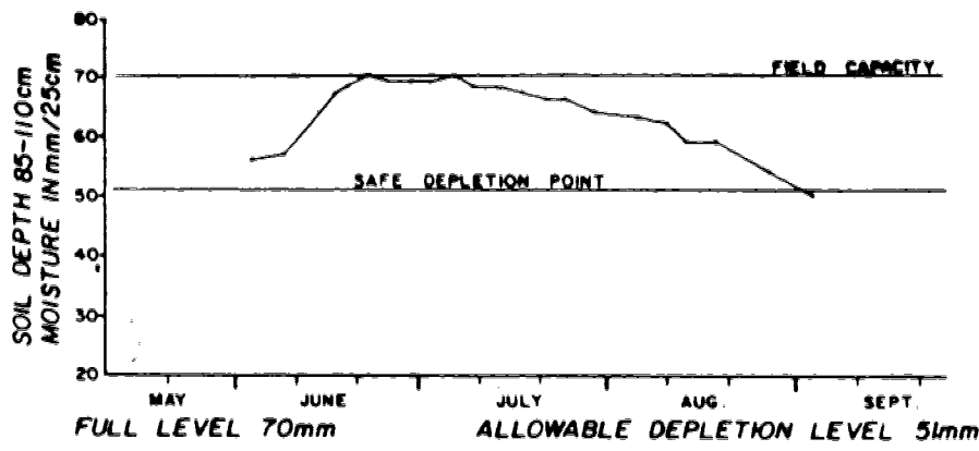
Figure 9(d) Soil moisture change in the 85-110cm zone
