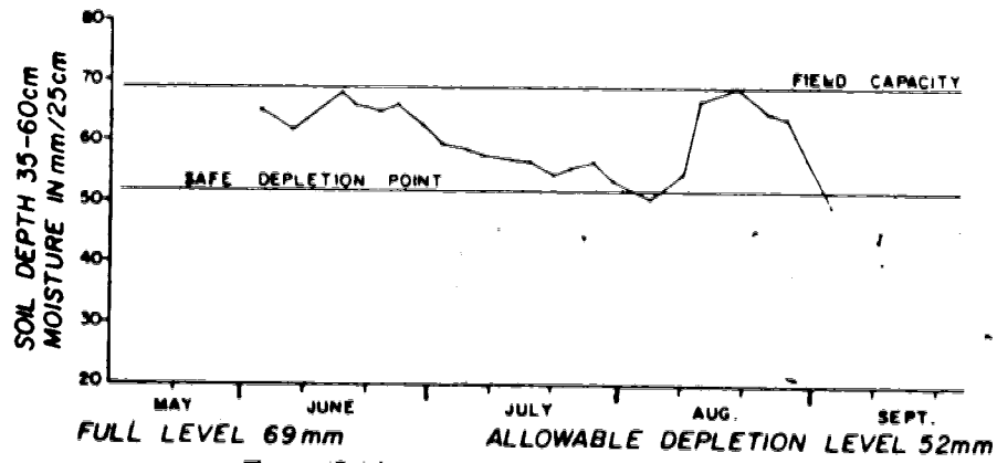
Figure 10(b) Soil moisture change in the 35-60cm zone
