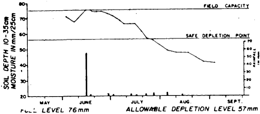
Figure 9(a) Soil moisture change in the 10-35cm zone
