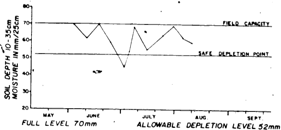
Figure 13(a) Soil moisture change in the 10-35cm zone
