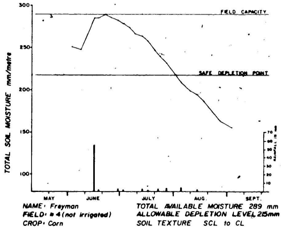
Figure 9(e) Soil moisture change in the total soil profile Figure 9 Soil moisture change in a non-irrigated corner of a corn field.
