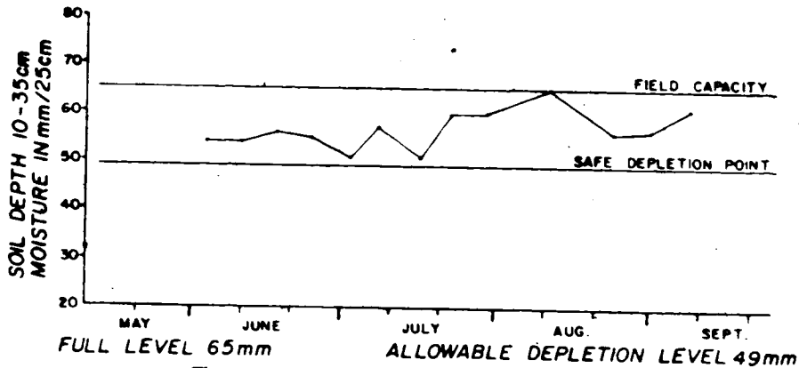
Figure 14(a) Soil moisture change in the 10-35cm zone
