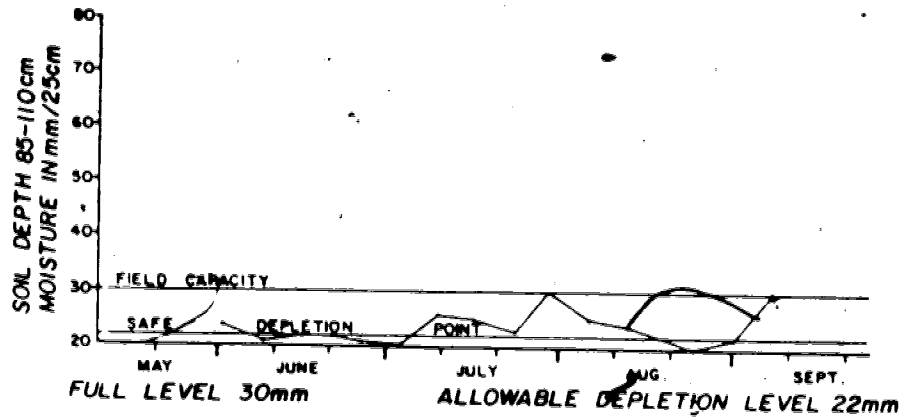
Figure 12(d) Soil moisture change in the 85-110cm zone
