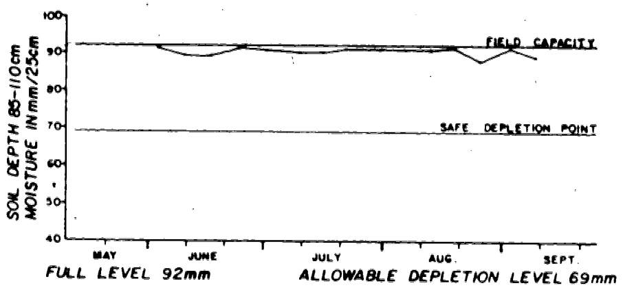
Figure 15 (p) Soil moisture change in the 85-110cm zone
