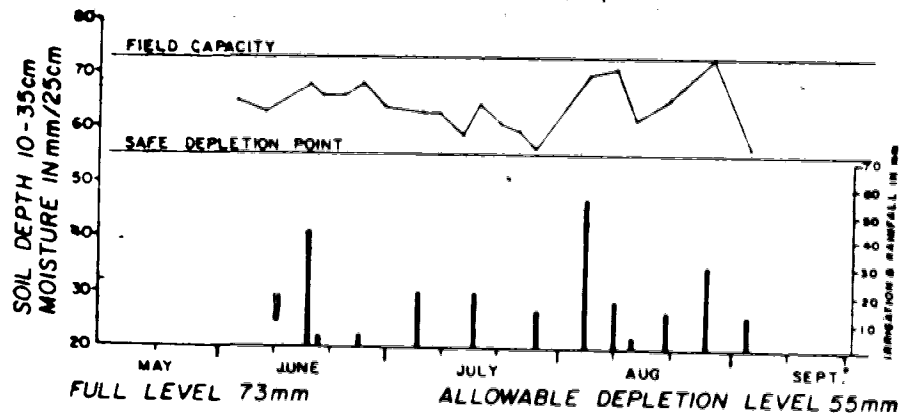
Figure II(a) Soil moisture change in the 10-35cm zone
