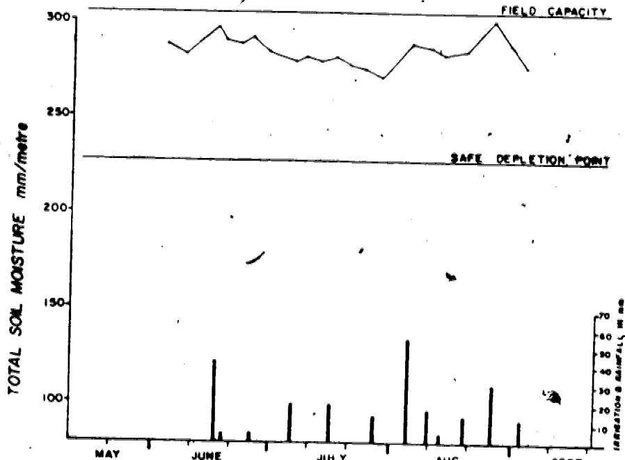
Figure II(d) Soil moisture change in the 85-110cm zone
