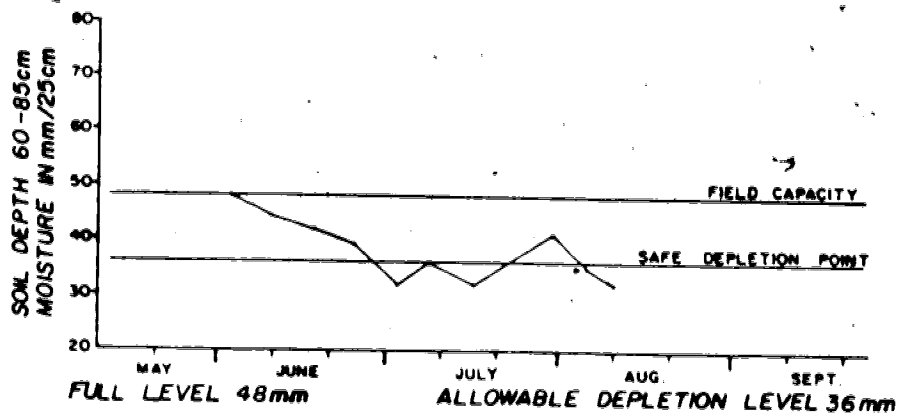
Figure 13(c) Soil moisture change in the 60-85cm zone
