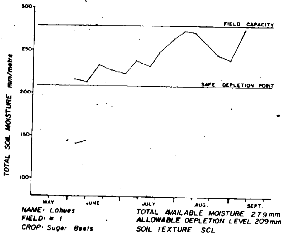
Figure 14(e) Soil moisture change in the total soil profile Figure 14 Soil moisture change in a sugar beet field with a wheel move irrigation system.
