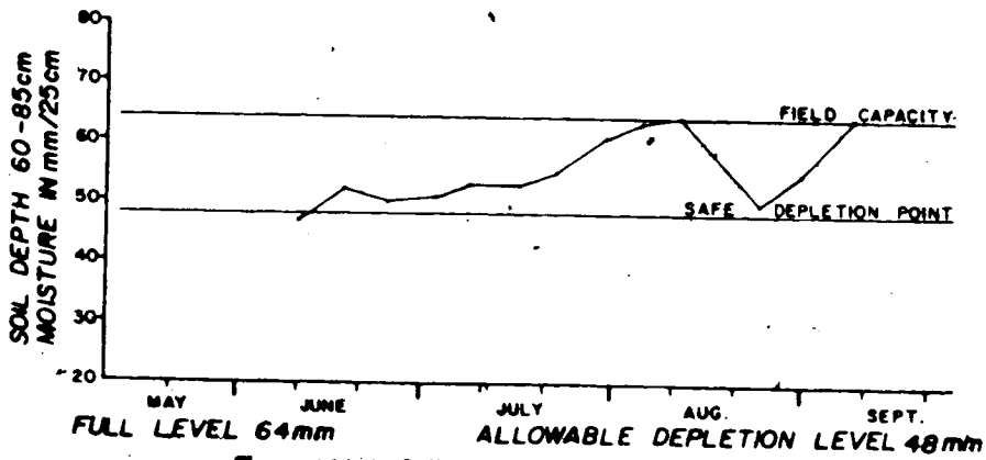
Figure 14(c) Soil moisture change in the 60-85cm zone
