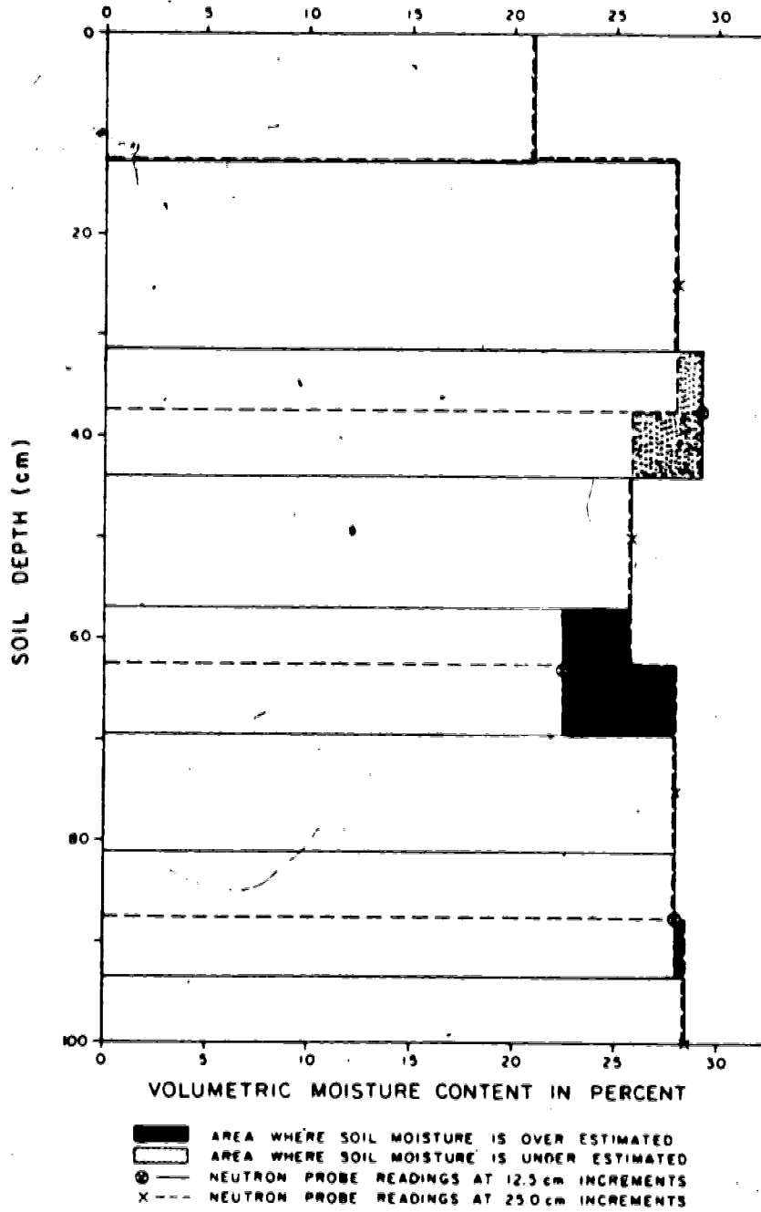
FIGURE 18 BAR GRAPH SHOWING MAXIMUM SOIL MOISTURE VARIATION BETWEEN 4 AND 7 READINGS PER SITE
