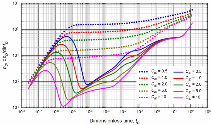
Figure 2-20. Pressure responses of the irregular-shaped horizontal fracture (shown in Figure 2-19) with different dimensionless fracture conductivities.
