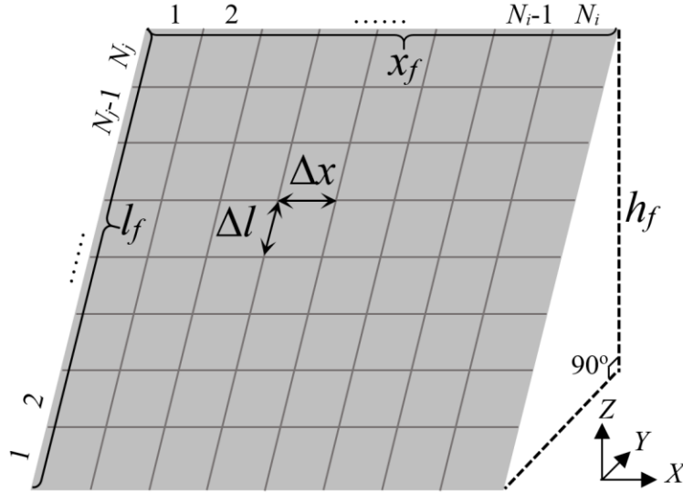
Figure 3-3. Discretization of the PPIF along both the horizontal axis and inclined axis.
