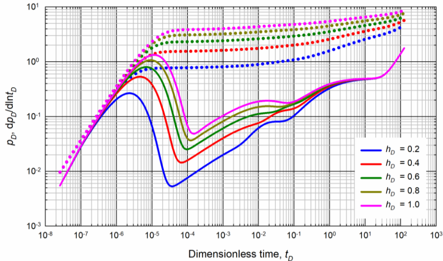
Figure 2-11. Impact of formation thickness on the pressure drops and their derivatives of a circular horizontal fracture. When h_D = 0.4 , the early pseudo-radial flow of first and a “dip” can be observed on the pressure derivative plot.
