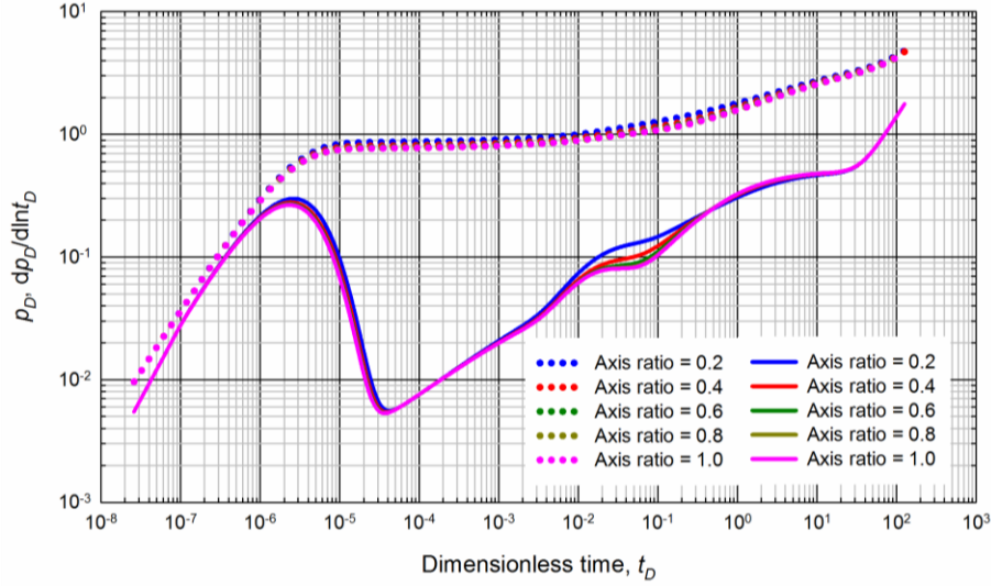
Figure 2-15. Impact of the axis ratios of the elliptical fracture on the pressure drops and their derivatives
