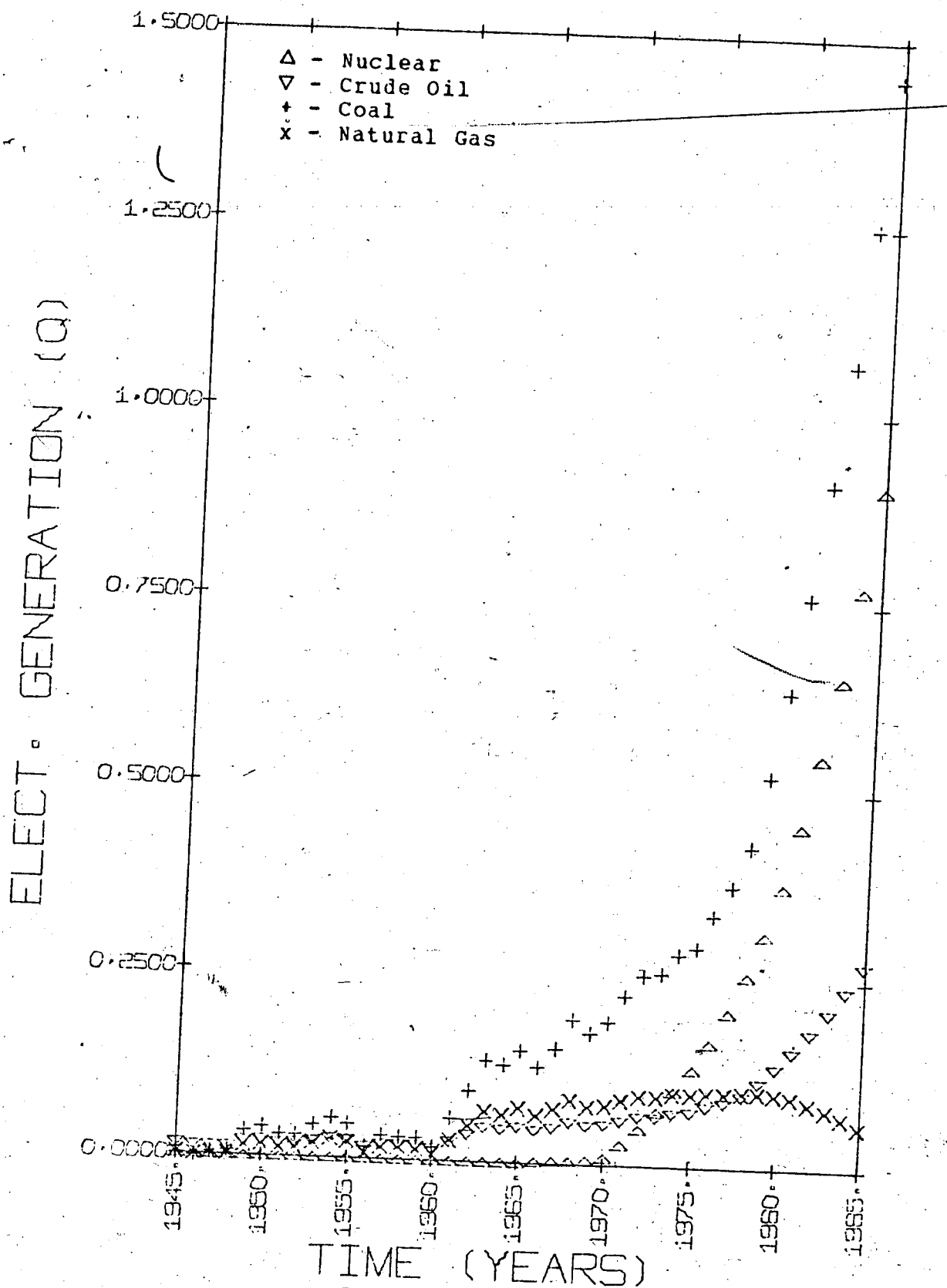
FIGURE IV.49 - ELECTRICITY GENERATED FROM PRIMARY FUEL FORMS, CASE III 1945-85.
