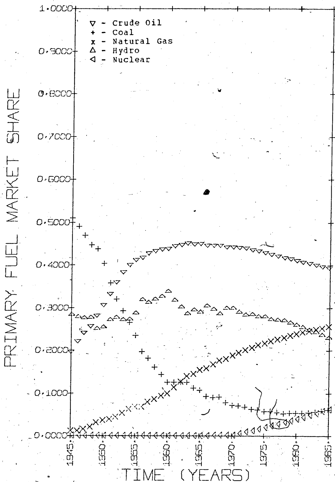
FIGURE IV.38 + PRIMARY FUEL MARKET SHARES FOR TOTAL CANADIAN ENERGY CONSUMPTION, CASE II 1945-85.
