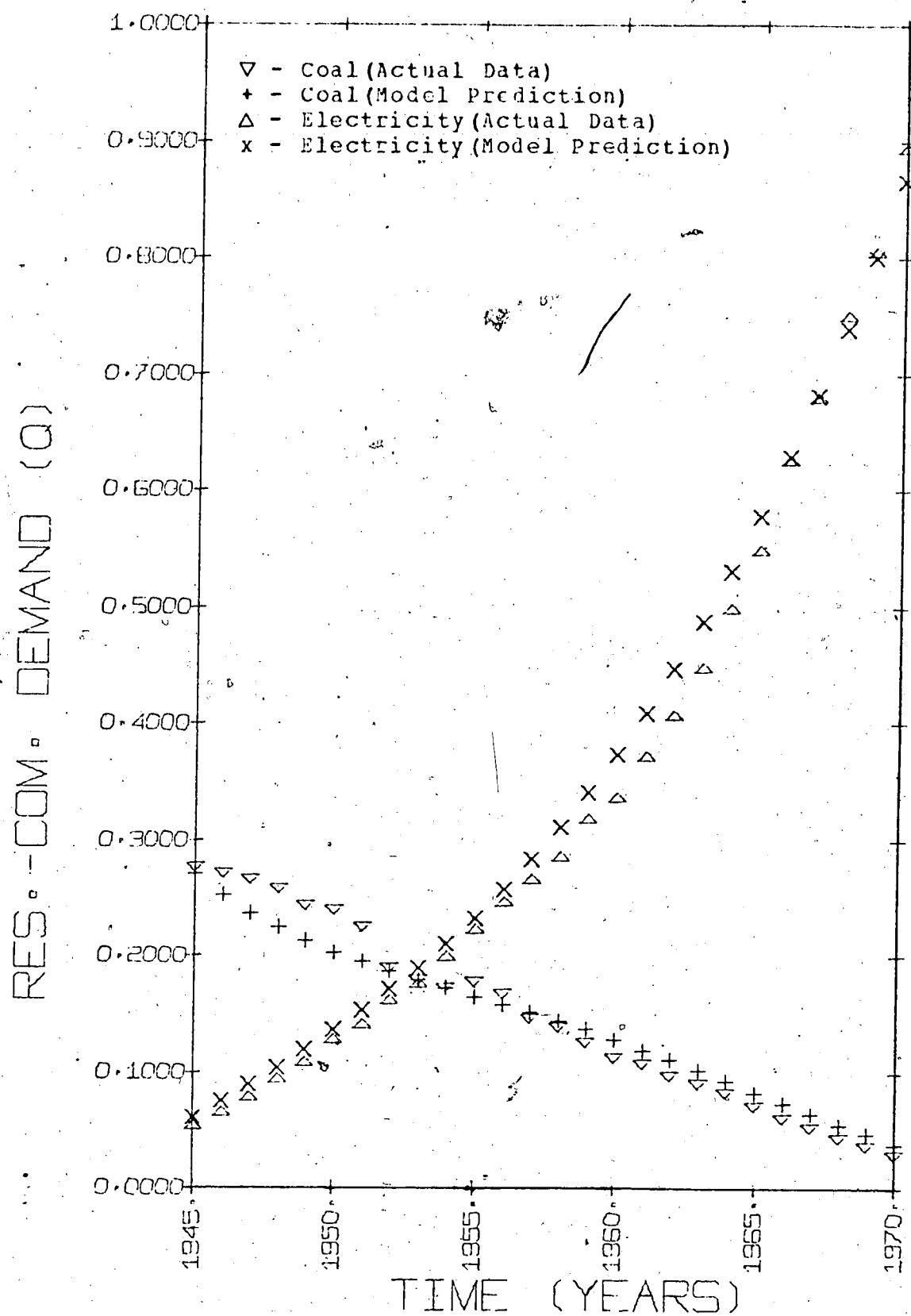
FIGURE IIT.8 - RESIDENTIAL-COMMERCIAL ENERGY DEMAND, BASE CASE 1945-70.
