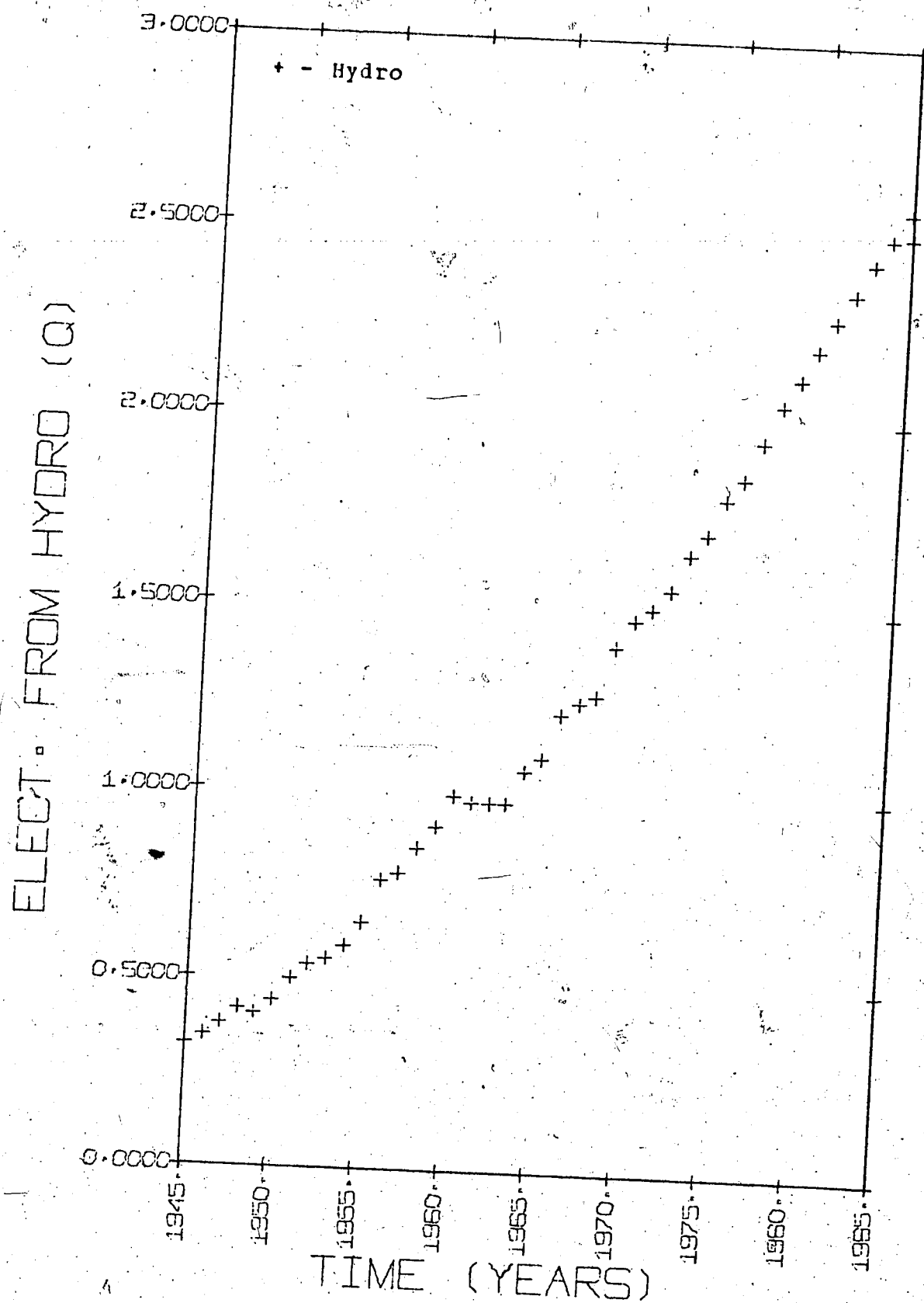
FIGURE IV.36 - ELECTRICITY GENERATED FROM HYDRO, CASE II 1945-85.
