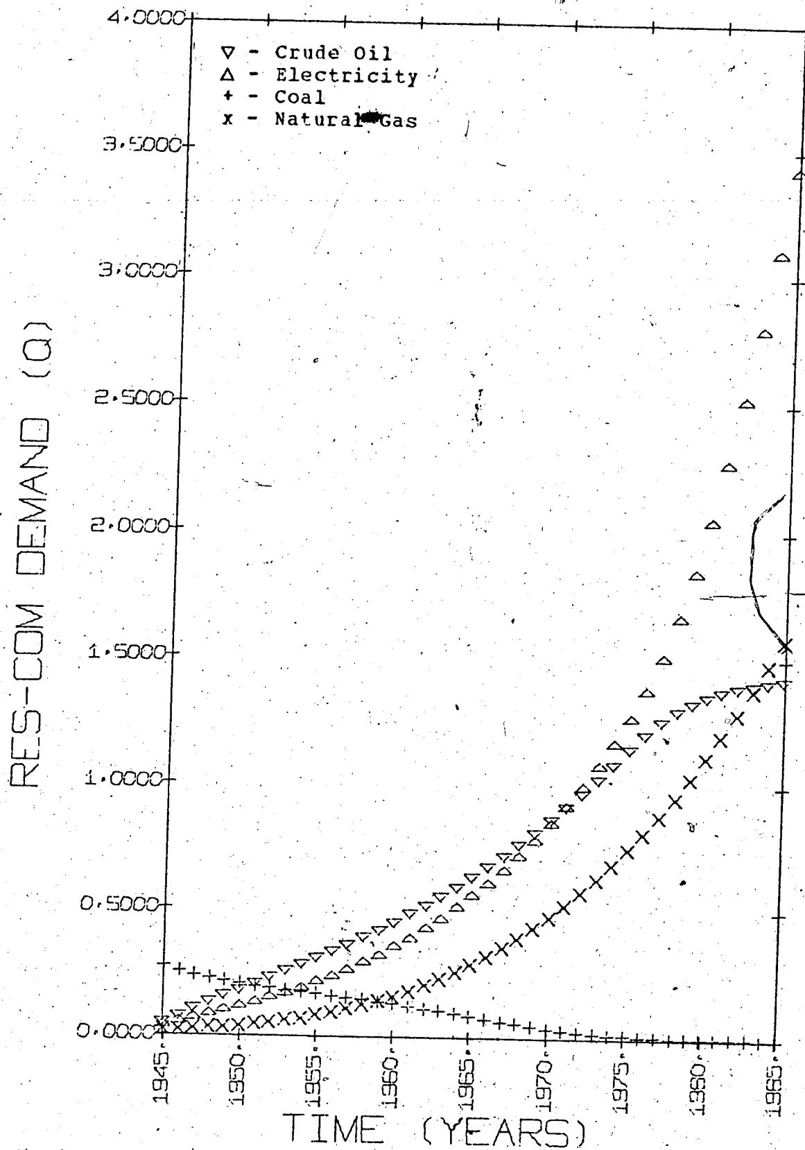
FIGURE IV.46 - RESIDENTIAL-COMMERCIAL DEMAND, CASE III 1945-85.
