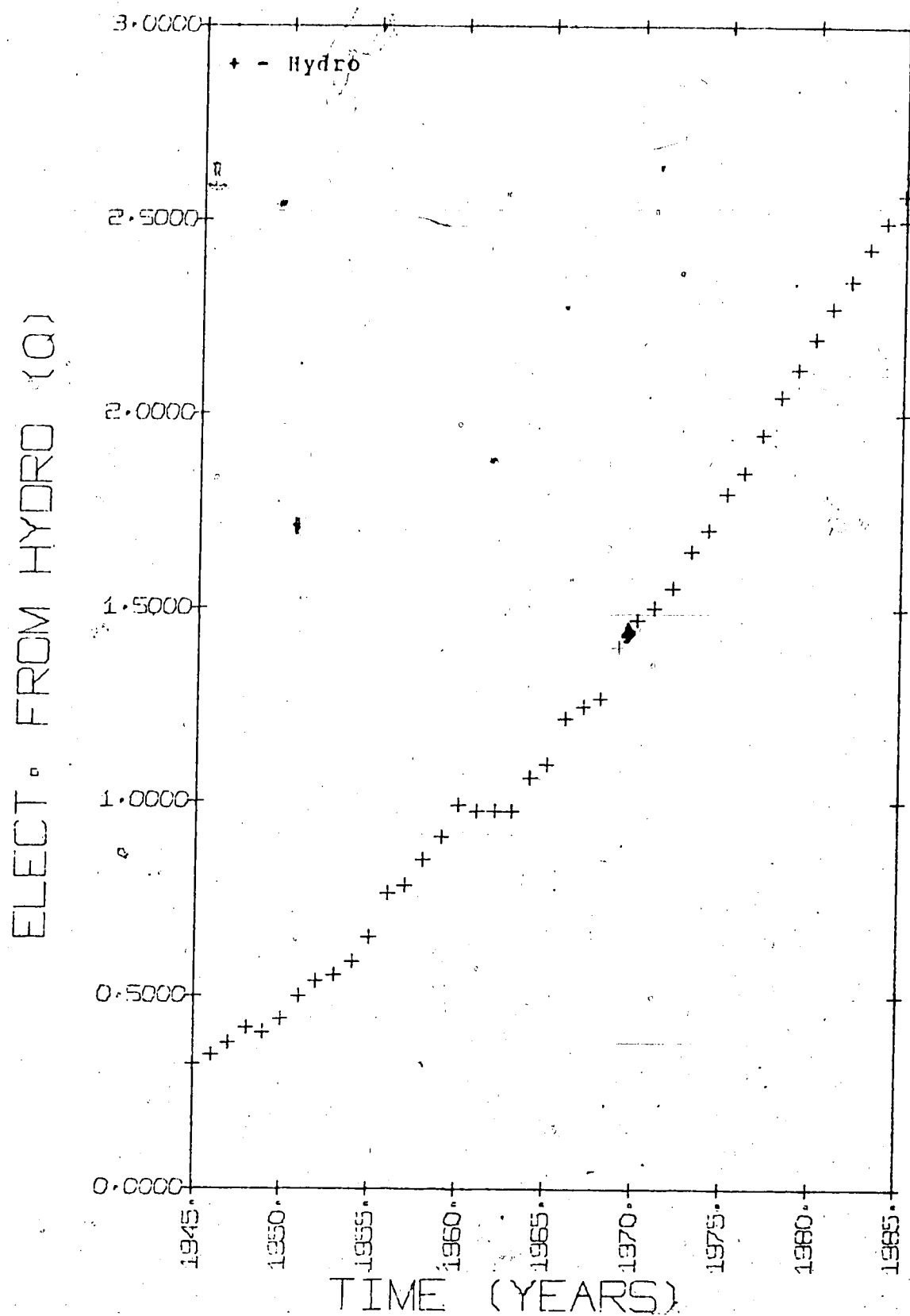
FIGURE IV.18 - ELECTRICITY GENERATED FROM HYDRO, CASE-I 1945-85.
