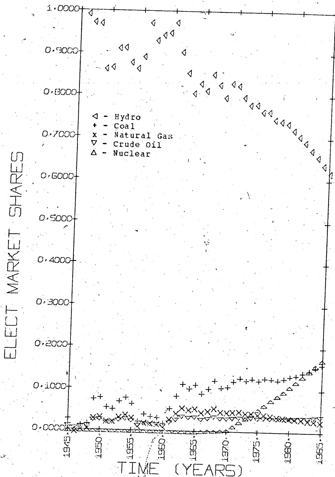
FIGURE IV.37 - PRIMARY FUEL MARKET SHARES IN THE ELECTRICITY GENERATING SECTOR, CASE II 1945-85.
