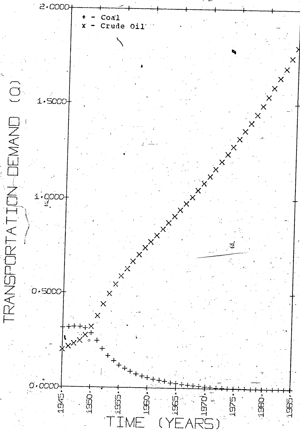
FIGURE IV.33 - TRANSPORTATION DEMAND, CASE II 1945-85.
