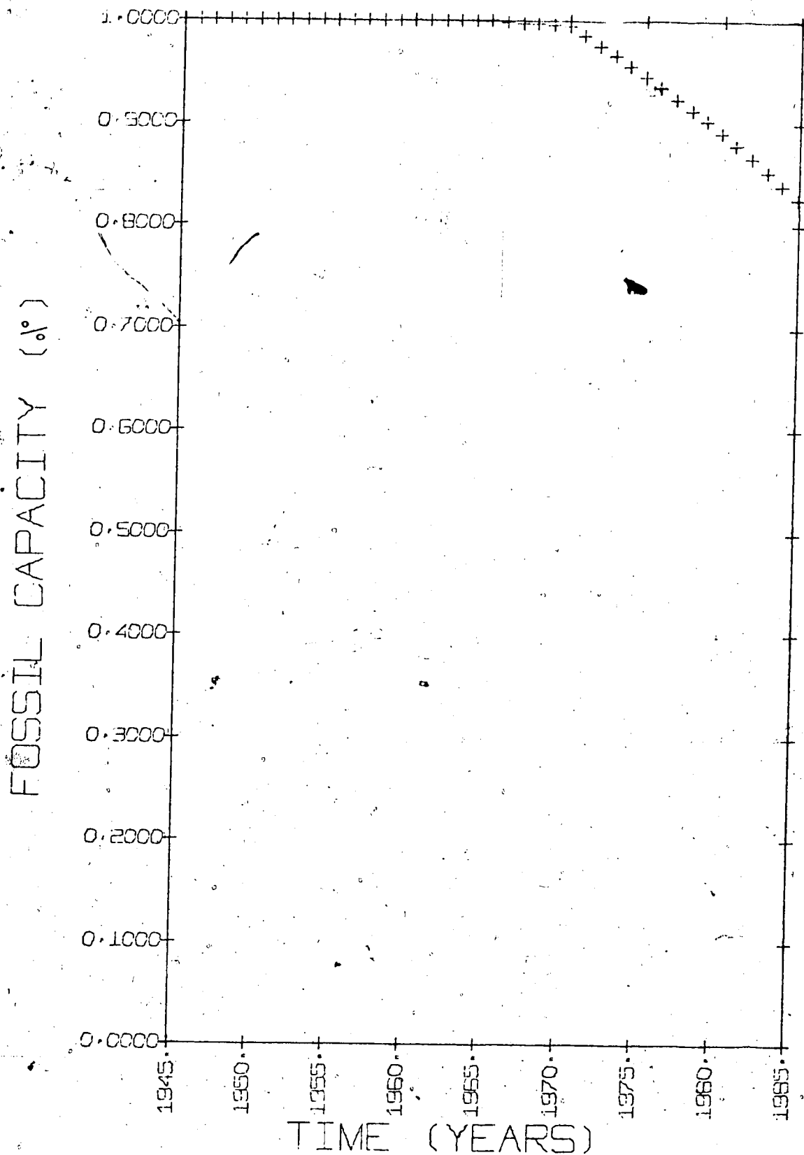
FIGURE IV.17 - PERCENTAGE OF TOTAL ELECTRICAL GENERATING CAPACITY WHICH IS DEPENDENT ON NON-NUCLEAR FUEL, CASE I 1945-85.
