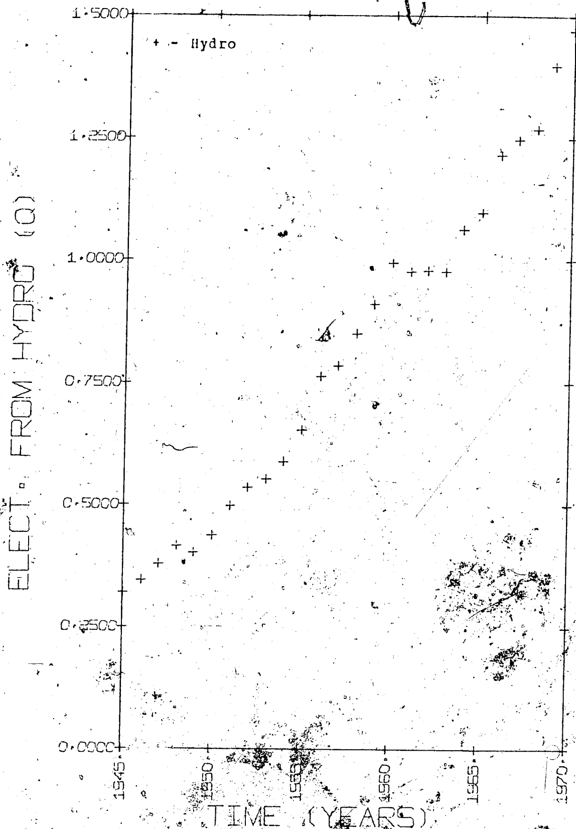
FIGURE III.20 • QUANTITY OF ELECTRICITY PRODUCED FROM HYDRO BASE CASE 1945-70
