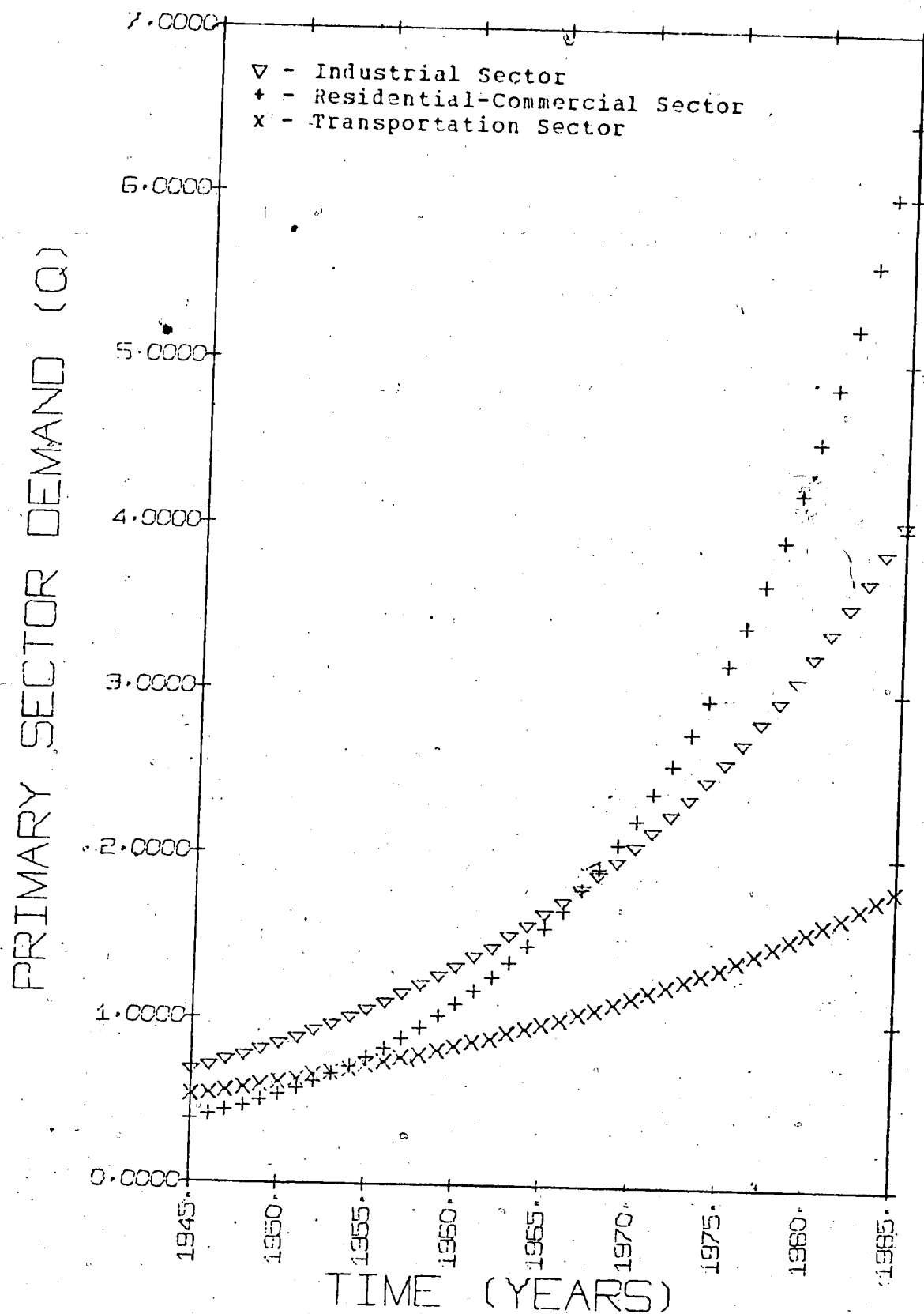
FIGURE IV.30 - ENERGY DEMAND BY THE PRIMARY CONSUMING SECTORS, CASE II 1945-85.
