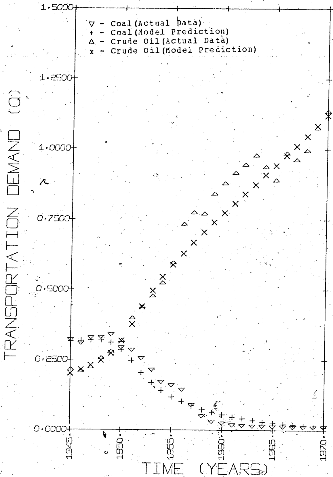
FIGURE III.12 - TRANSPORTATION ENERGY DEMAND, BASE CASE 1945-70.
