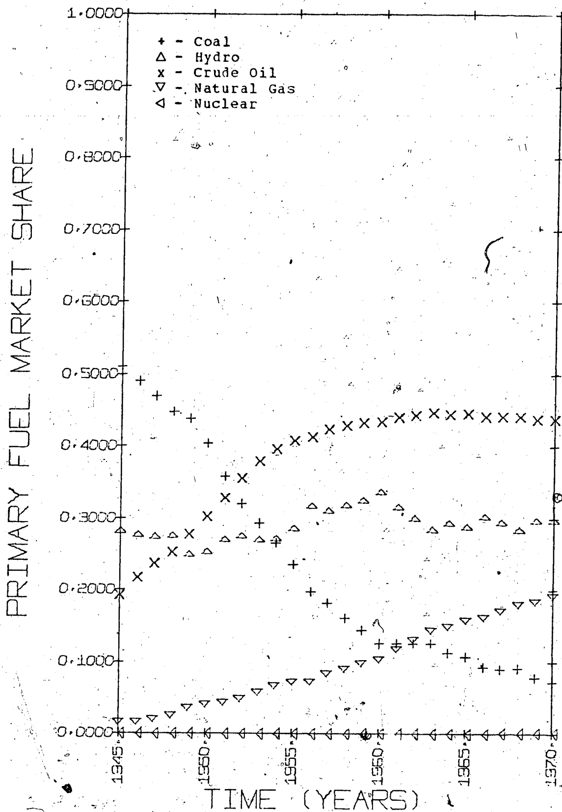
FIGURE III.19 - TOTAL MARKET SHARES OF PRIMARY FUELS, BASE CASE 1945-70.
