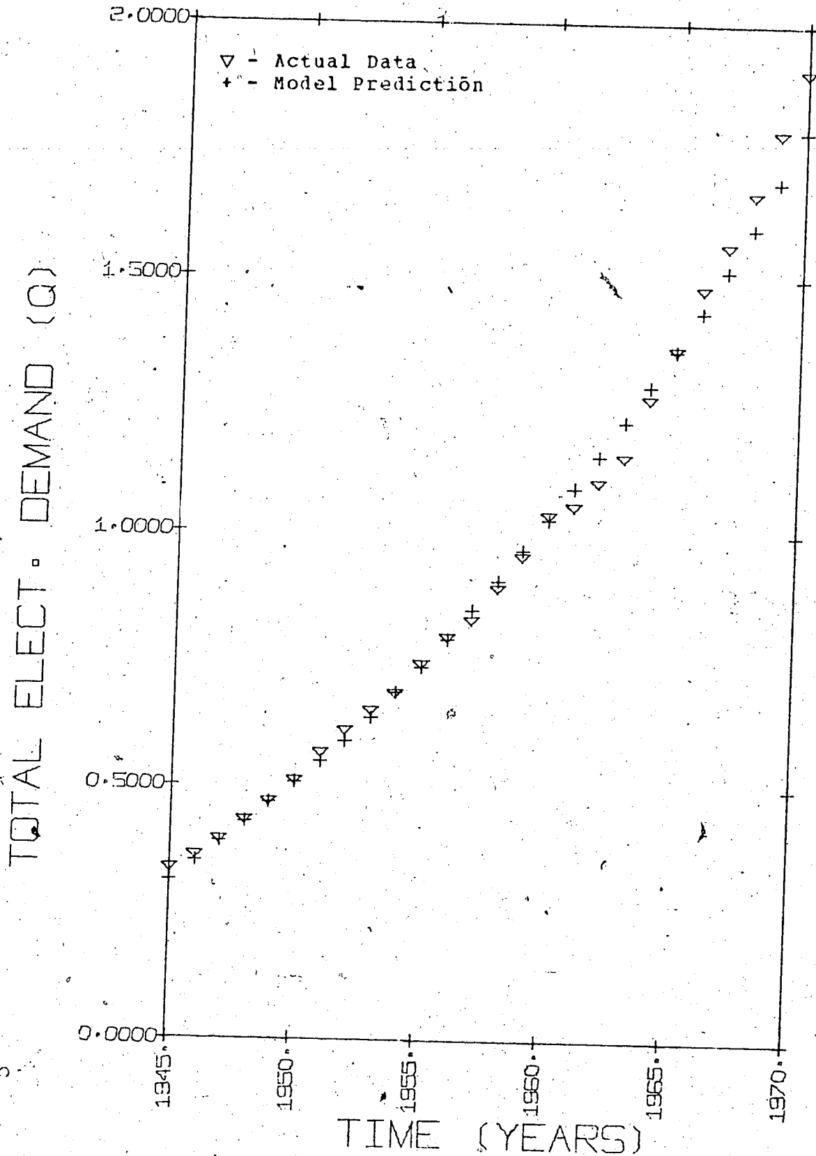
FIGURE III.13 - TOTAL DEMAND FOR ELECTRICITY (ZO), BASE CASE 1945-70.
