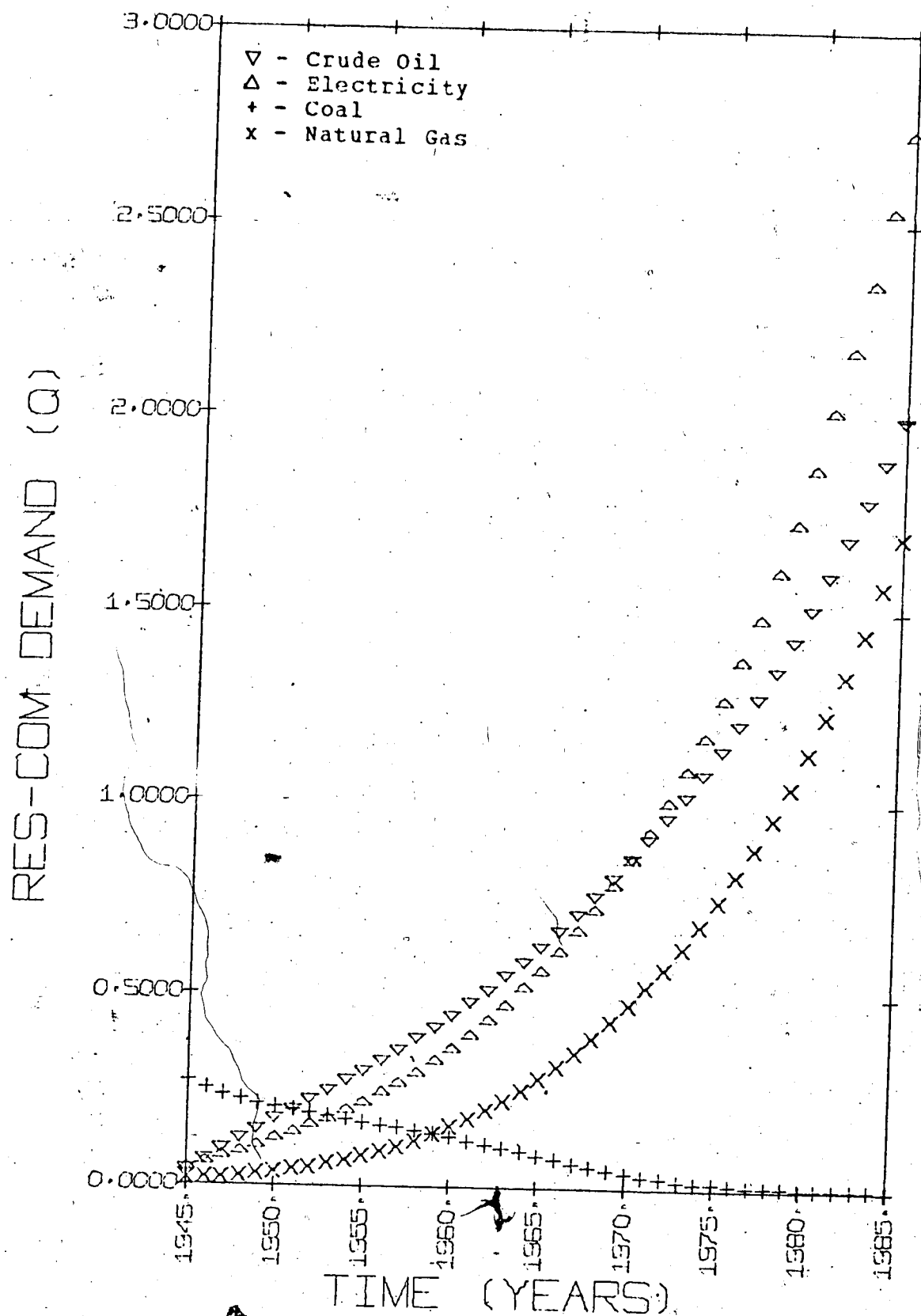
FIGURE IV.31 - RESIDENTIAL-COMMERCIAL DEMAND, CASE II 1945-85.
