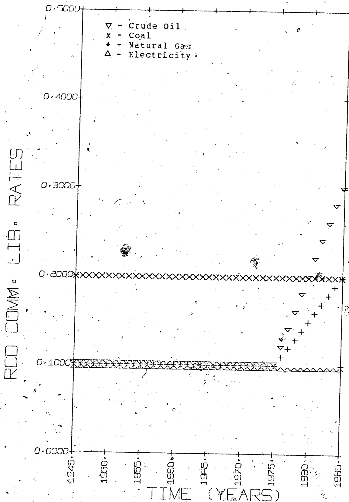
FIGURE IV.39 - CONSUMER COMMITMENT LIBERATION RATES FOR THE RESIDENTIAL-COMMERCIAL DEMAND SECTOR, CASE III 1945-85.
