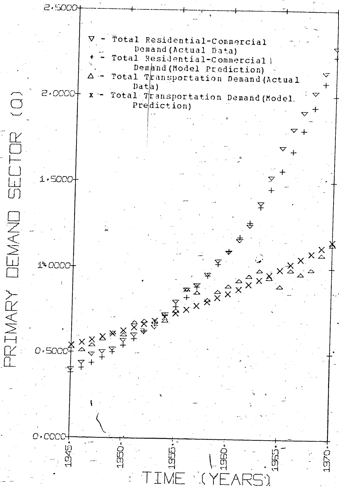
FIGURE III.2 - TOTAL ENERGY DEMAND BY RESIDENTIAL-COMMERCIAL AND TRANSPORTATION SECTORS, BASE CASE 1945-70.
