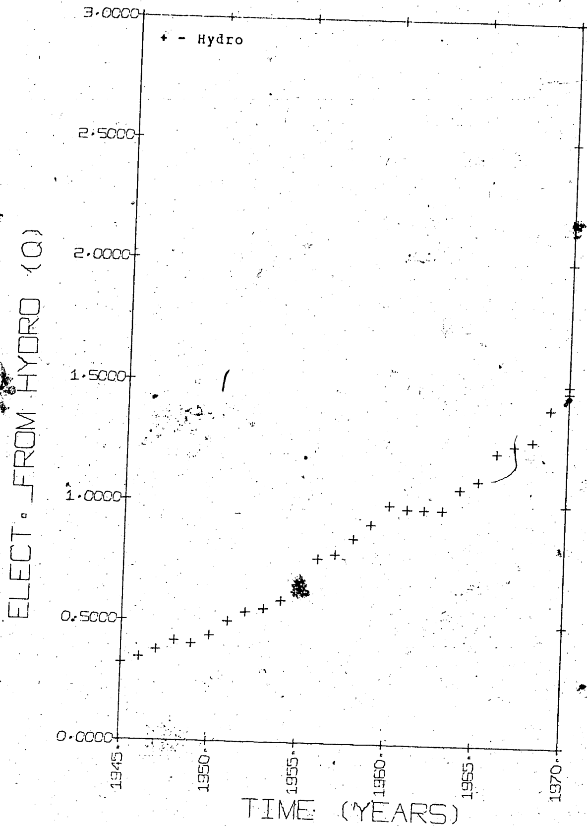
FIGURE IV.2 - ELECTRICITY GENERATED FROM HYDRO, BASE CASE 1945-70.
