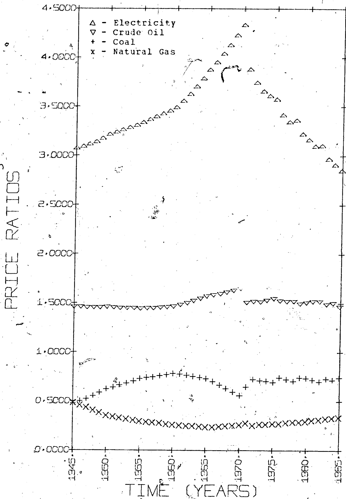
FIGURE IV.29 - RELATIVE PRICES OF THE FUEL FORMS, CASE II 1945-85.
