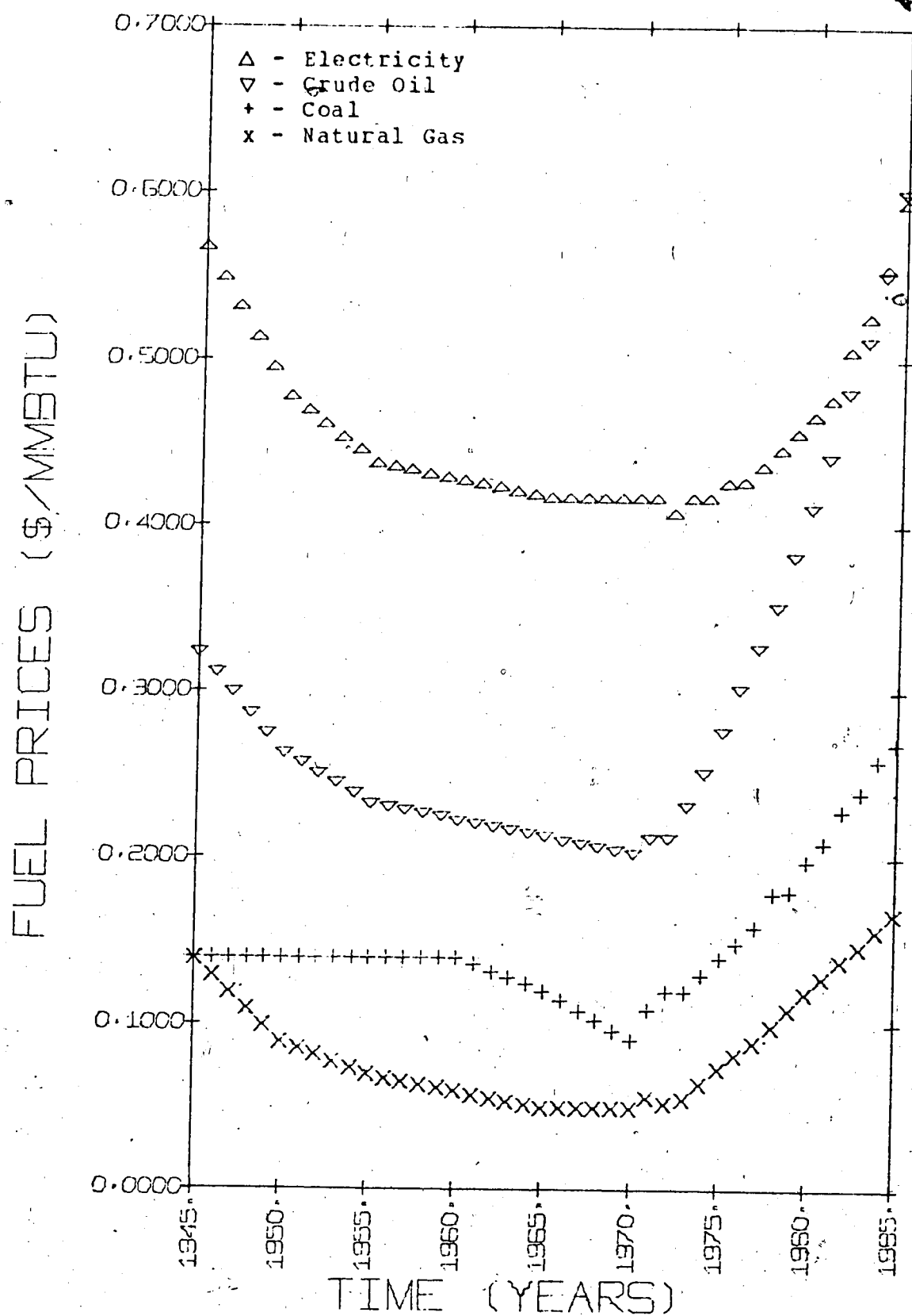
FIGURE IV.19 - FUEL PRICES, CASE I 1945-85.
