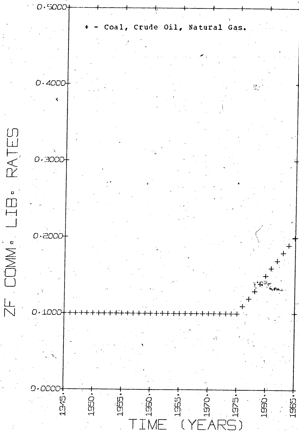
FIGURE IV.42 - PRODUCER COMMITMENT LIBERATION RATES FOR THE ELECTRICITY GENERATING SECTOR, CASE III 1945-85.
