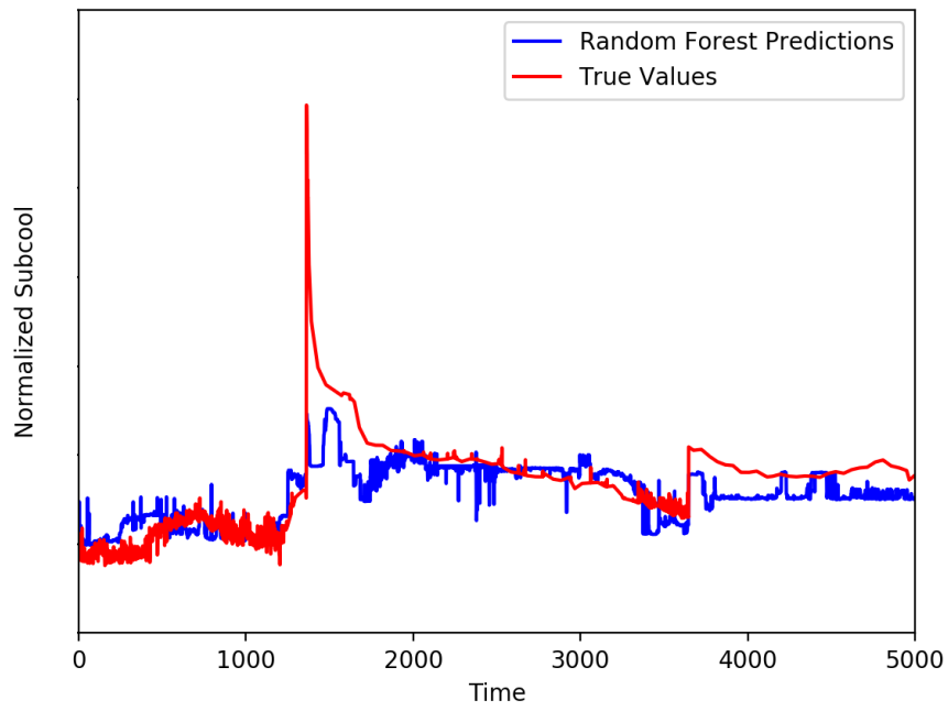
Figure 2.5: Test results of Random Forest
