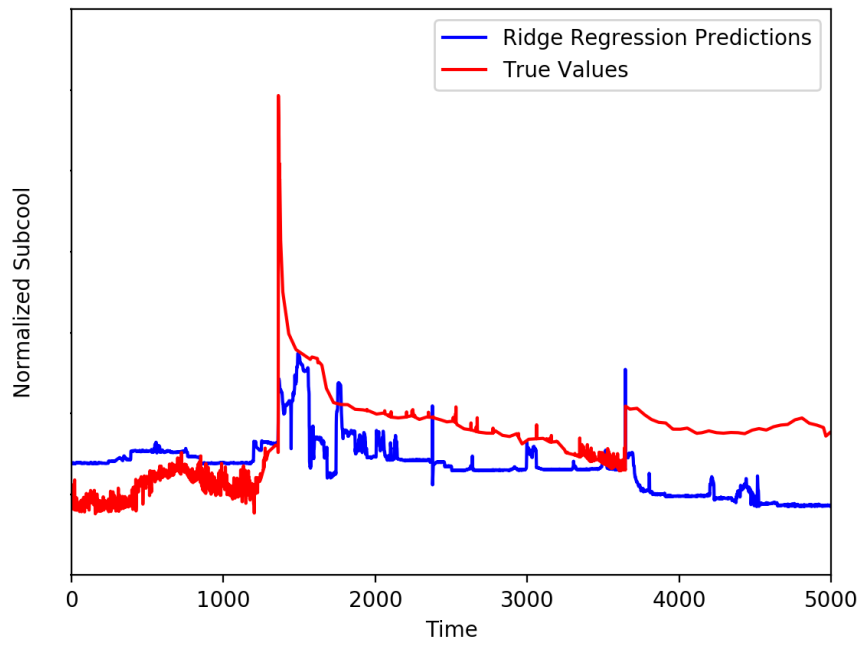
Figure 2.7: Test results of Ridge Regression
