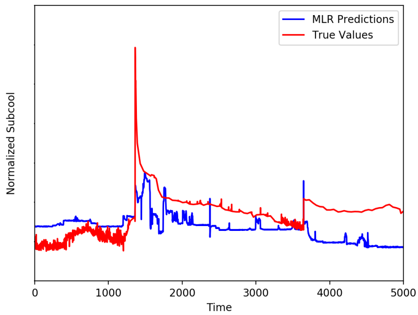
Figure 2.8: Test results of Multiple Linear Regression
