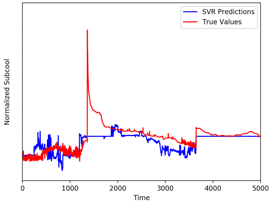
Figure 2.6: Test results of Support Vector Regression
