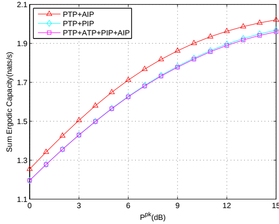
Fig. 3.7. Sum ergodic capacity vs P^{pk} .
