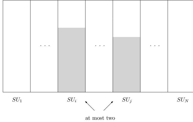
Fig. 3.5. Optimal power allocation under ATP + PIP constraints.
