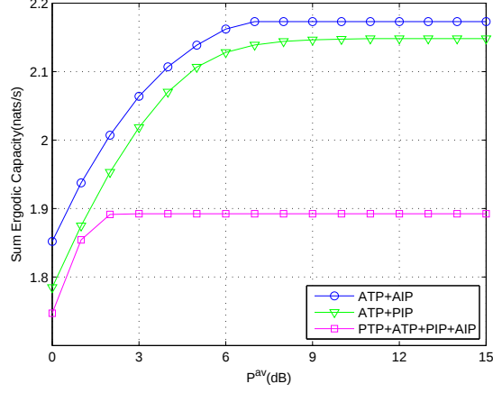
Fig. 3.8. Sum ergodic capacity vs P^{av} .
