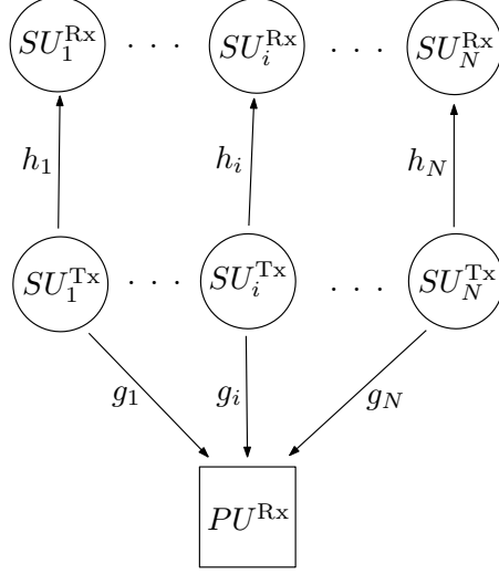
Fig. 3.1. Cognitive radio network.
