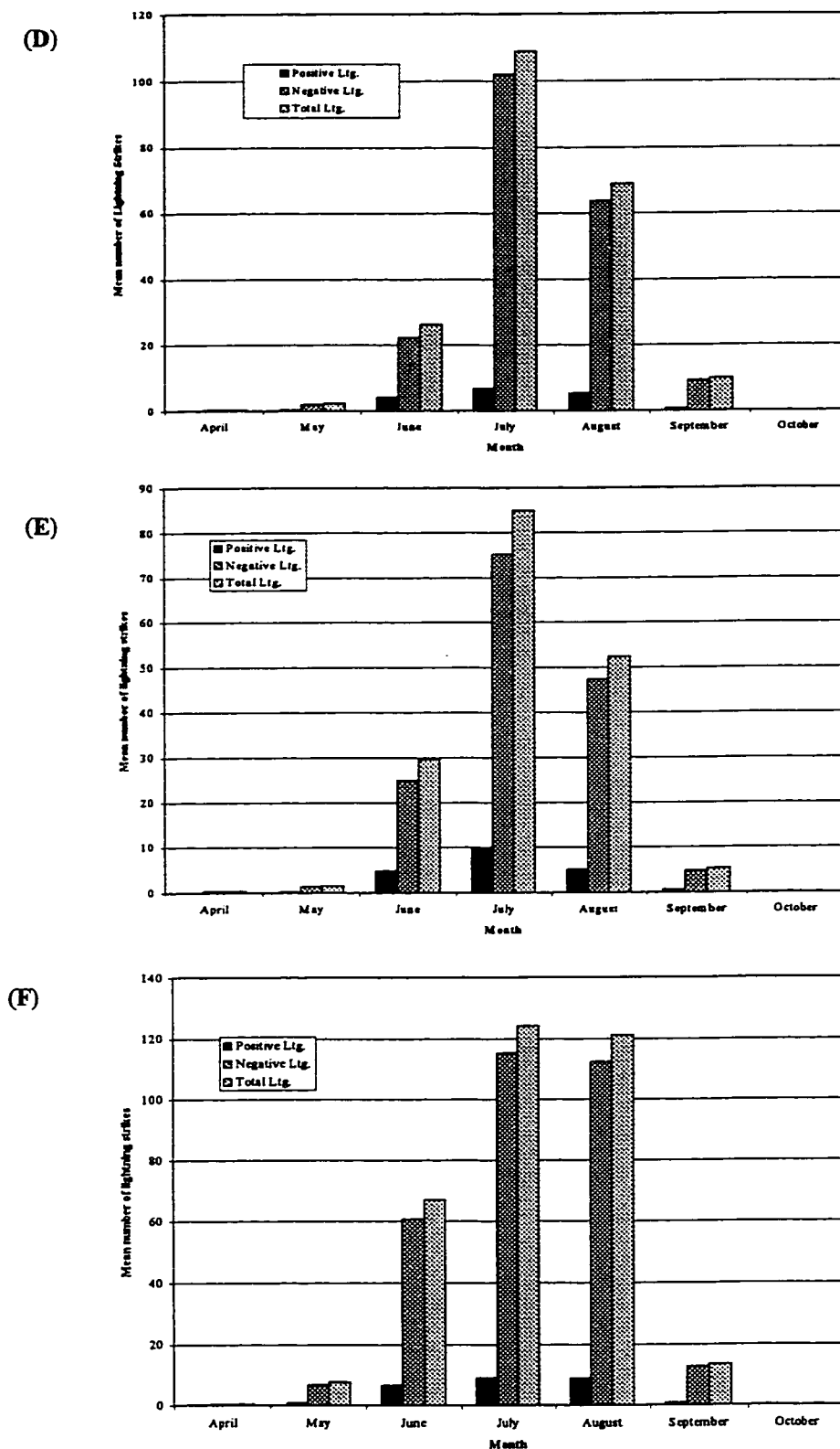
Figure 4-7 Mean number of lightning strikes, by month, recorded in the Muddy Creek (D), Saddle Hills (E), and Townships 62 & 63 (F) research area between 1984 and 1996.
