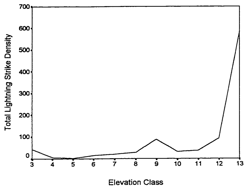
Figure E-11 The total number of lightning strikes per square kilometer by elevation class in the Mount Louie research area.
