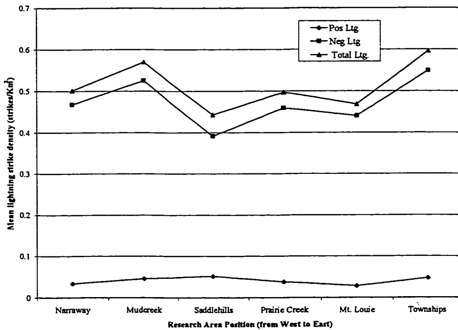
Figure 4-5 Mean lightning strikes density (1984-1996) by the relative location of the research areas from West to East within the FMA.
