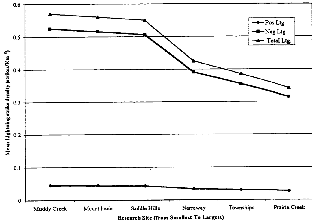
Figure 4-6 Mean lightning strike density (1984 -1996) by research area size (from smallest to largest).
