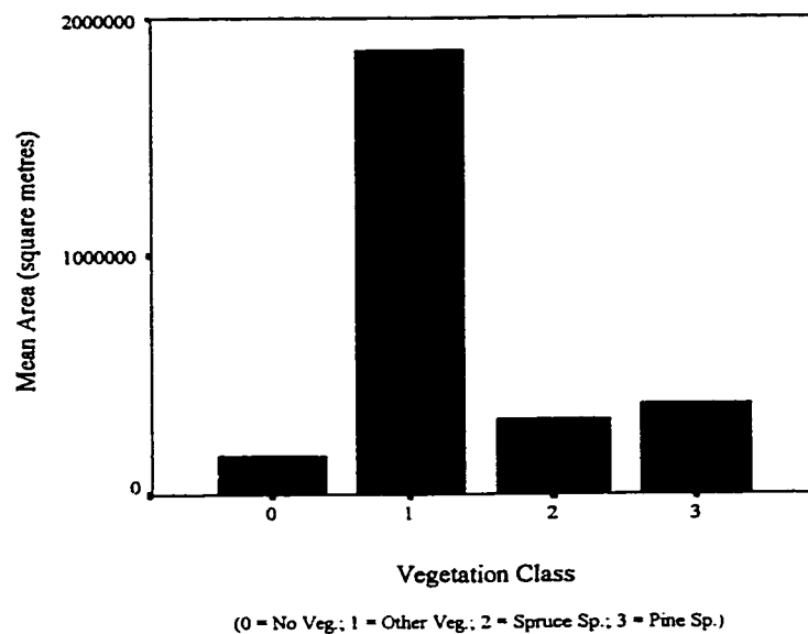
Figure E-22 The mean area by Vegetation Class for the Muddy Creek Vegetation Coverage.
