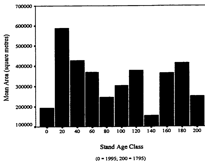
Figure E-34 The mean area by stand age class for the Township Stand Origin Coverage.
