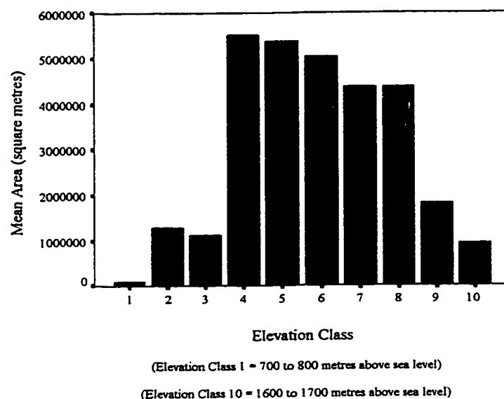
Figure E-7 The mean area by Elevation Class for the Elevation Coverage of the Narraway Research Area.
