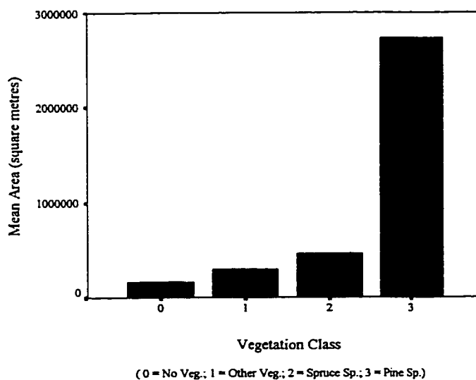
Figure E-17 The mean area by Vegetation Class for the Vegetation Coverage of the Narraway Research Area.
