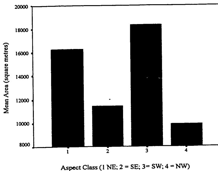
Figure E-3 The mean area by Aspect Class for the Mount Louie Aspect Coverage.
