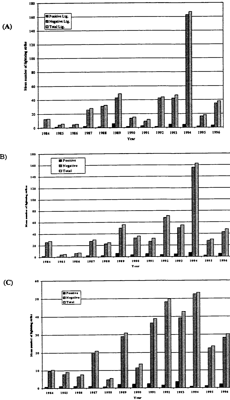
Figure 4-3. Mean number of lightning strikes, by year, recorded in the Narraway (A), Prairie Creek (B), and Mount Louie (C) research areas between 1984 and 1996.
