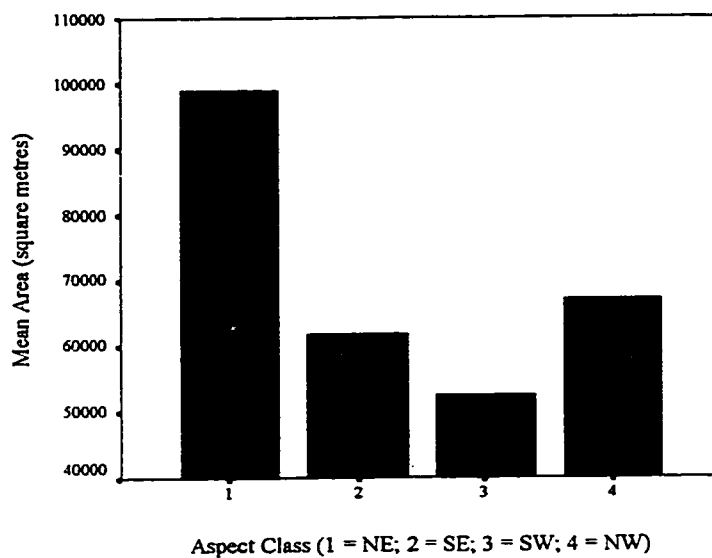
Figure E-6 The mean area by Aspect Class for the Township Aspect Coverage.
