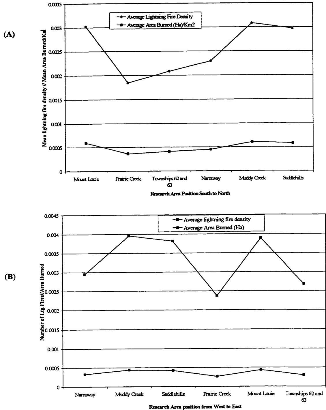
Figure 4-9 Mean lightning fires density, and average area burned per square kilometer by research area between 1984 and 1996 relative to the positions of the research areas within the FMA from (A) South to North, and (B) West to East.
