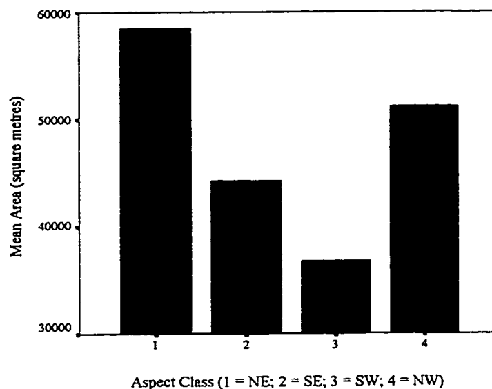
Figure E-4 The mean area by Aspect Class for the Muddy Creek Aspect Coverage.
