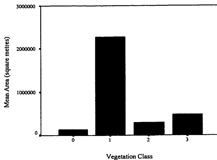
Figure E-23 The mean area by Vegetation Class for the Saddle Hills Vegetation Coverage.
