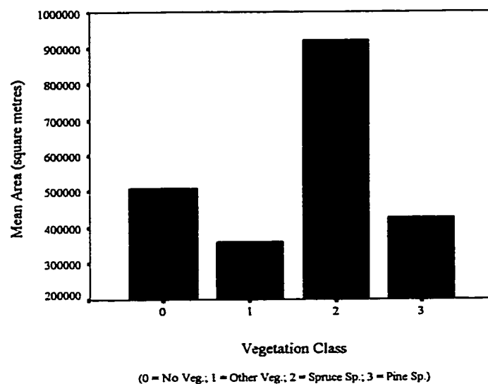
Figure E-24 The mean area by Vegetation Class for the Township Vegetation coverage.
