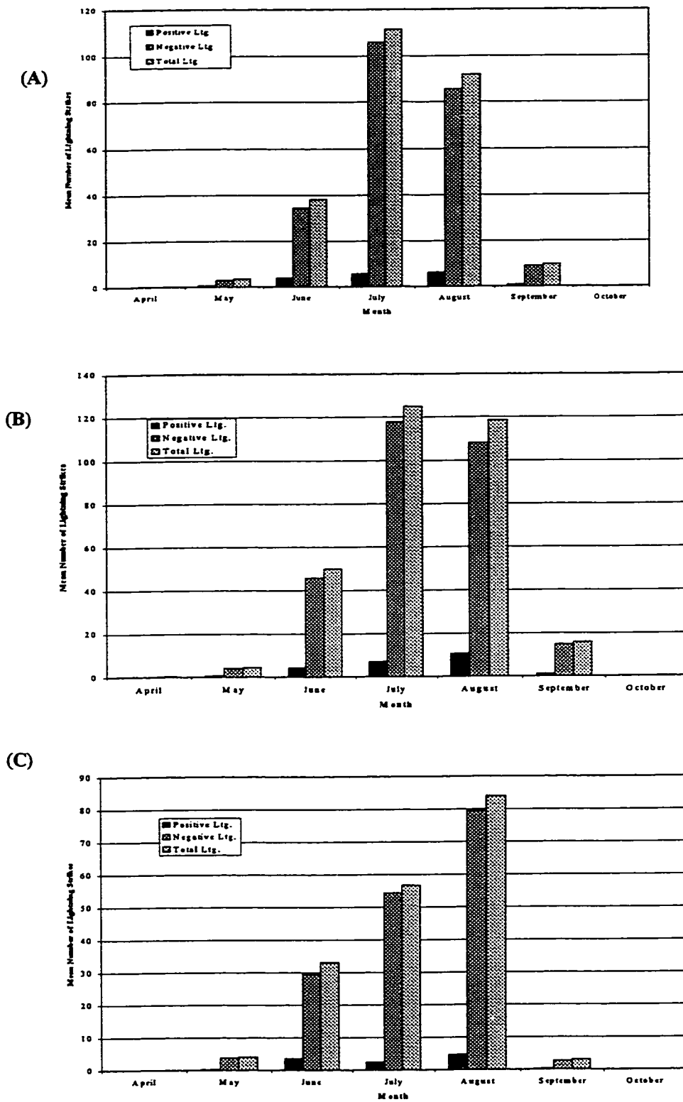
Figure 4-7. Mean number of lightning strikes, by month, recorded in the Narraway (A), Prairie Creek (B), and Mount Louie (C) research area between 1984 and 1996.
