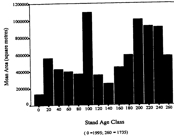
Figure E-28 The mean area by Stand Age Class for the Prairie Creek Stand Origin Coverage.
