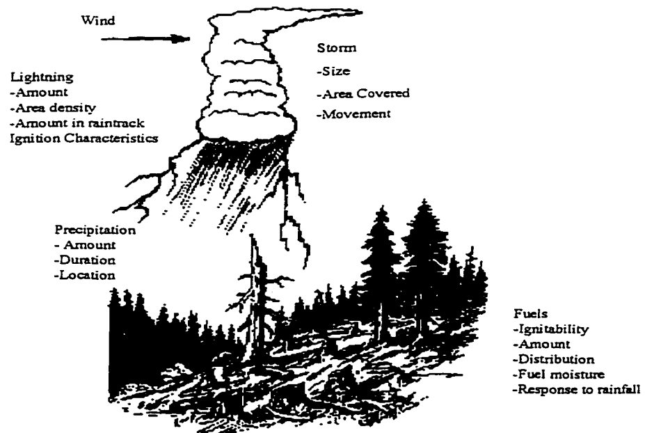
Figure 1-2 Various factors known to influence the ignition of a lightning fire (Source: Fuquay et. al 1972).
