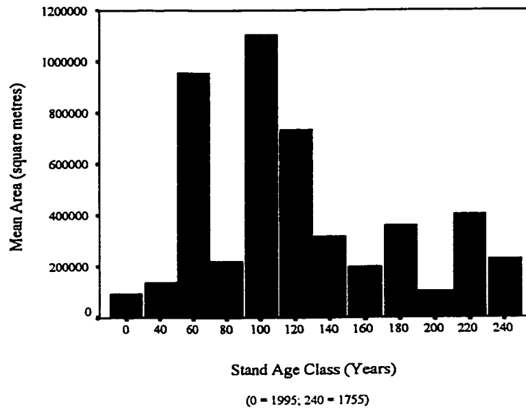
Figure E-25 The mean area by Stand Age Class for the Stand Origin Coverage of the Narraway research area.
