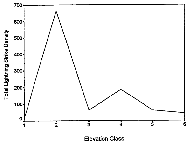
Figure E-16 Total Lightning Strike density, as measured by number of strikes per square kilometer, by Elevation Class in the Townships research area.
