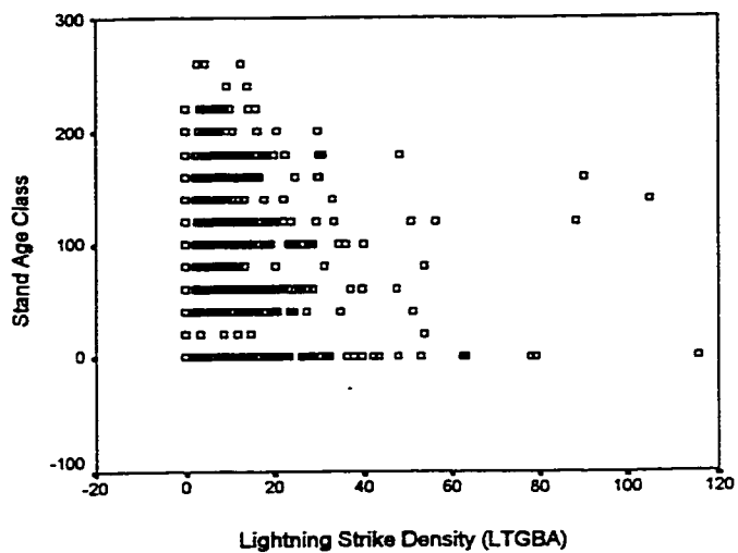
Figure E-29 A scatter plot of stand age class by lightning strike density for the Prairie Creek research area.
