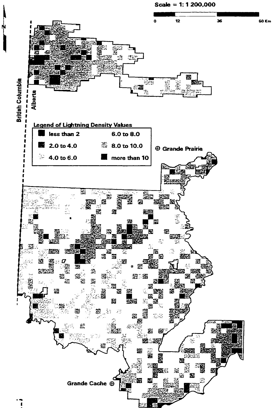
Figure 4-1 Cumulative lightning strike density, as measured by the number of strikes per square kilometer, in Weyerhaeuser Canada Limited's Grande Prairie FMA. Based on lightning strikes recorded between 1984 and 1996 input into a 3 Km x 3 Km raster grid.
