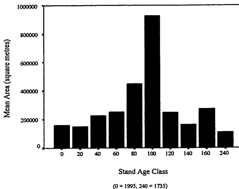
Figure E-22 The mean area by Stand Age Class for the Muddy Creek Stand Origin Coverage.
