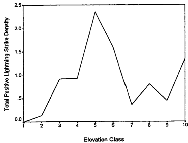
Figure E-8B Total Positive lightning strike density by Elevation class in the Narraway research area.
