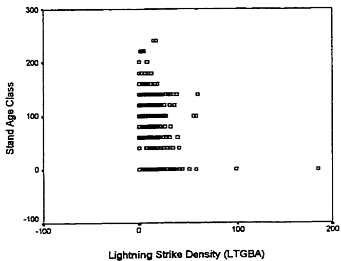
Figure E-26 A Scatter plot of stand age class by lightning strike density for the Narraway research area.
