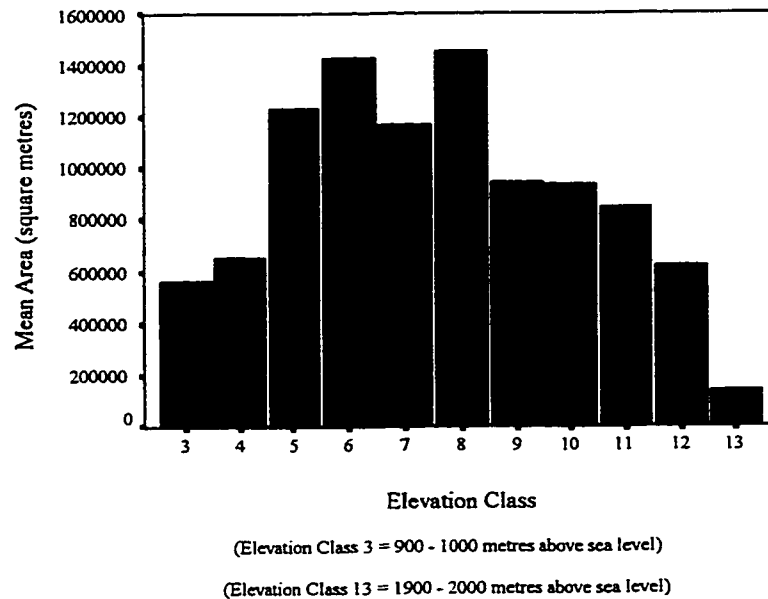
Figure E-10 The mean area by Elevation Class for the Mount Louie Elevation Coverage.
