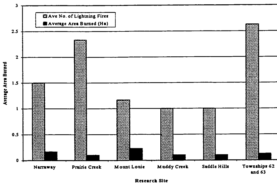
Figure 4-8B Mean number of lightning fires and average area burned by research area during the period between 1984 and 1996.
