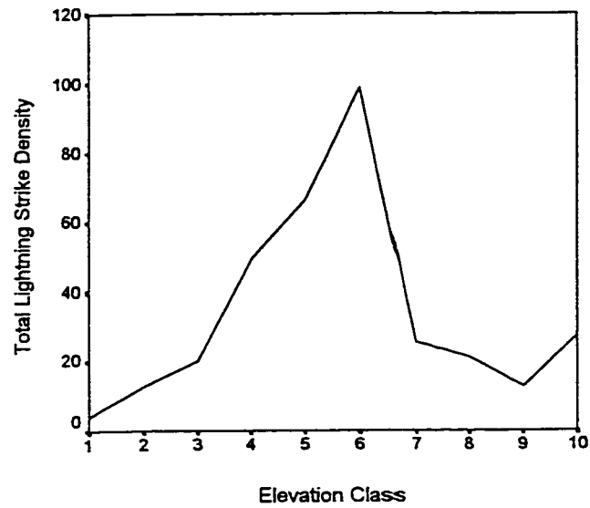
Figure E-8a Total lightning strike density by Elevation class in the Narraway research area.
