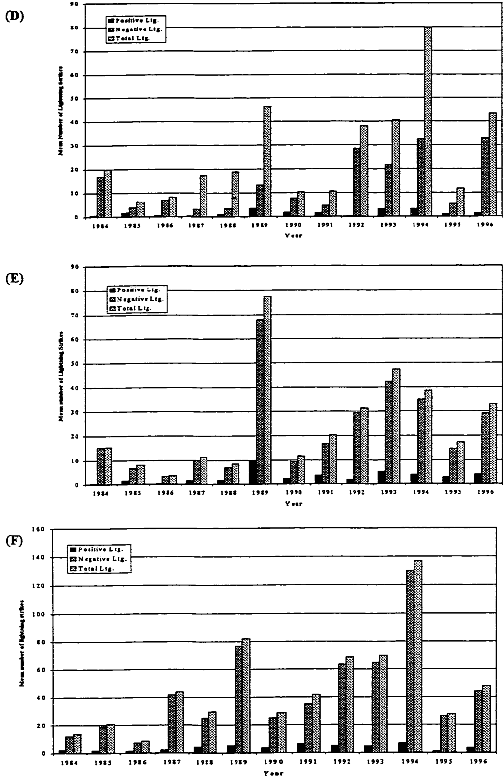
Figure 4-3. Mean number of lightning strikes, by year, recorded in the Muddy Creek (D), Saddle Hills (E), and Townships research (F) areas between 1984 and 1996.
