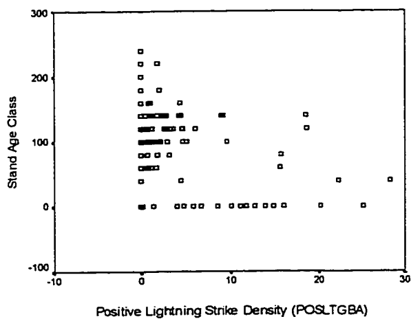
Figure E-27 A Scatter plot of stand age class by positive lightning strike density for the Narraway research area.
