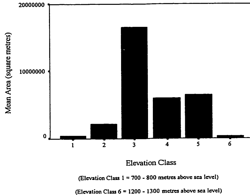
Figure E-15 The mean area by Elevation Class for the Township Elevation Coverage.
