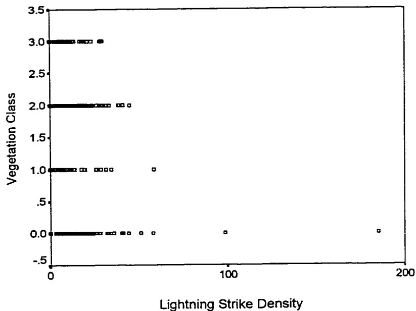
Figure E-18A Vegetation type by total lightning strike density in the Narraway research area.
