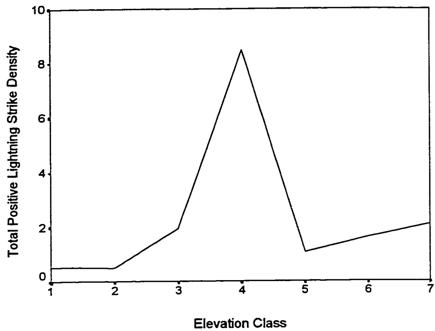
Figure E-13 Total Positive Lightning strike density by Elevation Class for the Muddy Creek Research area.
