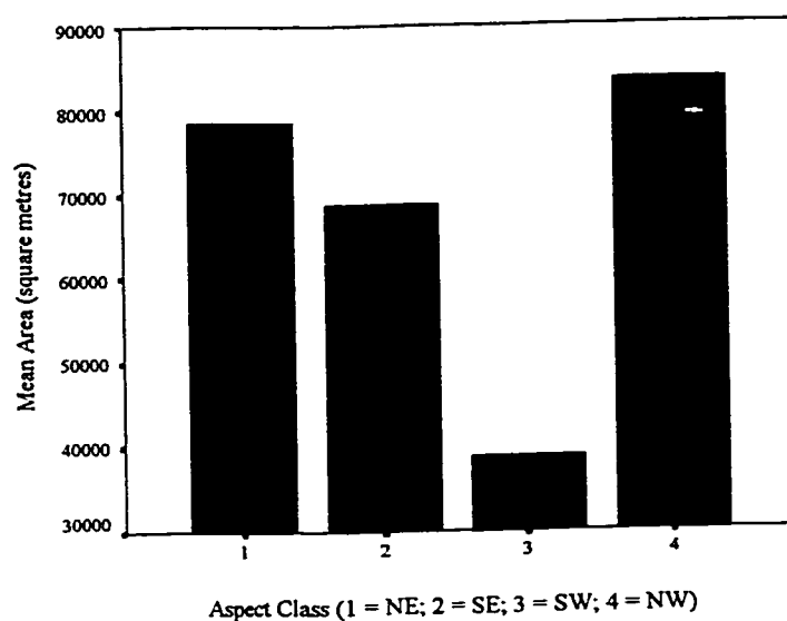
Figure E-2 The mean area by Aspect Class for the Prairie Creek Aspect Coverage
