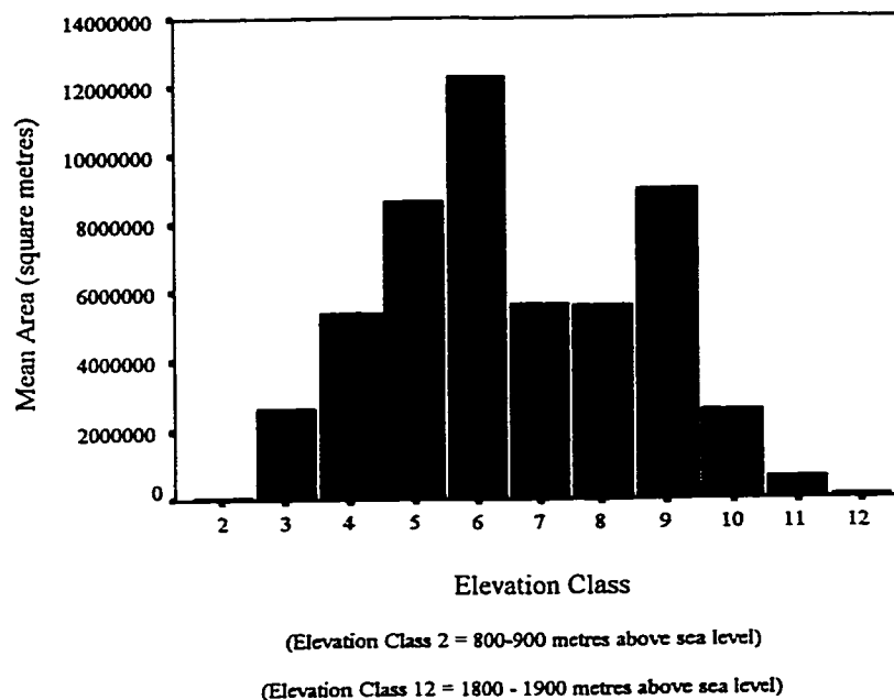
Figure E-9 The mean area by Elevation Class for the Prairie Creek Elevation Coverage.
