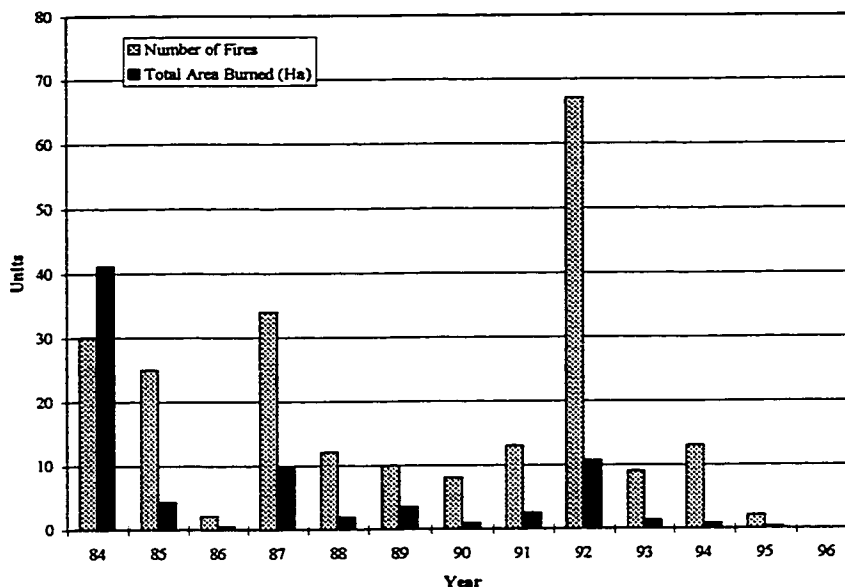
Figure 4-8A Mean annual number of lightning fires, and average area burned in the Grande Prairie Forest Management Area during the period between 1984 and 1996.
