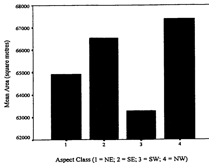
Figure E-5 The mean area by Aspect Class for the Saddle Hills Aspect Coverage.
