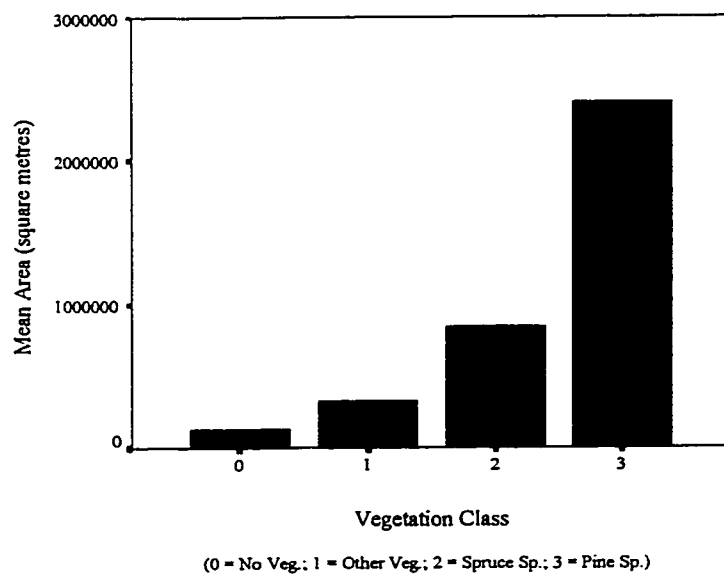
Figure E-19 The mean area by Vegetation Class for the Prairie Creek Vegetation Coverage.
