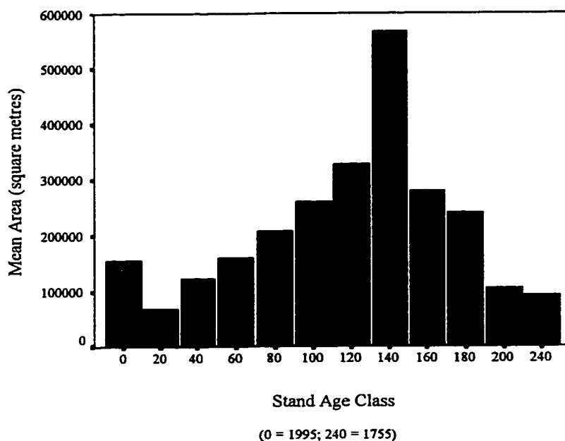
Figure E-31 The mean area by Stand Age Class for the Mount Louie Stand Origin Coverage.
