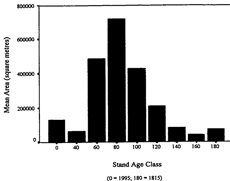
Figure E-33 The mean area by Stand Age Class for the Saddle Hills Stand Origin Coverage.
