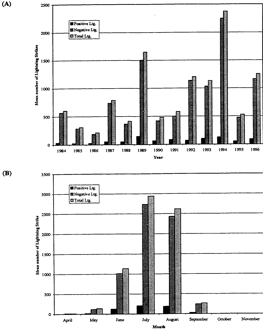
Figure 4-2 Mean Number of Lightning strikes by Year (A) and by Month (B) recorded in the FMA between 1984 and 1996.
