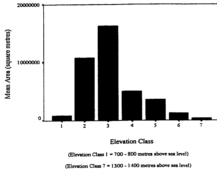
Figure E-12 The mean area by Elevation Class for the Muddy Creek Elevation Coverage.
