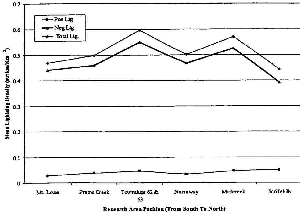
Figure 4-4 Mean lightning strike density (1984-1996) by relative location of research areas from south to north within the Grande Prairie FMA.
