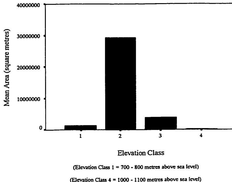
Figure E-14 The mean area by Elevation Class for the Saddle Hills Elevation Coverage.
