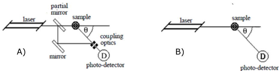
Figure 2.6: Scattering configuration A) Heterodyne B) Homodyne. 11 (used with permission)
