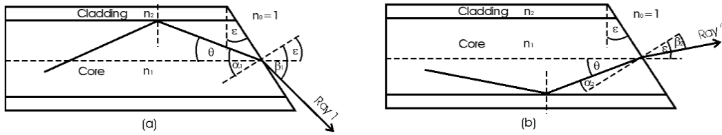
Figure E.2: Angle ended fiber Mayor Axis light propagation: a) \varepsilon \leq \theta , b) \varepsilon > \theta . 48 (used with permission)
