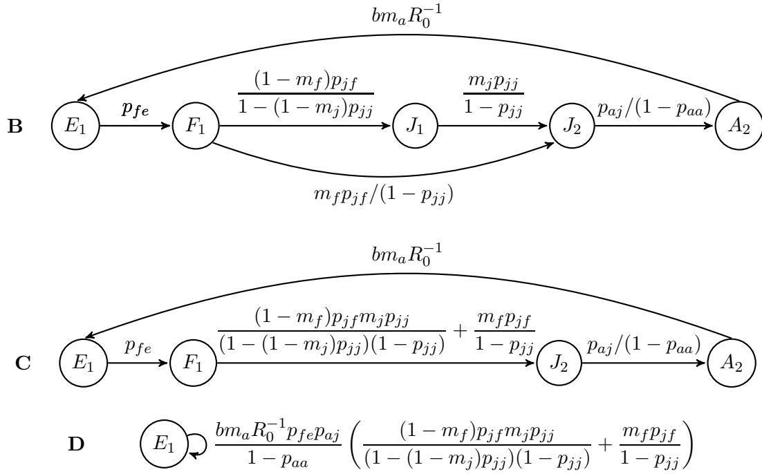
Figure 3: B Eliminating self-loops. C Eliminating node J_1 . D Eliminating nodes F_1 , J_2 , and A_2 .
