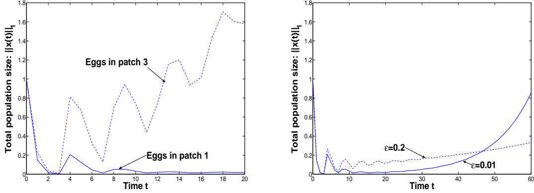
Figure 8: (Left) Comparison of overall population size with same \epsilon = 0.01 , but different initial population distribution: either x(0) = [1, 0, 0, 0, 0, 0, 0, 0, 0, 0]^T (solid line) or x(0) = [0, 0, 0, 1, 0, 0, 0, 0, 0, 0]^T (dashed line). (Right) Comparison of overall population size \|x(t)\|_1 with same initial population distribution x(0) = [1, 0, 0, 0, 0, 0, 0, 0, 0, 0]^T , but different connectivity strength \epsilon : \epsilon = 0.01 (solid line), \epsilon = 0.2 (dashed line). The solid lines in both panels show the same trajectory but over different time scales.
