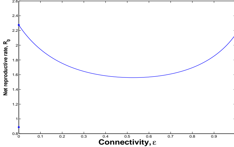
Figure 7: The relation between the mean of net reproductive rates of 2000 realizations and the connectivity strength \epsilon .
