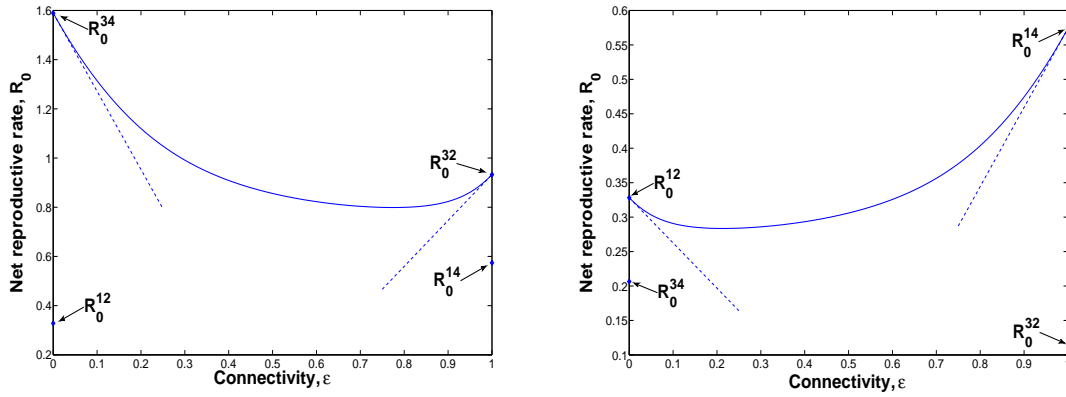
Figure 6: The relation between the R_0 and the connectivity strength \epsilon . (Left) Patch 3 is better than patch 1, patch 4 is better than patch 2. b_1 = 500, m_a^2 = 0.3, m_f^1 = 0.4, m_j^1 = 0.6, p_{fe}^1 = 0.15, p_{jf}^1 = 0.1, p_{jj}^1 = 0.12, p_{jj}^2 = 0.15, p_{aj}^2 = 0.18, p_{aa}^2 = 0.2, p_{jf}^{21} = 0.125, p_{jj}^{21} = 0.135, b_3 = 750, m_f^3 = 0.6, m_j^3 = 0.9, p_{fe}^3 = 0.23, p_{jf}^3 = 0.15, p_{jj}^3 = 0.18, p_{jj}^4 = 0.195, p_{aj}^4 = 0.234, p_{aa}^4 = 0.26, p_{jf}^{23} = 0.15, p_{jj}^{23} = 0.18, p_{jf}^{43} = 0.17, p_{jj}^{43} = 0.19 . (Right) Patch 1 is better than patch 3, patch 4 is better than patch 2. b_3 = 330, p_{fe}^3 = 0.1, m_f^3 = 0.3, m_j^3 = 0.4, p_{jf}^3 = 0.07, p_{jj}^3 = 0.08, p_{jf}^{23} = 0.11, p_{jj}^{23} = 0.12, p_{jf}^{43} = 0.13, p_{jj}^{43} = 0.14 . Other parameters are the same as in the left figure.
