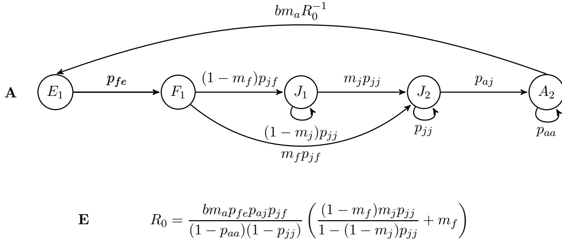
Figure 3: A The full transformed graph. E Resulting net reproductive rate.
