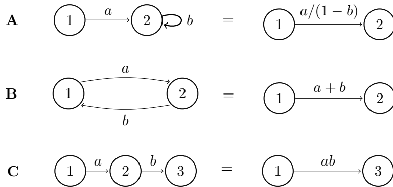
Figure I: Graph reduction rules. A self-loop elimination with b < 1 . B Parallel path elimination. C Node elimination. Rules A and B show elimination of paths, and rule C shows the elimination of node 2. Graph reduction is done by repeatedly applying these rules until only nodes are left.
