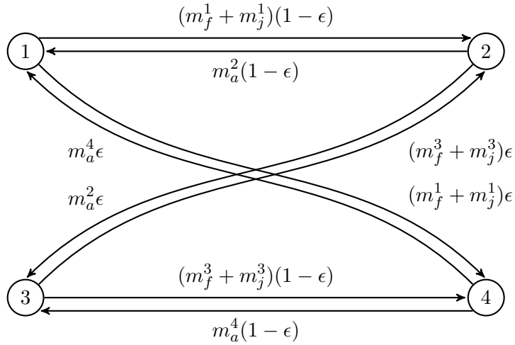
Figure 5: Connectivity strength \epsilon is realized by migration rates. Here m_a^2 represents the proportion that adults emigrate from the patch 2 to upstream for reproduction, that is, m_a^2 = m_a^{12} + m_a^{32} , here m_a^{12} = m_a^2(1 - \epsilon) and m_a^{32} = m_a^2\epsilon . Similar notations are applied to other migration rates.
