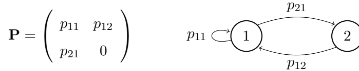
Figure 1: A simple projection matrix and its associated graph. There is a directed edge in the graph for every nonzero entry p_{ij} in the matrix. For a transition, the edge is directed from node j to node i .
