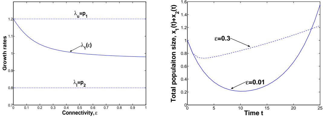
Figure 2: (Left) The dependence of growth rate \lambda_1 on migration rate \epsilon . (Right) The solutions of the model (1.3) with same initial distribution [x_1(0), x_2(0)] = [0, 1] but different connectivity: either \epsilon = 0.01 (solid line) or \epsilon = 0.3 (dashes line).
