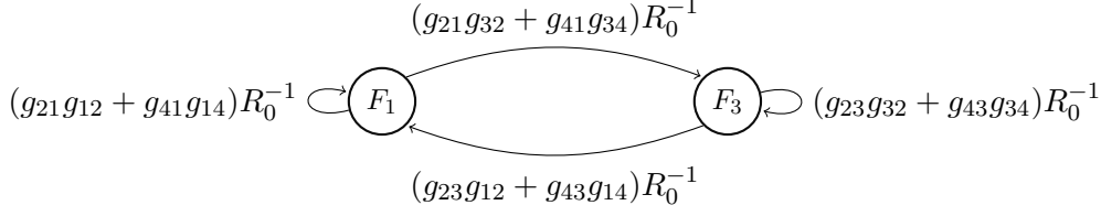
Figure 4: E Eliminating nodes J_2 and J_4 .
