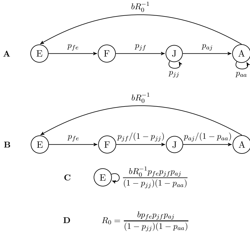
Figure II: A The full transformed graph. B Eliminating self-loops. C Eliminating nodes F , J , and A . D Solving for R_0 .
