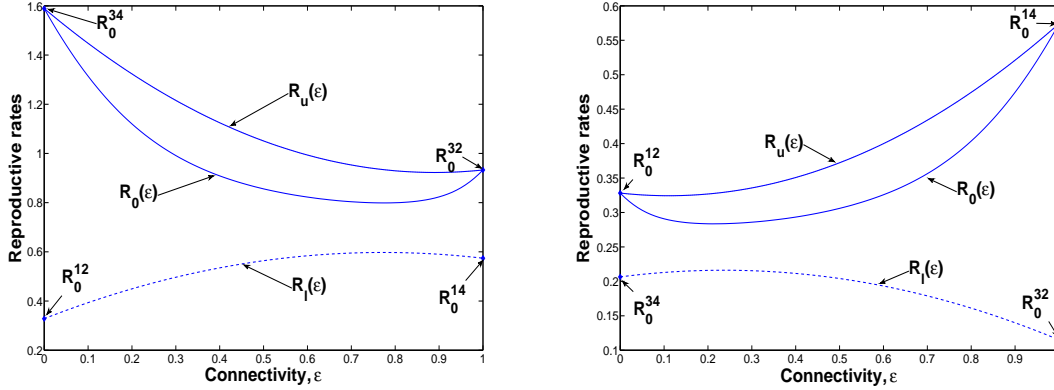
Figure 9: Comparison of the graphs of functions R_0(\epsilon) , R_l(\epsilon) , and R_u(\epsilon) . We use the same parameters as those in Figure 6.
