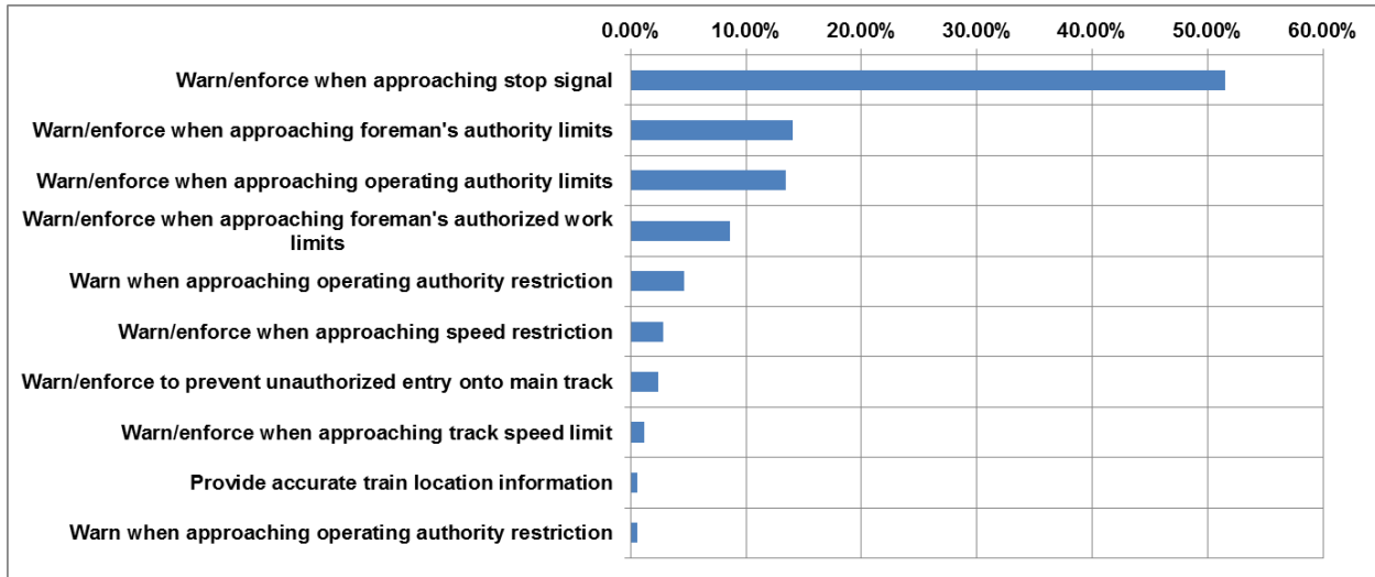
Figure 1-6. Breakdown in the key functionality of a Level 1 ETC system in terms of the number of preventable occurrences (498 in total).
