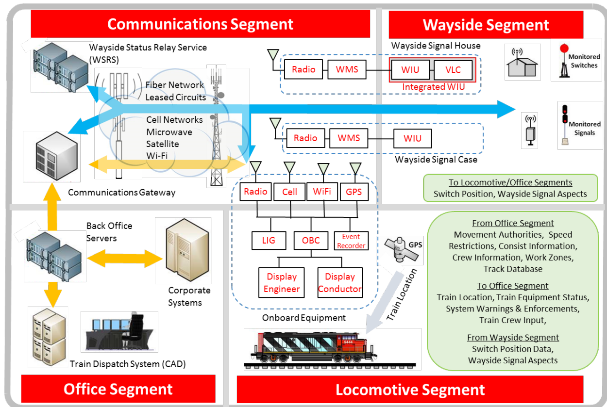
Figure 1-4. Level 3 ETC System.
