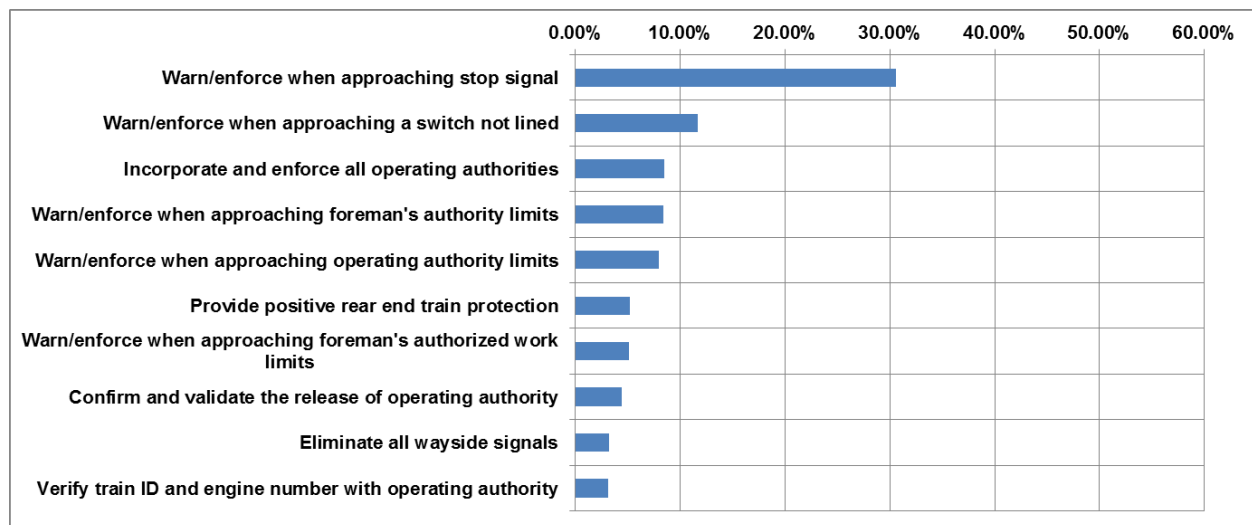
Figure 1-8. Breakdown in the key functionality of a Level 4 ETC system in terms of the number of preventable occurrences (837 in total).
