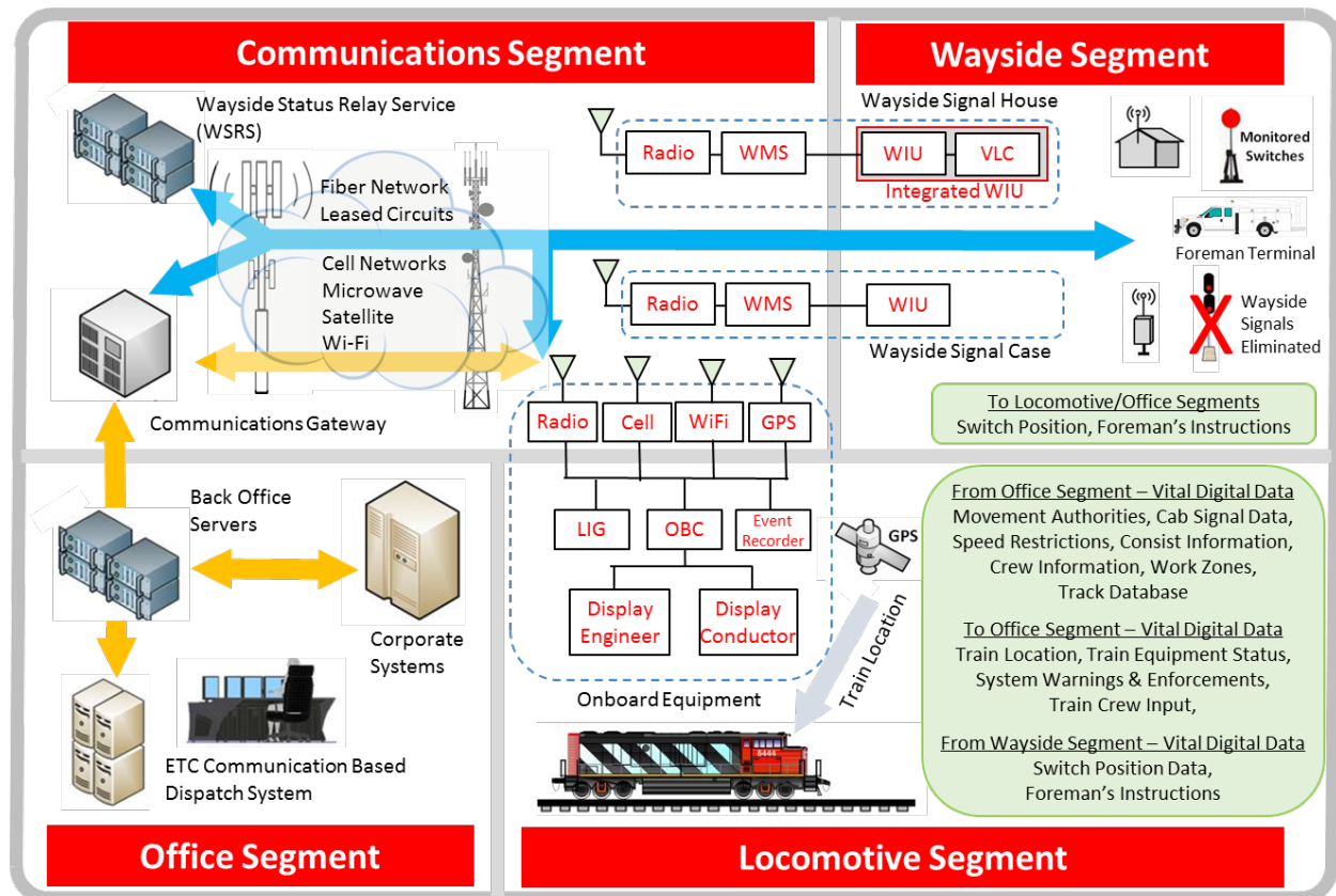
Figure 1-5. Level 4 ETC system.
