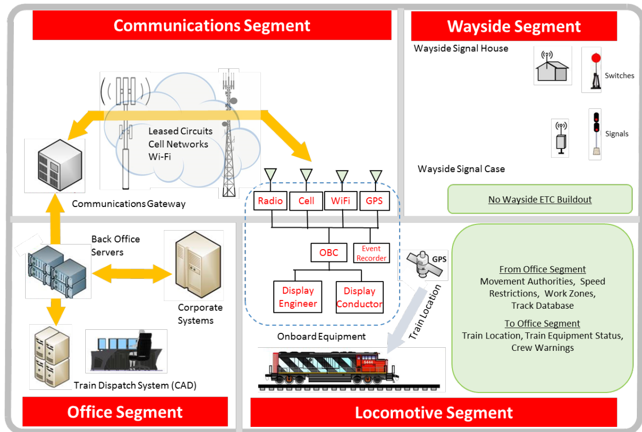
Figure 1-2. Level 1 ETC system.
