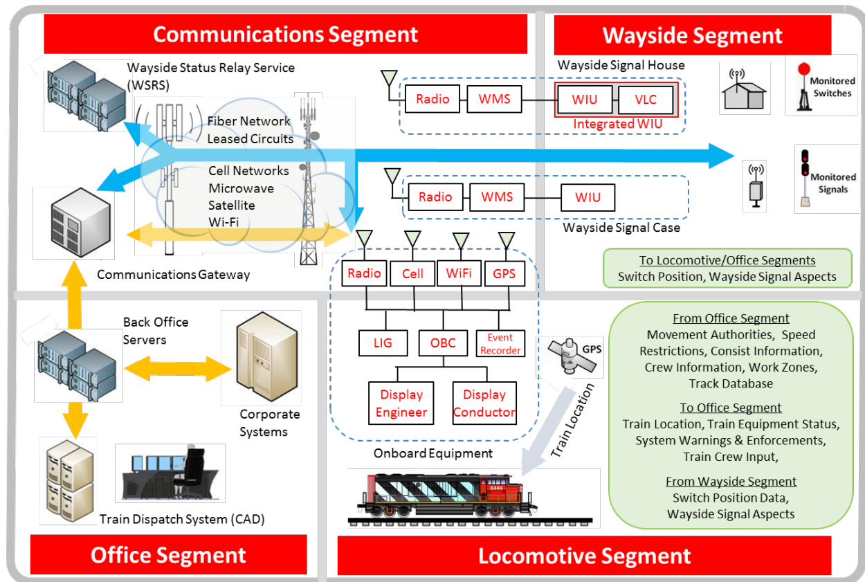
Figure 1-1. Four major components of the US PTC system (LIG: locomotive interface gateway, OBC: on board computer, WMS: wayside messaging server, WIU: wayside interface unit, VLC: vital logic controller).
