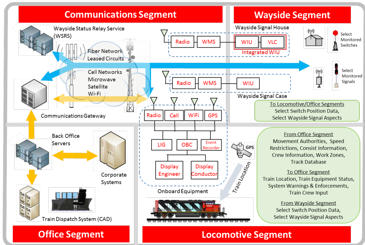
Figure 1-3. Level 2 ETC system.
