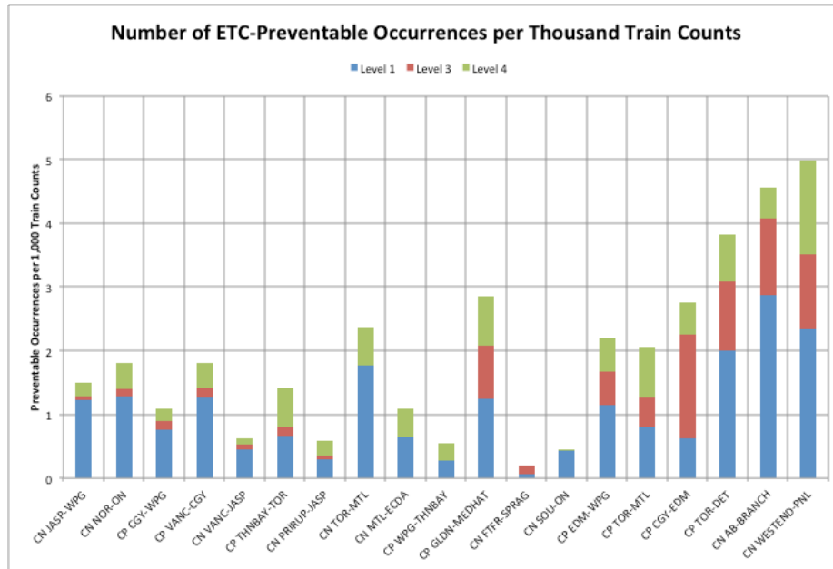
Figure 2-8. Normalized ETC preventable occurrences within each corridor at each ETC Level per thousand train counts.
