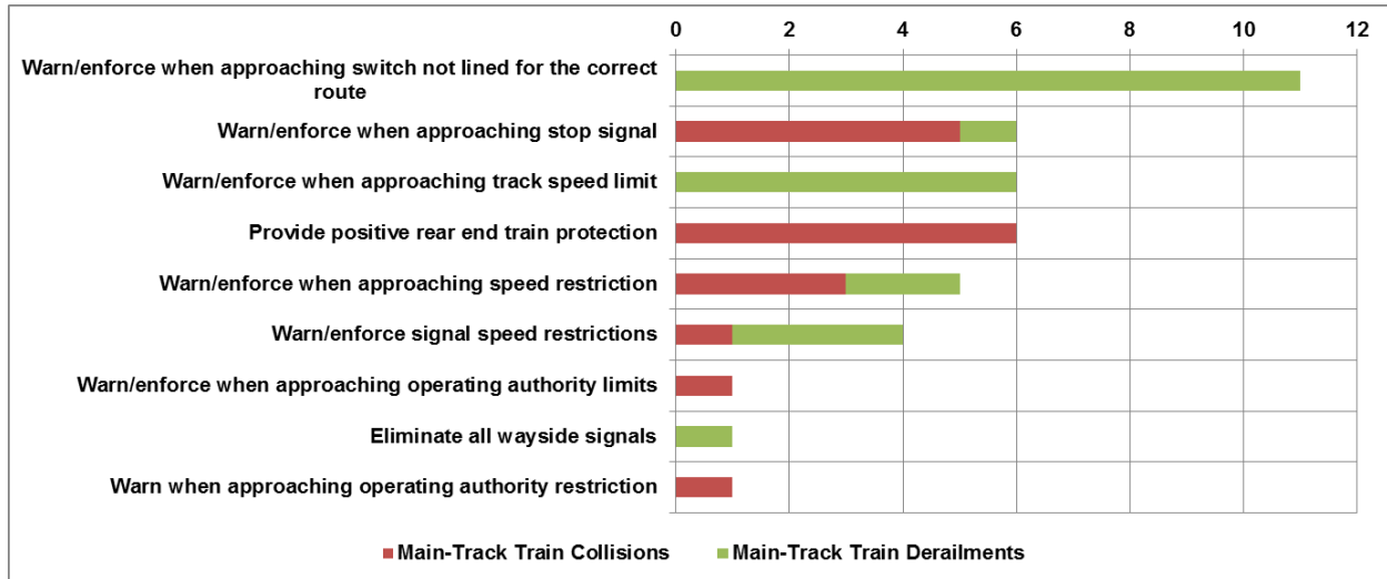
Figure 1-16. Breakdown in the key functionality of a Level 4 ETC system in terms of the number main-track train accidents it would prevent (40 in total). Red and green bars represent the main-track train collision and derailment contributions, respectively.
