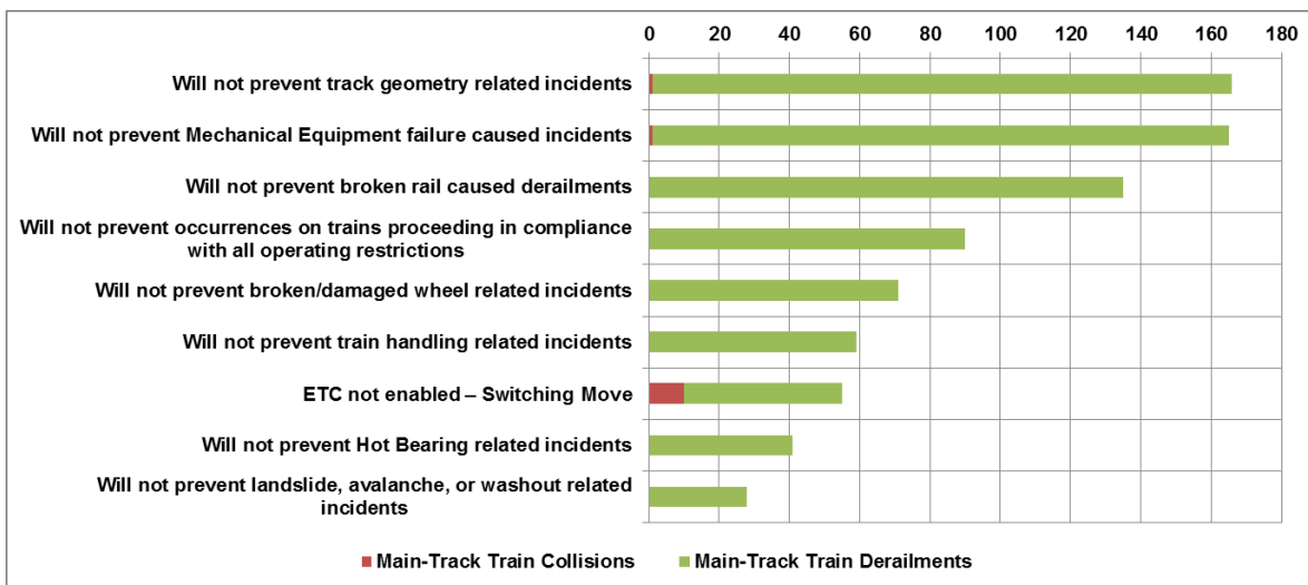
Figure 1-17. Breakdown of the most common reasons why main-track train accidents are not ETC-preventable. Red and green bars represent the main-track train collision and derailment contributions, respectively.
