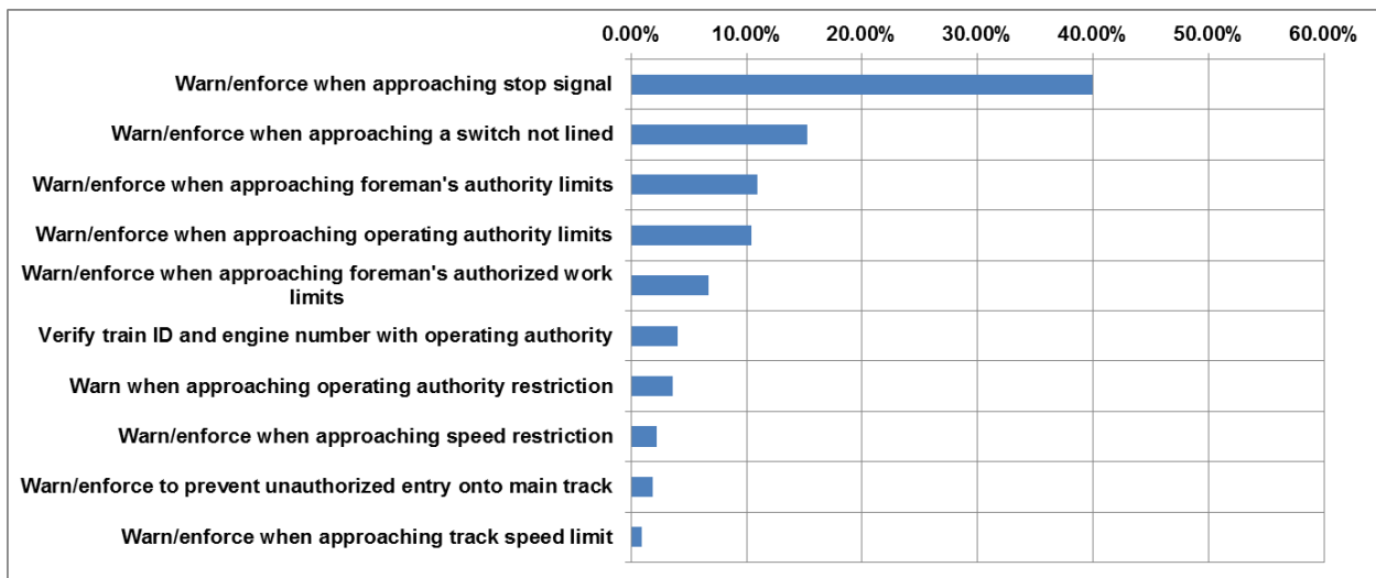
Figure 1-7. Breakdown in the key functionality of a Level 3 ETC system in terms of the number of preventable occurrences (642 in total).
