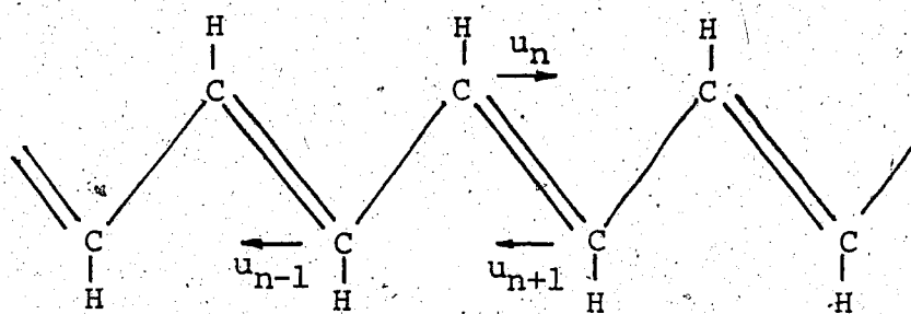
Fig. 2. B-phase of the trans-polyacetylene molecule.
