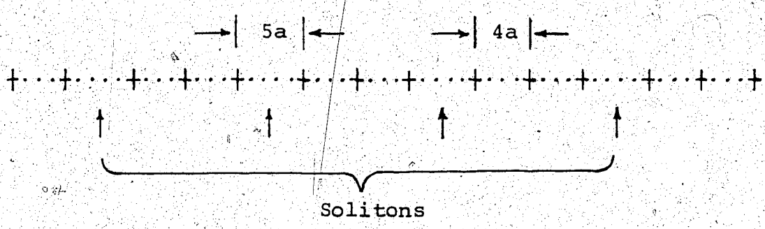
Fig. 5. Schematic structure of NbSe 3 with solitons.
