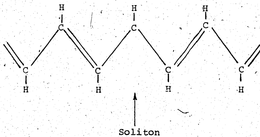
Fig. 3. Soliton in the chain structure of trans-polyacetylene.
