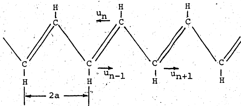
Fig. 1. A-phase of the trans-polyacetylene molecule.
