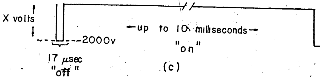
FIGURE 26 Pulsing Scheme for Drift Tube Studies.
