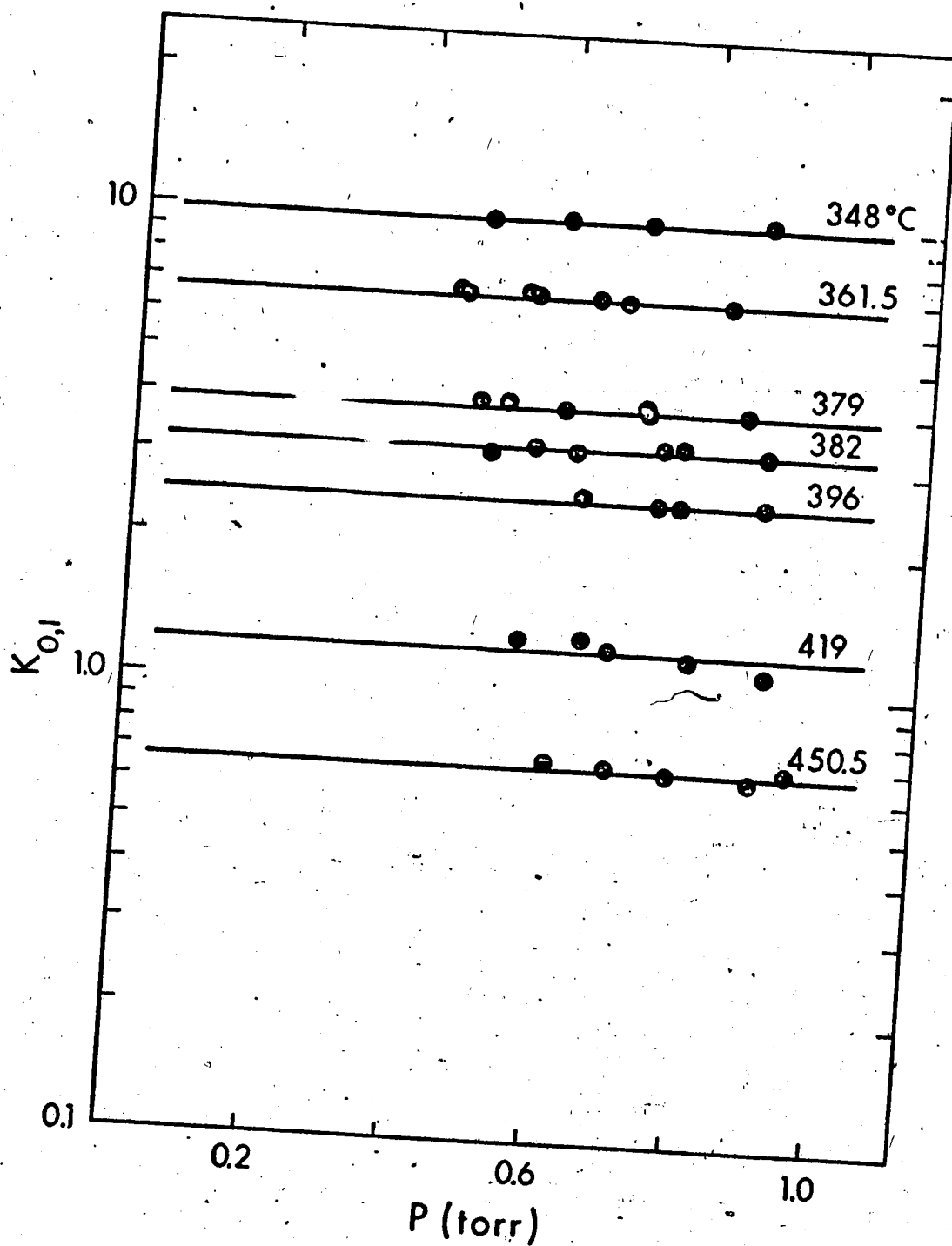
FIGURE 40 Equilibrium Constants versus Pressure of Acetonitrile at Various Temperatures for the Reaction:
