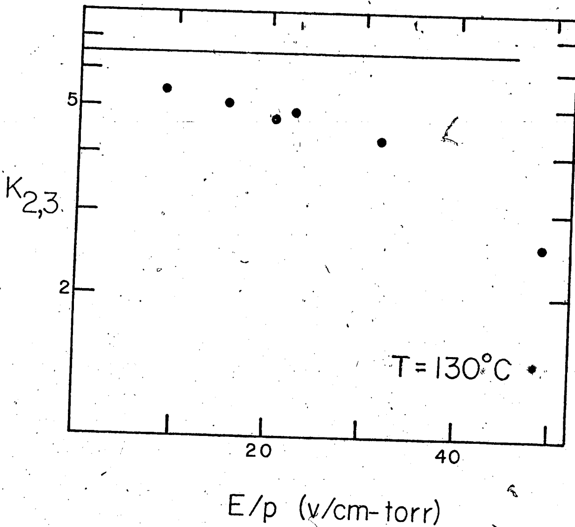
FIGURE 30 Variation of Equilibrium Constants with E/p for the Reaction:
