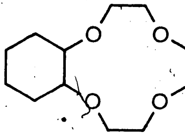
CYCLOHEXYL - 12 - CROWN - 4
