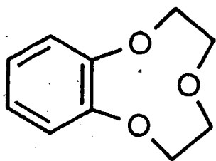
BENZO - 9 - CROWN - 3
