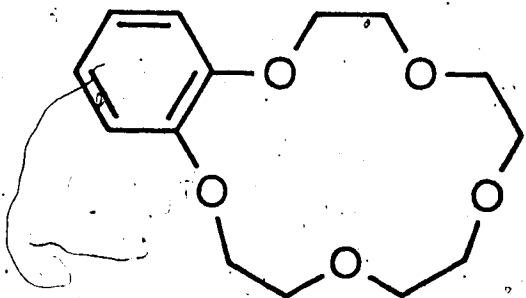
BENZO - 15 - CROWN - 5
