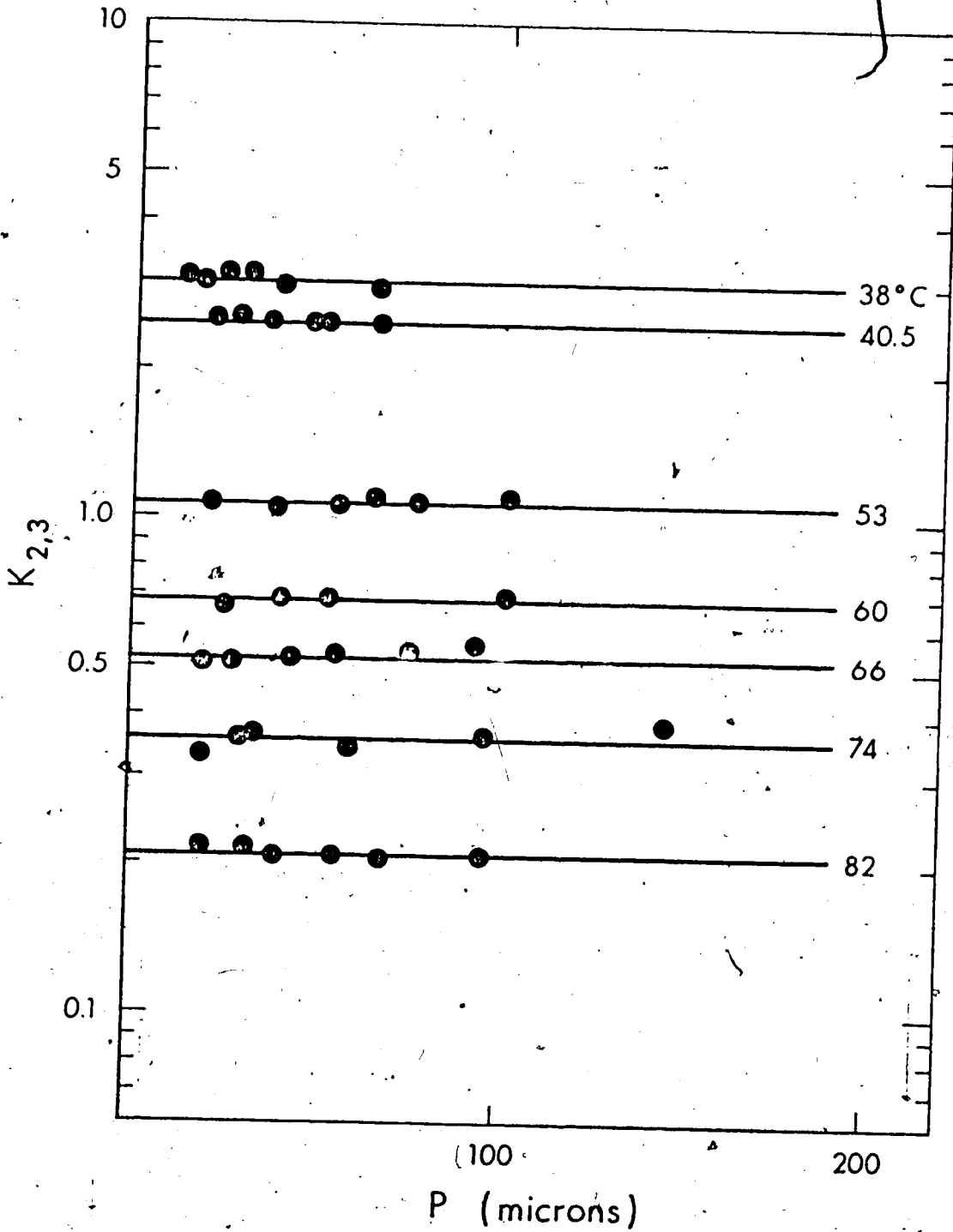
FIGURE 92 Equilibrium Constants versus Pressure of Ethylenediamine at Various Temperatures for the Reaction: K^+(en)_2 + en = K^+(en)_3 N_2 used as a third body.
