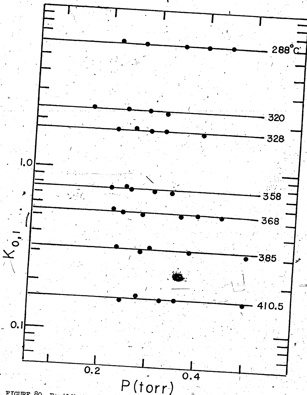
FIGURE 80 Equilibrium Constants versus Pressure at Various
