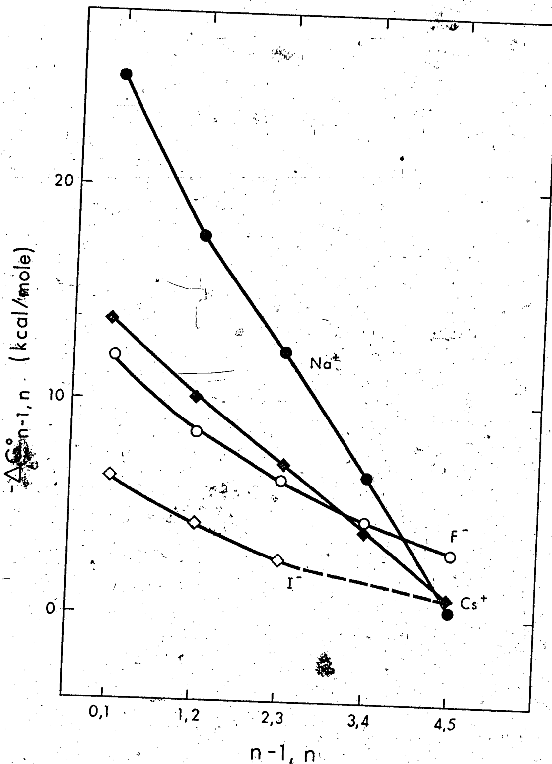
FIGURE 67 A Comparison of the Standard Free Energies of Gas Phase Solvation of Alkali and Halide Ions in Acetonitrile. Standard State: 1 atm. and 298° K.
