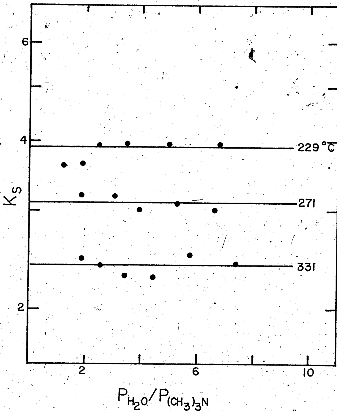
FIGURE 82 Switching Equilibrium Constants versus Pressure Ratio at Representative Temperatures for the Reaction: K^+(H_2O) + (CH_3)_3N = K^+((CH_3)_3N) + H_2O
