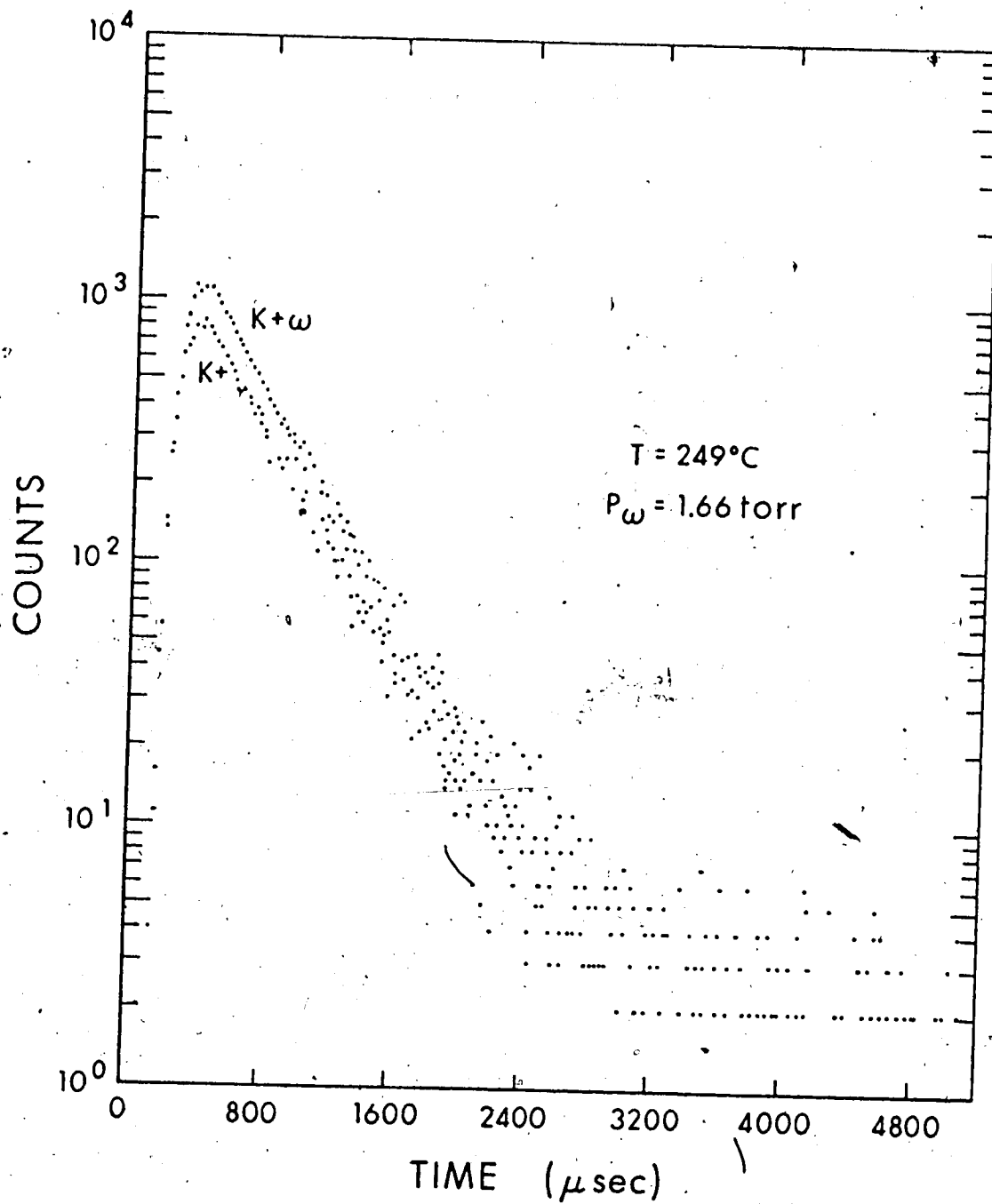
FIGURE 23 Time Dependent Output for the Reaction:
