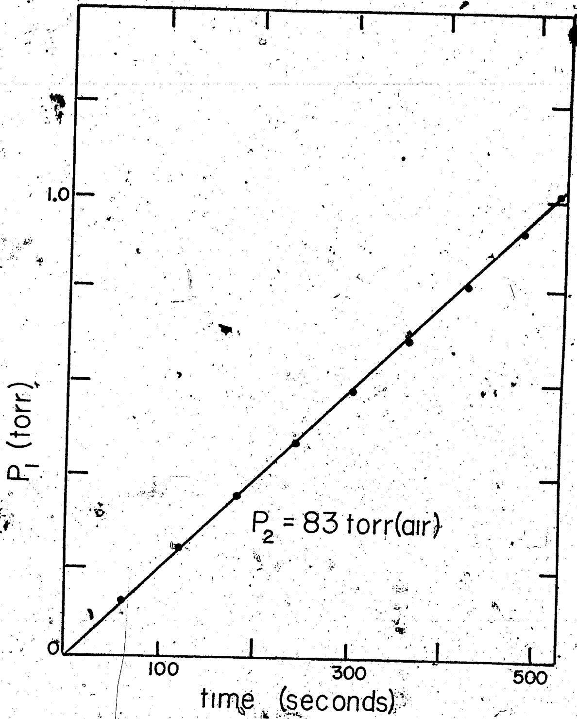
FIGURE 7 Calibration of Capillary Demonstrating Viscous Flow. (see text).
