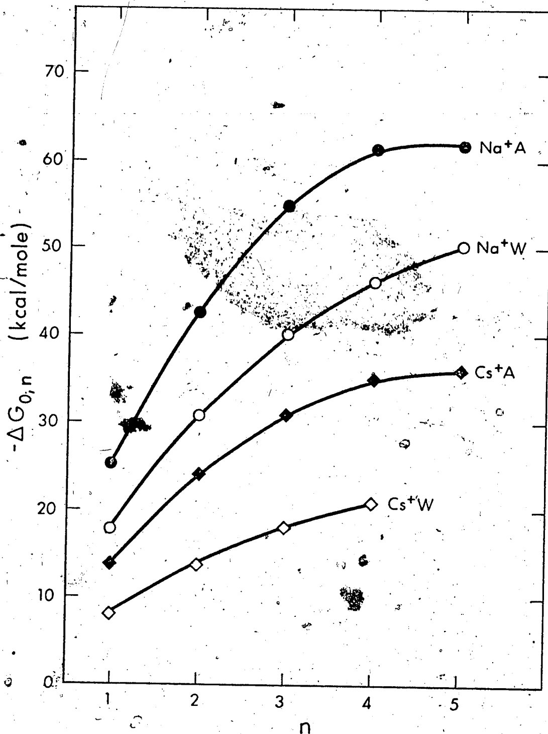
FIGURE 66. A Comparison of the Total Standard Free Energy of the Gas Phase Solvation of \text{Na}^+ and \text{Cs}^+ in Water and Acetonitrile versus the Number of Ligands. Standard State: 1 atm. and 298^\circ \text{K} .
