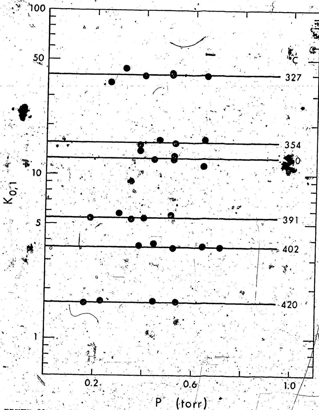
FIGURE 90 Equilibrium Constants versus Pressure at Various Temperatures for the Reaction:
