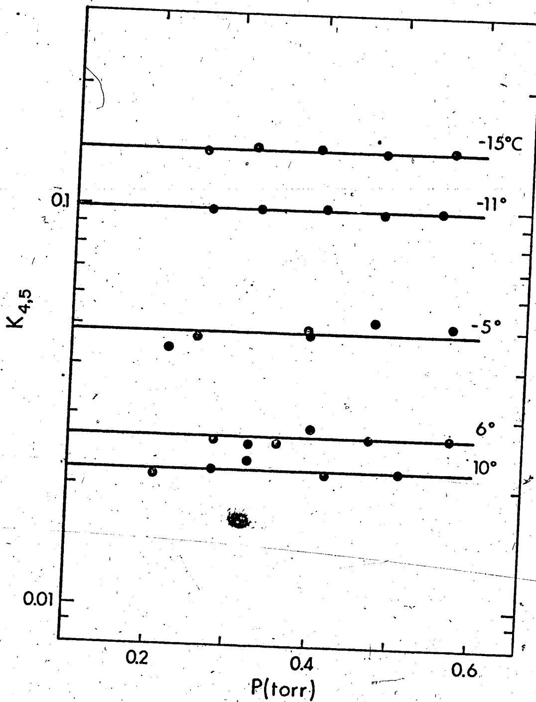
FIGURE 50 Equilibrium Constants versus Pressure of Acetonitrile at Various Temperatures for the Reaction:
