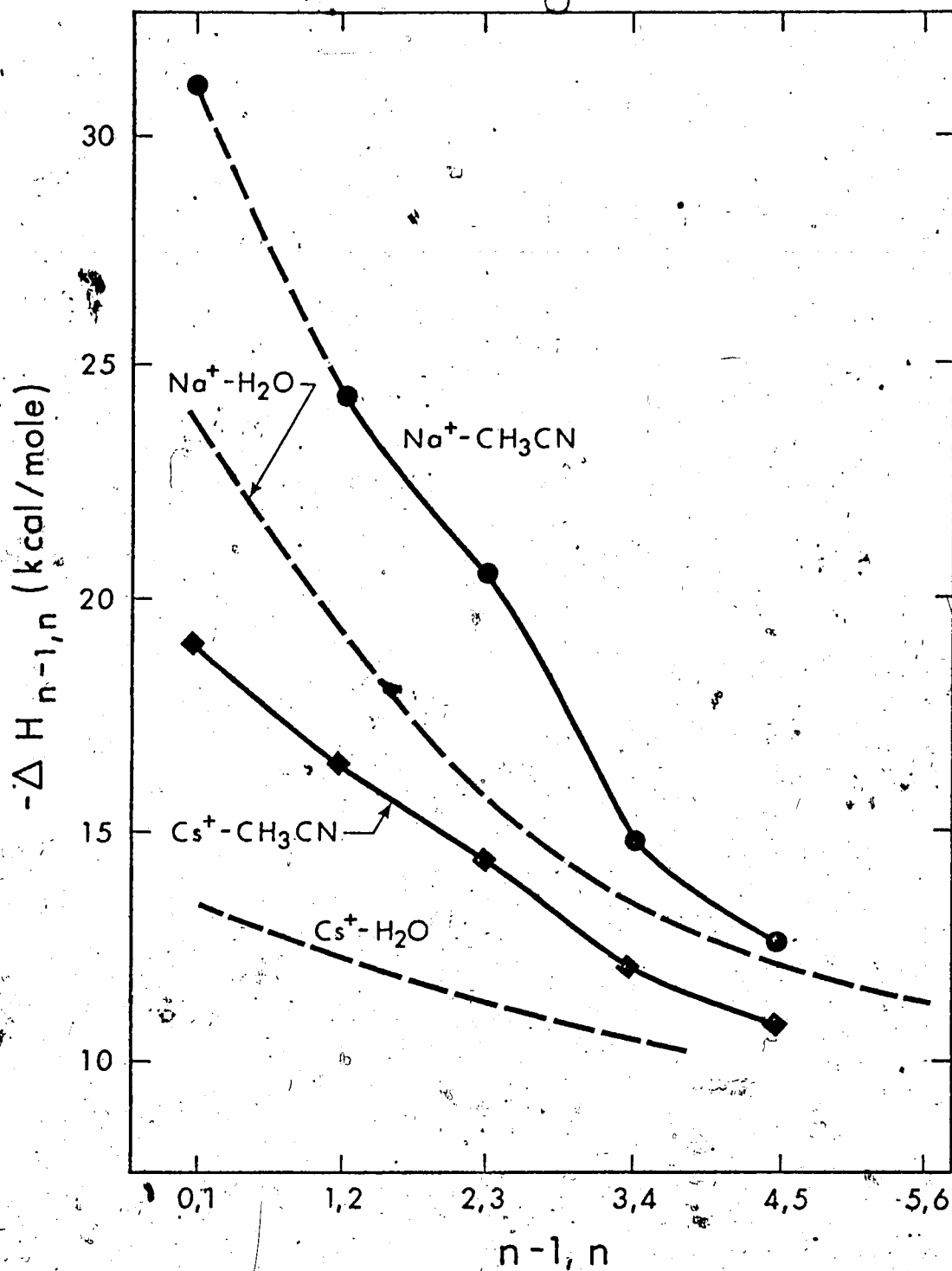
FIGURE 64 A Comparison of the Enthalpies of the Gas Phase Solvation of Na + and Cs + in Water and Acetonitrile.
