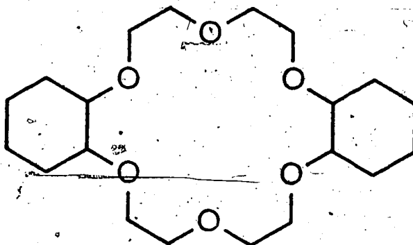
DICYCLOHEXYL - 18 - CROWN - 6
