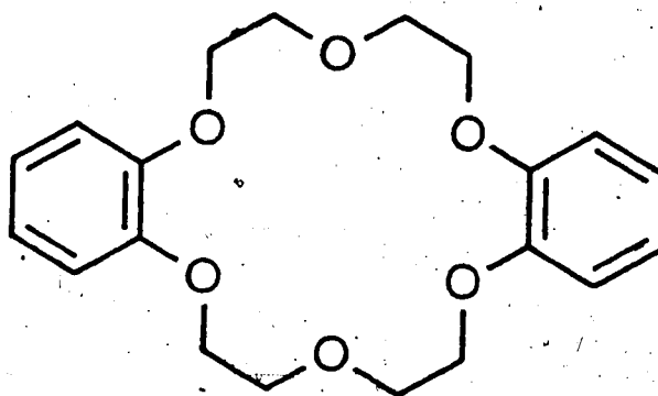
STRUCTURAL FORMULA
