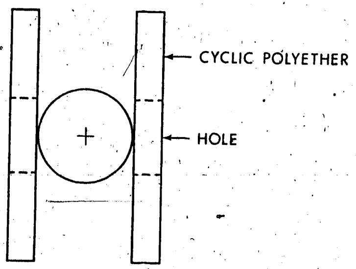
"SANDWICH" COMPLEX
