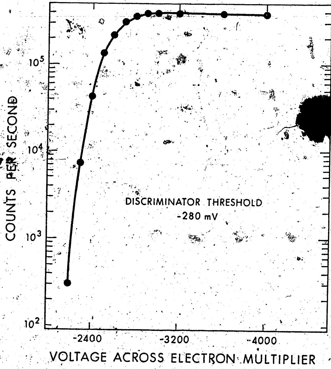
FIGURE 17 Counts per second versus Voltage Across Spiraltron Electron Multiplier.
