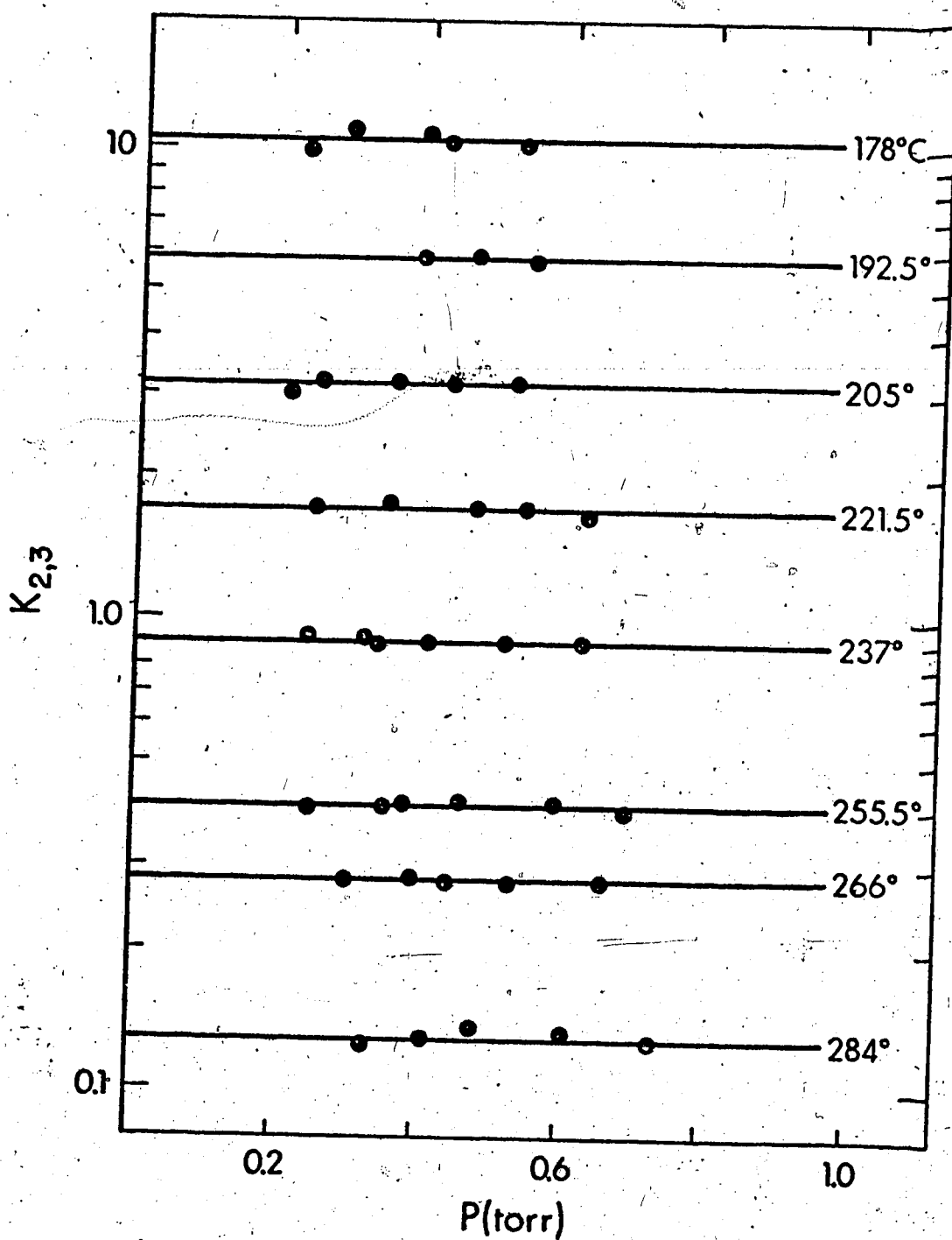
FIGURE 37 Equilibrium Constants versus Pressure of Acetonitrile at Various Temperatures for the Reaction:
