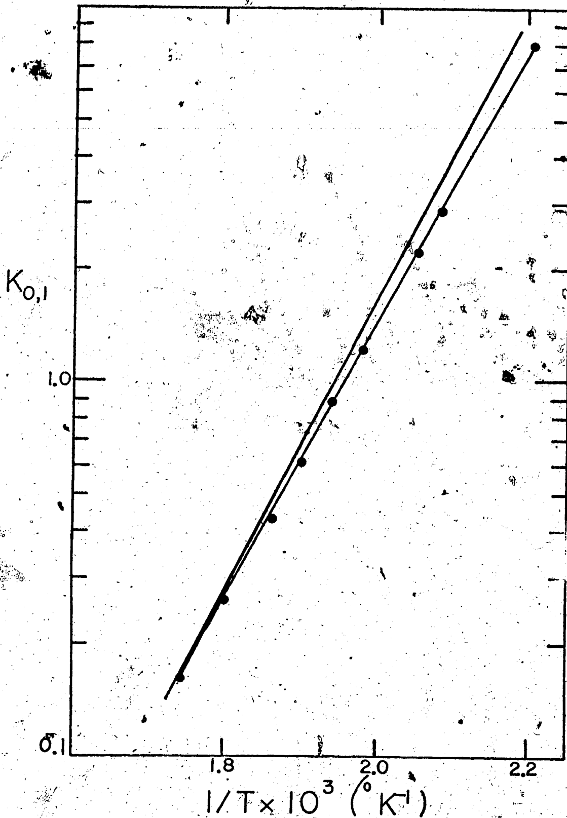
FIGURE 18 A Comparison of K_{0,1} Obtained in this Study (line with points) with that of Searles (solid line) versus 1/T for the Reaction:
