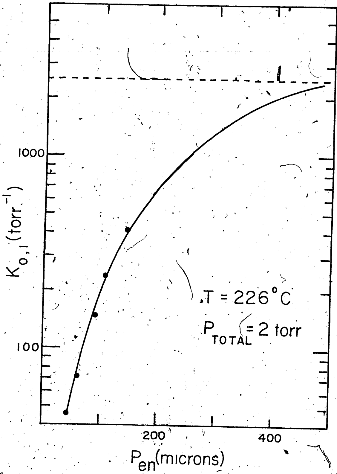
FIGURE 94 Plot of K_{O,1} for the Complexing of K^+ with Ethylenediamine versus Pressure of en, Demonstrating Non-equilibrium. Dashed line represents value from Van'Hoff Plot.
