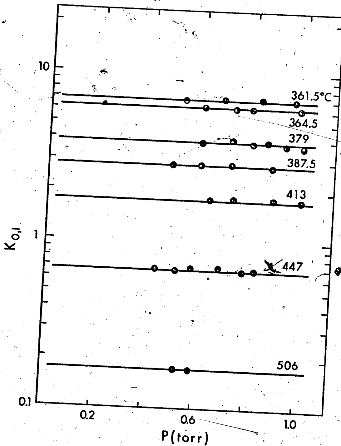
FIGURE 41 Equilibrium Constants versus Pressure of Acetonitrile at Various Temperatures for the Reaction:
