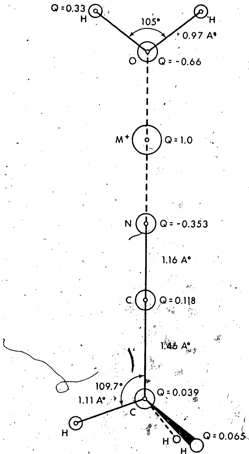
FIGURE 72 Bond Distances, Angles, and Point Charge Distribution for Water and Acetonitrile.
