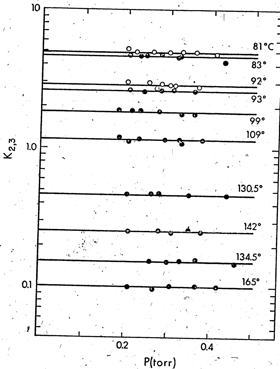
FIGURE 48 Equilibrium Constants versus Pressure of Acetonitrile at Various Temperatures for the Reaction:
