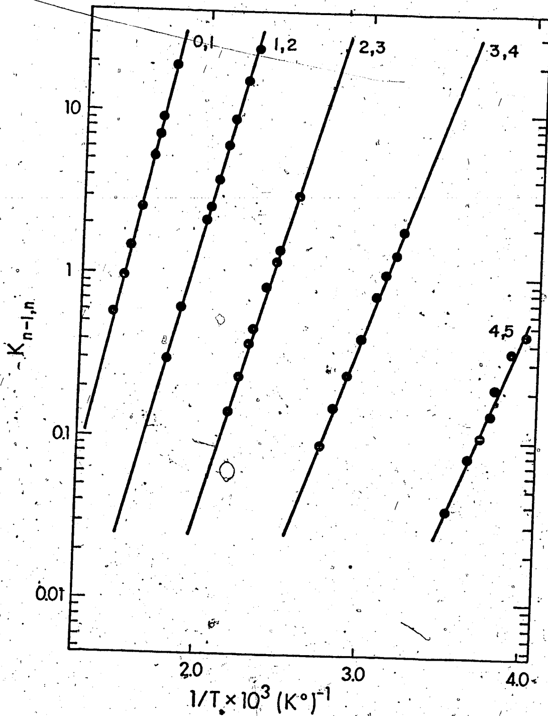
FIGURE 58 Van't Hoff Type Plots of the Equilibrium Constants for the Gas Phase Solvation of the Rubidium Ion by Acetonitrile.
