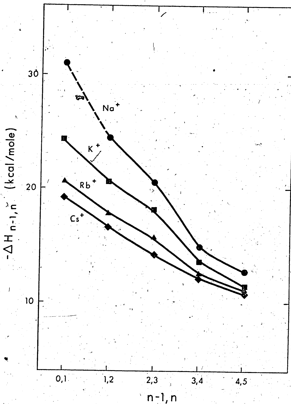
FIGURE 60 Enthalpies for the Clustering Reactions:
