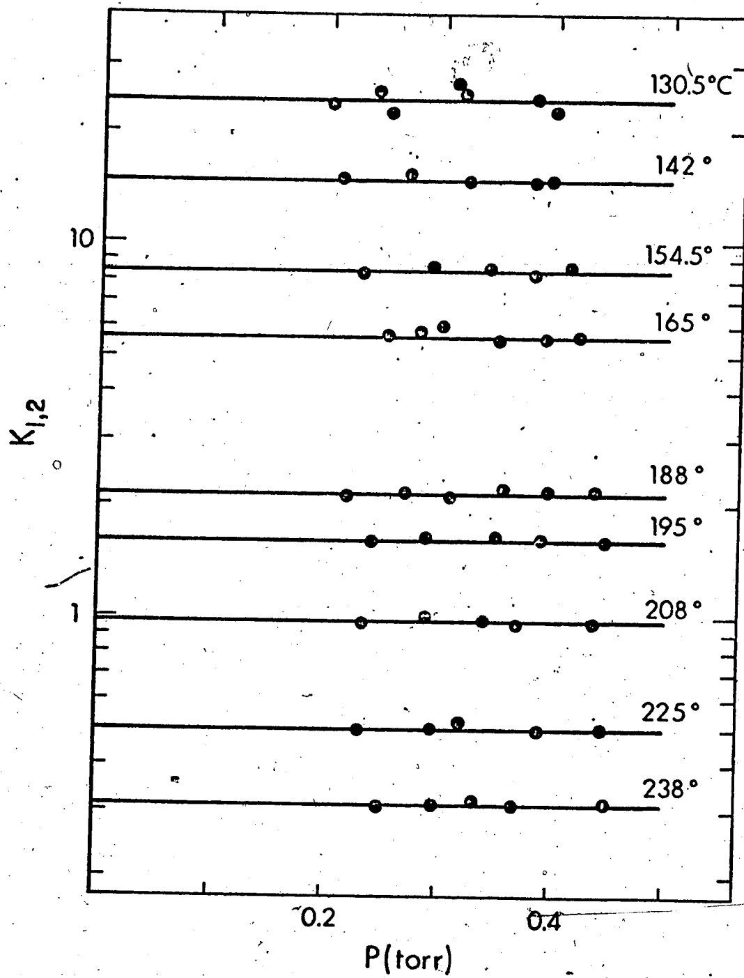
FIGURE 47 Equilibrium Constants versus Pressure of Acetonitrile at Various Temperatures for the Reaction:
