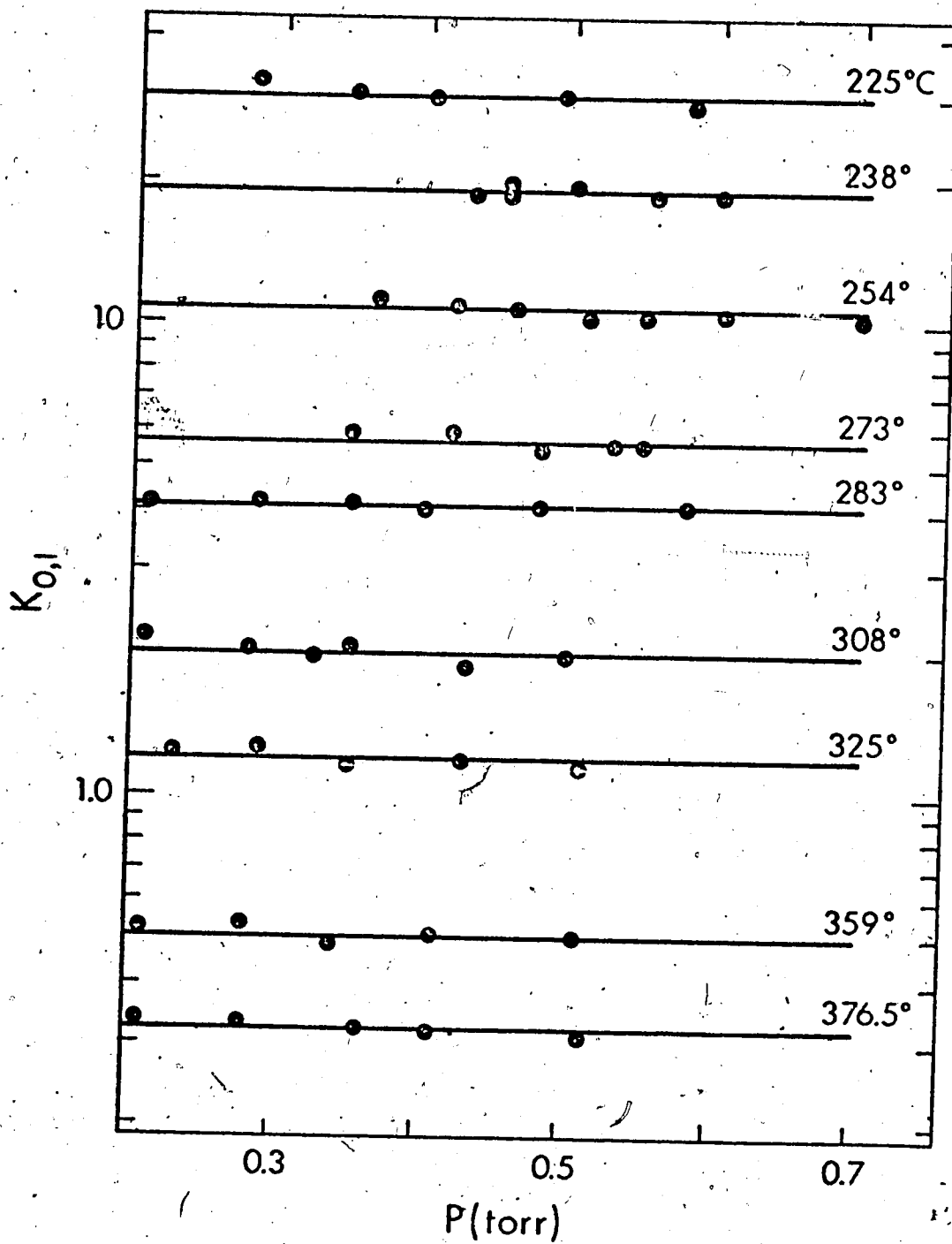
FIGURE 46 Equilibrium Constants versus Pressure of Acetonitrile at Various Temperatures for the Reaction: \text{Rb}^+ + \text{CH}_3\text{CN} = \text{Rb}^+(\text{CH}_3\text{CN})
