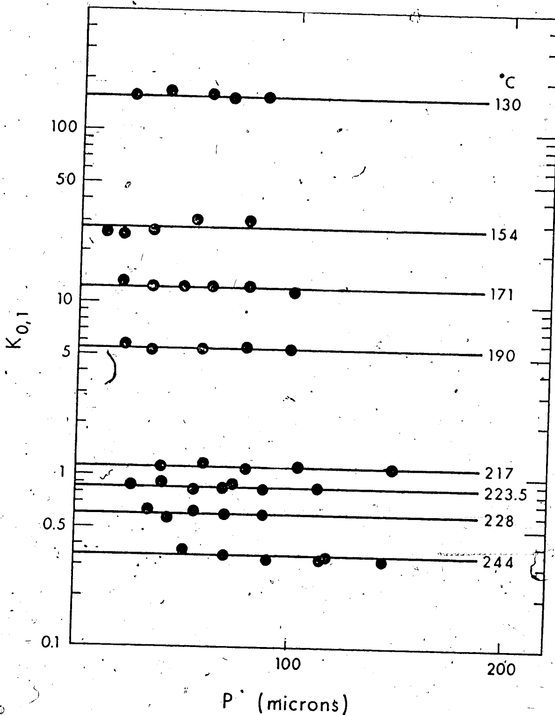
FIGURE 91 Equilibrium Constants versus Pressure at Various
