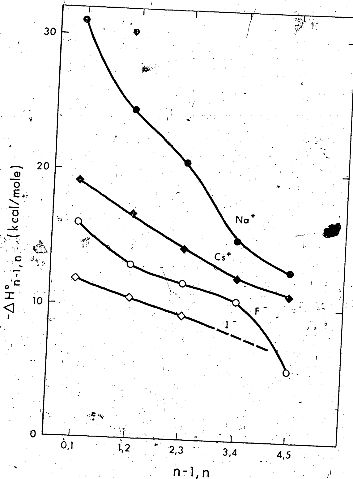
FIGURE 68 A Comparison of the Enthalpies of Gas Phase Solvation of Alkali and Halide Ions in Acetonitrile.
