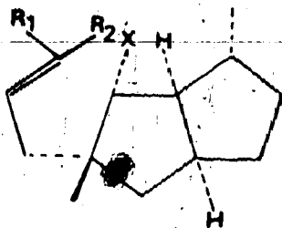
51 X = LEAVING GROUP R 1 , R 2 = CHO, CH 3
