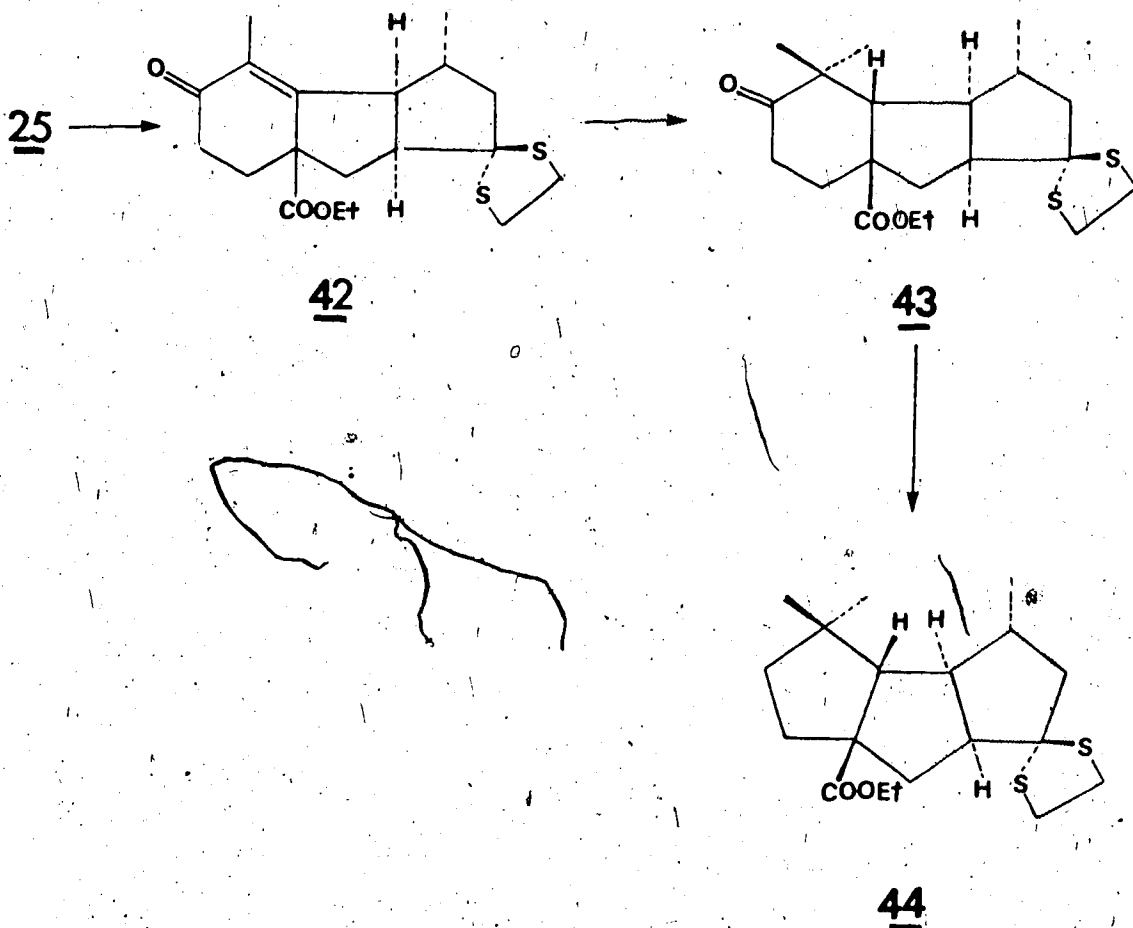
SCHEME III
