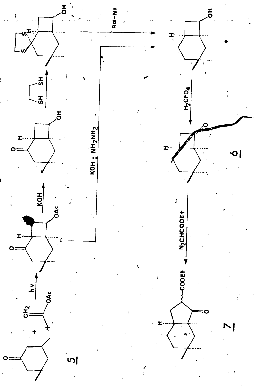
SCHEME I
