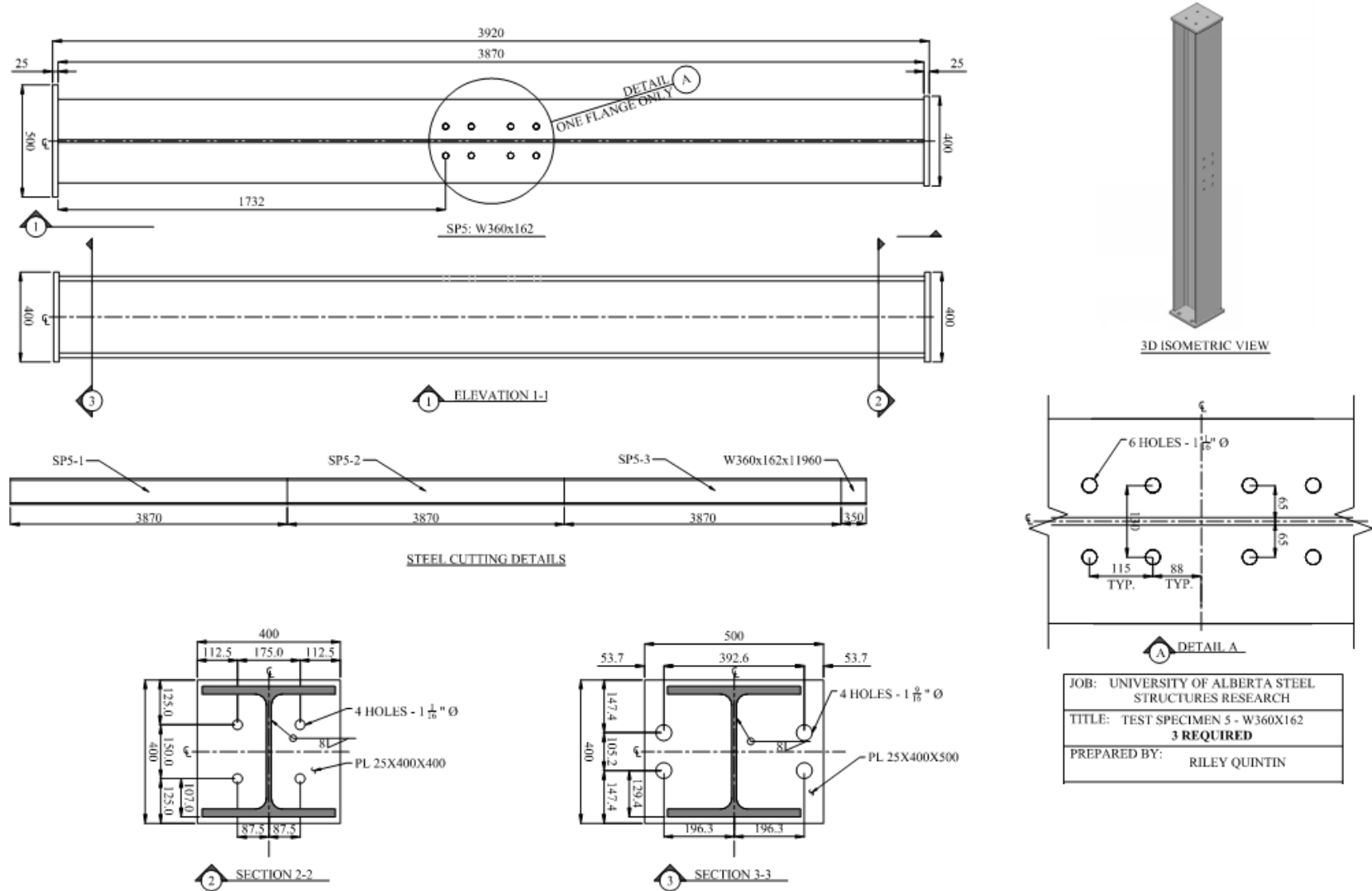
Figure A.5: Drawing SP5
