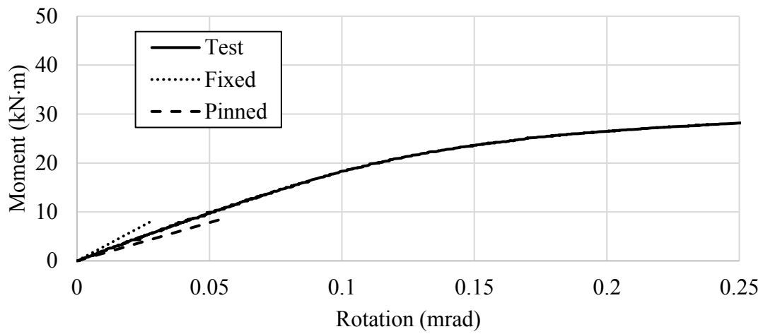
Figure 5.6: Evaluation of Torsional Boundary Conditions for W250×89 (50% Axial Load)
