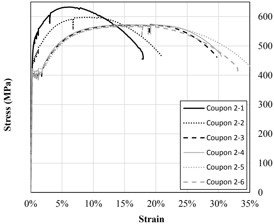
Figure B.2: Stress–Strain Curves for Coupons SP2
