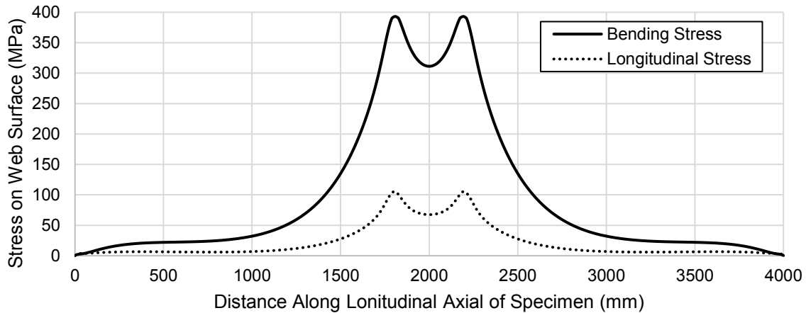
Figure 3.9: W250x89 Stress Components Under Zero Applied Axial Load
