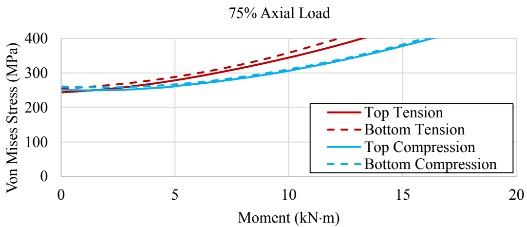
Figure 4.11: W360×162 Von Mises Stress Under Different Levels of Axial Load
