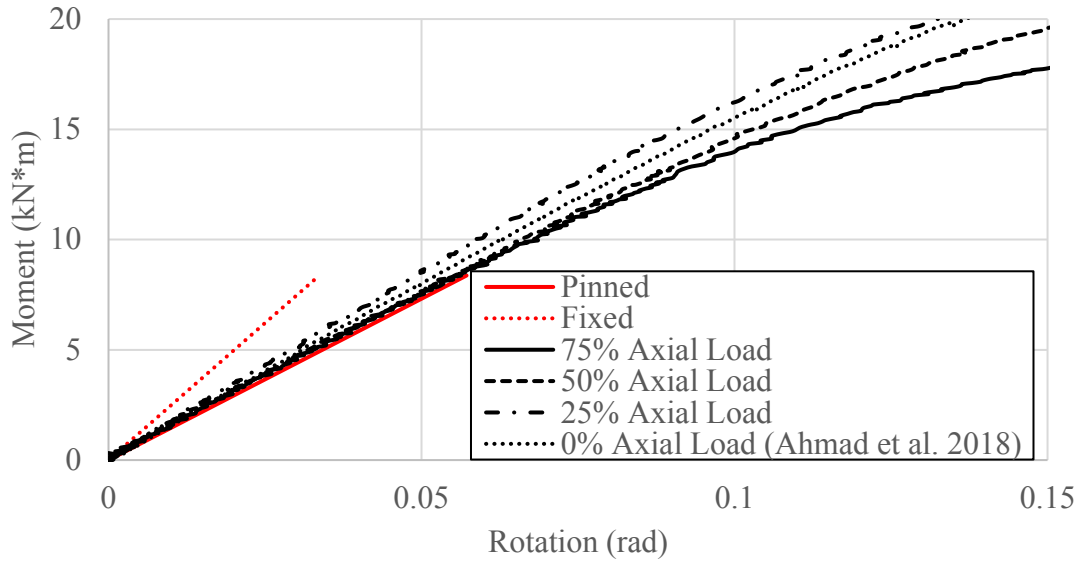
Figure 5.2: W310x86 Moment–Rotation Comparison
