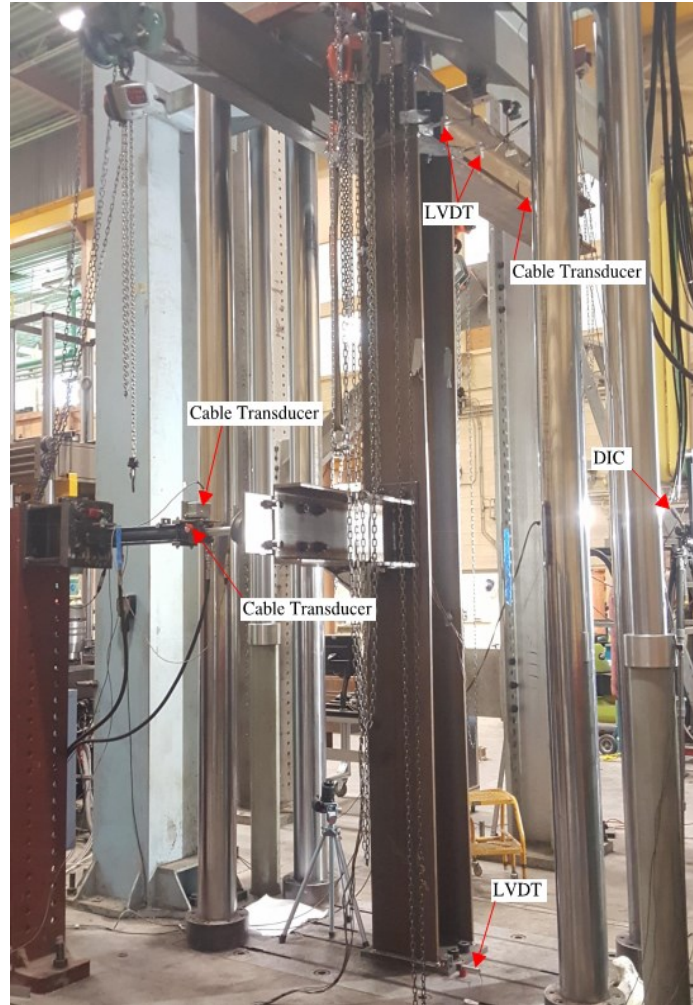
Figure 4.7: Instrumentation Details
