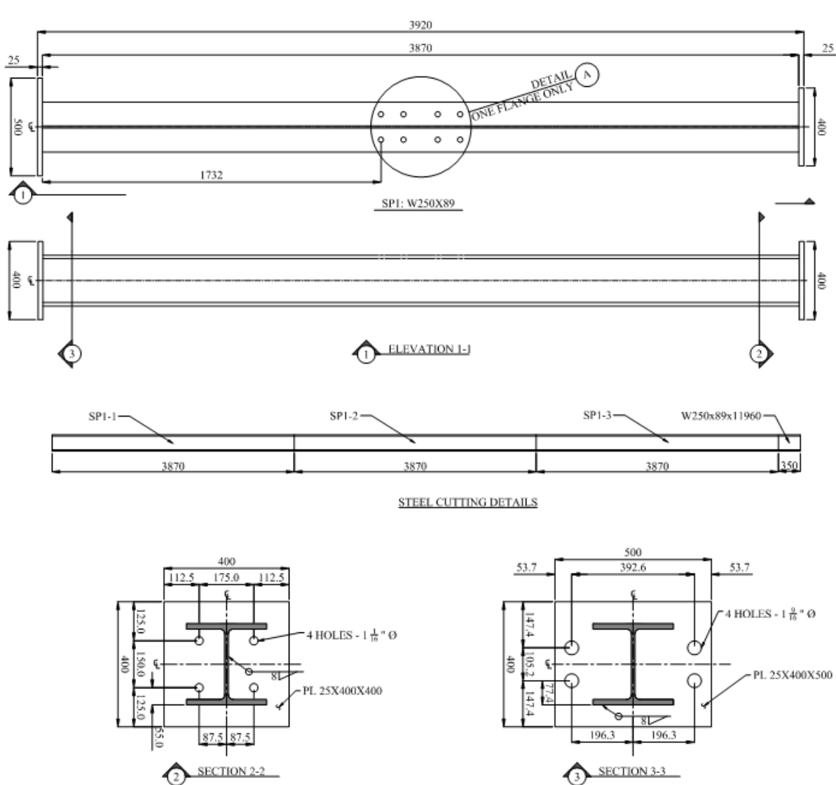
Figure A.1: Drawing SP1
