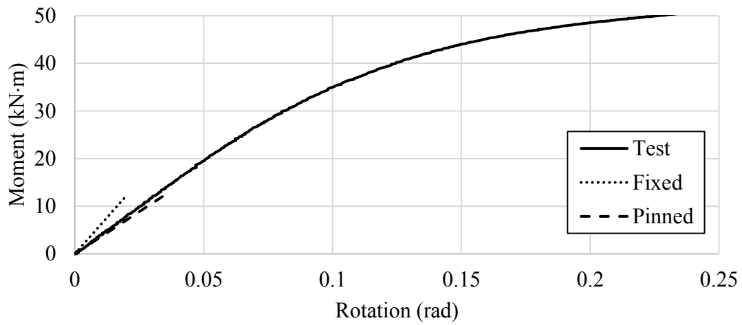
Figure 5.15: Evaluation of Torsional Boundary Conditions for W310×129 (50% Axial Load)
