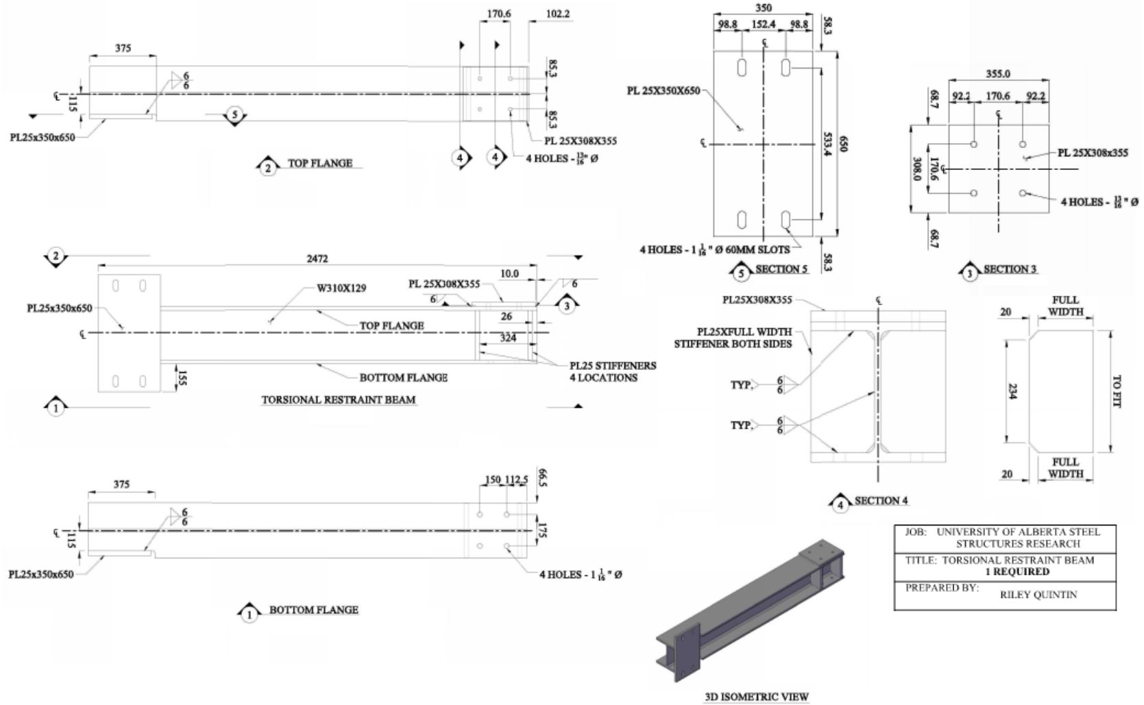
Figure A.6: Drawing Torsional Restraint Beam
