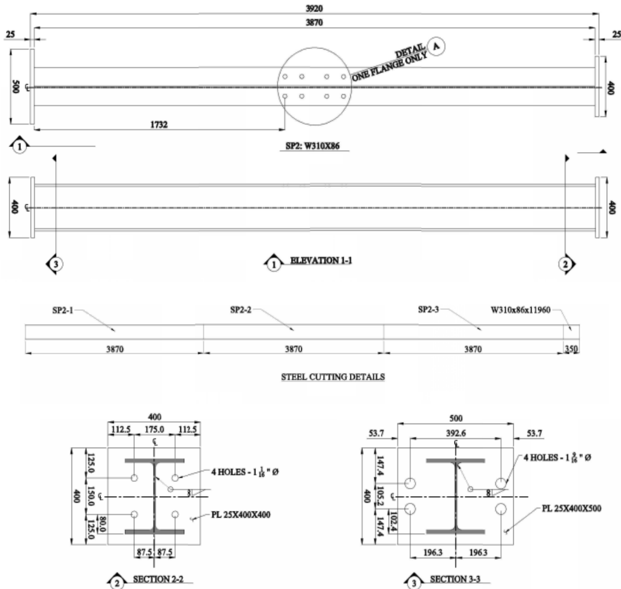
Figure A.2: Drawing SP2
