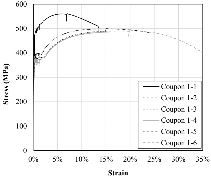
Figure B.1: Stress–Strain Curves for Coupons SP1
