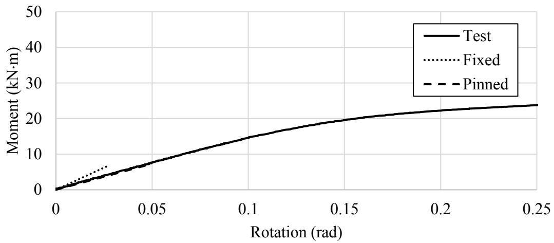
Figure 5.12: Evaluation of Torsional Boundary Conditions for W310×86 (50% Axial Load)
