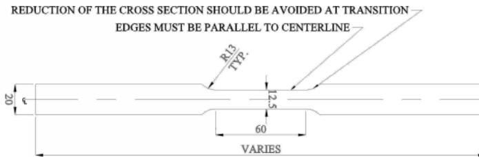
TENSION COUPON DETAILS (RELEVANT FOR ALL COUPONS)
