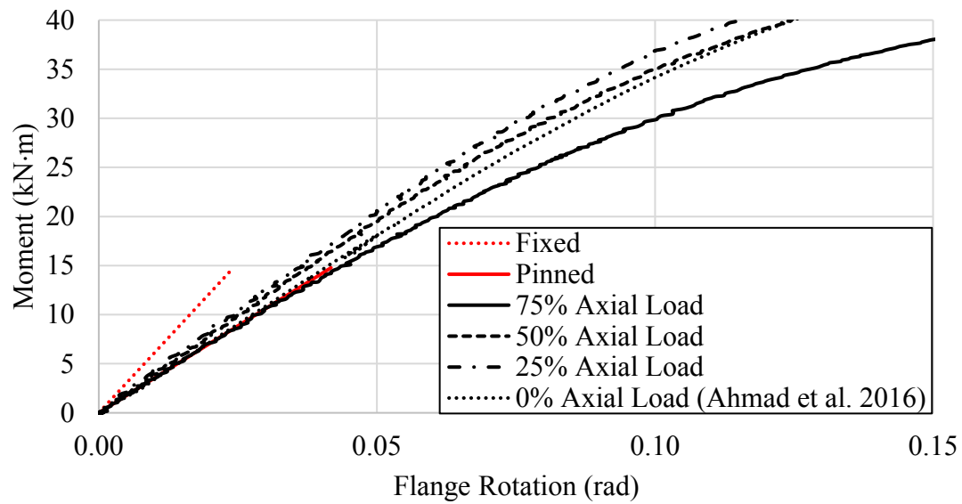
Figure 5.3: W310x129 Moment–Rotation Comparison
