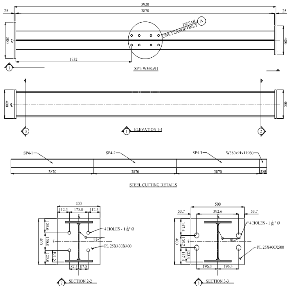
Figure A.4: Drawing SP4
