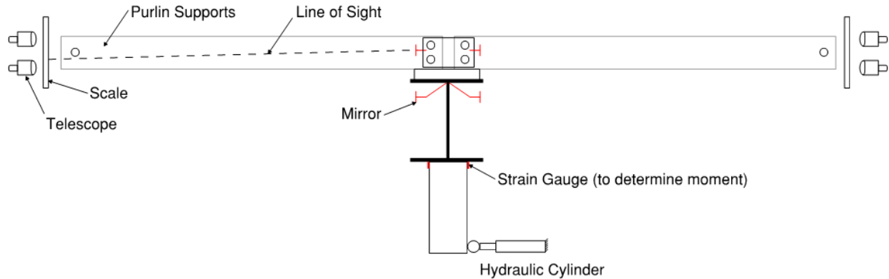
Figure 2.2: Test Setup for I-Shaped Members Braced by Lipped Chanel Purlins (Adapted from Milner and Rao (1978))
