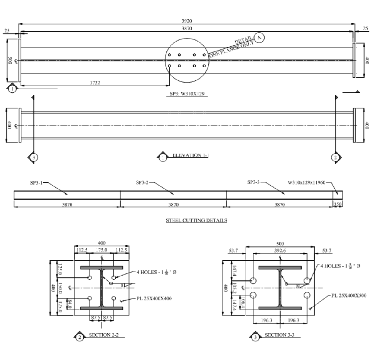
Figure A.3: Drawing SP3
