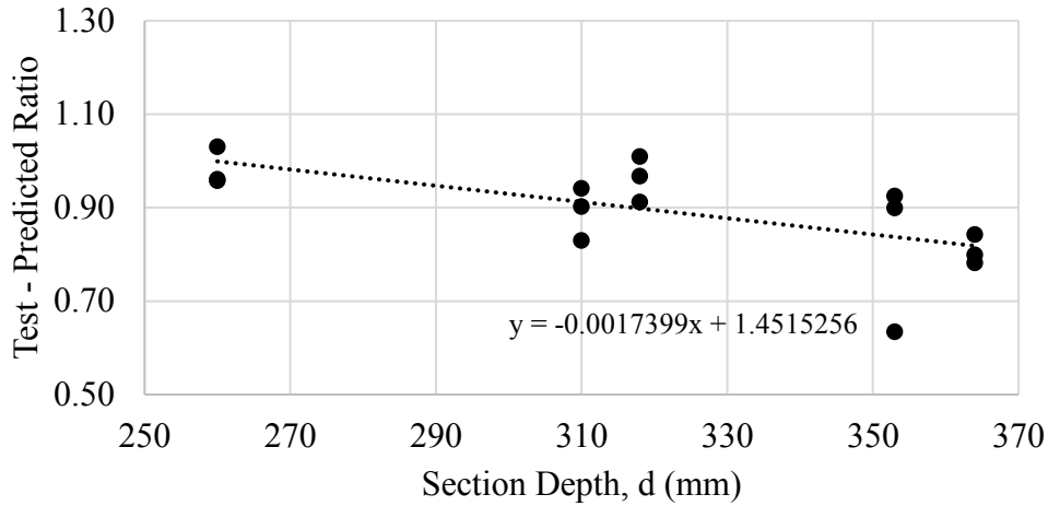
Figure 5.1: Effect of Section Depth on Test-to-Predicted Ratios of Equation 3-4
