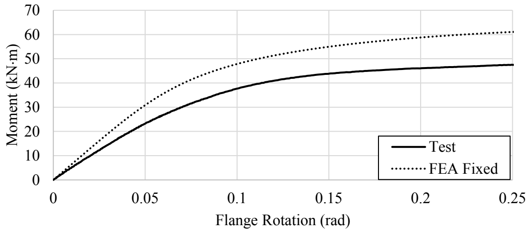
Figure C.10: Moment–Rotation Response for SP5-3
