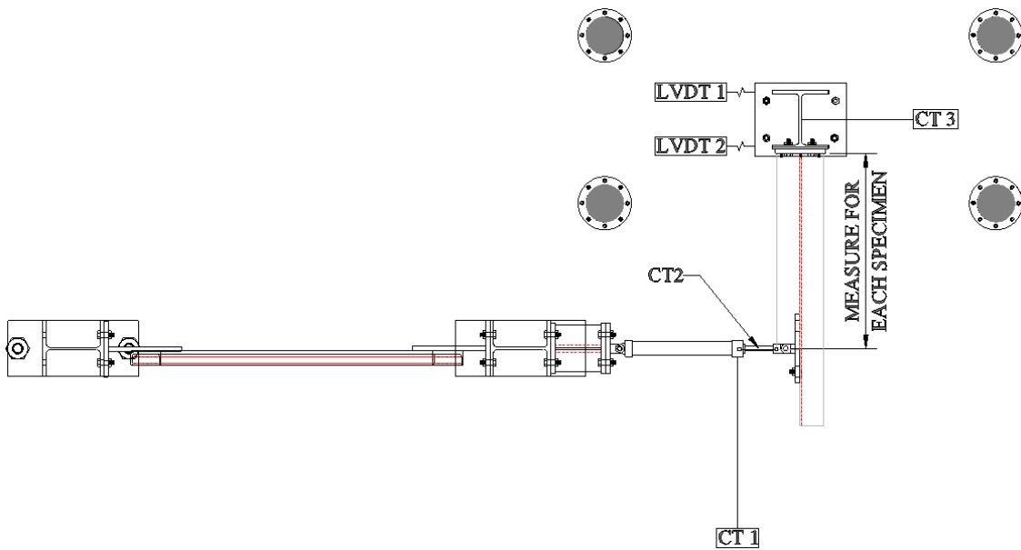
Figure 4.6: Instrumentation Layout
