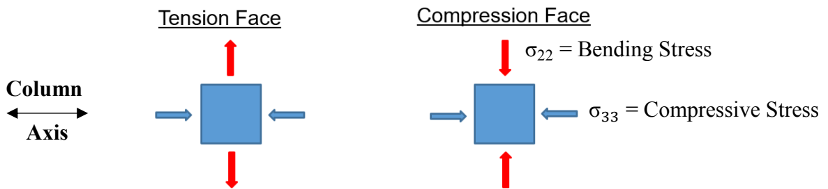
Figure 3.7: Web Surface Stress States
