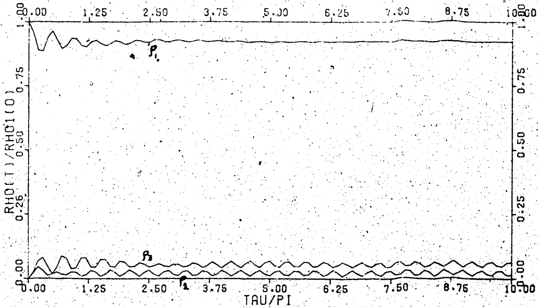
Fig. A.7. r_2 = 3. ; r_3 = 5. ; \frac{m_1}{m_2} = \frac{m_1}{m_3} = 0. ; U_1 = 1. ; U_2 = 5. ; \delta = 1.
