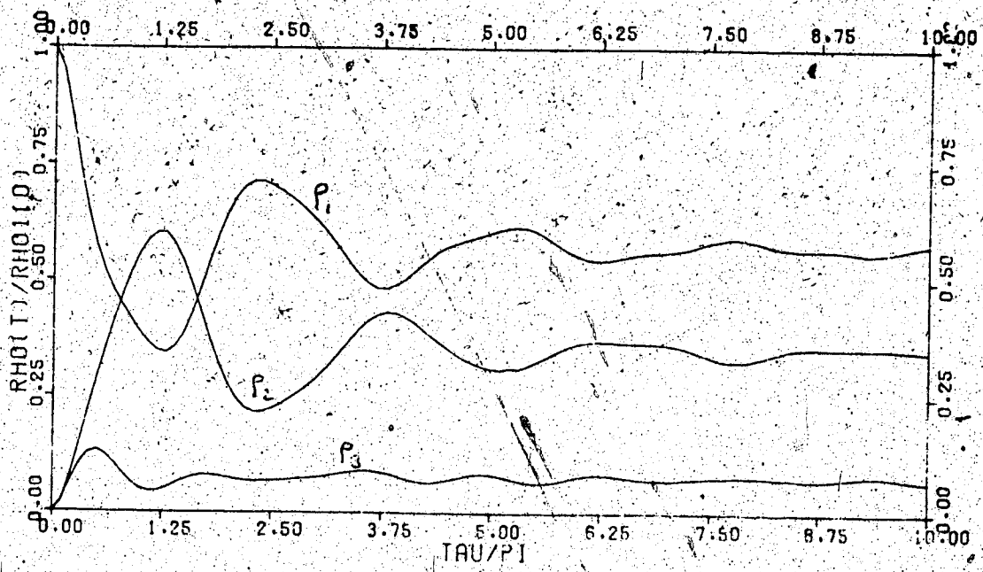
Fig. 2.9(d) r_2 = r_3 = 1. ; \frac{m_1}{m_2} = 0. ; \frac{m_1}{m_3} = 5. ; U_1 = U_2 = \delta = 1.
