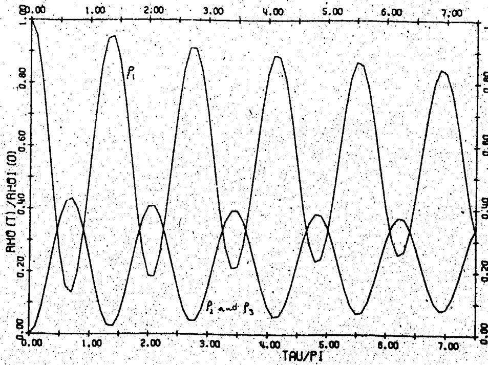
Fig. 2.8(a) \frac{m_1}{m_2} = \frac{m_1}{m_3} = 0 ; r_2 = r_3 = \delta = U_1 = 1 ; U_2 = 0 .
