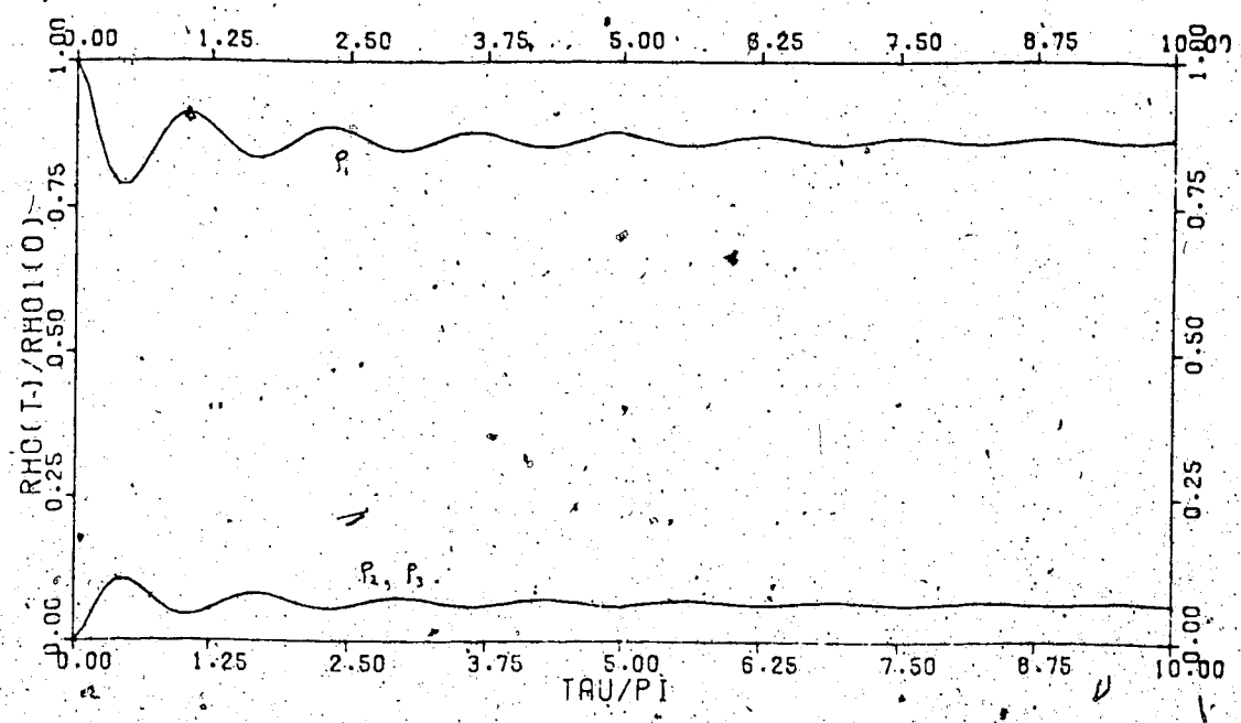
Fig. A.14. r_2 = r_3 = 1. ; \frac{m_1}{m_2} = \frac{m_1}{m_3} = 5. ; U_1 = 1. ; U_2 = 0. ; \delta = 1.
