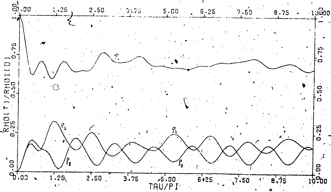
Fig. A.4. r_2 = 3. ; r_3 = 5. ; \frac{m_1}{m_2} = \frac{m_1}{m_3} = 0. ; U_1 = U_2 = 1. ;
