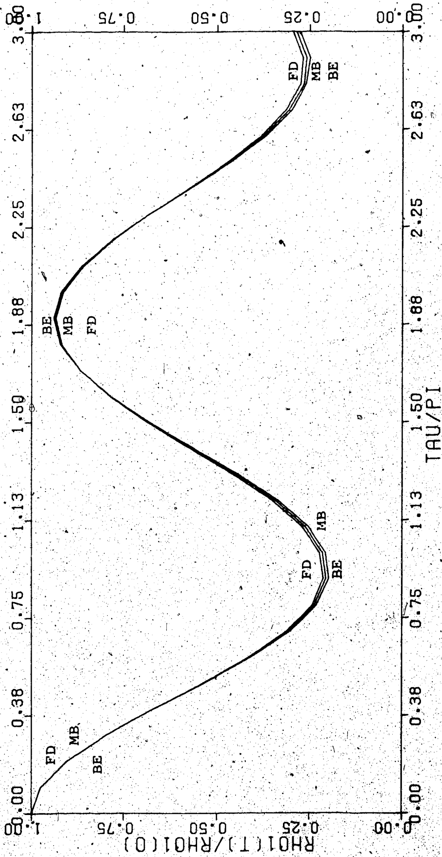
Fig. 5.2. r = 1. ; \delta = 1. ; \gamma = 0.2. ; Density oscillations in a weakly degenerate system.
