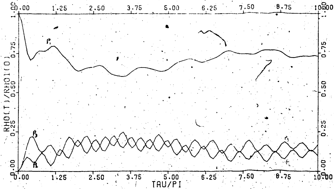
Fig. A.6. r_2 = 3. ; r_3 = 5. ; \frac{m_1}{m_2} = \frac{m_1}{m_3} = 0. ; U_1 = 1. ; U_2 = 3. ; \delta = 0.5.
