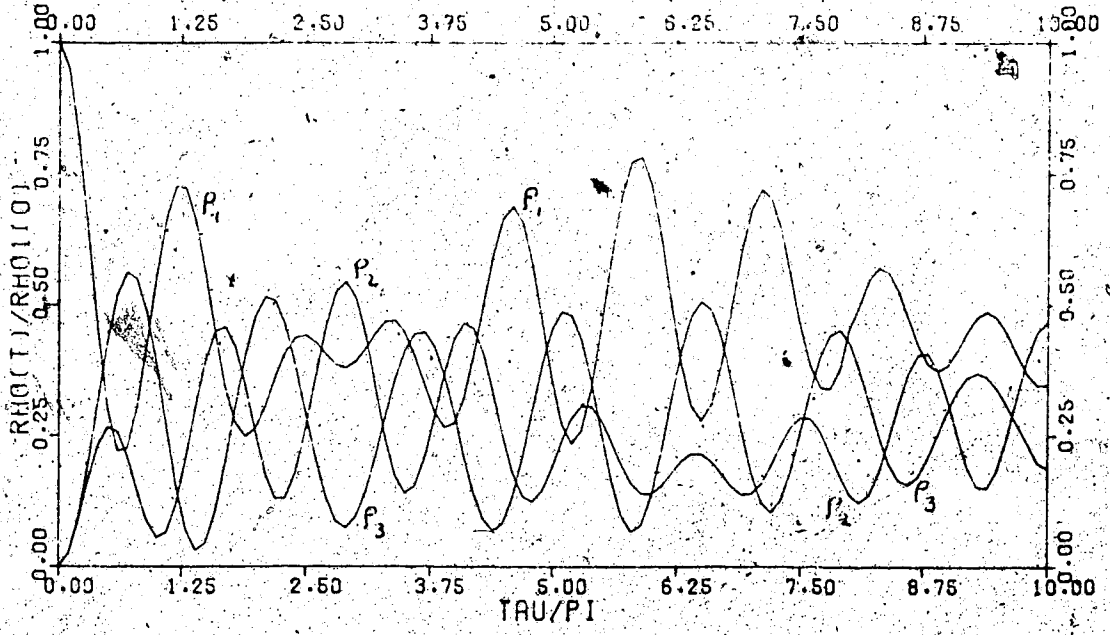
Fig. 2.9(c) r_2 = r_3 = 1. ; \frac{m_1}{m_2} = 0. ; \frac{m_1}{m_3} = 1. ; U_1 = U_2 = \delta = 1.
