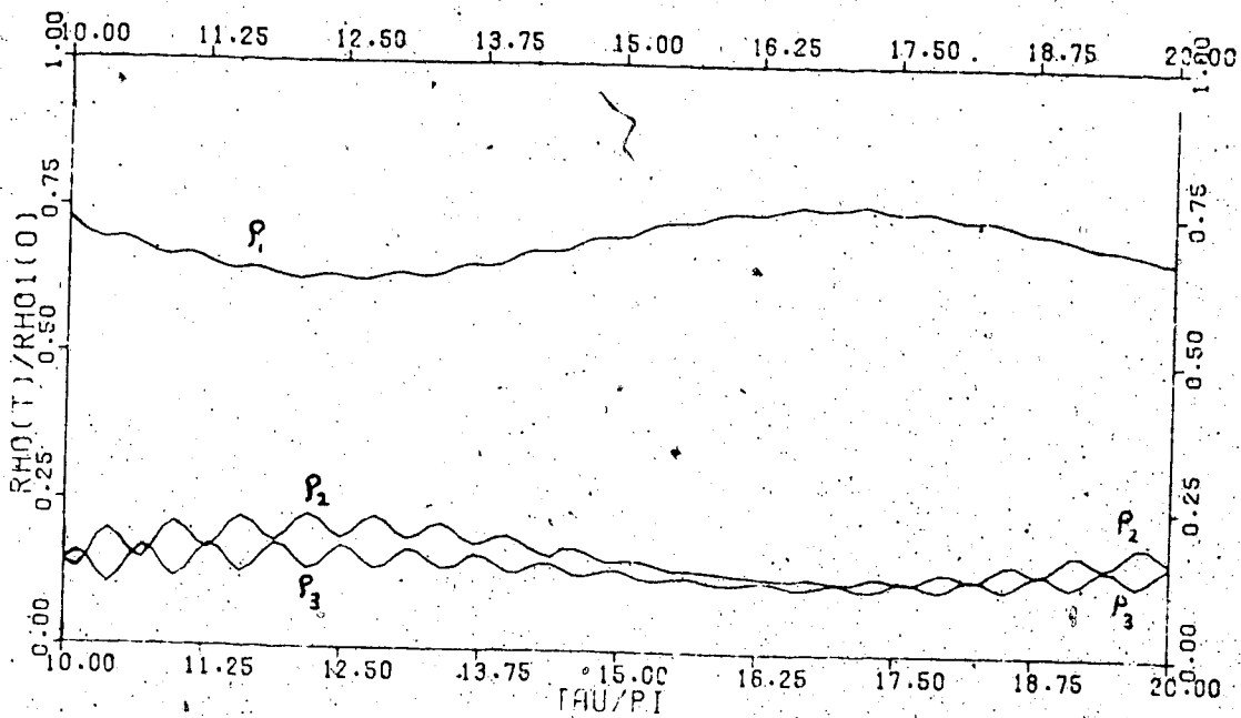
FIG. A.1. r_2 = 3. ; r_3 = 5. ; \frac{m_1}{m_2} = \frac{m_1}{m_3} = 0. ; U_1 = 1. ; U_2 = 3. ; \delta = 1.
