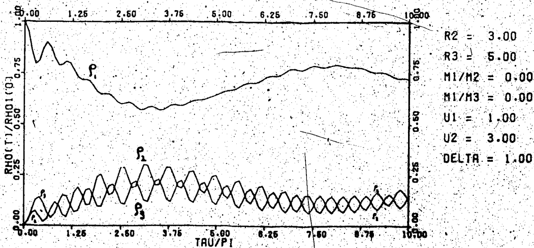
Fig. 2.7(b) Exact solution.
