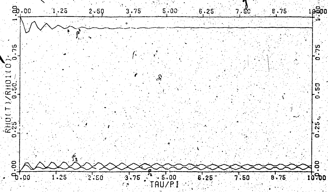
Fig. A.9. r_2 = 4. ; r_3 = 5. ; \frac{m_1}{m_2} = \frac{m_1}{m_3} = 0. ; U_1 = 1. ; U_2 = 5. ; \delta = 1.
