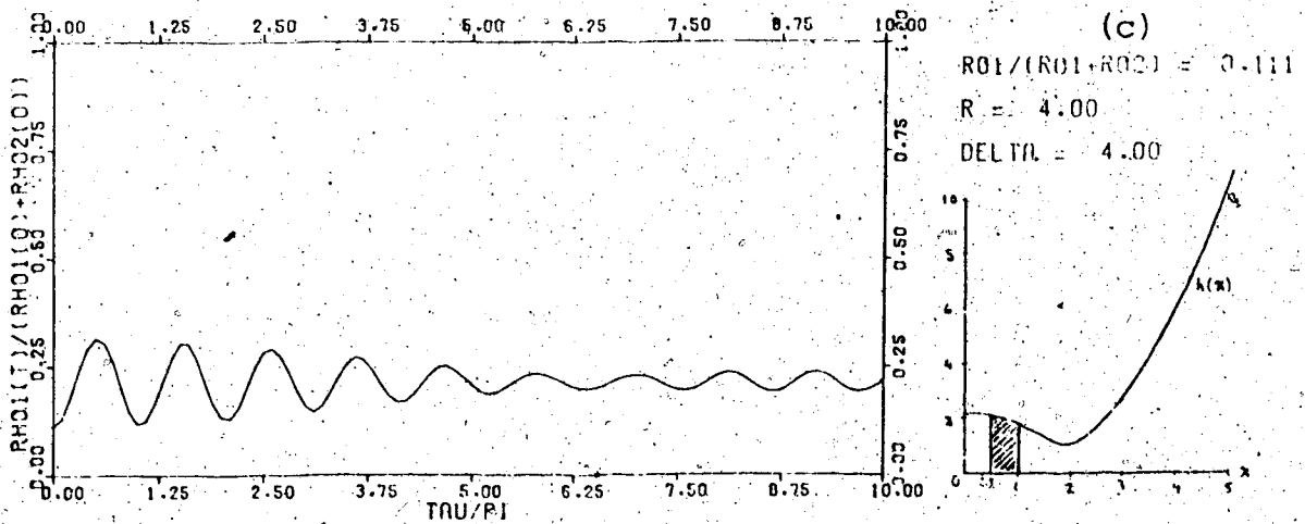
Fig. 3.1. Examples of zero temperature oscillations.
