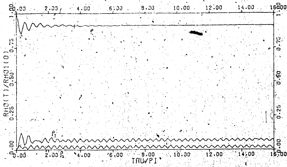
Fig. A.8. r_2 = 1. ; r_3 = 5. ; \frac{m_1}{m_2} = \frac{m_1}{m_3} = 0. ; U_1 = 1. ; U_2 = 5. ; \delta = 1.
