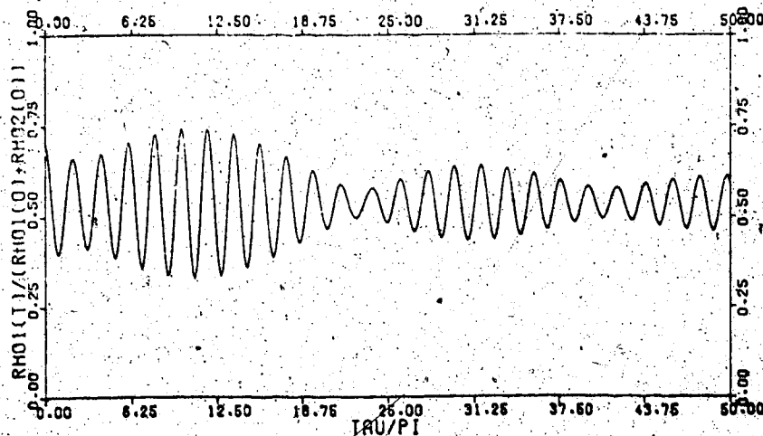
Fig. 4.3. Examples of the two-temperature model with \gamma large.
