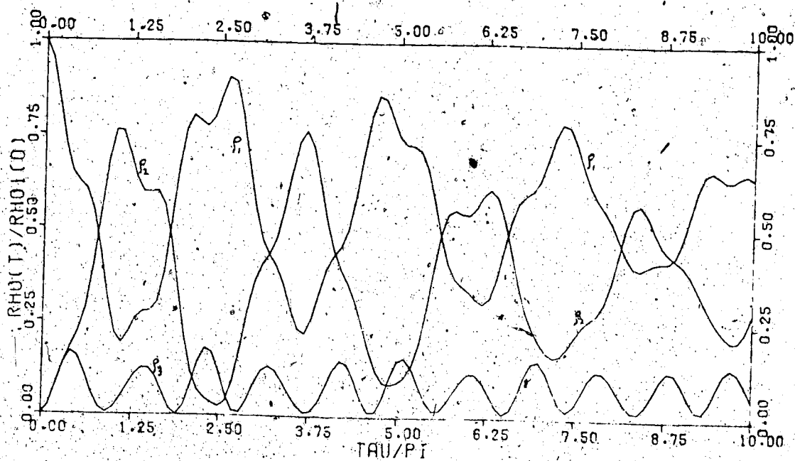
Fig. A.10. r_2 = 1. ; r_3 = 5. ; \frac{m_1}{m_2} = \frac{m_1}{m_3} = 0. ; U_1 = U_2 = 1. ; \delta = 5.
