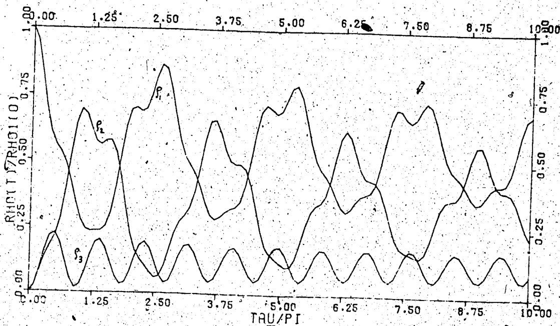
Fig. A.11. r_2 = 1. ; r_3 = 5. ; \frac{m_1}{m_2} = 0. ; \frac{m_1}{m_3} = 0.5. ; U_1 = U_2 = \delta = 1.
