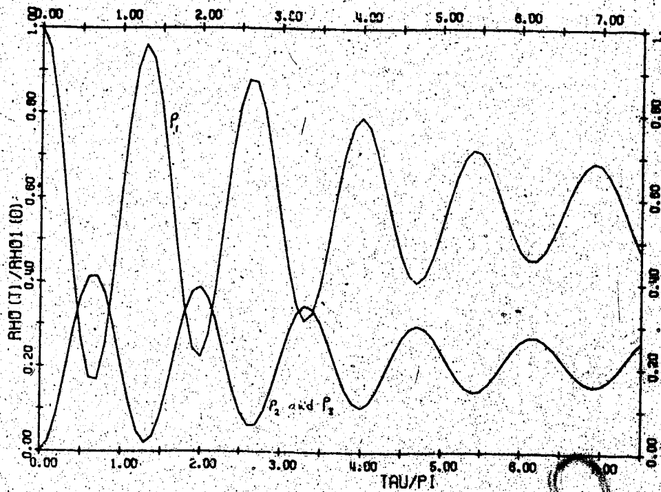
Fig. 2.8(b) \frac{m_1}{m_2} = \frac{m_1}{m_3} = 0 ; r_2 = r_3 = \delta = U_1 = 1 ; U_2 = 1 .
