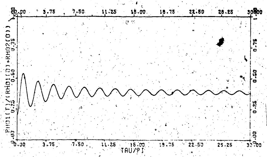
Fig. 4.2. Examples of the two temperature model with \rho_1(0) \ll \rho_2(0) .
