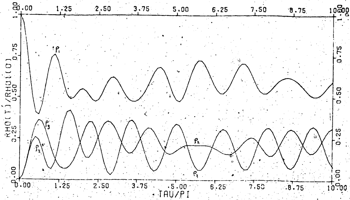
Fig. A.12. r_2 = 2. ; r_3 = 3. ; \frac{m_1}{m_2} = \frac{m_1}{m_3} = 0. ; U_1 = U_2 = \delta = 1.
