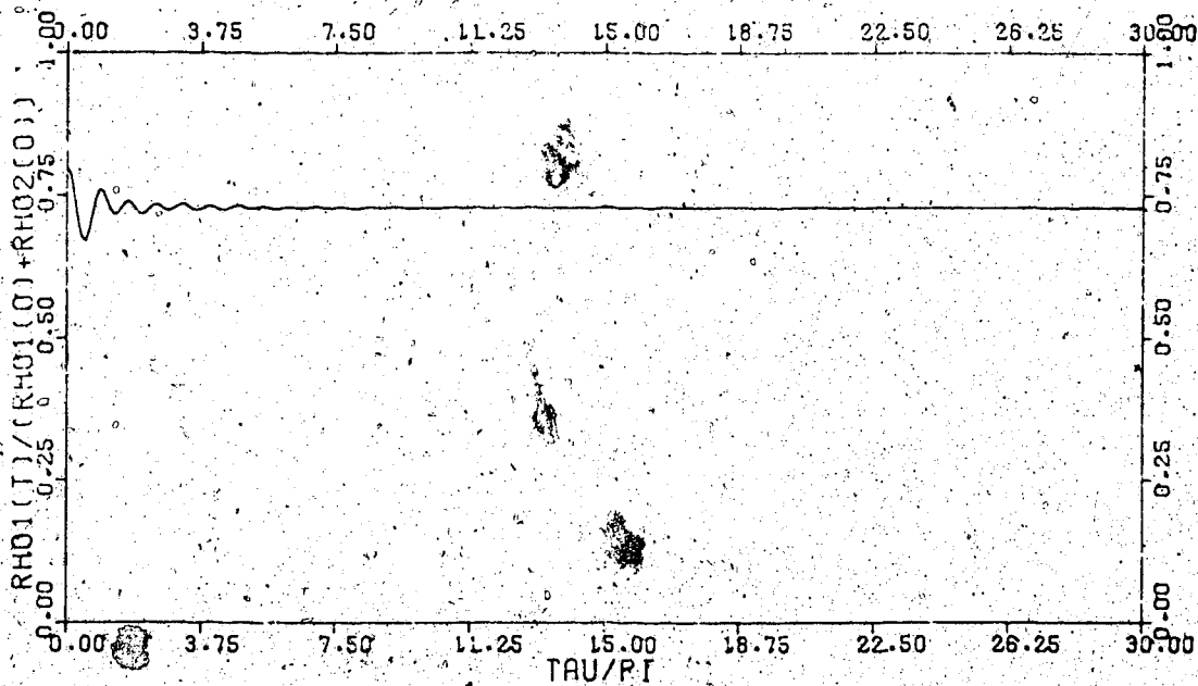
Fig. 4.1(b) \frac{\rho_2(0)}{\rho_1(0)} = 0.25 ; r = 5. ; \delta = 1. ; \gamma = 0.5.
