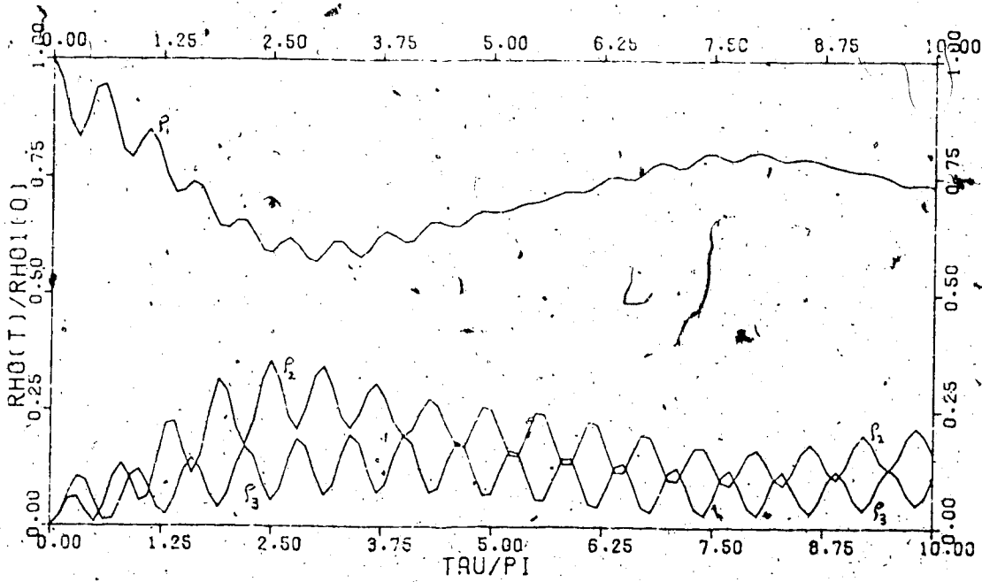
Fig. A.2. r_2 = 3. ; r_3 = 5. ; \frac{m_1}{m_2} = \frac{m_1}{m_3} = .5. ; U_1 = 1. ; U_2 = 3. ; \delta = 1.
