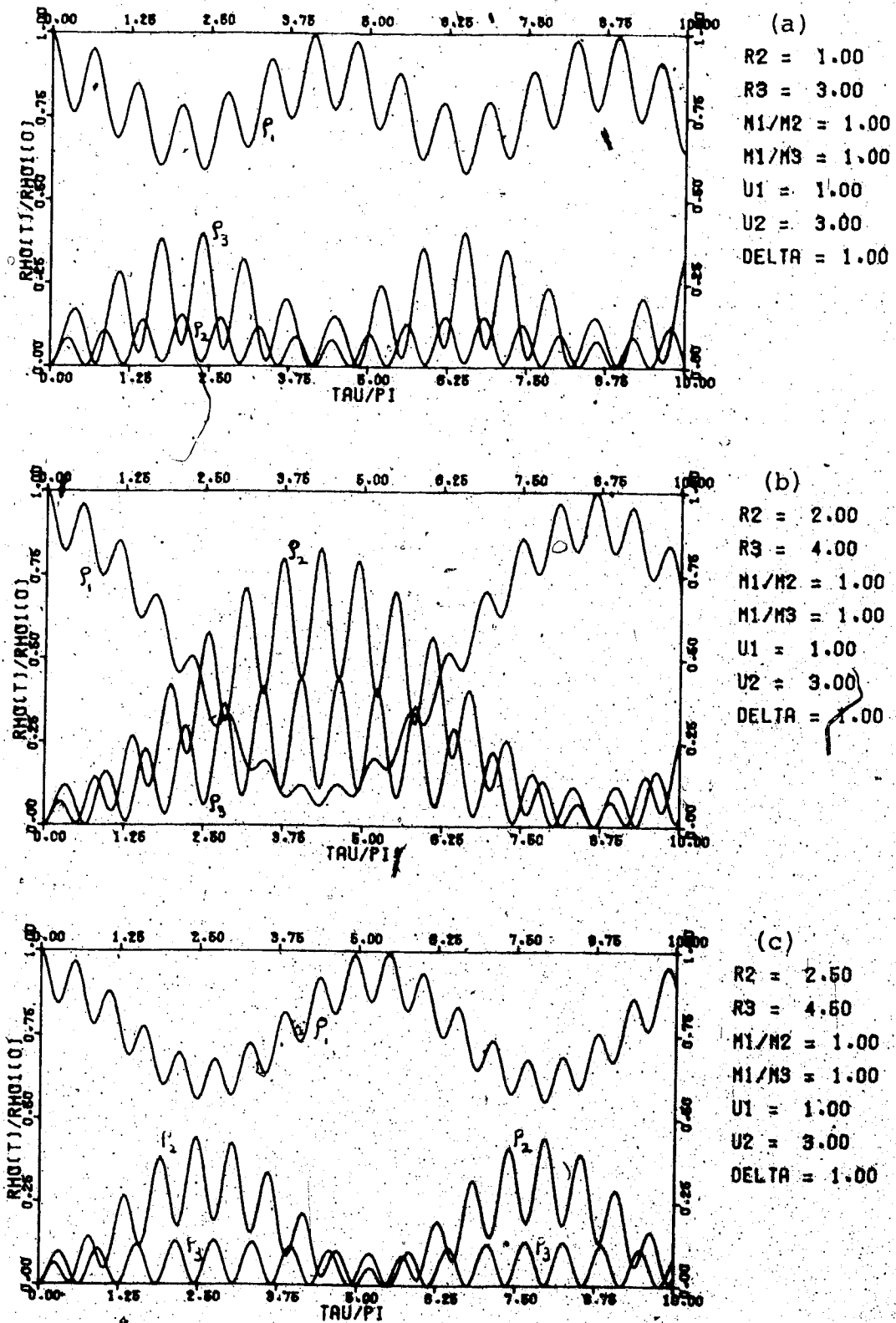
Fig. 2.4. Long period oscillations in the 3-channel system.
