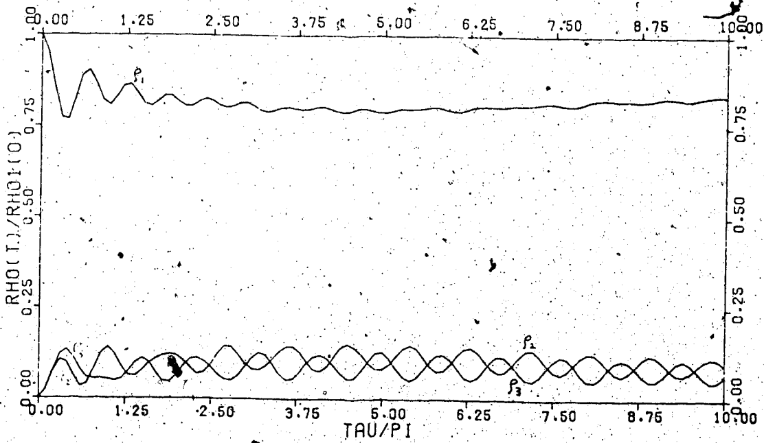
Fig. A.3. r_2 = 4. ; r_3 = 5. ; \frac{m_1}{m_2} = \frac{m_1}{m_3} = 0. ; U_1 = 1. ; U_2 = 2. ; \delta = 1.
