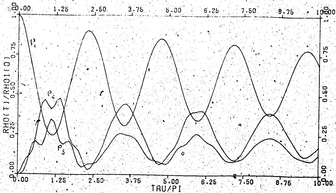
Fig. A.13. r_2 = 3. ; r_3 = 5. ; \frac{m_1}{m_2} = \frac{m_1}{m_3} = 0. ; U_1 = 0. ; U_2 = 3. ; \delta = 1.
