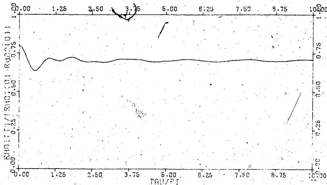
Fig. 4.1(a) \frac{\rho_2(0)}{\rho_1(0)} = 0.25 ; r = 5. ; \delta = 1. ; \gamma = 3.
