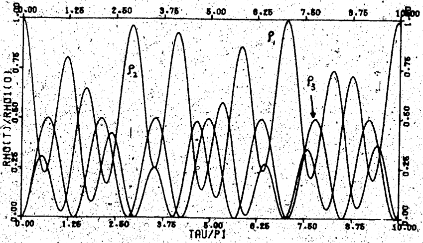
Fig. 2.3. Equal mass systems with r_3 = 0, 0.2 and 1 .
