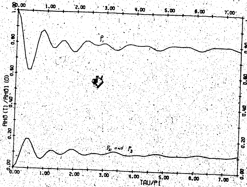
Fig. 2.8 (c) \frac{m_1}{m_2} = \frac{m_1}{m_3} = 0. ; r_2 = r_3 = \delta = U_1 = 1. ; U_2 = 4.
