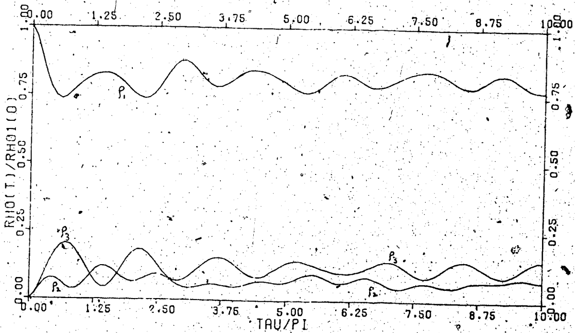
Fig. A.5. r_2 = 3. ; r_3 = 5. ; \frac{m_1}{m_2} = \frac{m_1}{m_3} = 0. ; U_1 = U_2 = 1. ;
