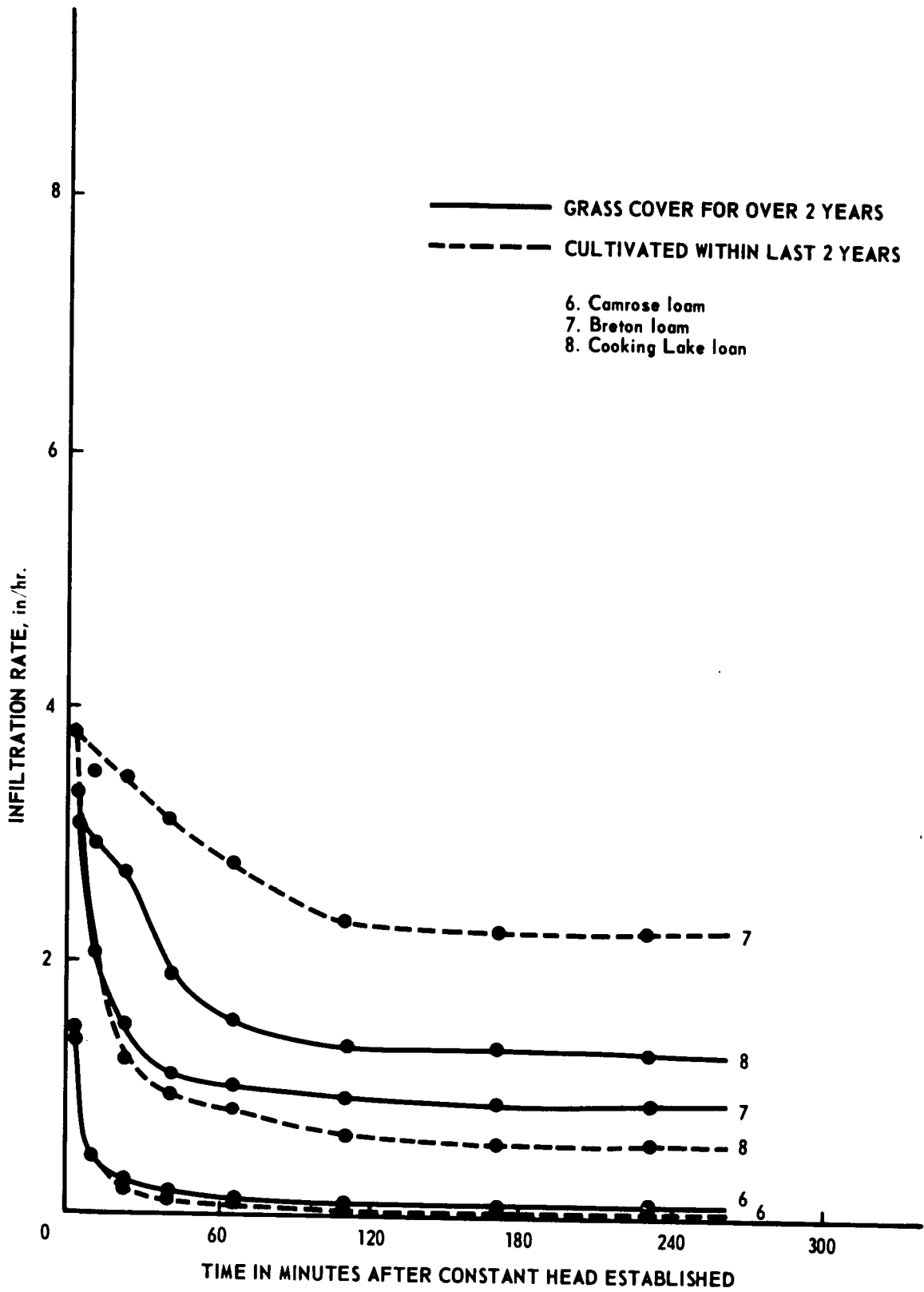
Fig. 6. Infiltration curves.
