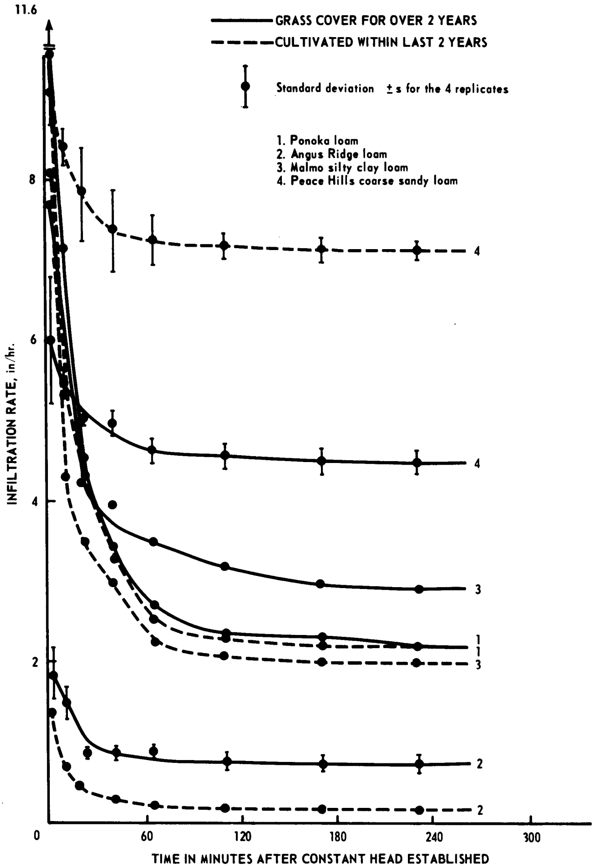
Fig. 5. Infiltration Curves.
