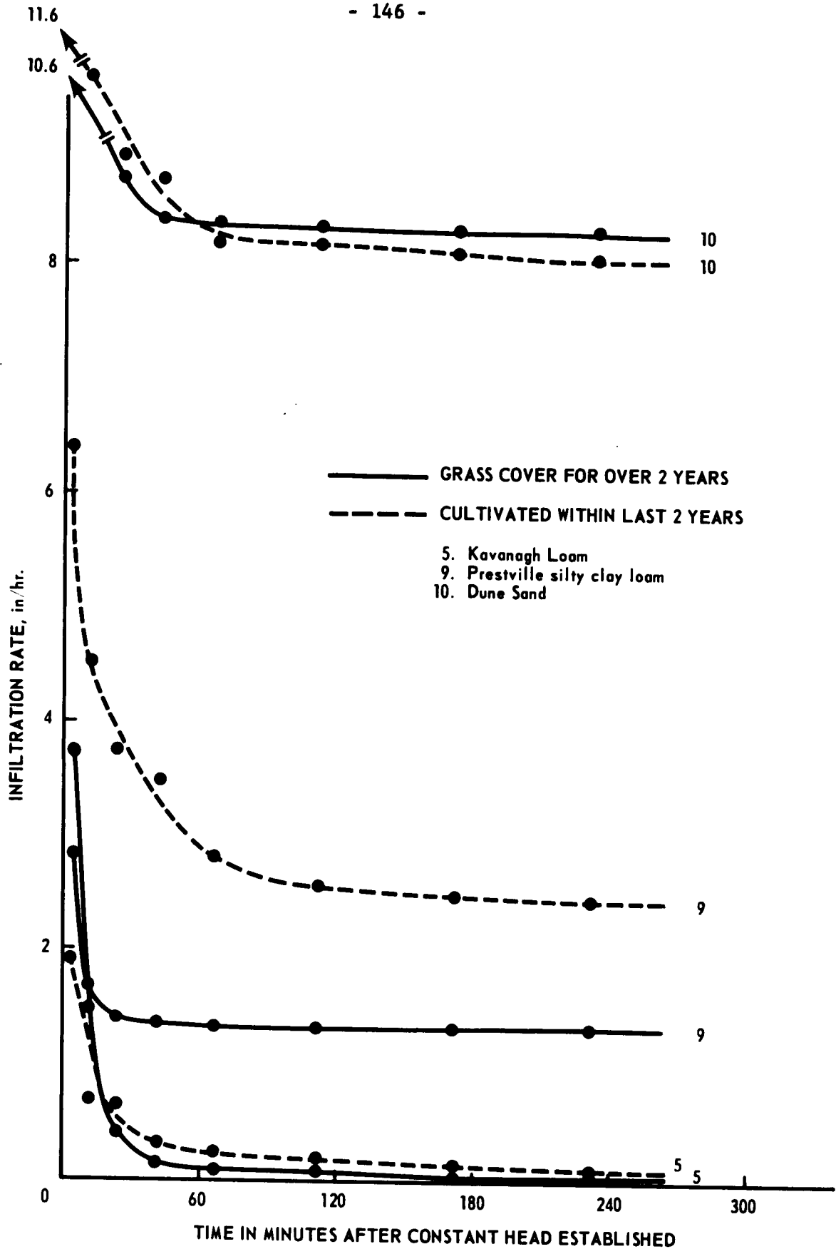
Fig. 7. Infiltration Curves.
