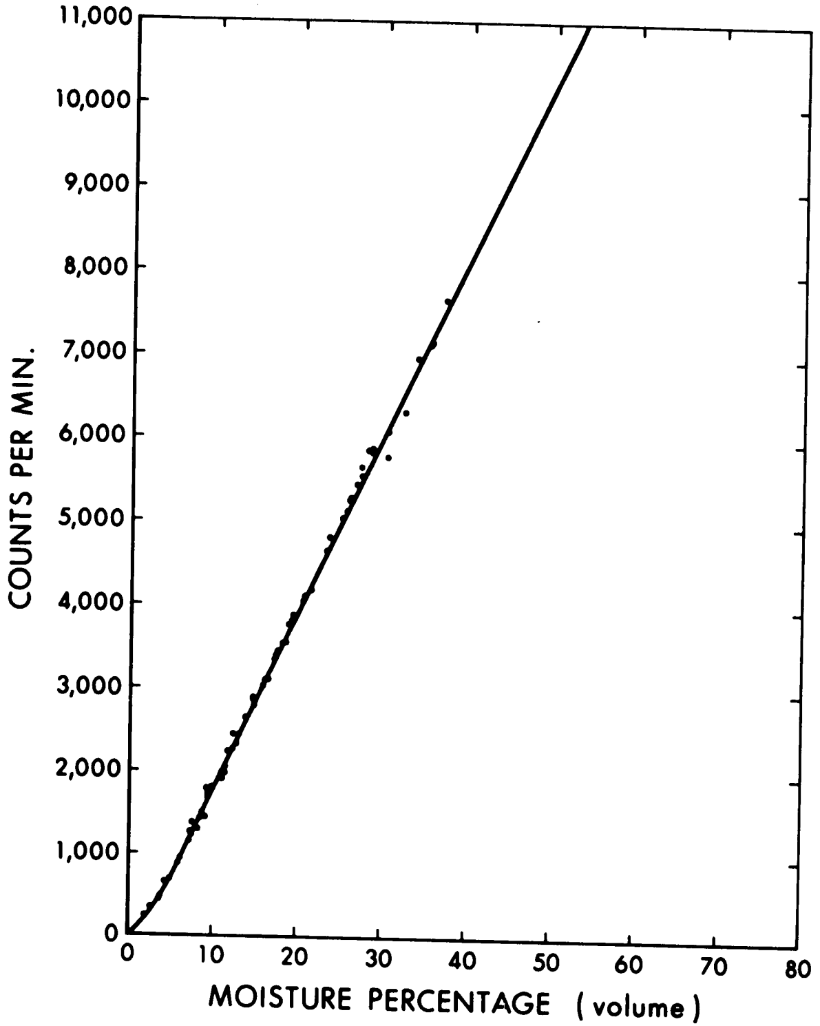
Calibration Curve for the Neutron Moisture Probe.
