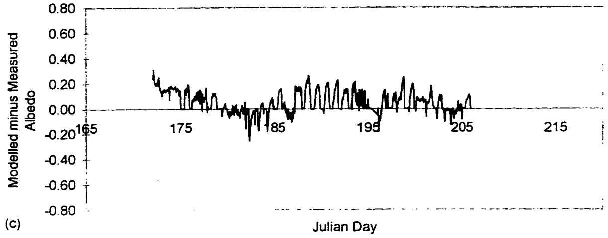
Figure 2.19: Difference between measured and modelled albedo (using EBM_Albedo) (a) L-AWS; (b) M-AWS; (c) U-AWS.
