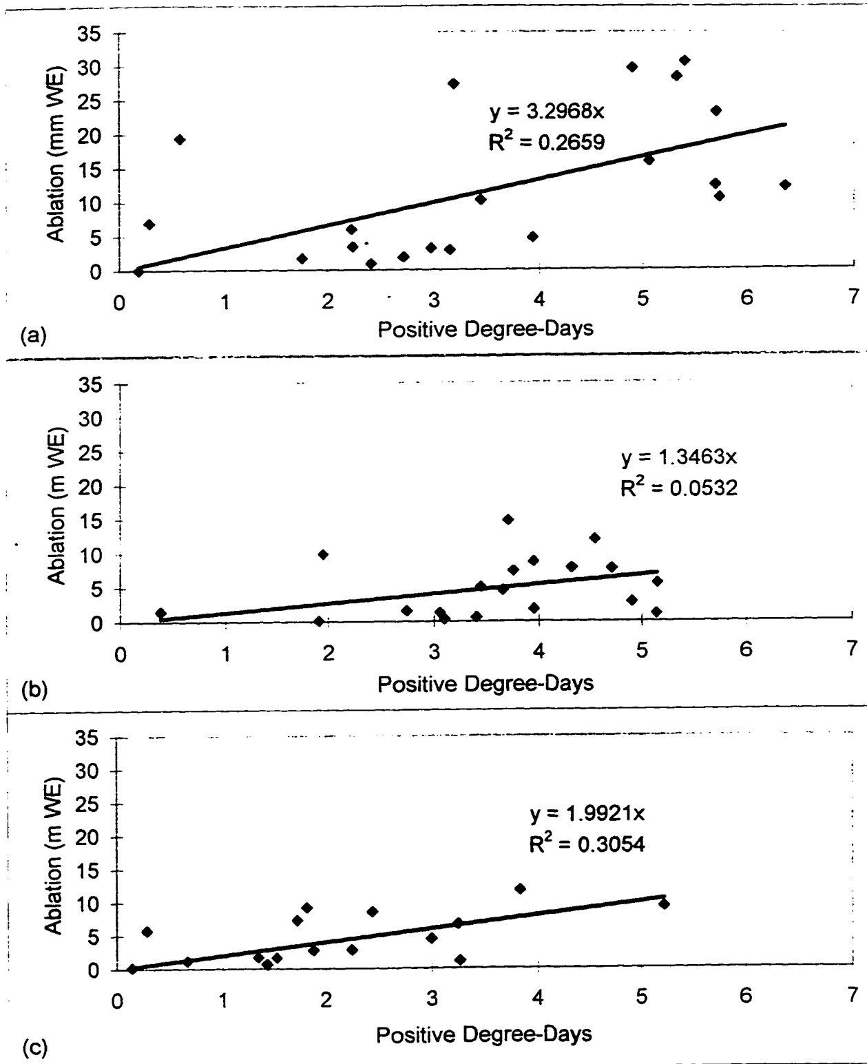
Figure 5.9: Total daily ablation for snow versus positive degree-days at each of the weather stations. (a) L-AWS; (b) M-AWS; (c) U-AWS.
