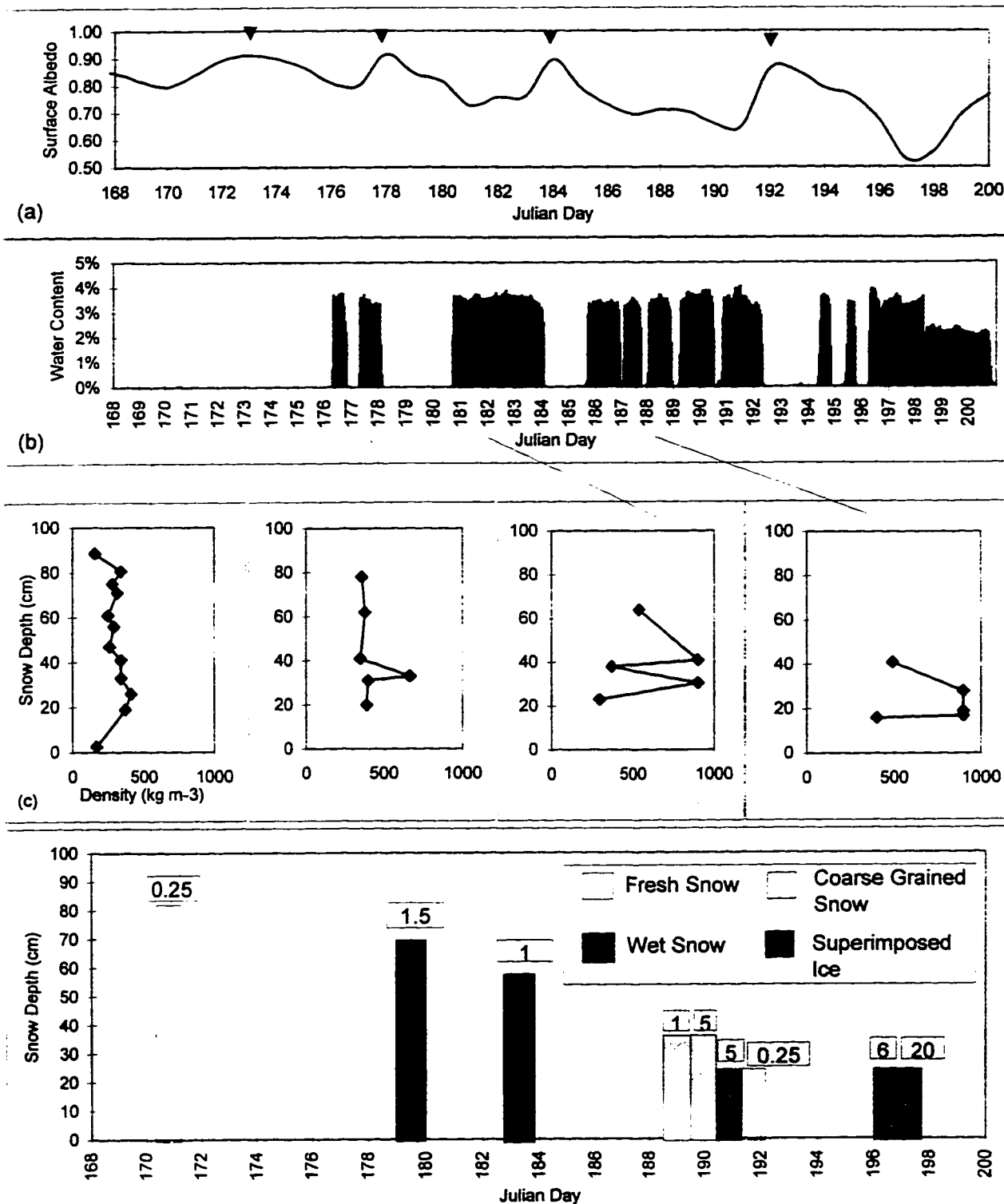
Figure 2.11: (a) Daily average albedo at the M-AWS, corrected for a sloping surface; (b) Fractional free water in the uppermost snow layer at the M-AWS, as determined from the SNTHERM model; (c) Measured snowpack density at the M-AWS; (d) Observed snow characteristics, snow depth and grain radius of snow in the uppermost layer at the M-AWS. (arrows in (a) mark the timing of new snowfall events).
