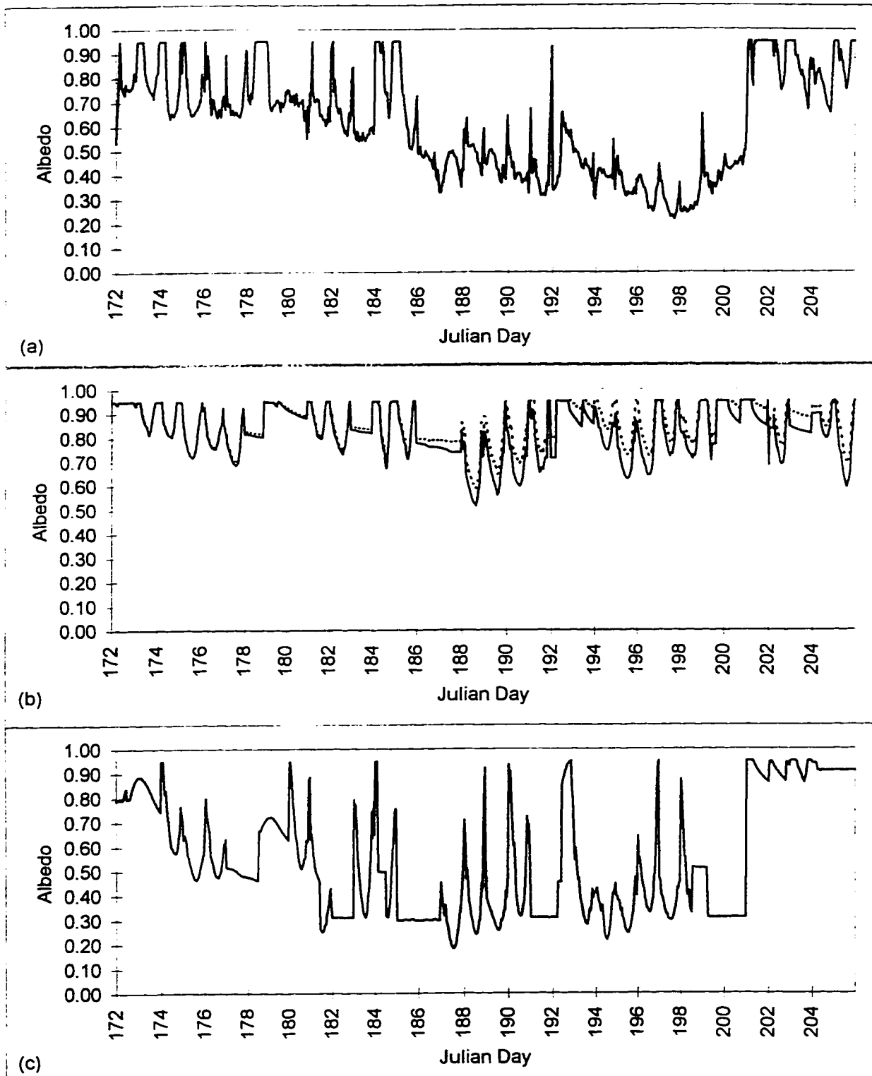
Figure 2.17: Albedo simulations at the L-AWS compared with measured albedo. (a) Measured albedo corrected for a sloping surface; (b) Run # 1 (dashed line) showing albedo simulations with no correction for snow contamination or free water content, Run # 2 (solid line) showing albedo simulations with correction for free water content; (c) Run # 3 showing albedo simulations with corrections for free water content and snow contamination.
