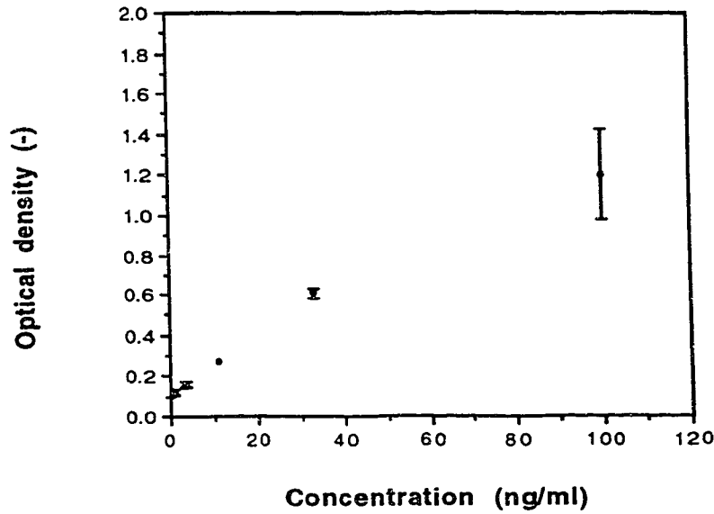
Figure 10a. Typical error in ELISA standard curve. Standard deviation resulting from triplicate sample measurement.
