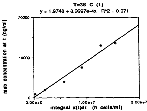
Figure A5-5. Regression results agitated cultures at 34, 37 and 38°C. Determination of \beta . Same number of samples as in A5-4.
