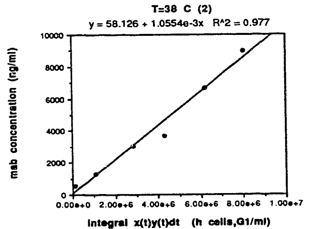
Figure A5-4. Regression results agitated cultures at 34, 37 and 38°C. Determination of \beta' .
