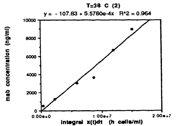
Figure A5-5. Regression results agitated cultures at 34, 37 and 38°C. Determination of \beta . Same number of samples as in A5-4.
