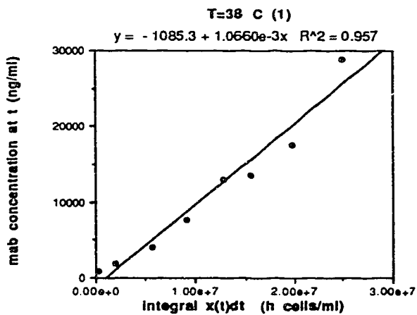
Figure A5-3. Regression results agitated cultures at 34, 37 and 38°C. Determination of \beta .
