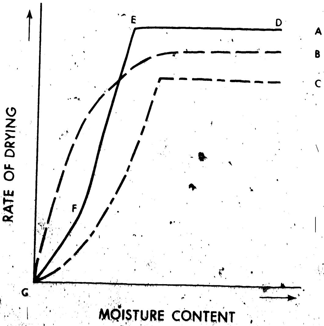
Figure T Typical Drying Rate Curves in Beds of Granular Solids [Adapted from Sherwood (14)]
