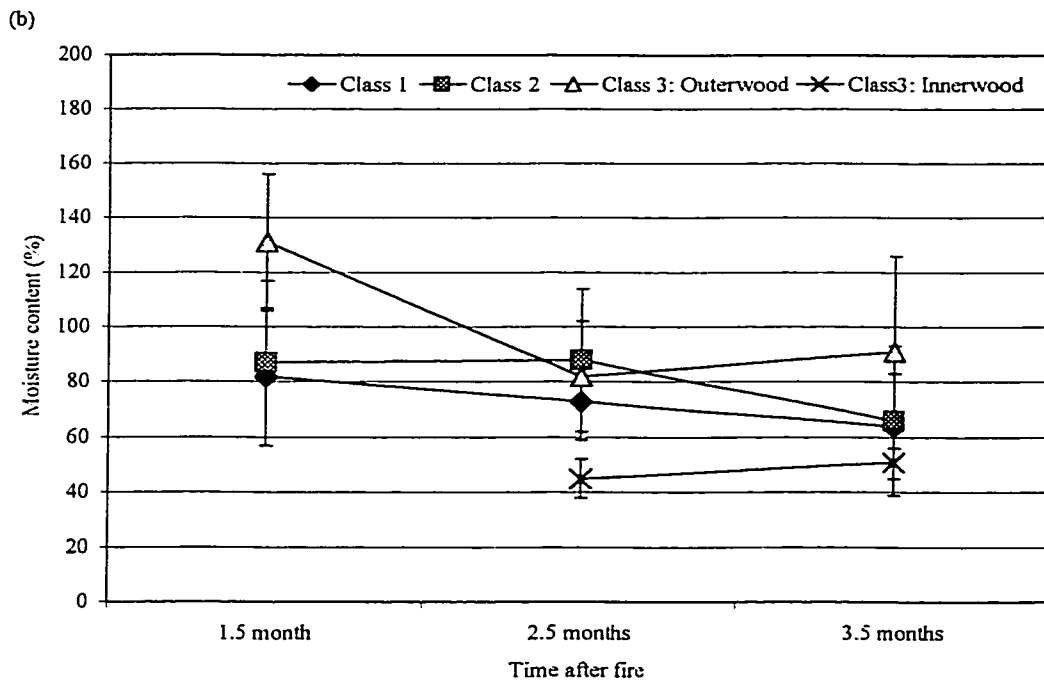
Figure 12. Moisture content relative to time after fire (1.5 months [45-47 days], 2.5 months [77-81 days], 3.5 months [107-110 days]) in (a) live and (b) fire-killed white spruce trees as stratified by the three diameter at breast height (DBH) size classes (Class 1 [DBH: 15-22cm]; Class 2 [DBH: 23-33cm]; Class 3 [DBH: >33cm]) sampled in Study Area 2. The bars indicate the standard deviations.
