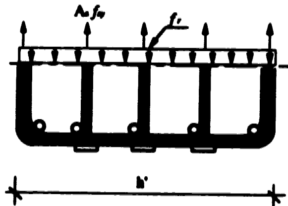
Figure 2.6.c Idealized "confining pressure" f_c
