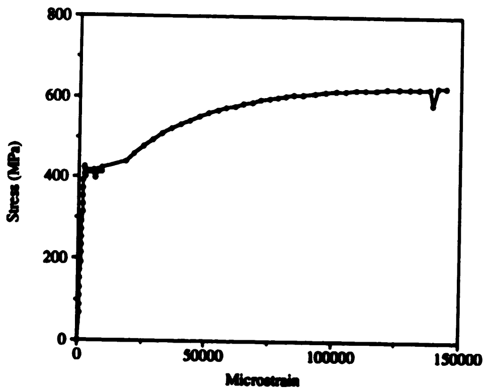
Figure 3.10 Stress Strain Curve for No.8 Bar
