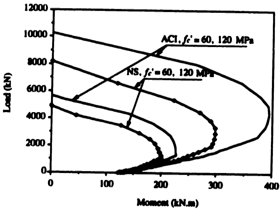
Figure 7.4 Interaction Diagrams of Different Design Codes
