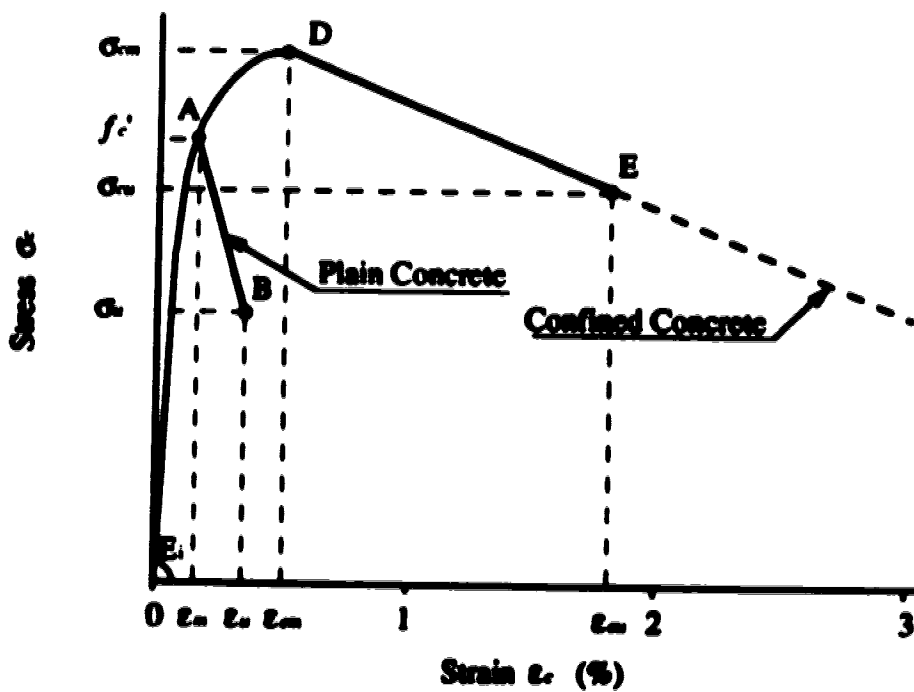
Figure 2.3 Idealized Stress Strain Curves by Maguruma et al. (1983), (1989)
