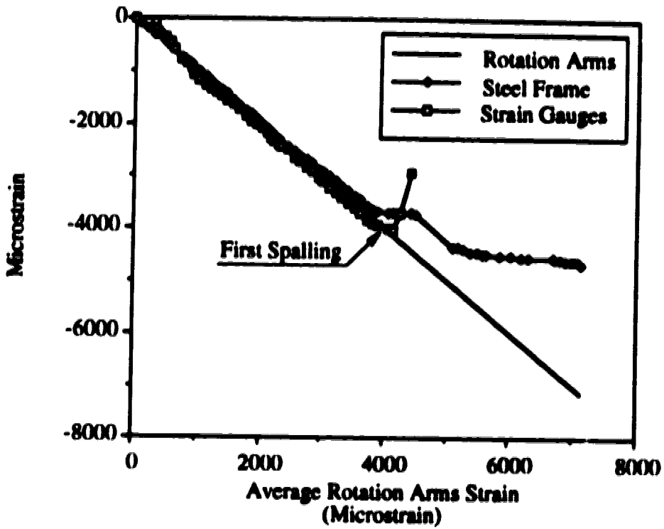
Figure 4.30 Average Longitudinal Strain at the Compression Face of Specimen VII
