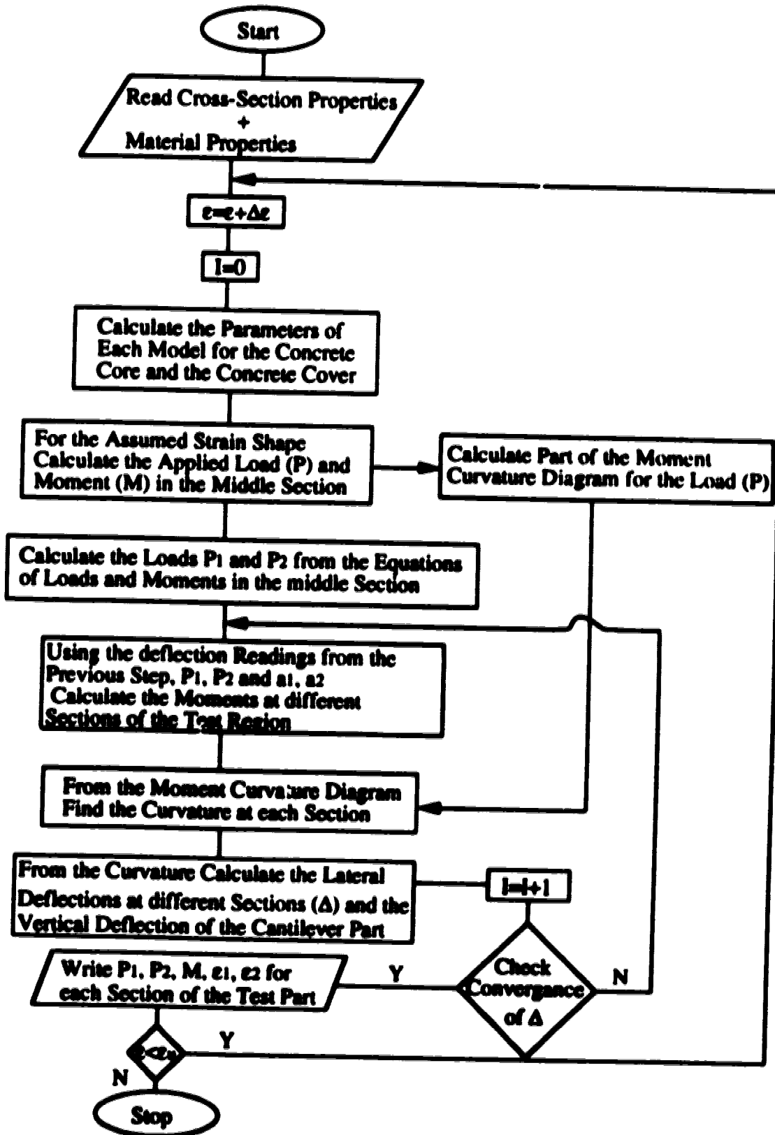
Figure 8.2 Flow Chart of the Computer Analysis
