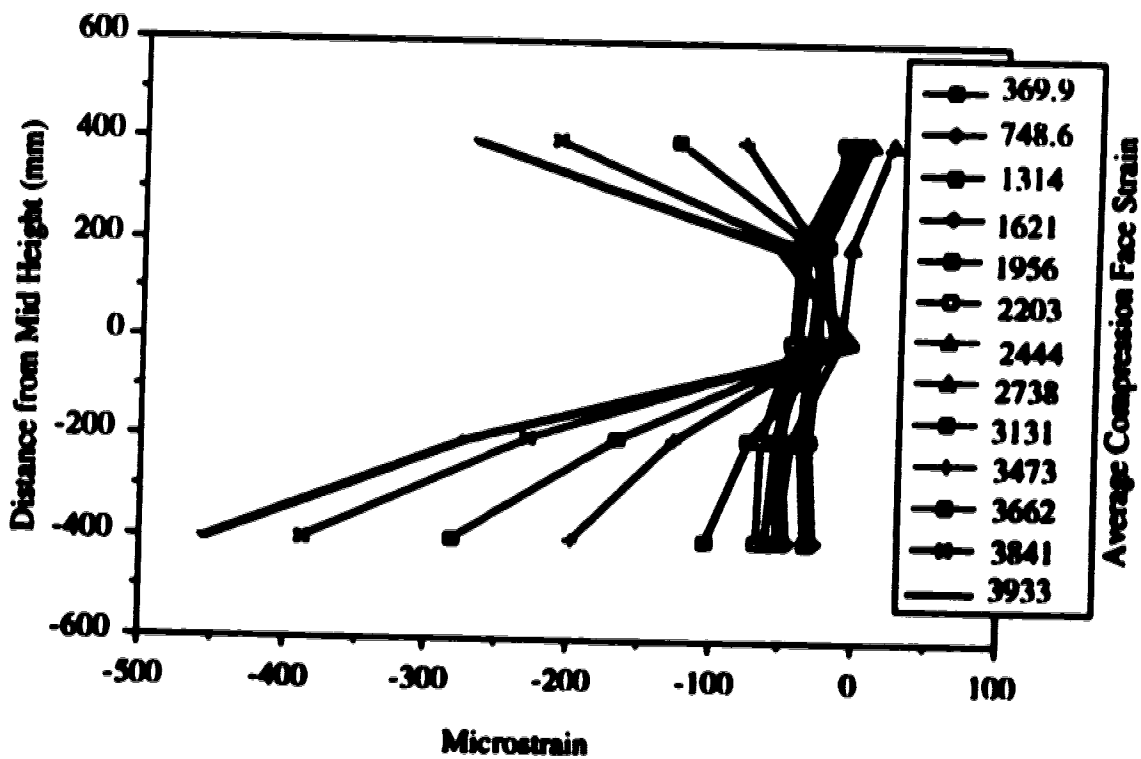
Figure 4.19 Longitudinal Strain Distribution at the Back Face of Specimen V4
