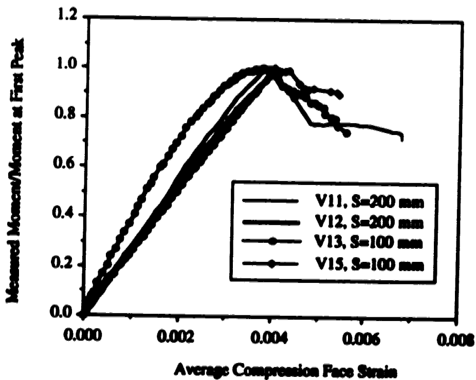
Figure 4.45 Effect of Tie Spacing on the Normalized Moment
