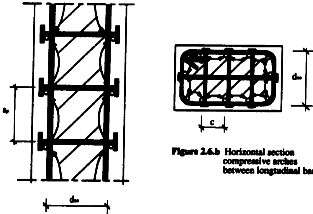
Figure 2.6.a Vertical section Compressive arches between the confinement reinforcement layers
