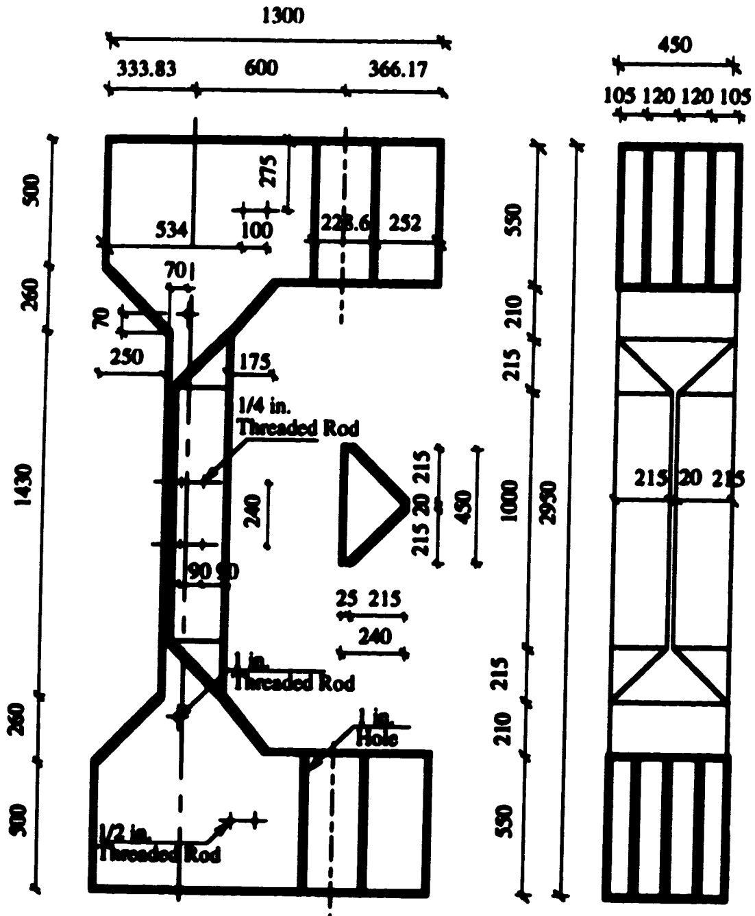
Figure 3.3 Concrete Dimensions for The Triangular Specimens
