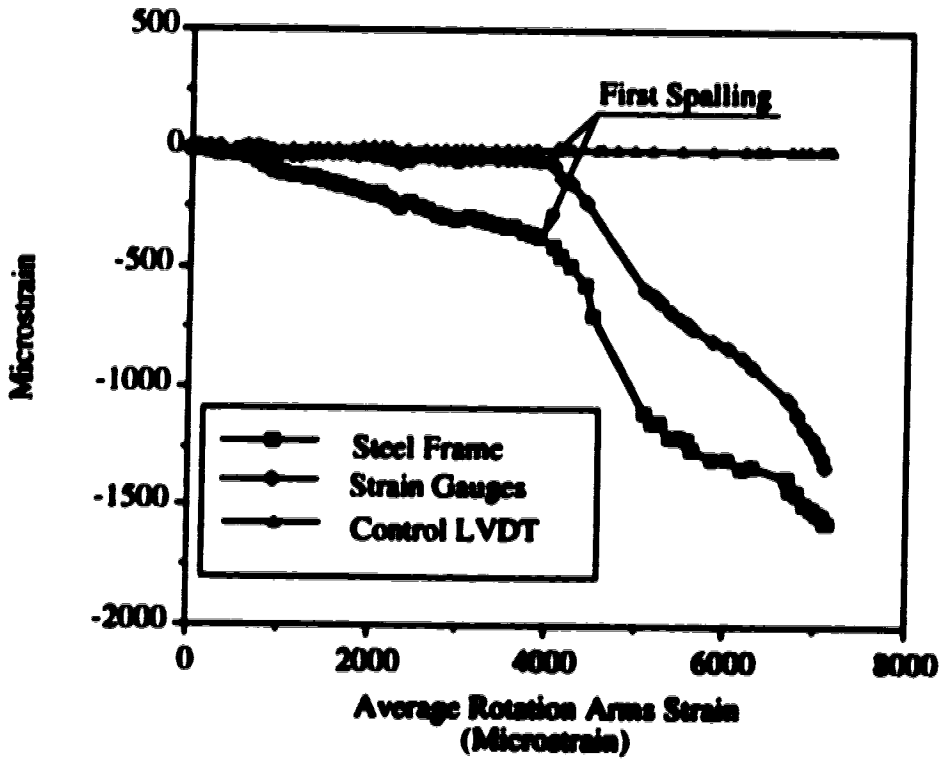
Figure 4.31 Average Longitudinal Strain at the Back Face of Specimen VII
