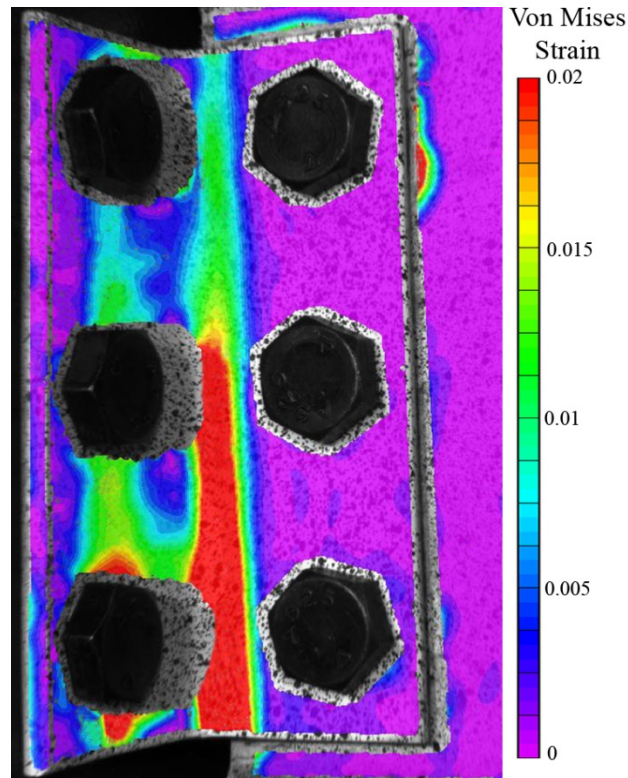
Figure 6.1. Von Mises strain showing plastic hinge formation along angle heel and column bolt line (at left).
