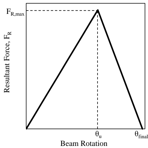
Figure 5.20. Generalized bilinear force versus rotation relationship.
