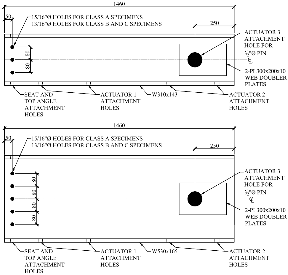
Figure 3.10. Test beam details.
