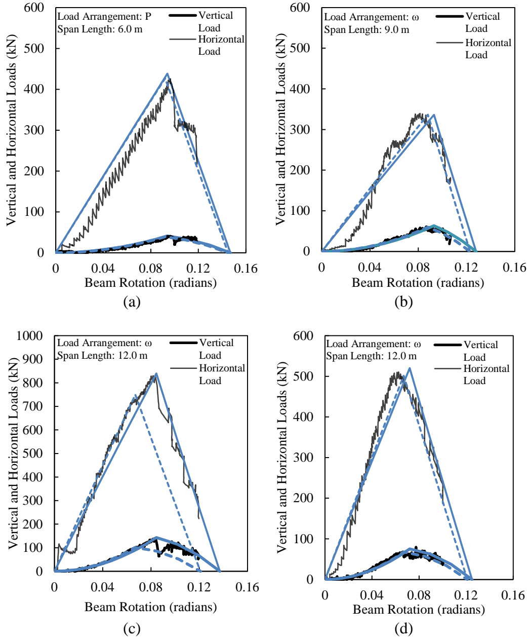
Figure 5.21. Simplified connection modelling results for: (a) WA3A-1, (b) ST3B-2, (c) ST5A-2, and (d) ST5B-2.
