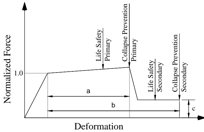
Figure 2.1. Generalized component force–deformation curve for nonlinear modelling and acceptance criteria (adapted from ASCE/SEI 41-06 (ASCE, 2007)).
