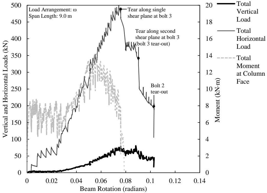
Figure D.12. Load versus rotation for WA3A-3.
