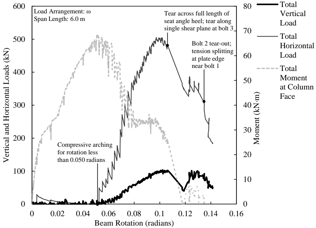
Figure D.36. Load versus rotation for ST3C-1.
