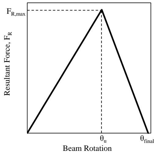
Figure 6.20. Generalized bilinear force versus rotation relationship.
