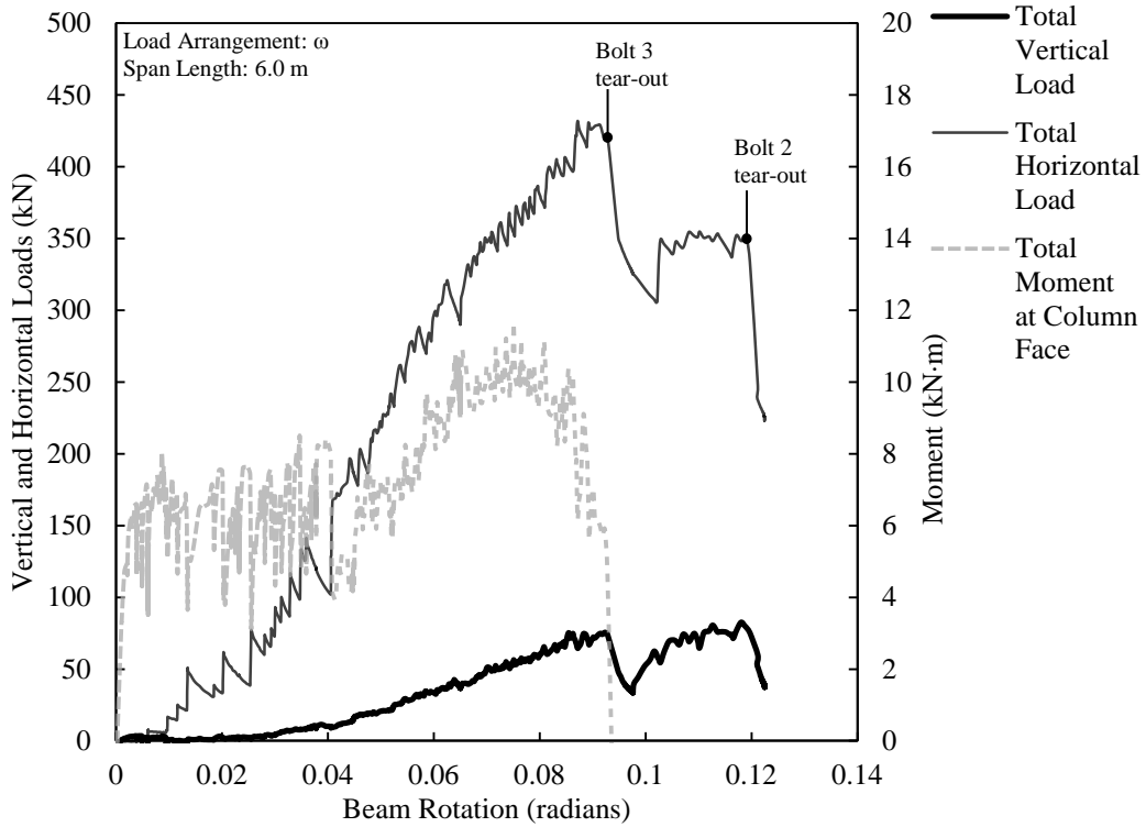
Figure D.11. Load versus rotation for WA3A-2.
