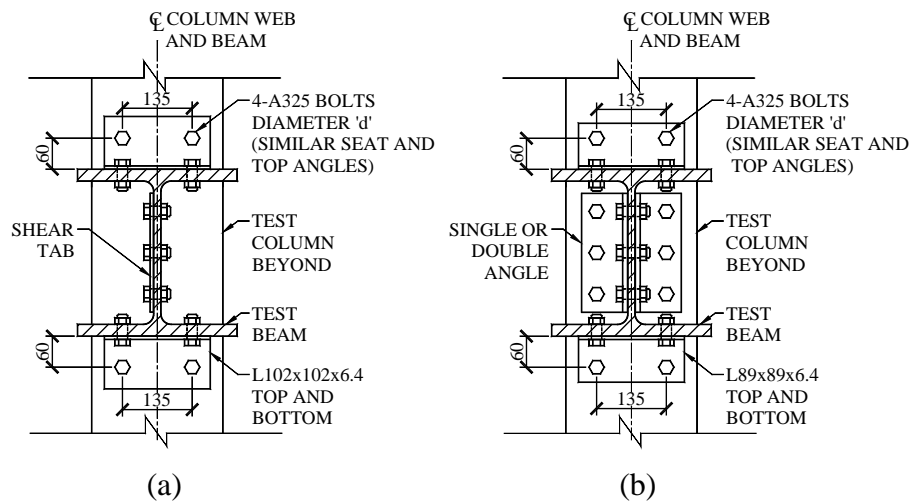
Figure 3.15. Sections from Figure 3.14 for seat and top angle combined with: (a) shear tab (Section B-B), and (b) angle connections (Section C-C).
