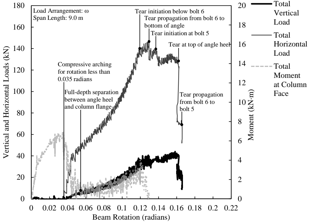
Figure D.21. Load versus rotation for SA3B-3.
