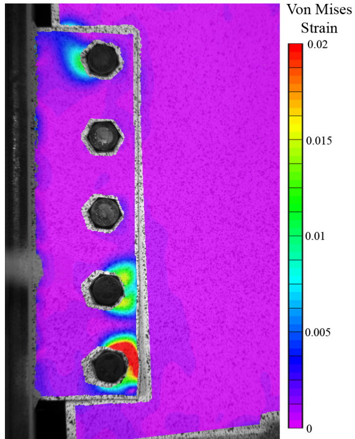
Figure 5.1. Von Mises strain showing localized bearing effects at bolt locations.
