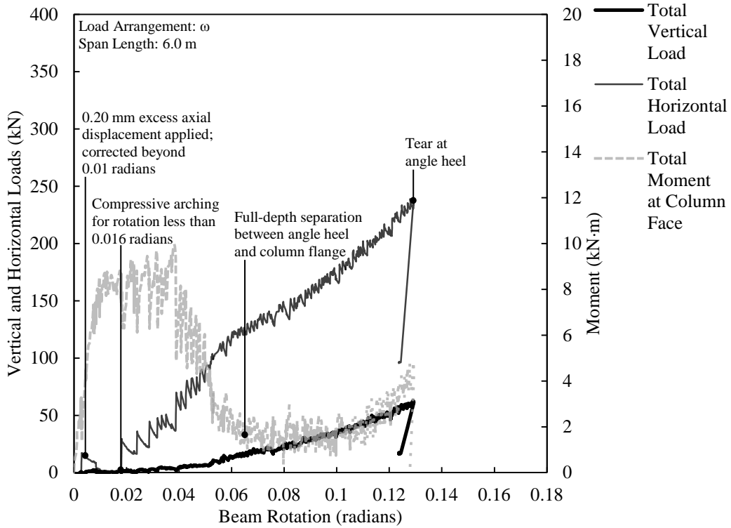
Figure D.16. Load versus rotation for SA3A-2.
