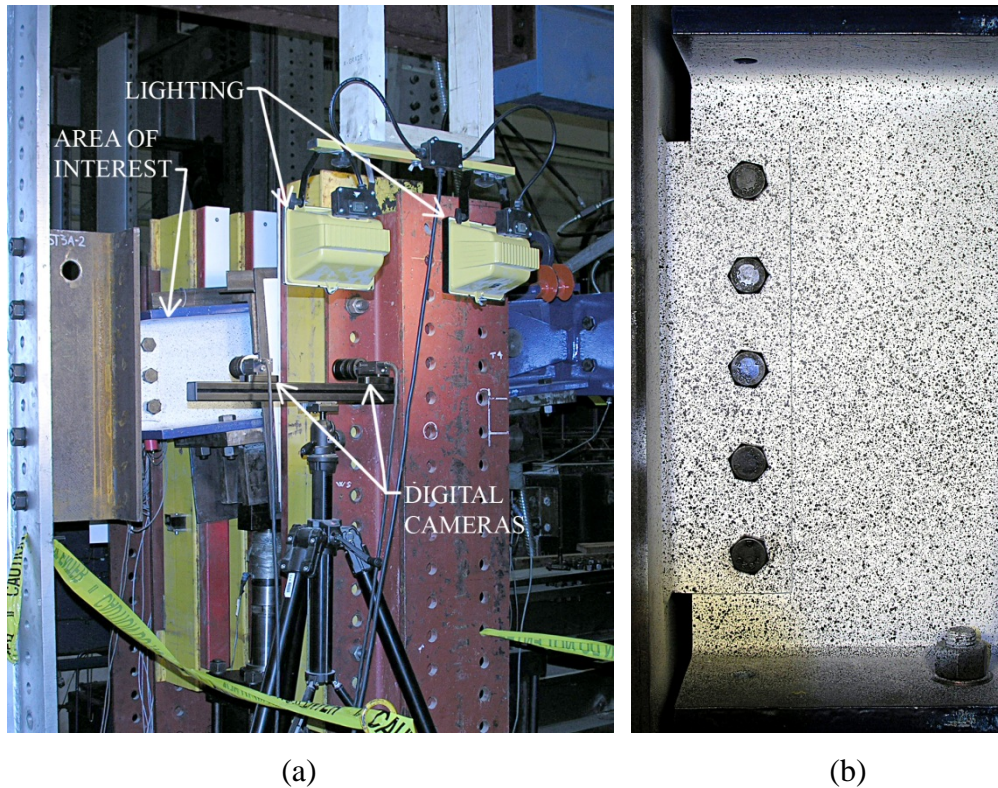
Figure 3.4. Optical strain imaging: (a) camera set-up, and (b) typical speckle pattern in area of interest.
