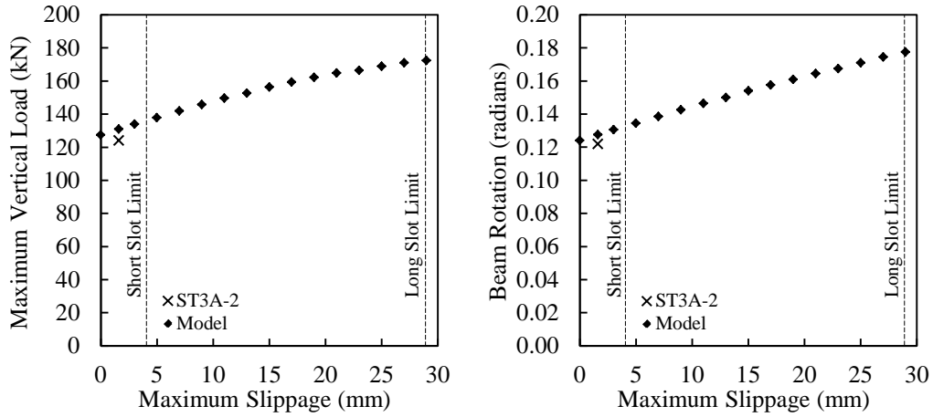
Figure 5.17. Parametric study: maximum bolt slippage.
