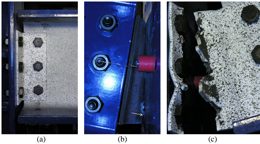
Figure 4.13. Specimen SA3B-2 at: (a) 0 radians (undeformed), (b) 0.142 radians (tear initiation), and (c) 0.202 radians (tear propagation).
