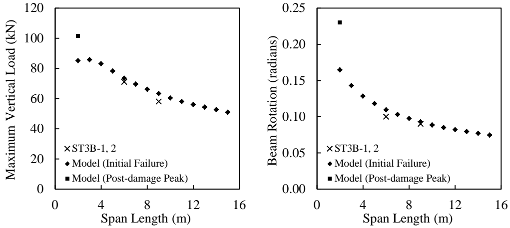
Figure 5.14. Parametric study: span length (three-bolt connections).
