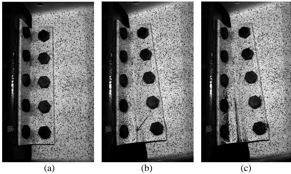
Figure 4.11. Specimen SA5A-1 at: (a) 0 radians (undeformed), (b) 0.133 radians (tear initiation at angle heel), and (c) 0.147 radians (tear propagation upwards).
