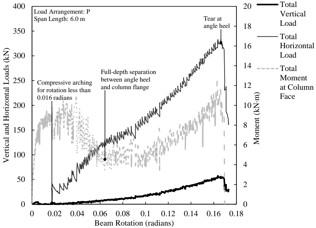
Figure D.15. Load versus rotation for SA3A-1.
