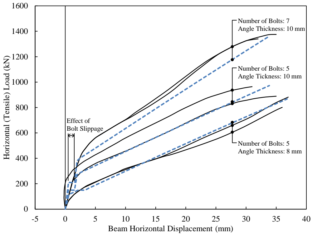
Figure 6.11. Comparison of mechanical model and test results for pure tension tests by Owens and Moore (1992).
