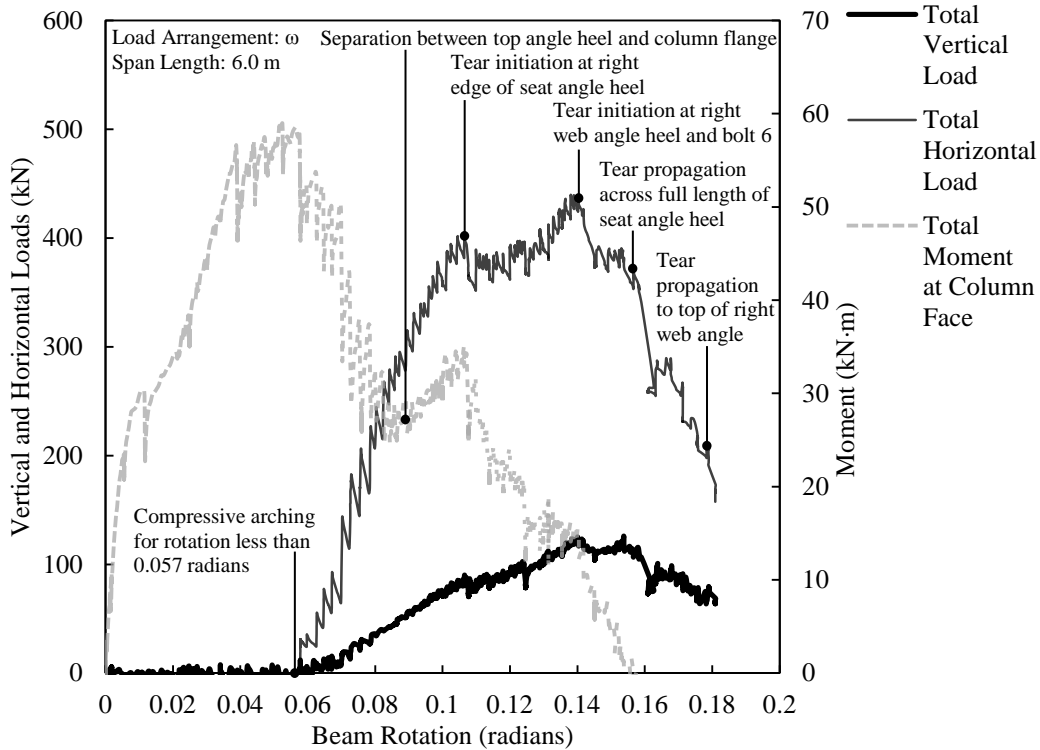
Figure D.44. Load versus rotation for DA3C-1.
