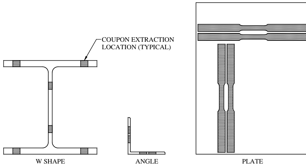
Figure 3.17. Tension coupon extraction locations.
