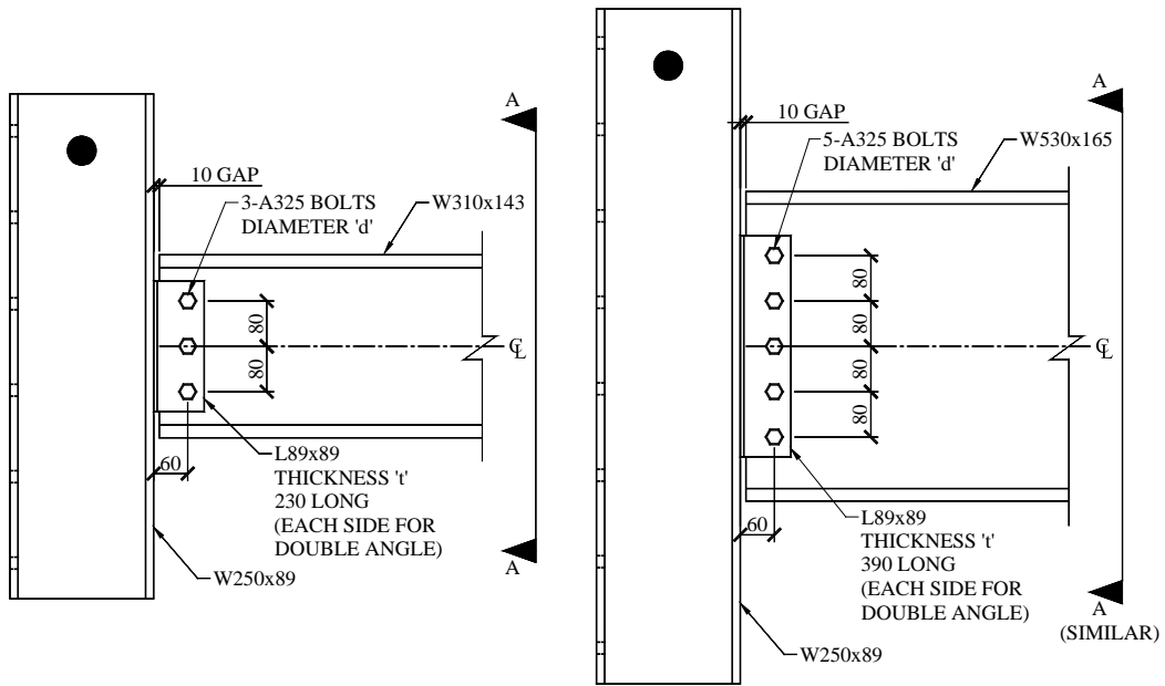
Figure 3.12. Single and double angle connection details.
