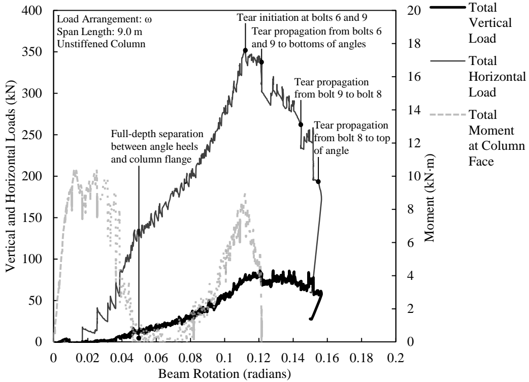
Figure D.32. Load versus rotation for DA3B-3.
