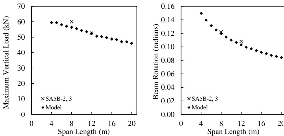
Figure 6.14. Parametric study: span length (five-bolt Series B connections).
