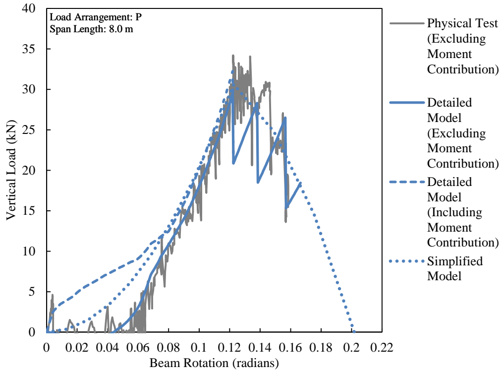
Figure 6.22. Prediction of vertical load by simplified connection model for specimen SA5B-1.
