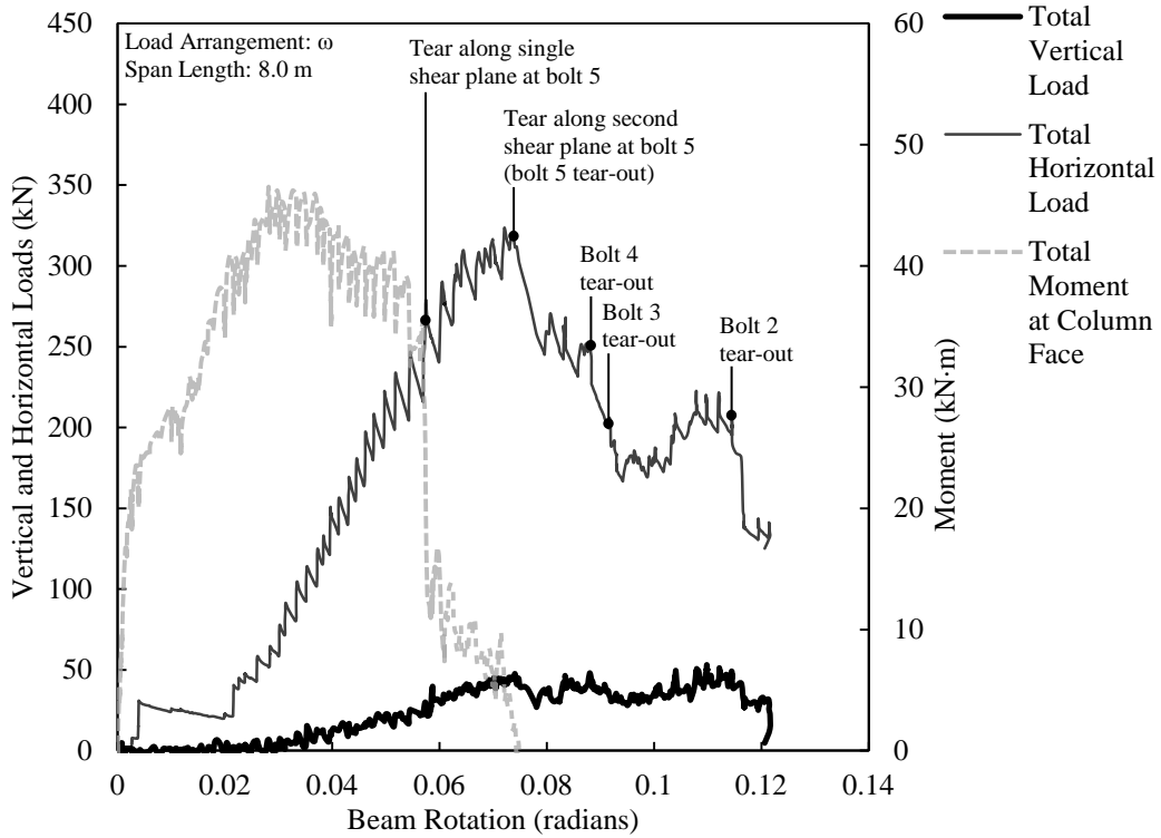
Figure D.13. Load versus rotation for WA5B-1.
