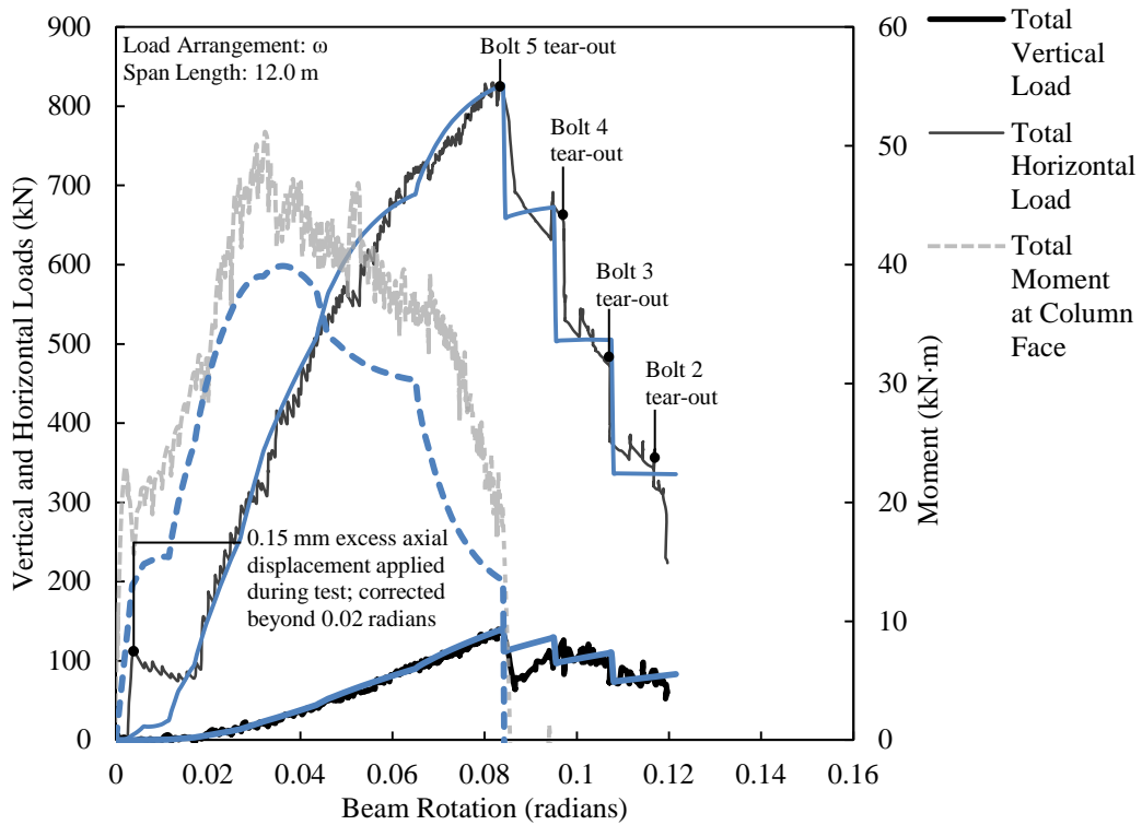
Figure 5.9. Comparison of mechanical model and test results for ST5A-2.
