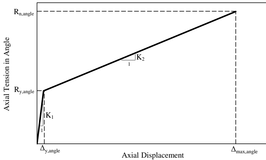
Figure 6.2. Force versus displacement for angle segments bending under tension.
