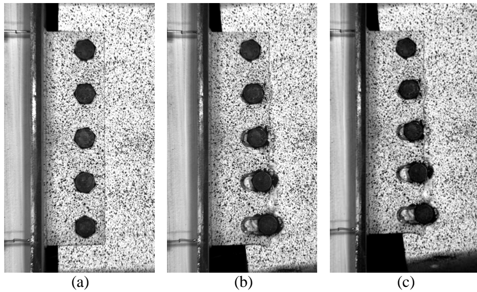
Figure 4.4. Specimen ST5A-1 at: (a) 0 radians (undeformed), (b) 0.094 radians (extreme bolt tear-out), and (c) 0.110 radians (bolt 4 tear-out, peak post-damage response).
