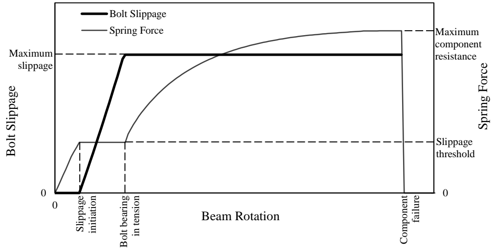
Figure 5.6. Representative behaviour of the bolt slippage function for a bottom bolt.
