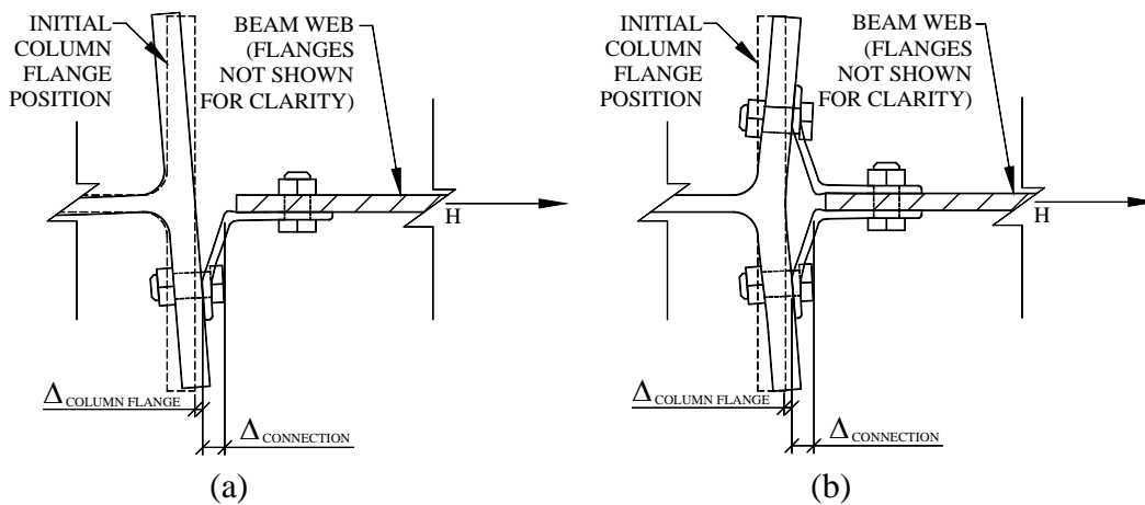
Figure 4.8. Deformation of unstiffened column for: (a) bolted–bolted single angle connection, and (b) bolted–bolted double angle connection.
