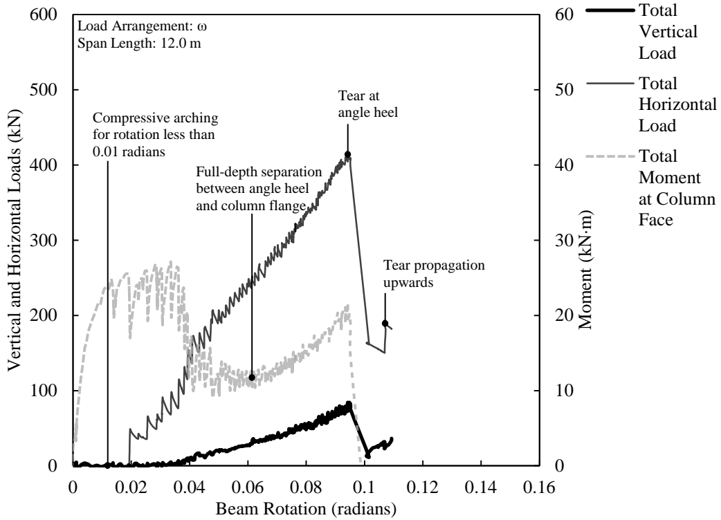
Figure D.25. Load versus rotation for SA5A-2.
