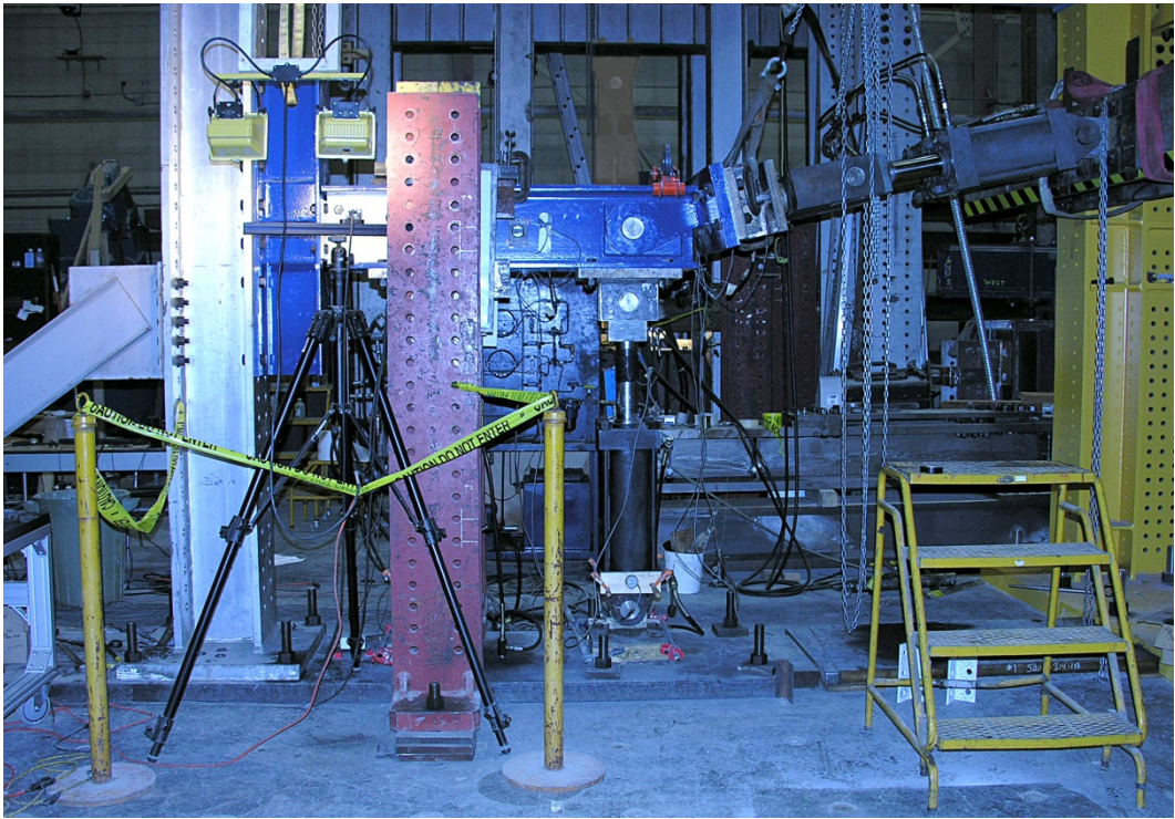
Figure 3.2. Typical test set-up.
