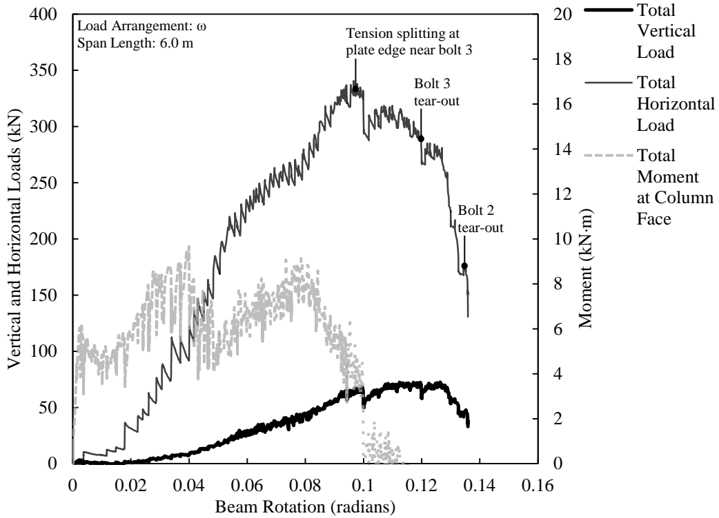
Figure D.4. Load versus rotation for ST3B-1.
