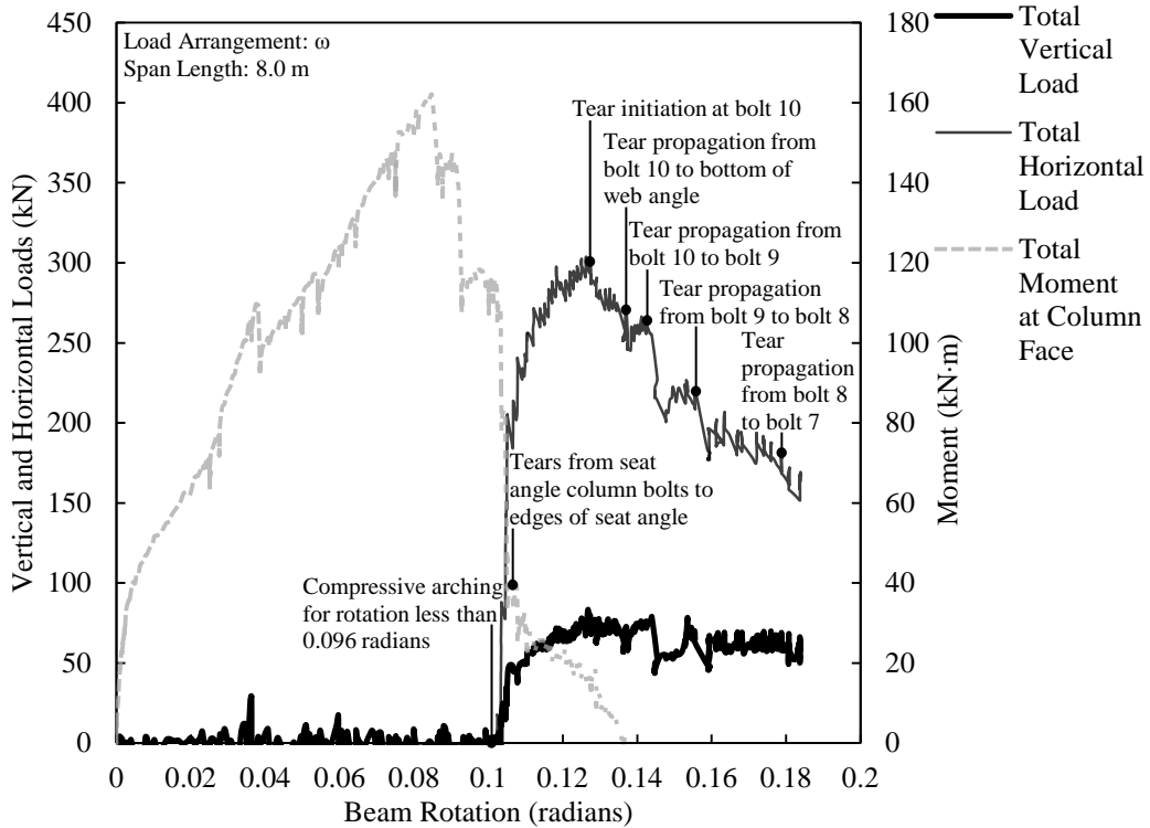
Figure D.42. Load versus rotation for SA5C-1.
