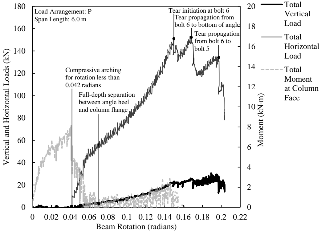
Figure D.22. Load versus rotation for SA3B-4.
