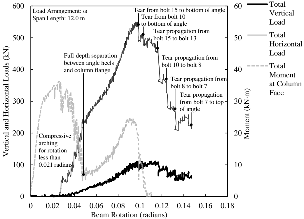
Figure D.34. Load versus rotation for DA5B-2.
