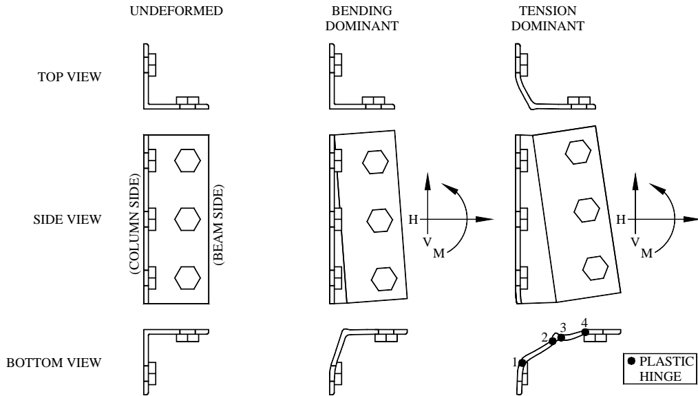
Figure 4.7. Deformation of bolted–bolted angle connections under combined loading.
