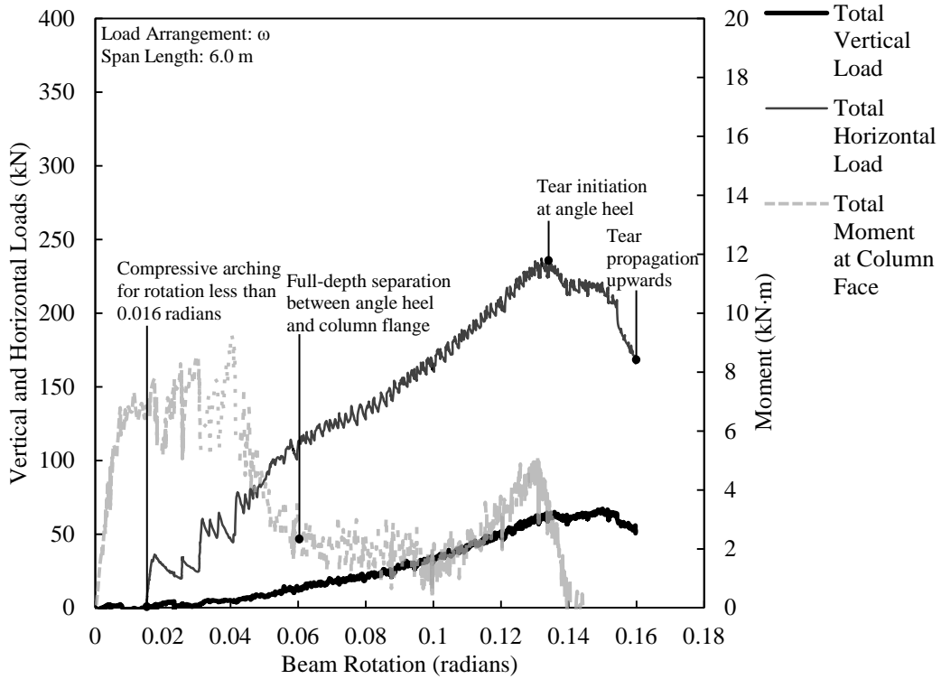
Figure D.18. Load versus rotation for SA3A-4.
