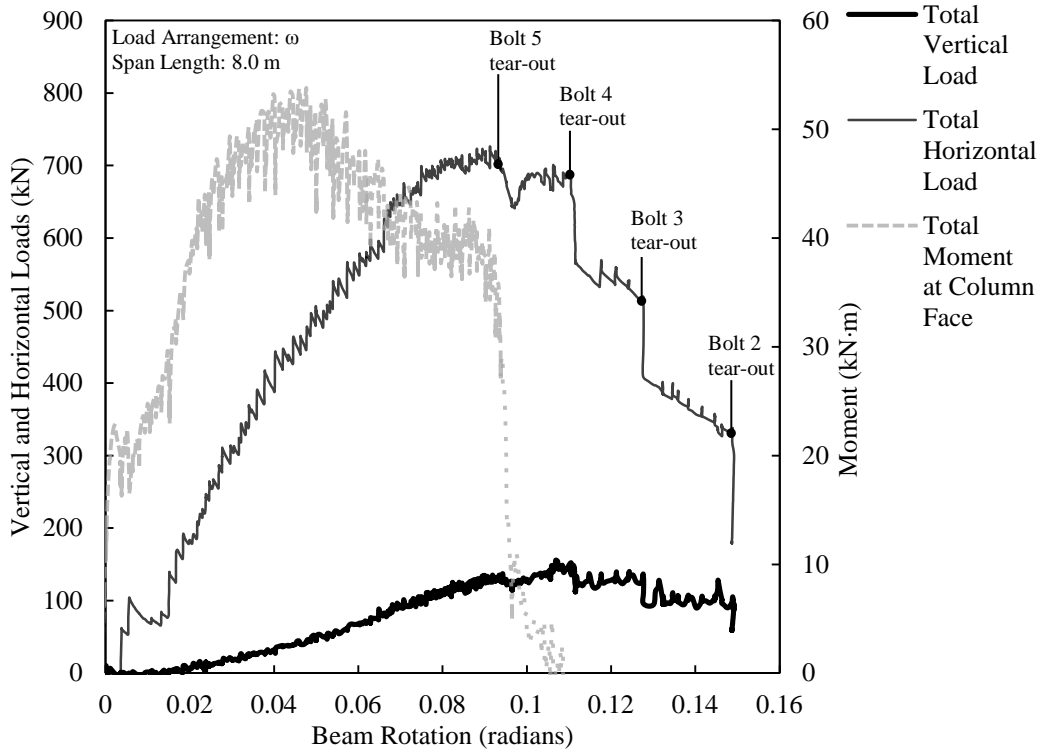
Figure D.6. Load versus rotation for ST5A-1.
