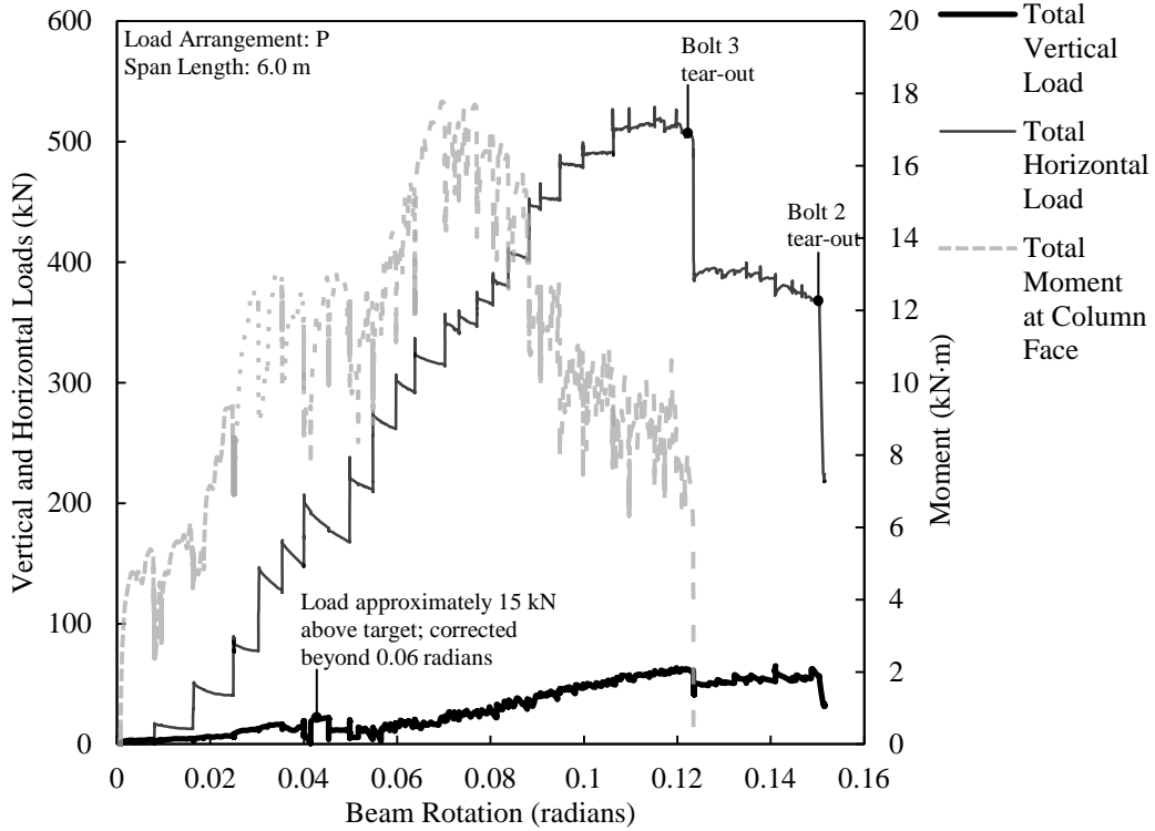
Figure D.1. Load versus rotation for ST3A-1.
