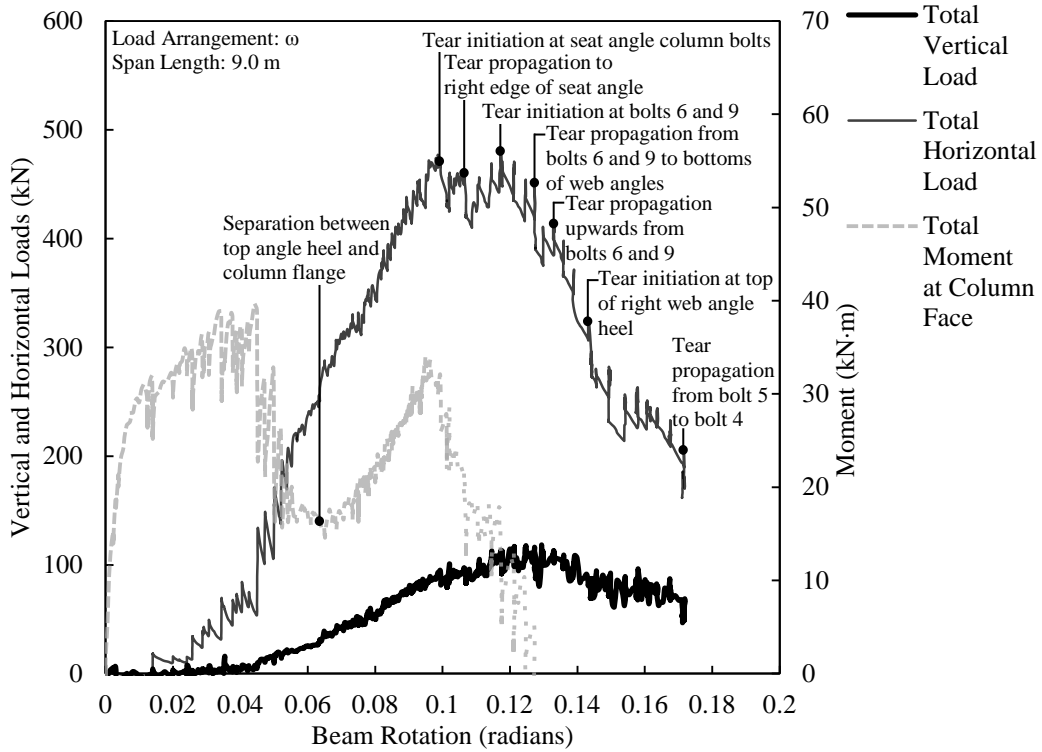
Figure D.45. Load versus rotation for DA3C-2.
