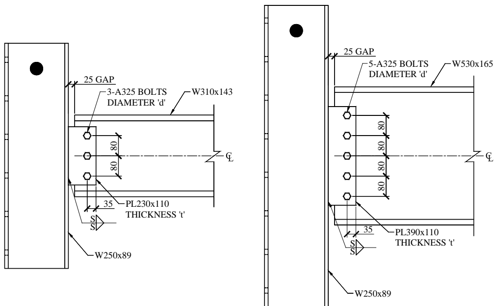
Figure 3.11. Shear tab details.
