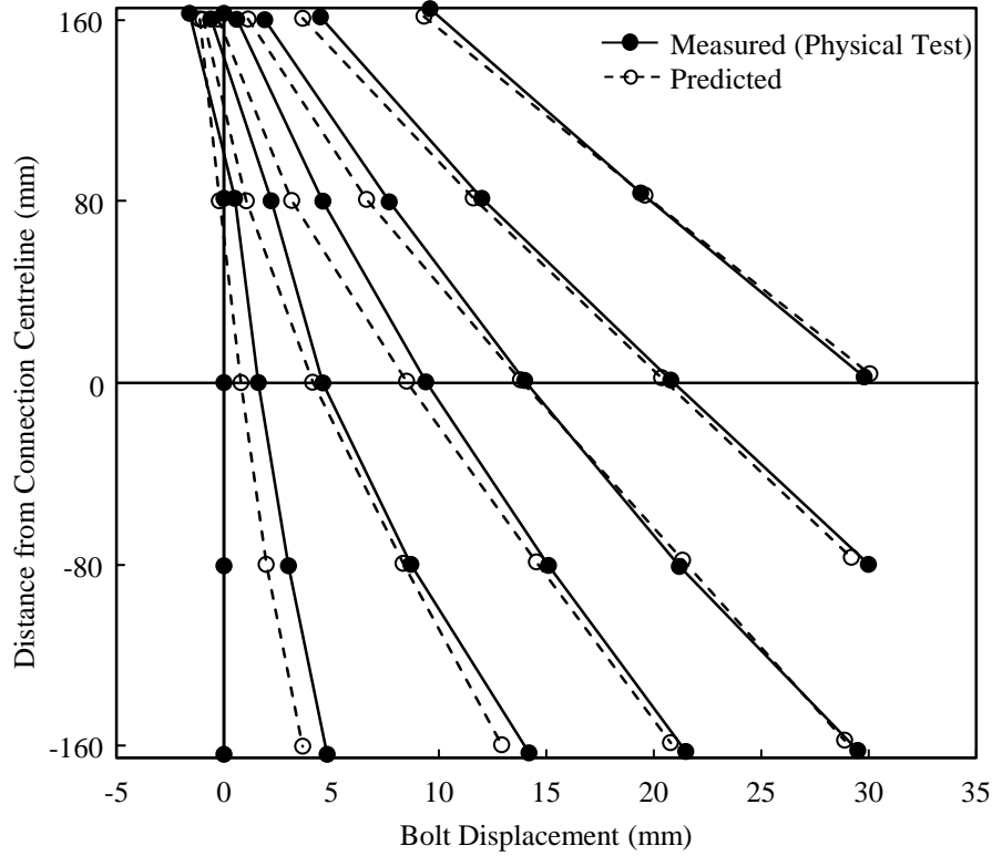
Figure 5.8. Prediction of bolt displacements.
