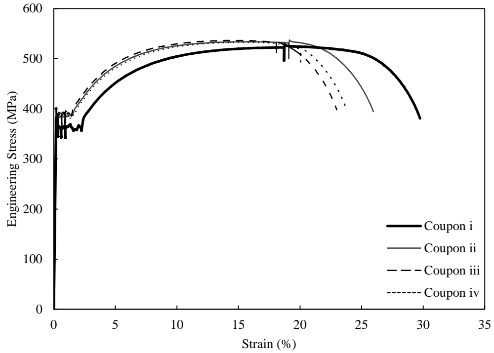
Figure C.5. Stress–strain curves for L102×102×6.4.
