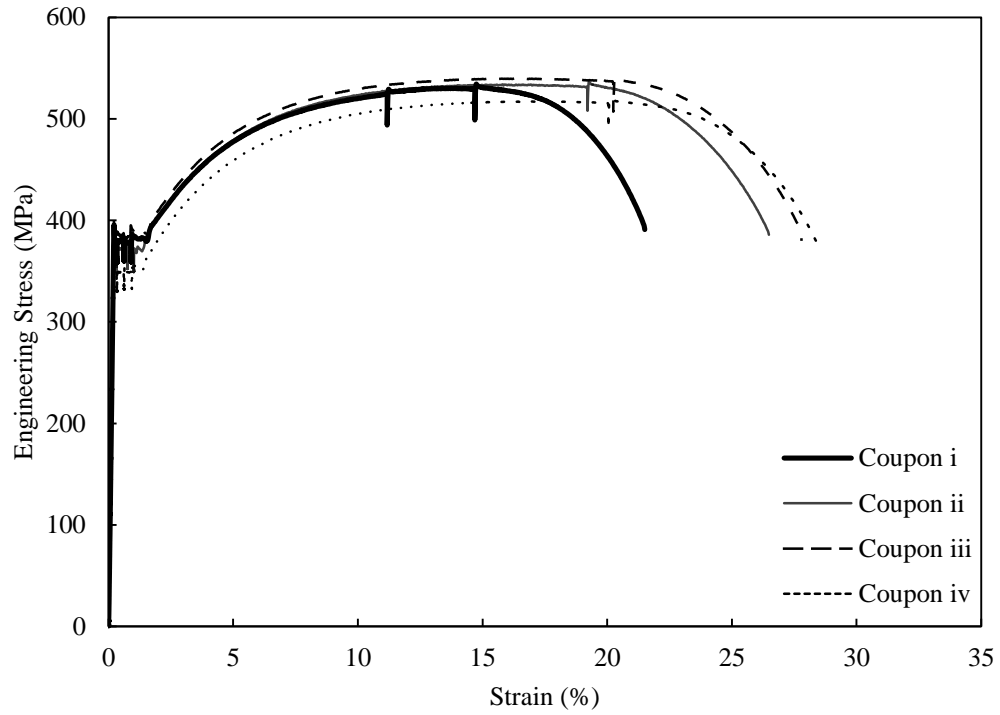
Figure C.3. Stress–strain curves for L89×89×9.5.
