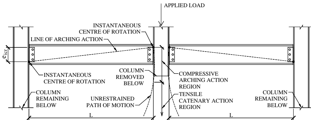
Figure 6.5. Development of compressive arching and tensile catenary action.
