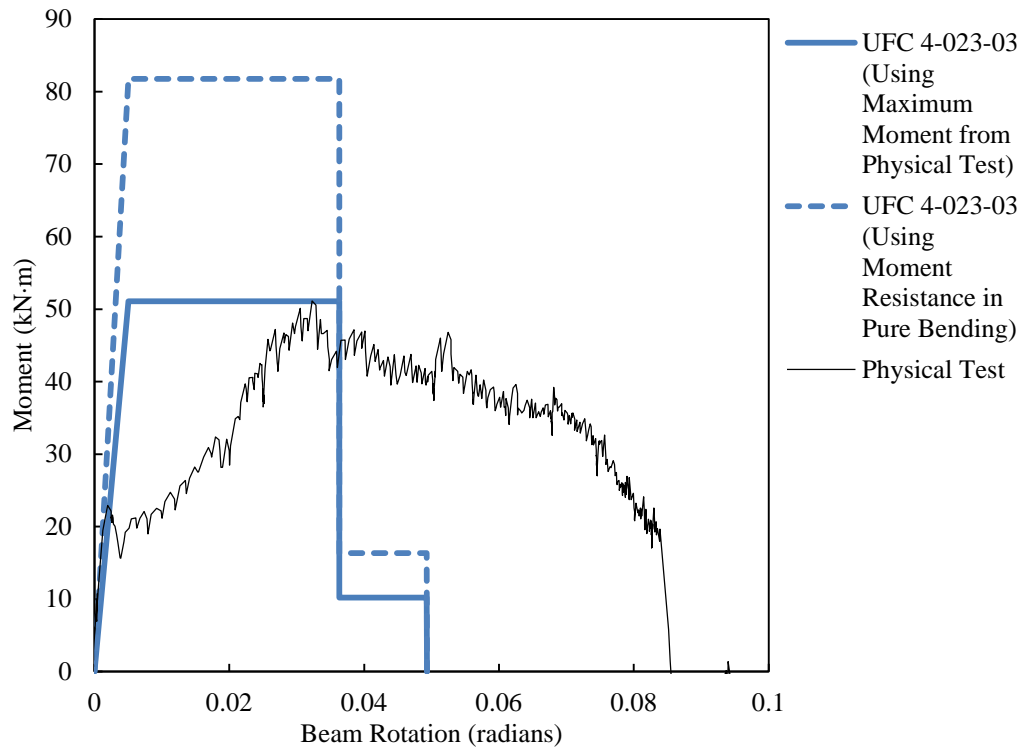
Figure 5.19. Comparison of moment versus rotation from UFC 4-023-03 (DoD, 2009) and test results for ST5A-2.
