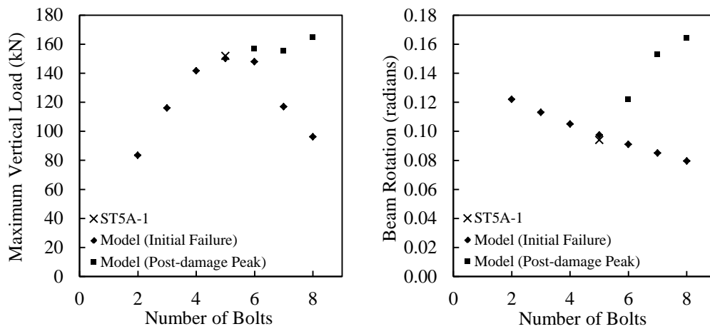
Figure 5.13. Parametric study: number of bolts.
