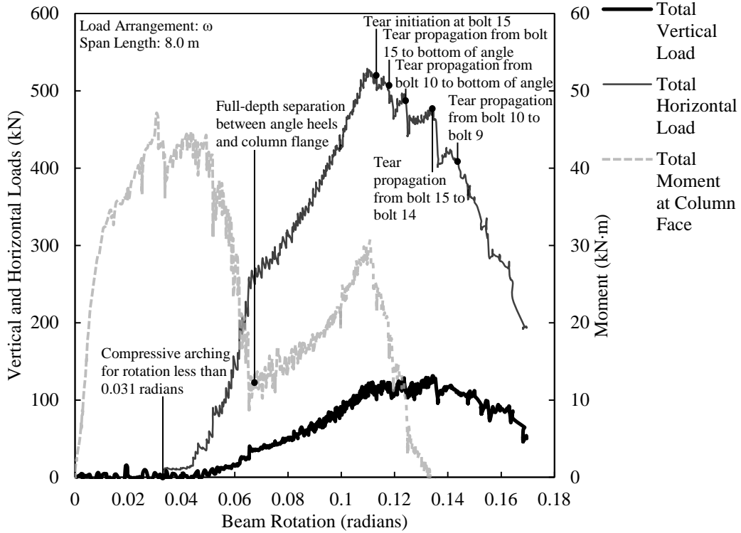
Figure D.33. Load versus rotation for DA5B-1.
