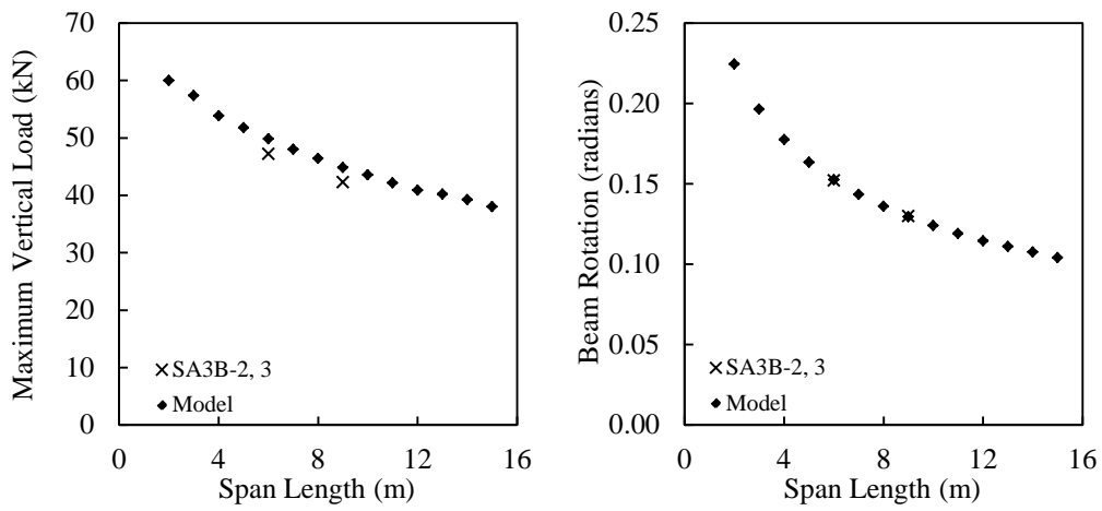
Figure 6.13. Parametric study: span length (three-bolt Series B connections).
