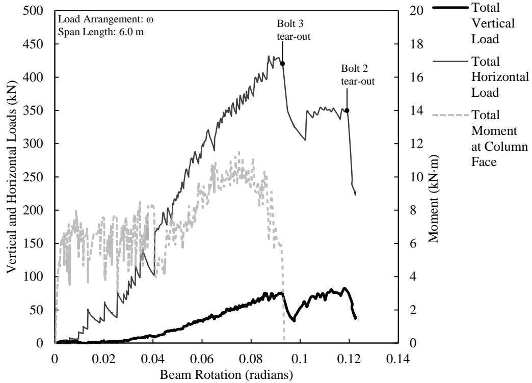
Figure 4.5. Load versus rotation for WA3A-2.
