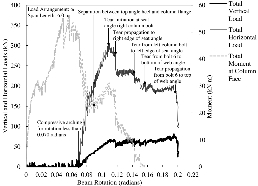
Figure D.40. Load versus rotation for SA3C-1.
