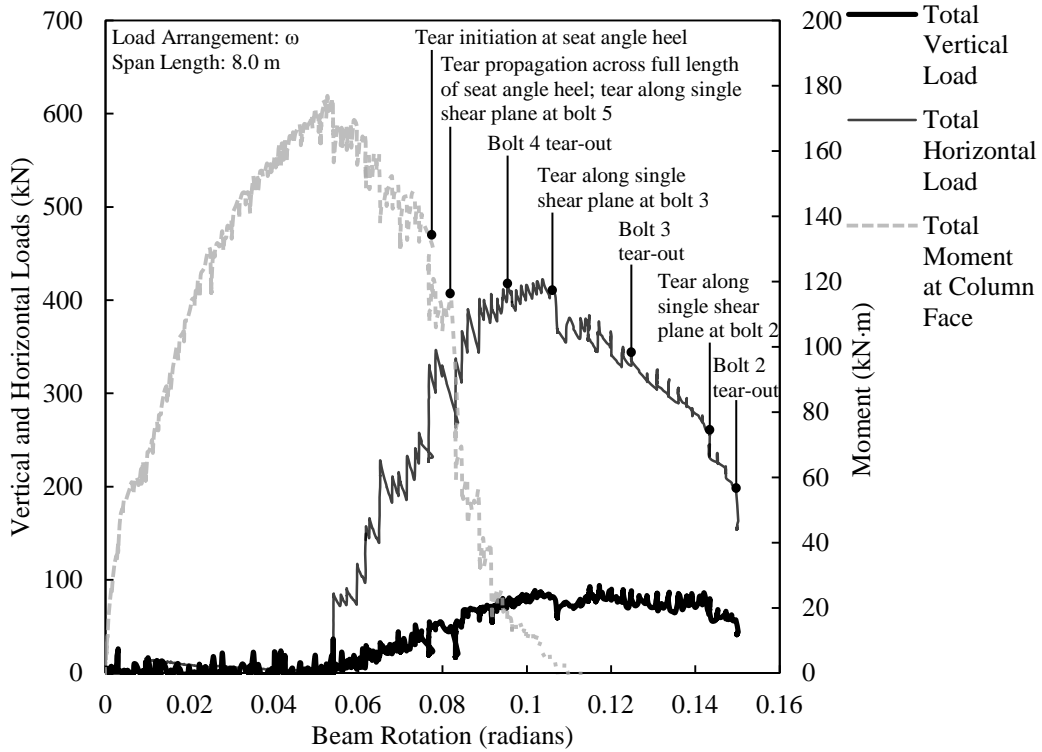
Figure D.38. Load versus rotation for ST5C-1.
