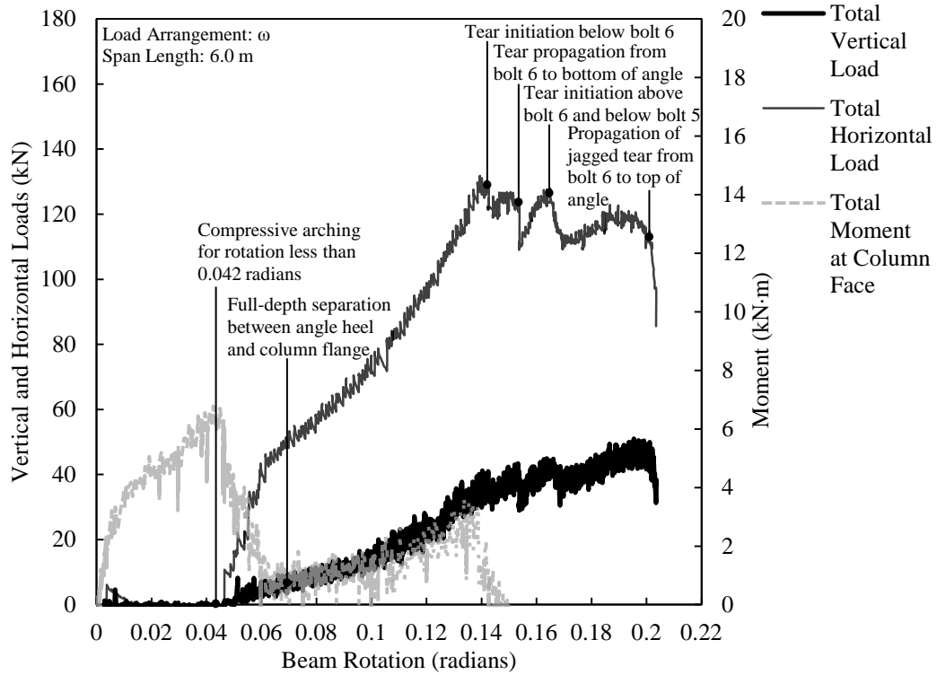
Figure 4.12. Load versus rotation for SA3B-2.
