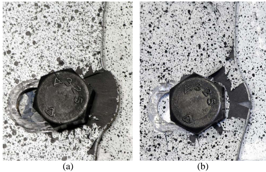
Figure 4.1. Deformation of shear tab connections under combined loading.
