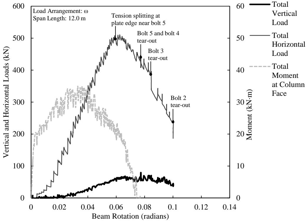
Figure D.9. Load versus rotation for ST5B-2.
