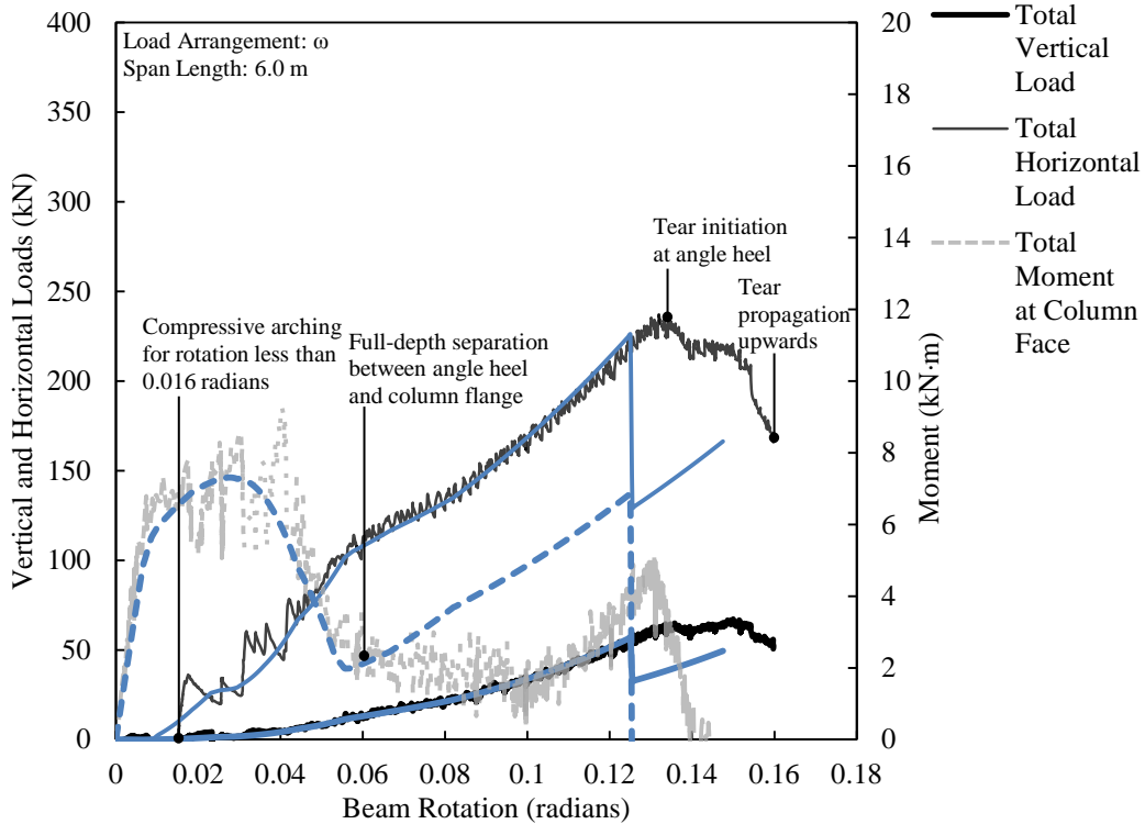
Figure 6.9. Comparison of mechanical model and test results for SA3A-4.
