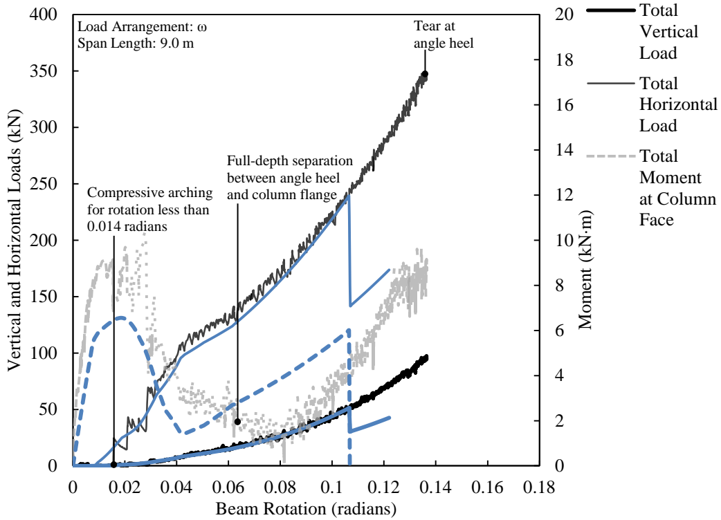
Figure 6.8. Comparison of mechanical model and test results for SA3A-3.
