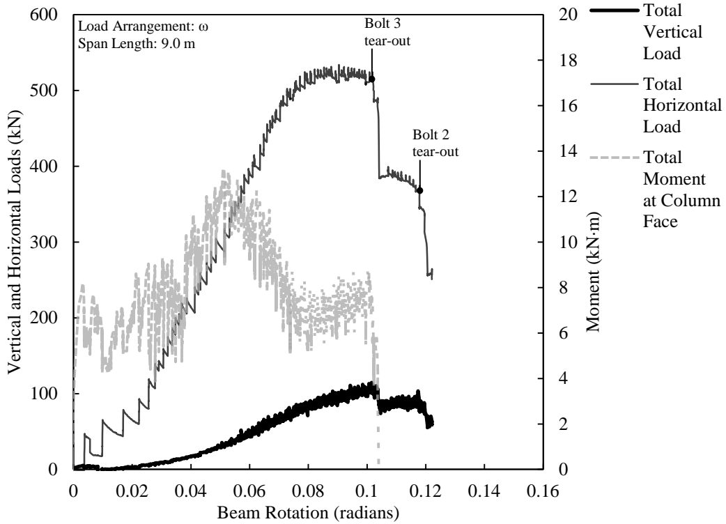
Figure D.3. Load versus rotation for ST3A-3.
