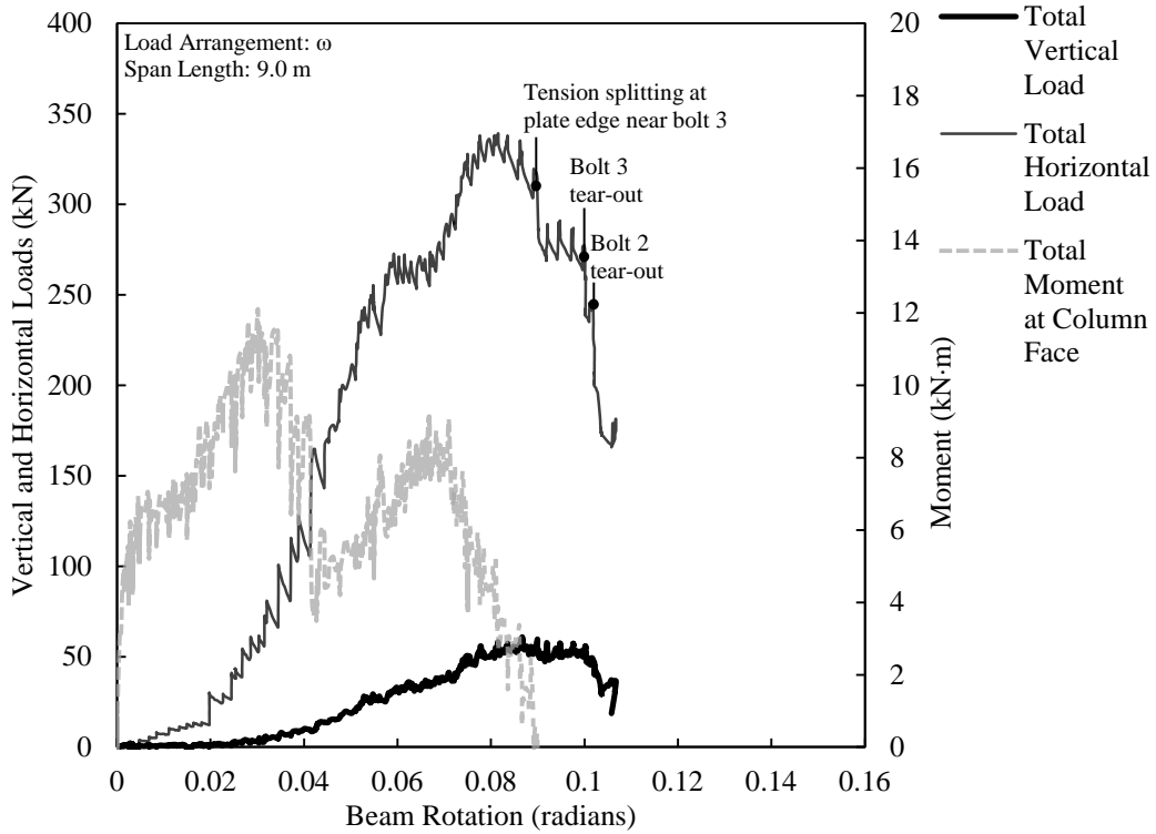
Figure D.5. Load versus rotation for ST3B-2.
