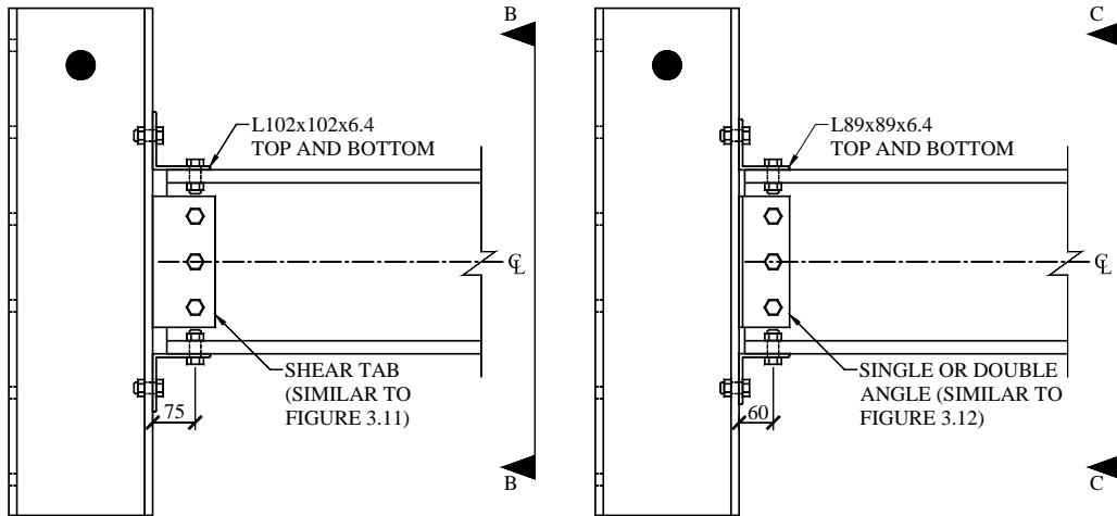
Figure 3.14. Combined seat and top angle connection details.
