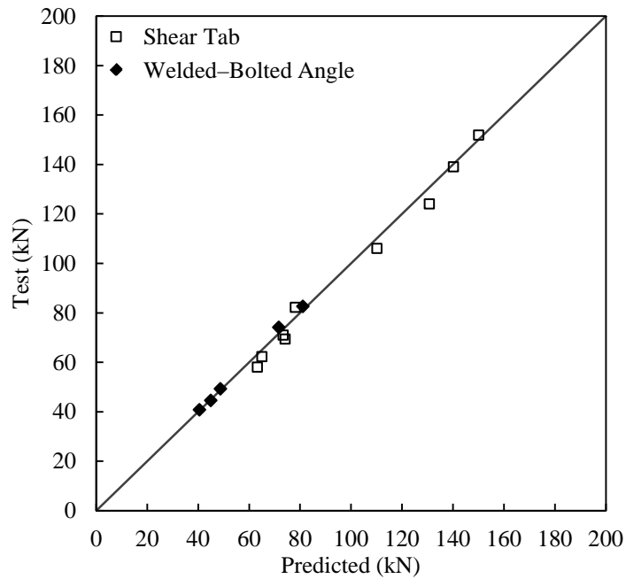
Figure 5.11. Comparison of mechanical model and test results for maximum vertical load.
