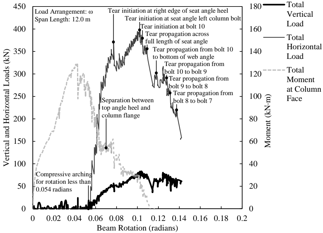
Figure D.43. Load versus rotation for SA5C-2.
