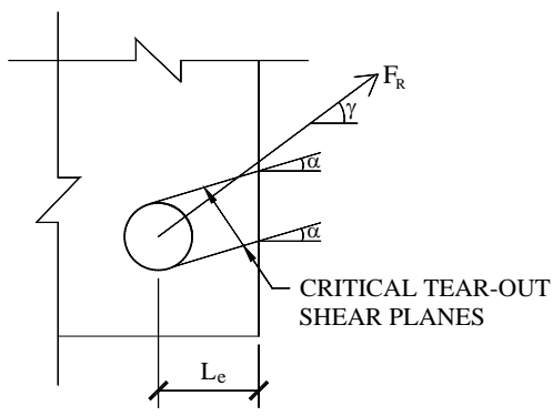
Figure 5.3. Bolt tear-out under an inclined force.
