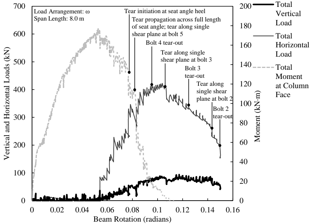
Figure 4.18. Load versus rotation for ST5C-1.
