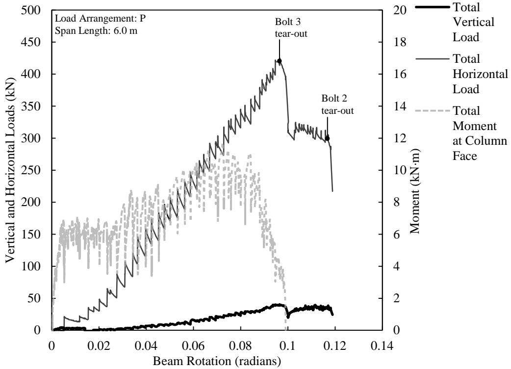
Figure D.10. Load versus rotation for WA3A-1.
