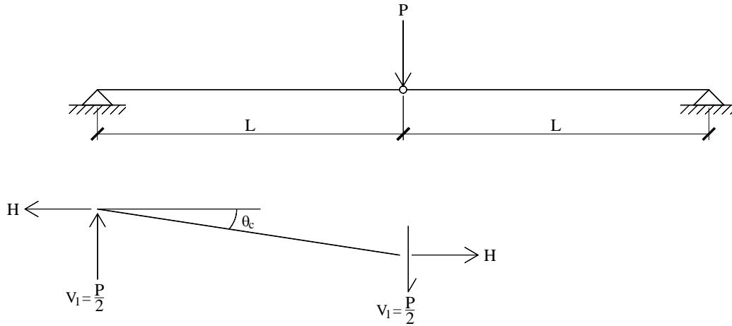
Figure 3.5. Three-hinged beam under point load (after Timoshenko, 1955).
