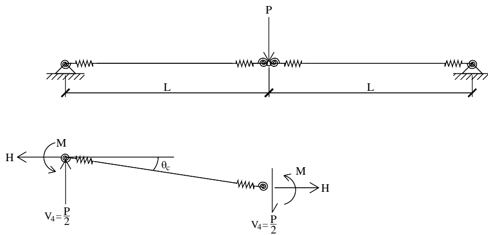
Figure 3.7. Modified three-hinged beam with connections represented by springs.
