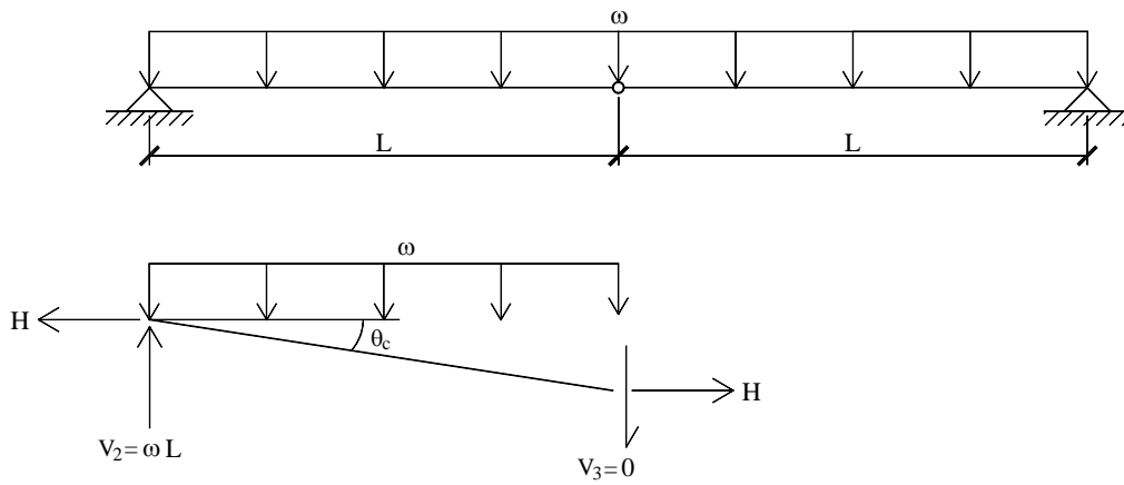
Figure 3.6. Three-hinged beam under uniformly distributed load.
