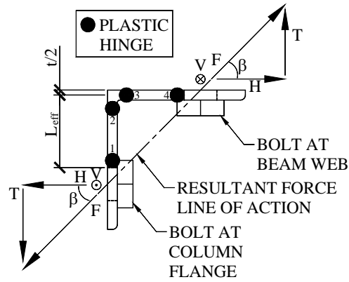
Figure 6.3. Plastic hinge formation in angle segments under tension.
