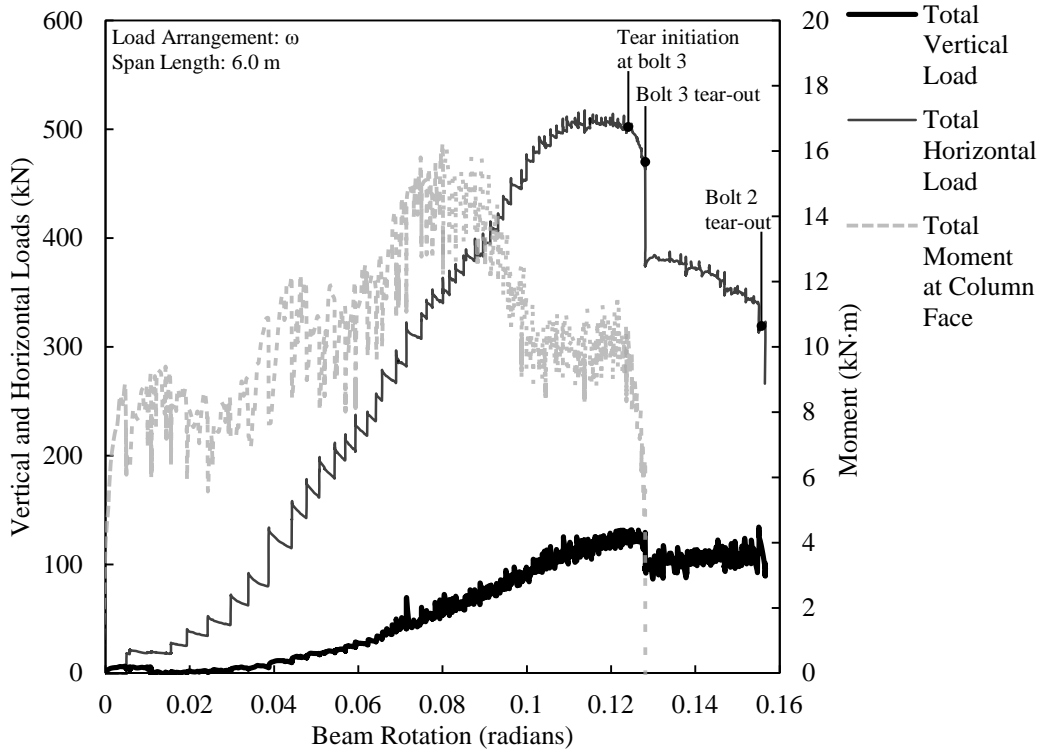
Figure D.2. Load versus rotation for ST3A-2.
