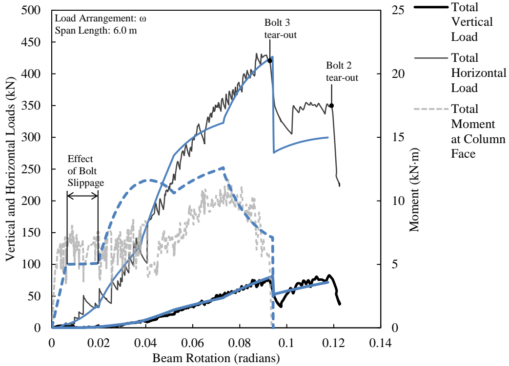
Figure 5.10. Comparison of mechanical model and test results for WA3A-2.
