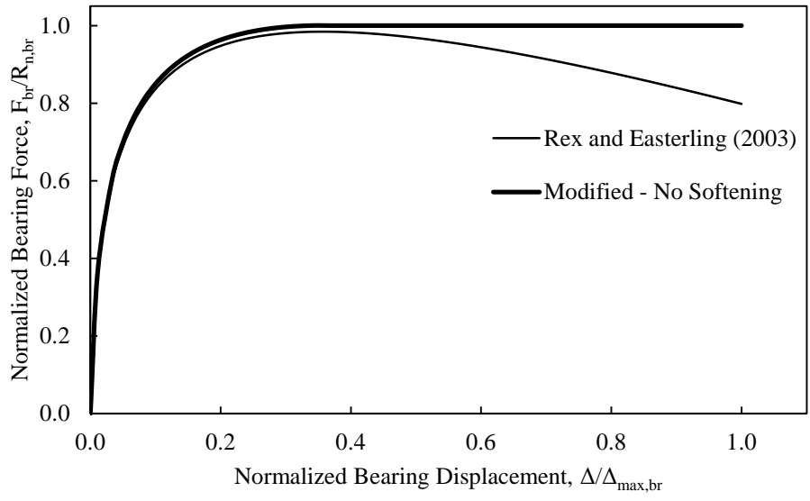
Figure 5.4. Force versus displacement for bearing deformations.
