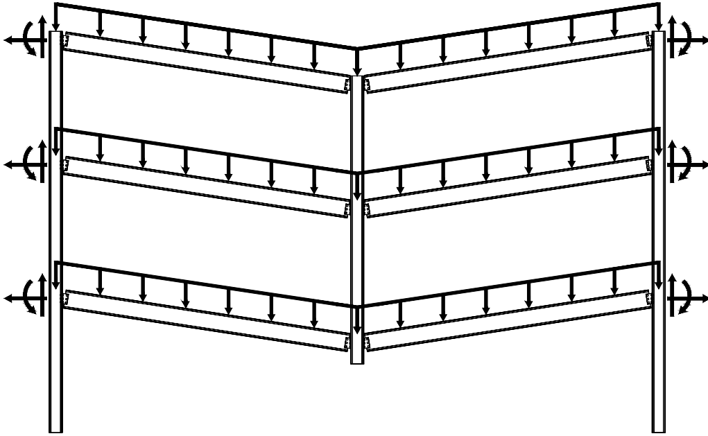
Figure 1.1. Catenary action in a gravity frame following column removal.
