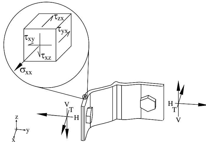
Figure 6.4. Stress state at plastic hinge near column bolt line.
