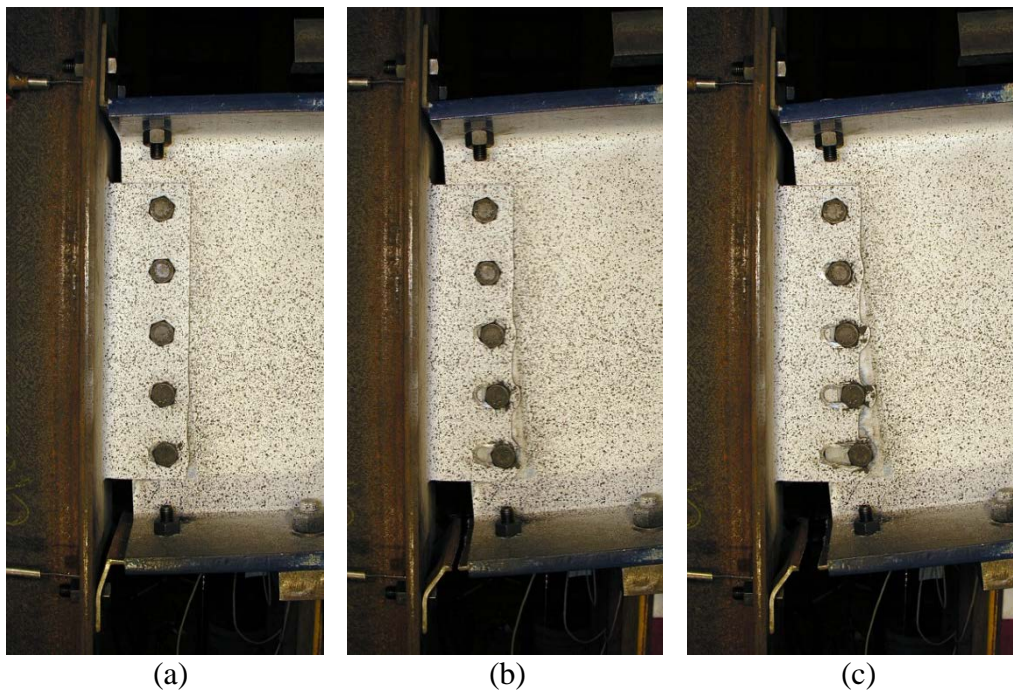
Figure 4.19. Shear tab with seat and top angles specimen ST5C-1 at: (a) 0.05 radians (maximum moment), (b) 0.083 radians (seat angle failure), and (c) 0.114 radians (peak post-damage response).
