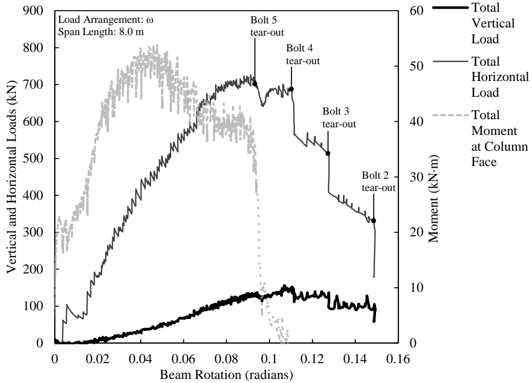
Figure 4.3. Load versus rotation for ST5A-1.
