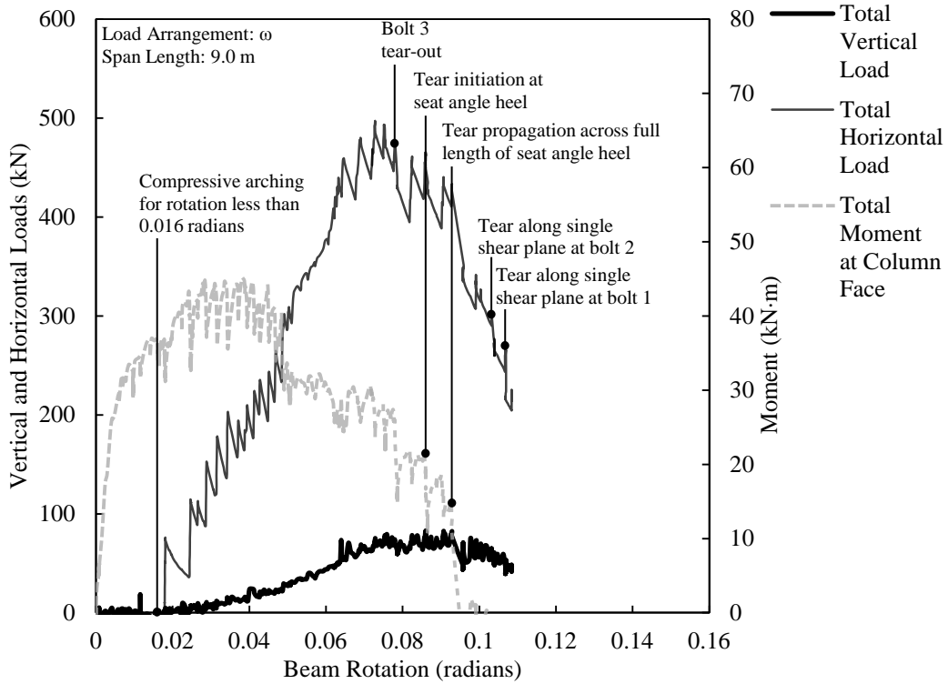
Figure D.37. Load versus rotation for ST3C-2.
