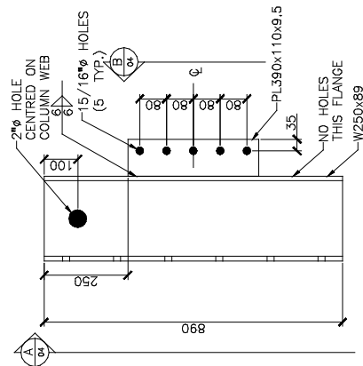
DETAIL 3 SHEAR TAB ASSEMBLY ST15A (QTY. 2) SCALE: 1:20
