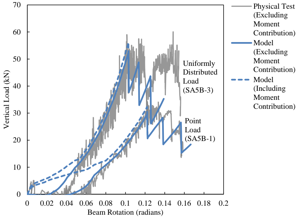
Figure 6.17. Parametric study: loading arrangement (proportion of vertical to horizontal load).
