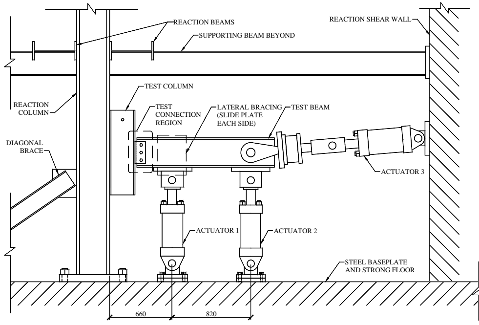
Figure 3.1. Schematic of test set-up.
