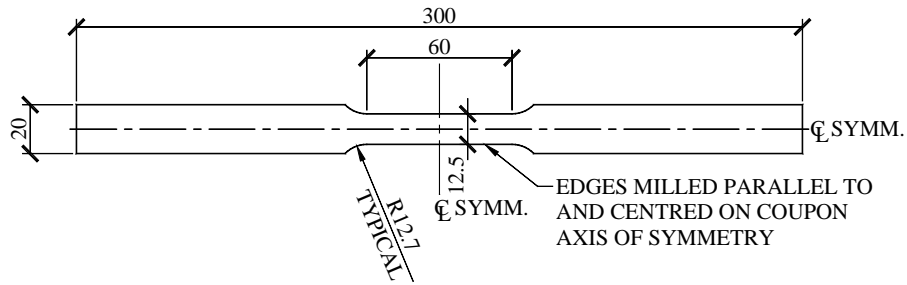
Figure 3.16. Tension coupon profile.
