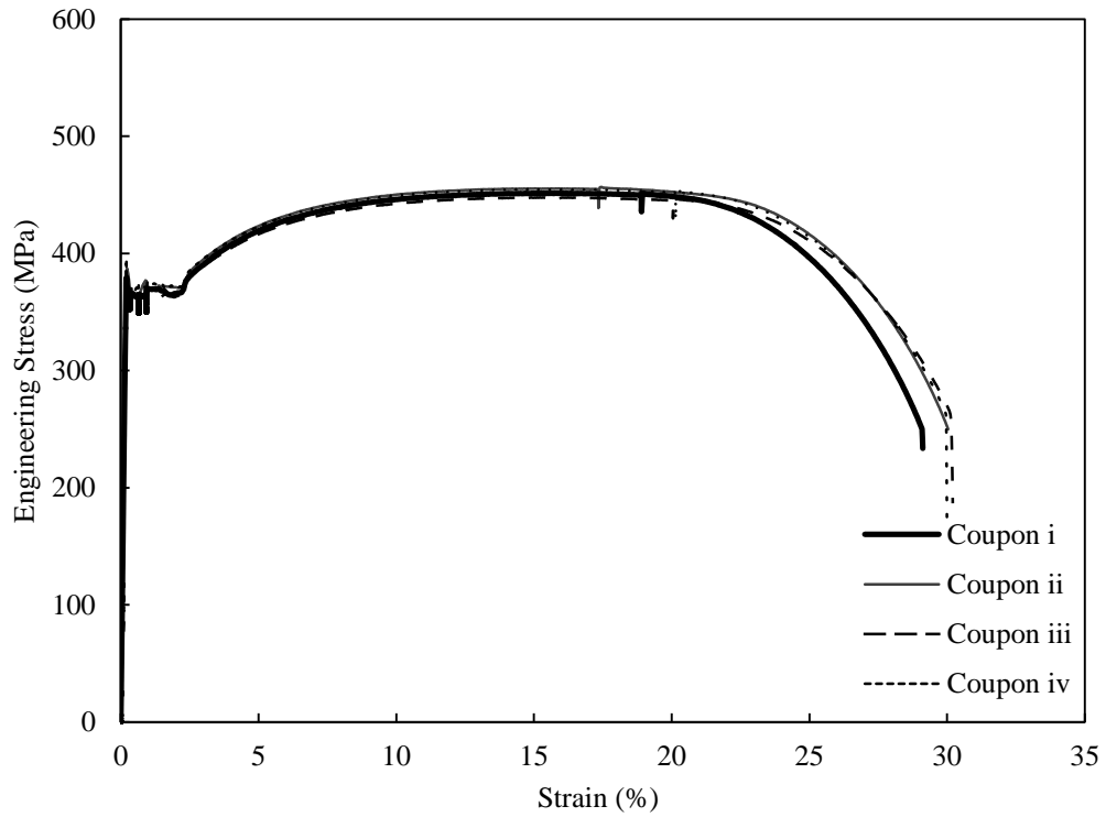
Figure C.1. Stress–strain curves for 9.5 mm plate.
