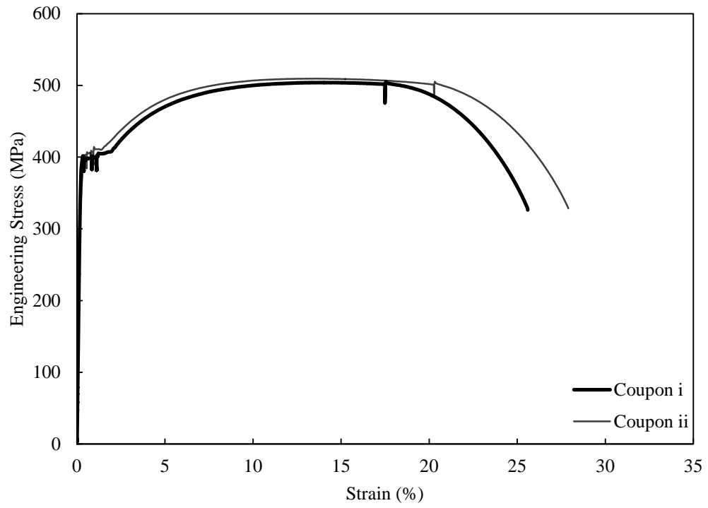
Figure C.7. Stress–strain curves for W250×89 web.
