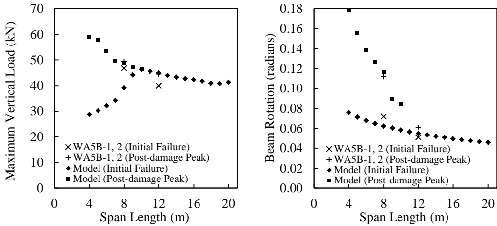
Figure 5.15. Parametric study: span length (five-bolt connections).
