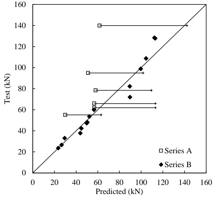
Figure 6.10. Comparison of mechanical model and test results for maximum vertical load.
