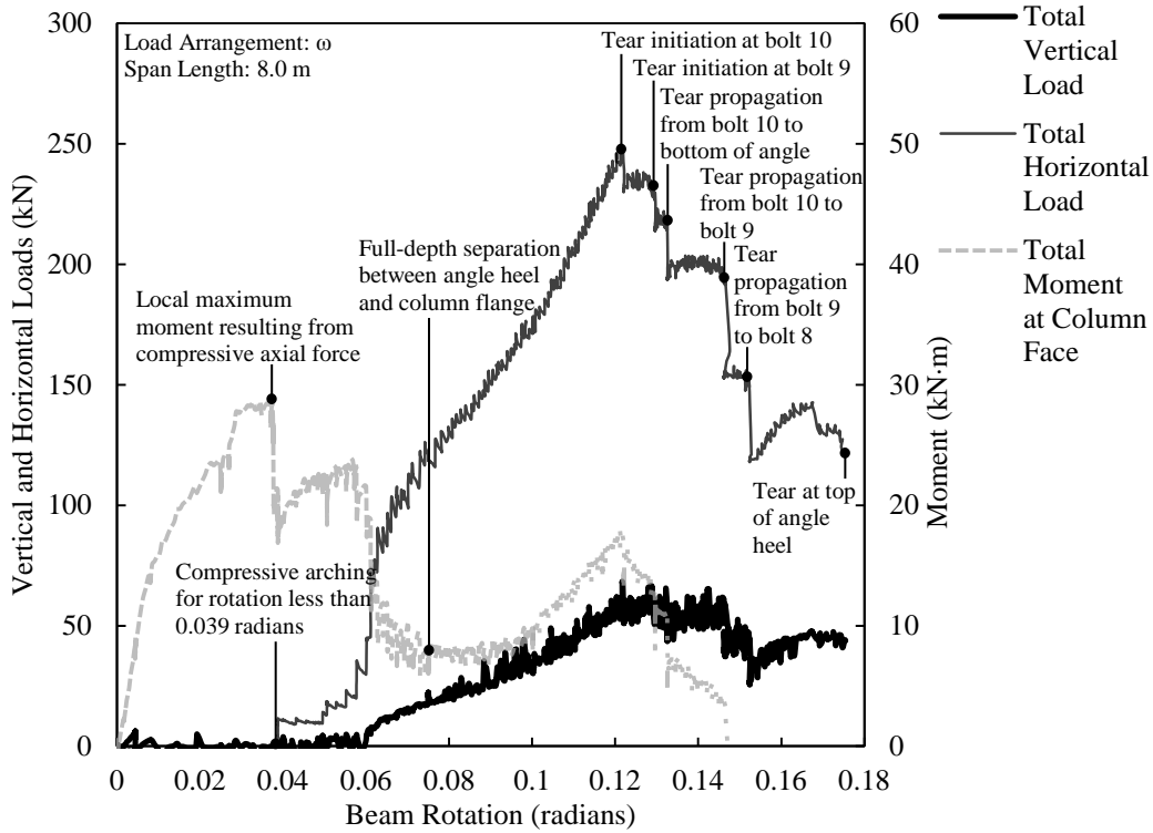
Figure D.27. Load versus rotation for SA5B-2.
