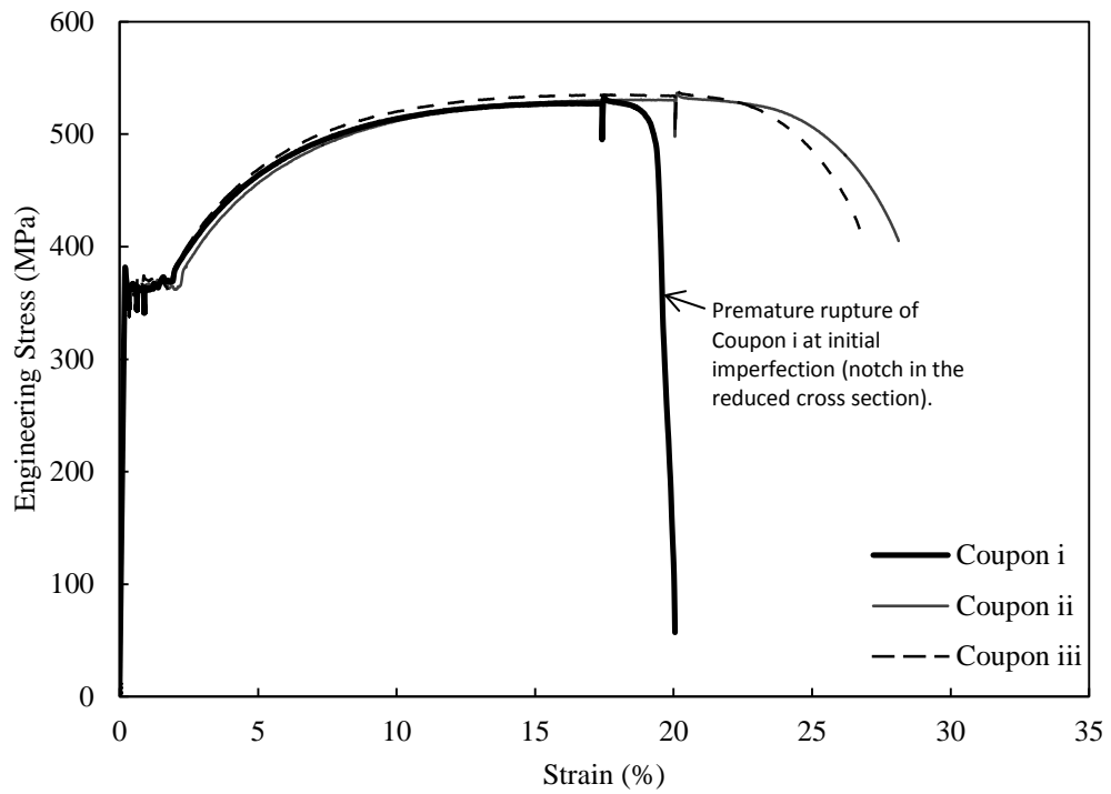
Figure C.4. Stress–strain curves for L89×89×6.4.
