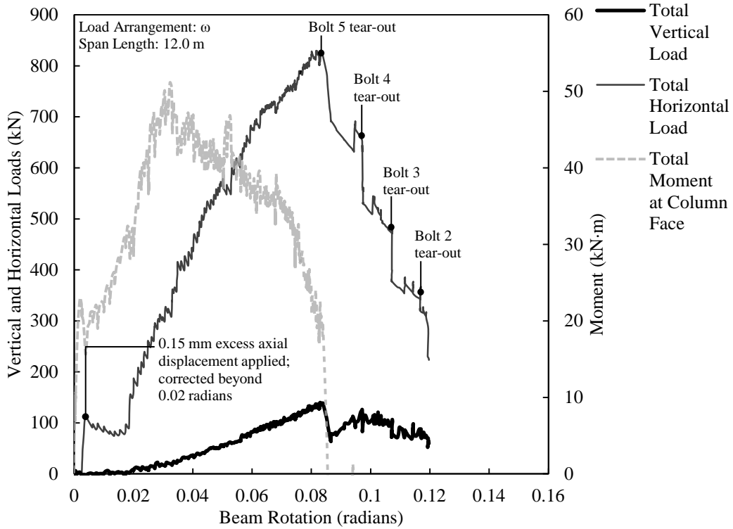
Figure D.7. Load versus rotation for ST5A-2.
