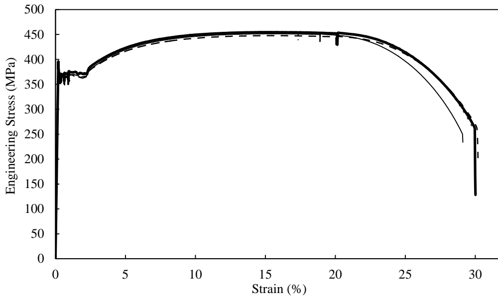
Figure 3.18. Stress-strain curves for tension coupons from 9.5 mm plate.
