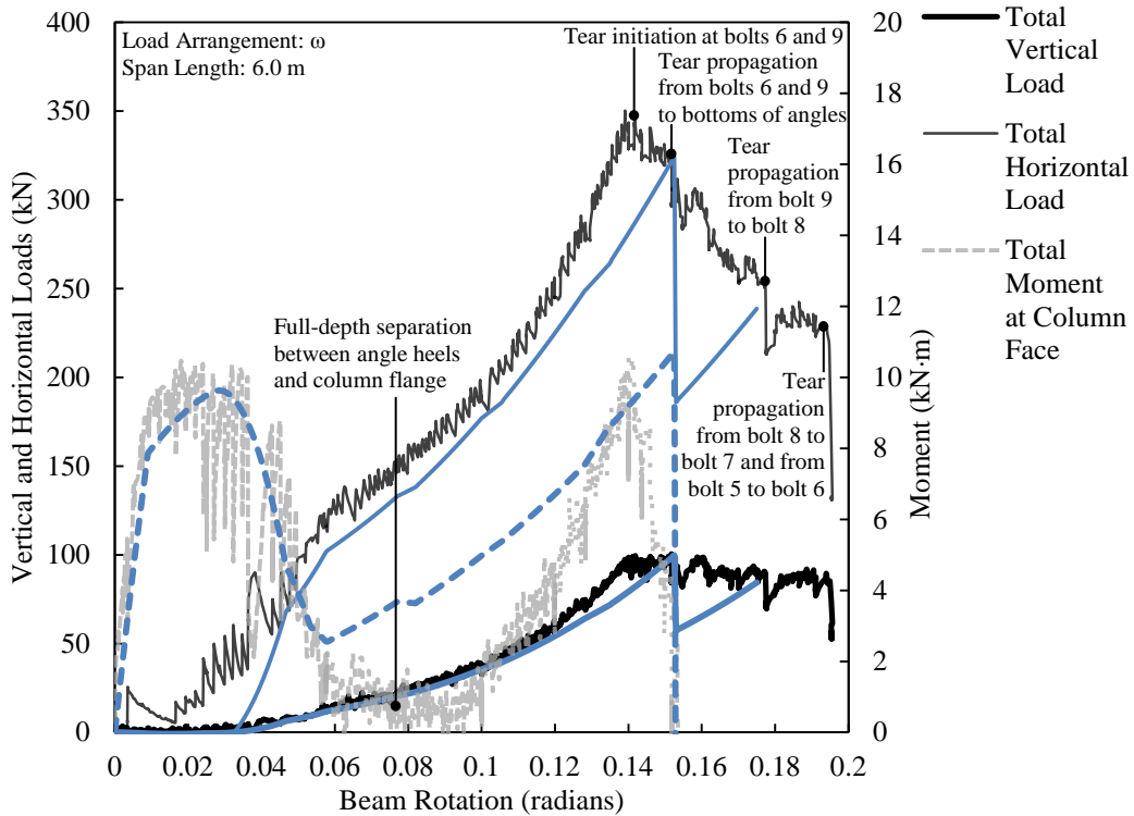
Figure 6.7. Comparison of mechanical model and test results for DA3B-1.
