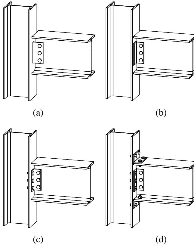
Figure 1.2. Common shear connection types: (a) shear tab, (b) welded-bolted angle, (c) bolted-bolted angle, and (d) combined seat and top angle with bolted-bolted web angle.
