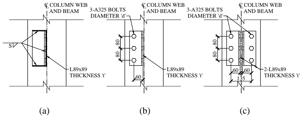
Figure 3.13. Section A-A from Figure 3.12 for: (a) welded-bolted single angle, (b) bolted-bolted single angle, and (c) bolted-bolted double angle.
