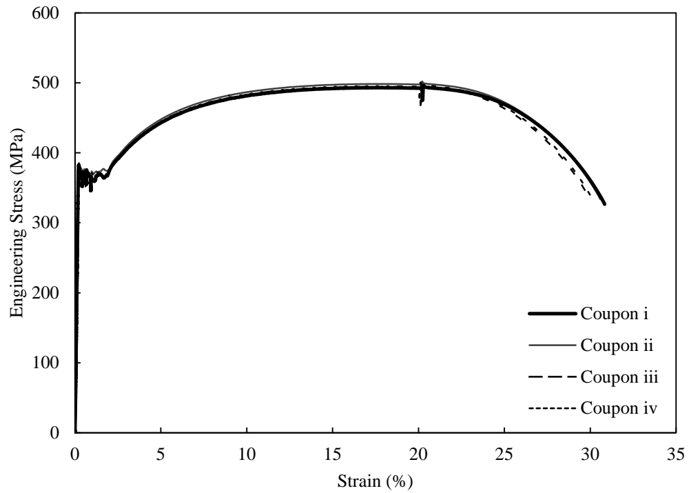
Figure C.6. Stress–strain curves for W250×89 flanges.
