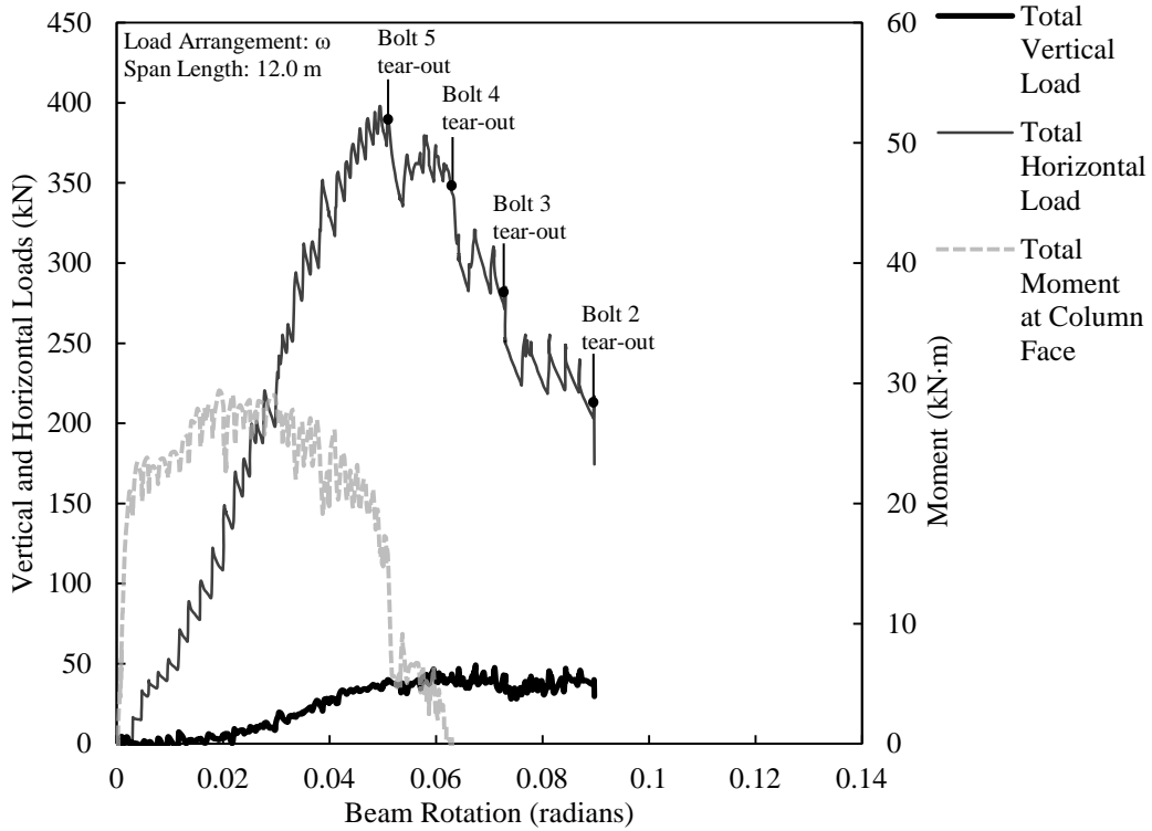
Figure D.14. Load versus rotation for WA5B-2.
