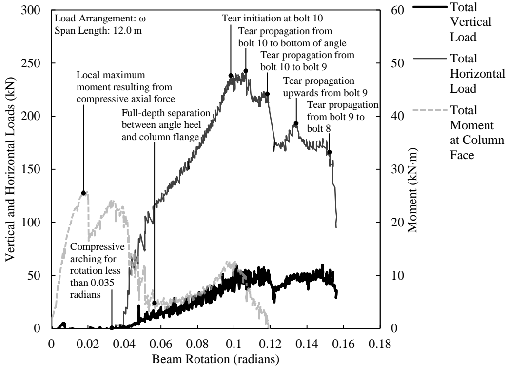
Figure D.28. Load versus rotation for SA5B-3.
