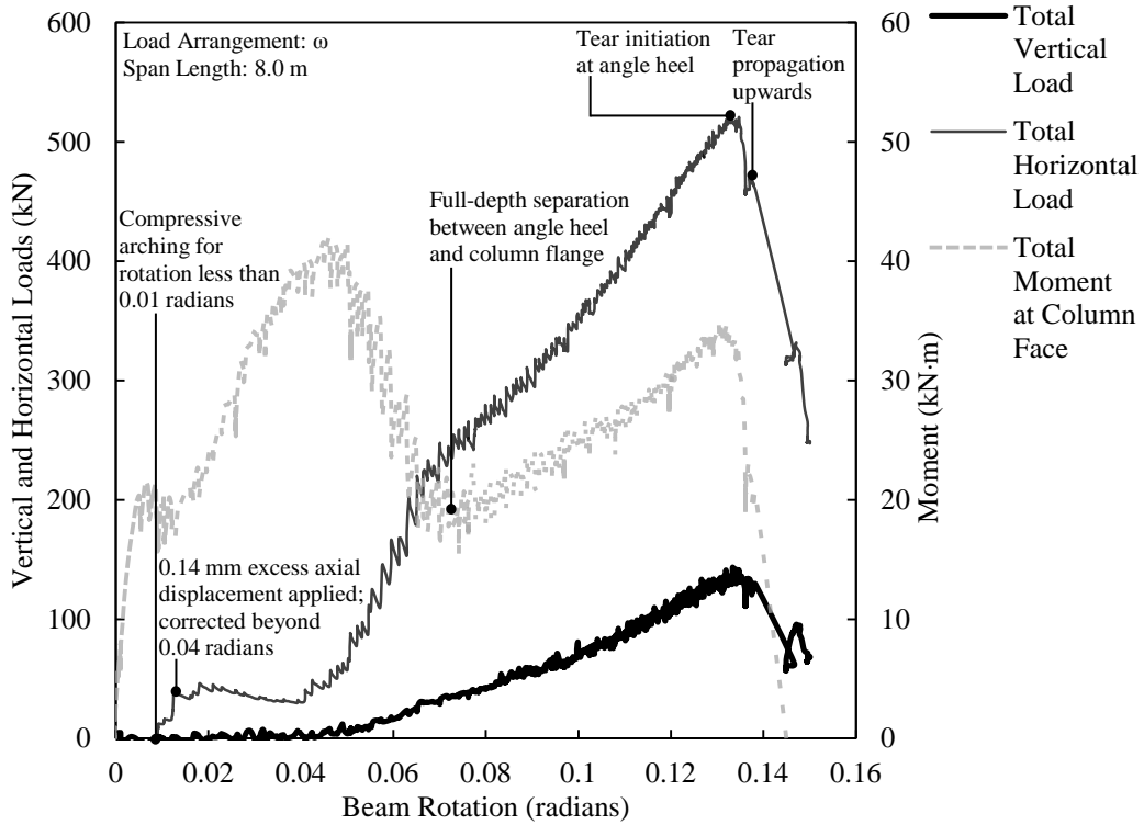
Figure D.24. Load versus rotation for SA5A-1.
