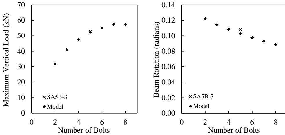
Figure 6.12. Parametric study: number of bolts.
