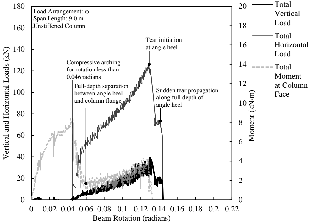
Figure D.23. Load versus rotation for SA3B-5.
