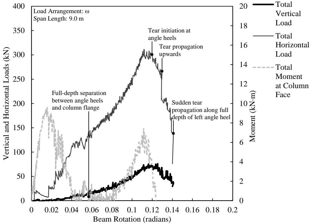
Figure D.31. Load versus rotation for DA3B-2.
