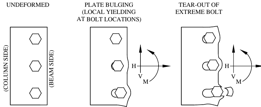
Figure 4.1. Deformation of shear tab connections under combined loading.
