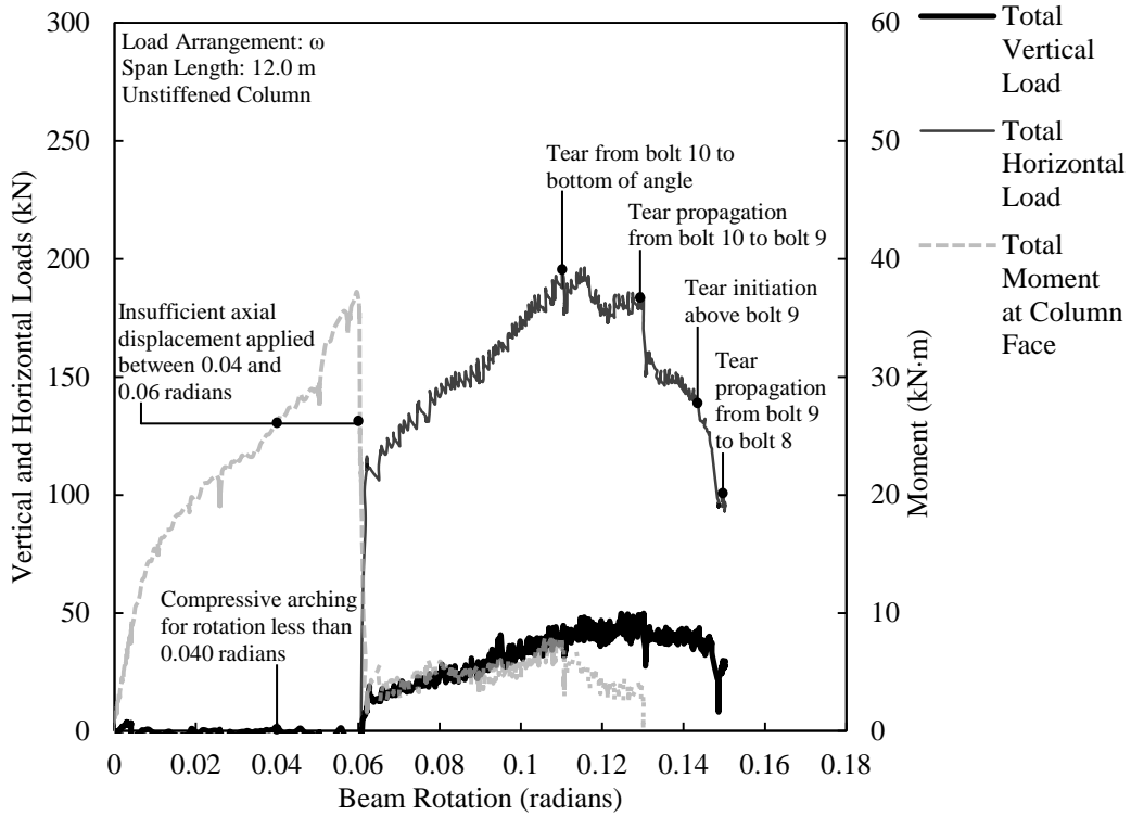
Figure D.29. Load versus rotation for SA5B-4.
