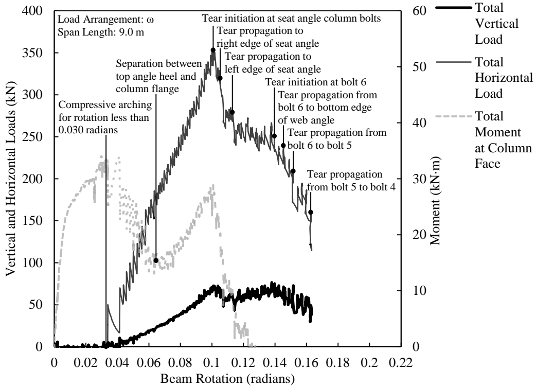
Figure D.41. Load versus rotation for SA3C-2.
