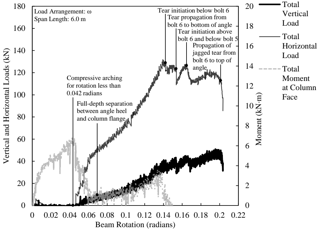
Figure D.20. Load versus rotation for SA3B-2.
