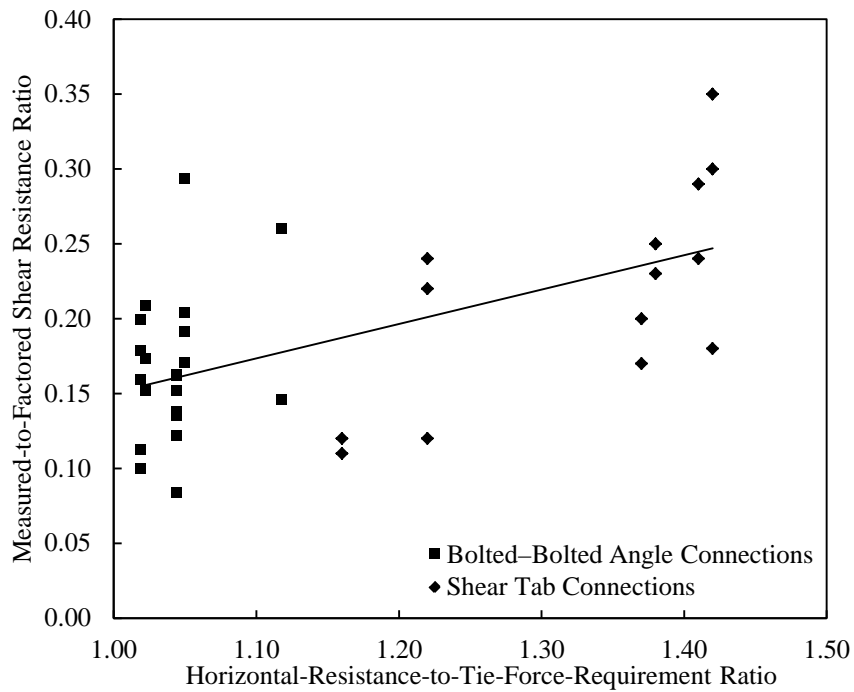
Figure 6.18. Comparison of tie force resistance and vertical load performance following column removal.
