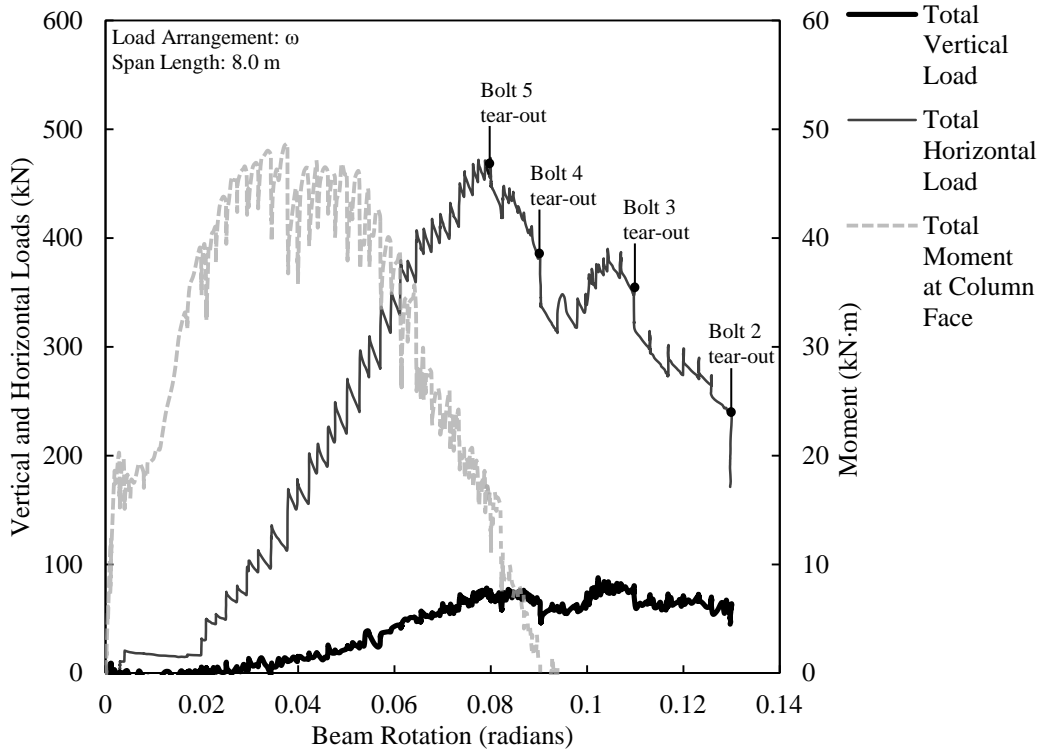
Figure D.8. Load versus rotation for ST5B-1.
