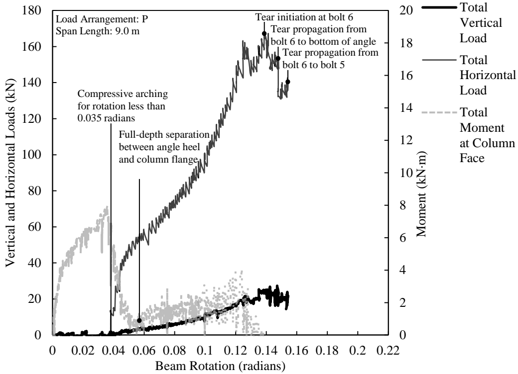
Figure D.19. Load versus rotation for SA3B-1.
