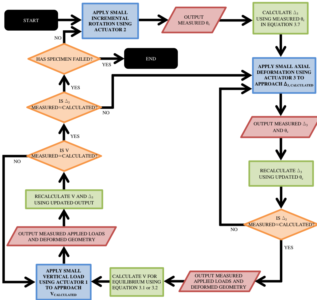
Figure 3.8. Load application flow chart.
