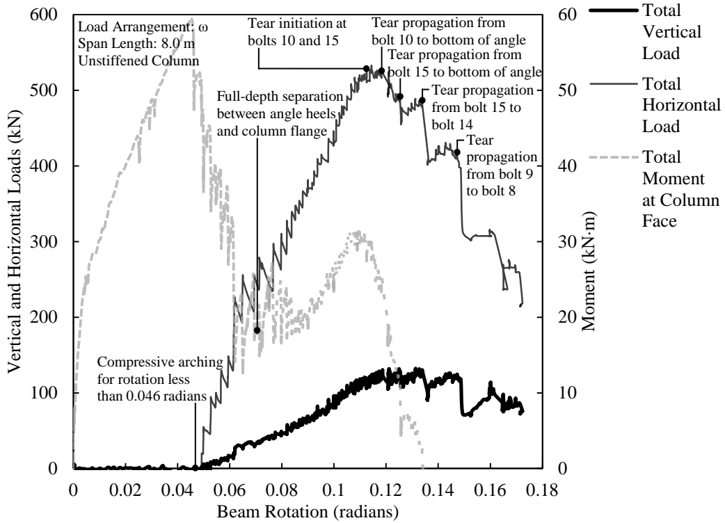
Figure D.35. Load versus rotation for DA5B-3.
