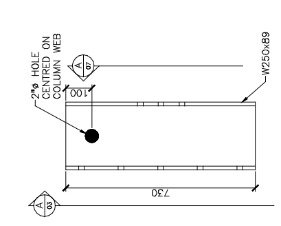
DETAIL 1 COLUMN FOR S43B/DA3B (QTY. 2) SCALE: 1:20
