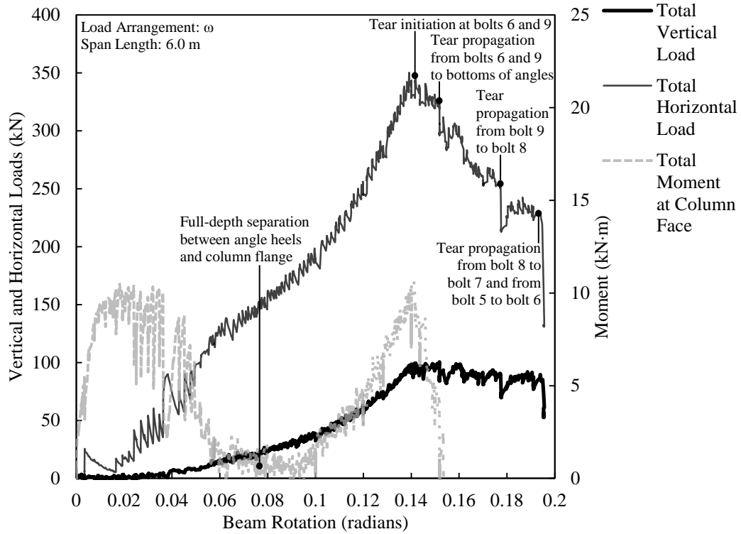
Figure 4.14. Load versus rotation for DA3B-1.
