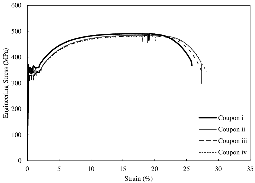
Figure C.2. Stress–strain curves for 6.4 mm plate.
