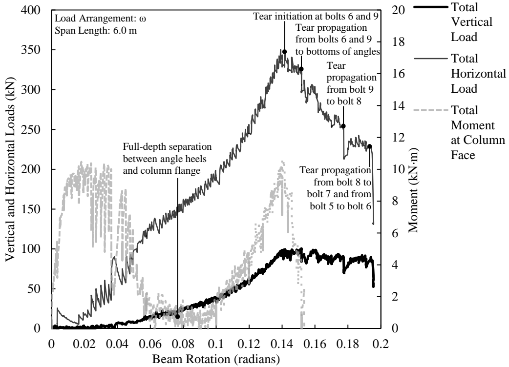
Figure D.30. Load versus rotation for DA3B-1.
