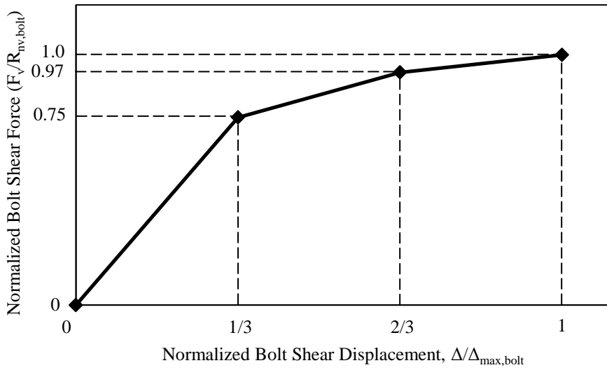
Figure 5.5. Force versus displacement for bolts in single shear.
