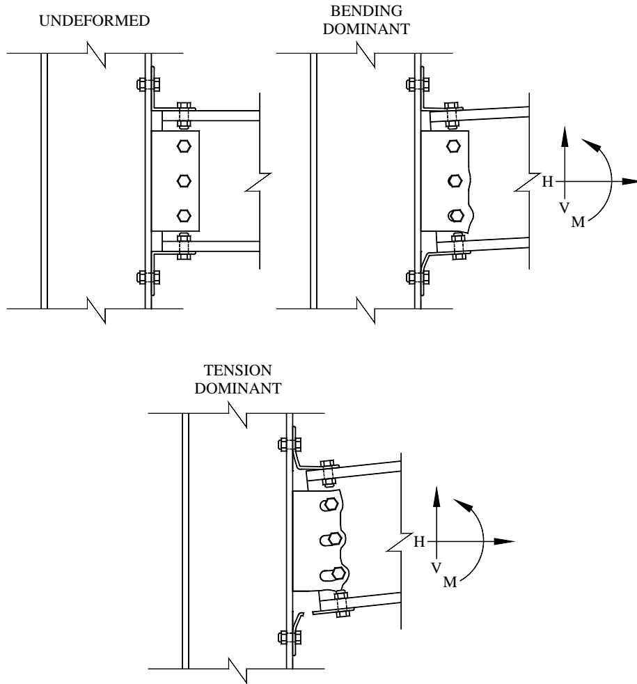
Figure 4.16. Deformation of combined seat and top angle connections (with shear tab) under combined loading.
