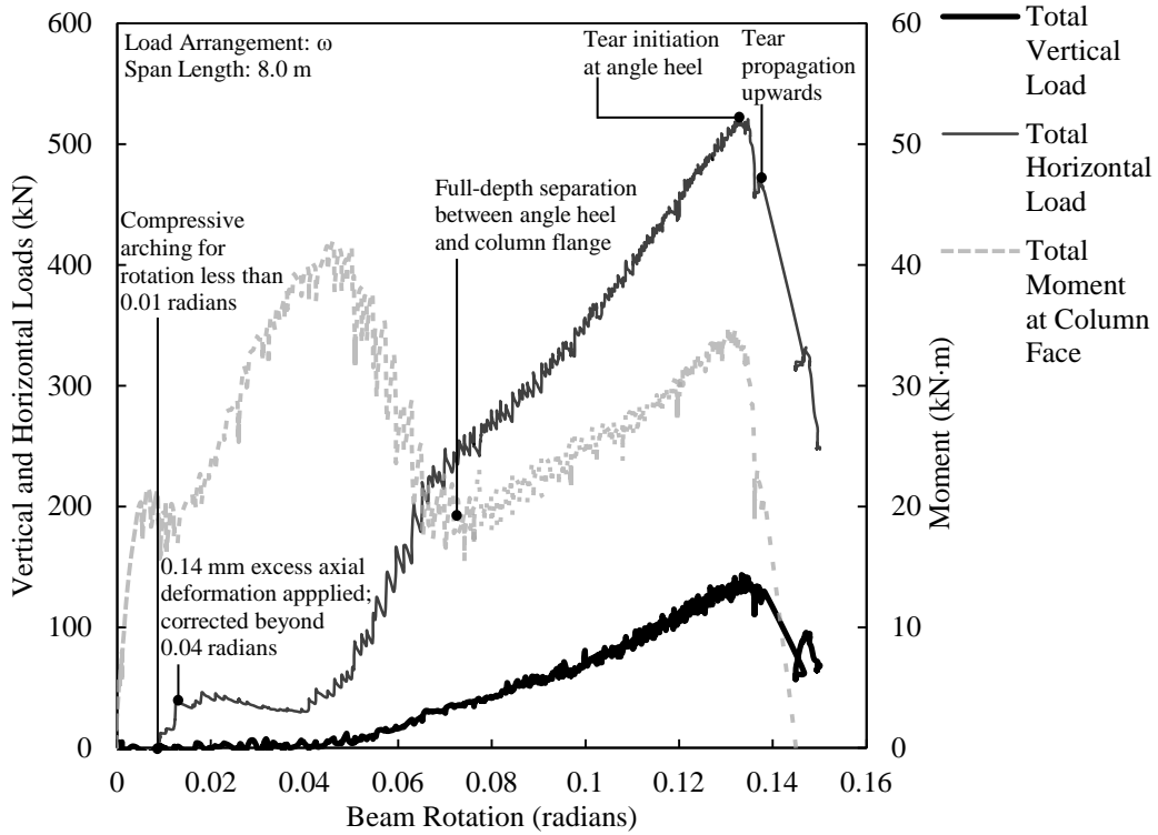
Figure 4.10. Load versus rotation for SA5A-1.
