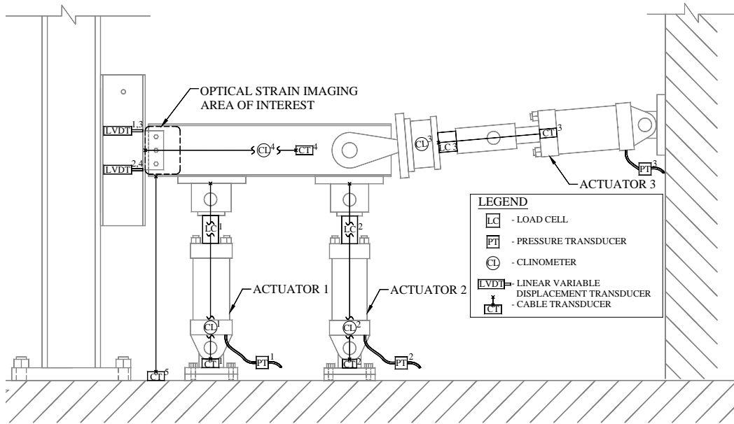
Figure 3.3. Instrumentation diagram.
