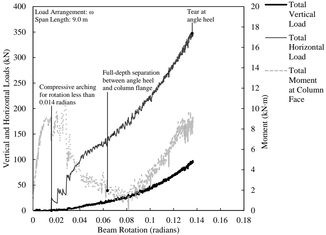
Figure D.17. Load versus rotation for SA3A-3.
