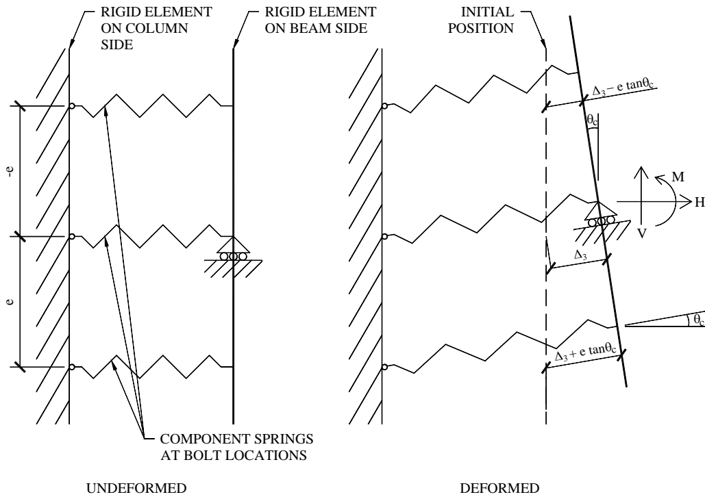
Figure 5.2. Mechanical model of shear tab connections.
