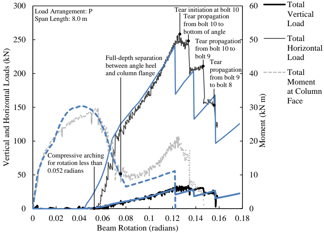
Figure 6.6. Comparison of mechanical model and test results for SA5B-1.
