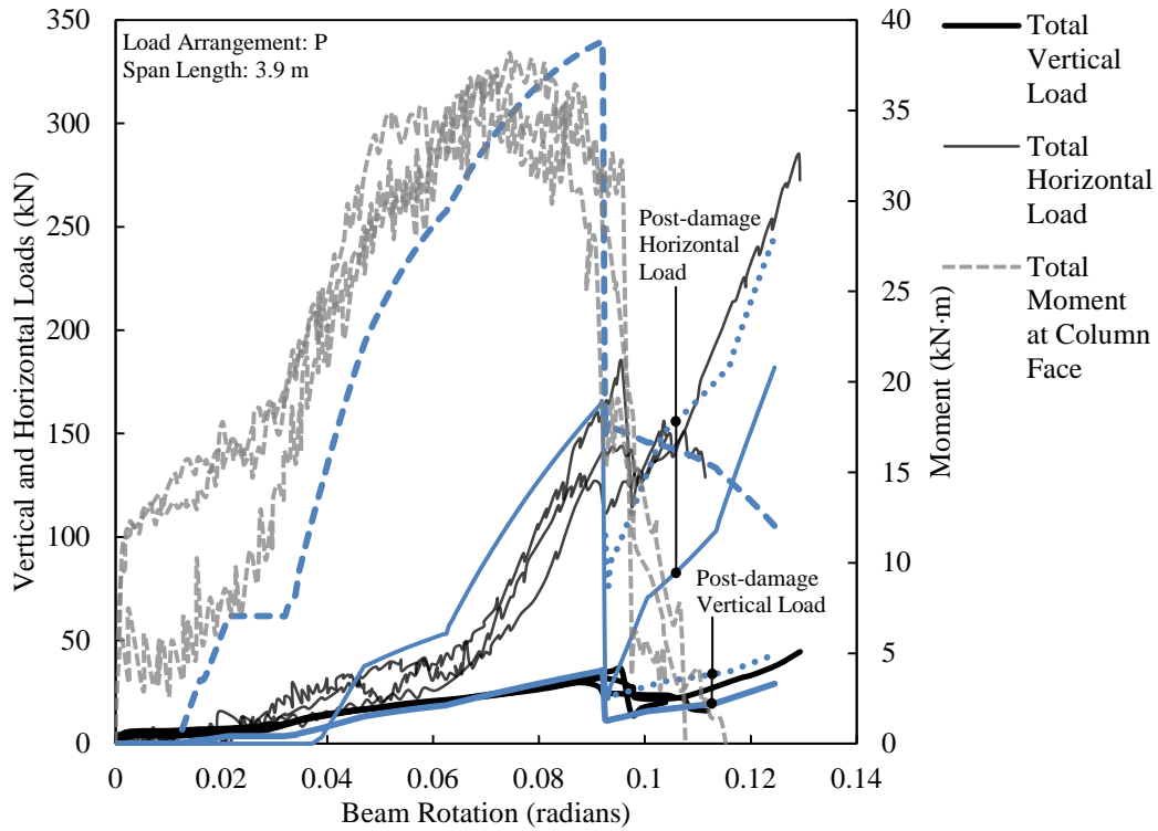
Figure 5.12. Comparison of mechanical model and test results for four-bolt column removal tests by Thompson (2009).
