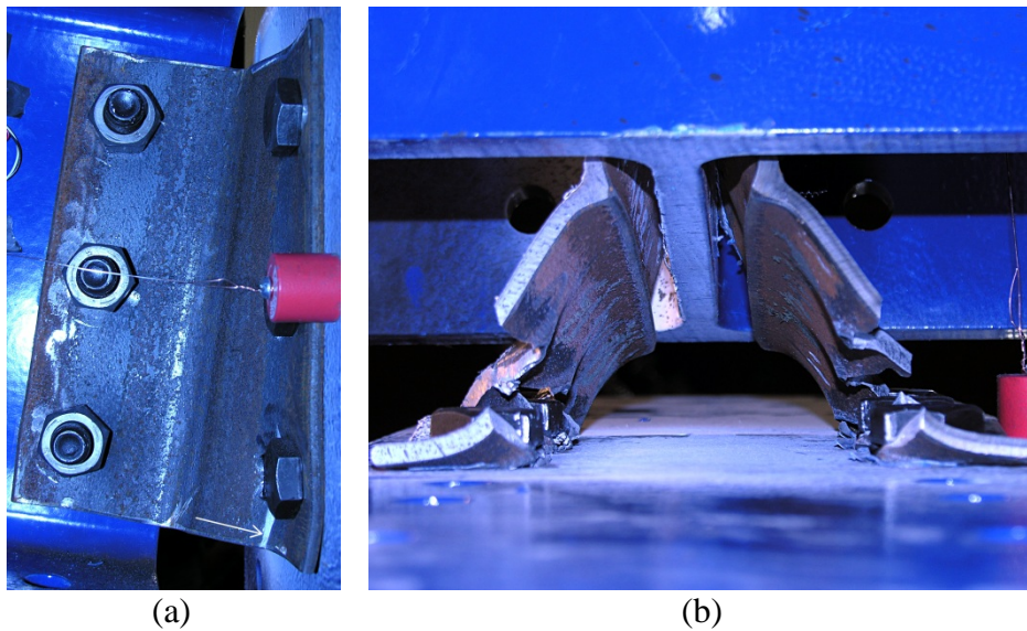
Figure 4.15. Double angle specimen DA3B-1 at: (a) 0.149 radians (tear to angle bottom), and (b) 0.194 radians (bottom view).
