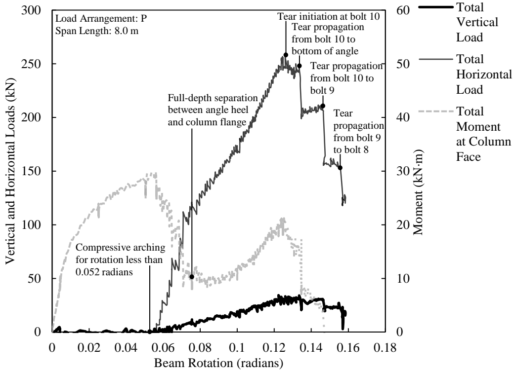
Figure D.26. Load versus rotation for SA5B-1.
