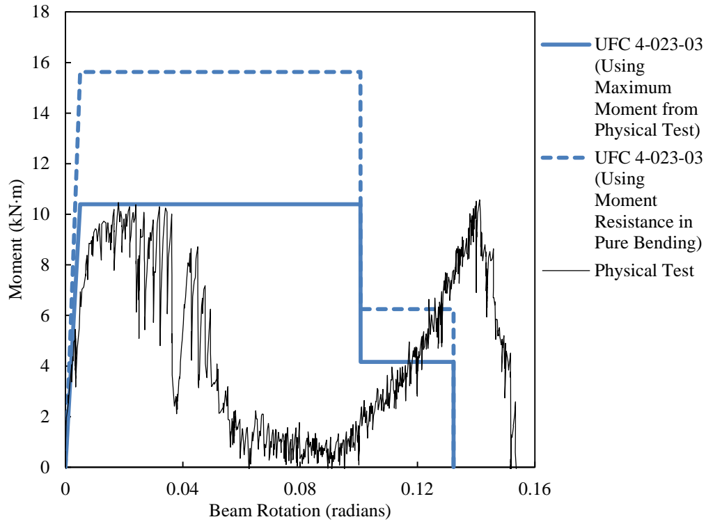
Figure 6.19. Comparison of moment versus rotation from UFC 4-023-03 (DoD, 2009) and test results for DA3B-1.
