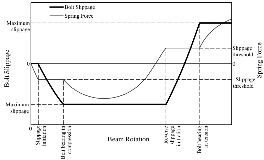
Figure 5.7. Representative behaviour of the bolt slippage function for a top bolt (including force direction change).
