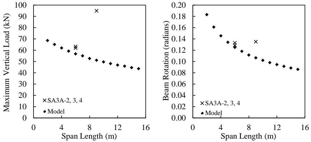
Figure 6.15. Parametric study: span length (three-bolt Series A connections).
