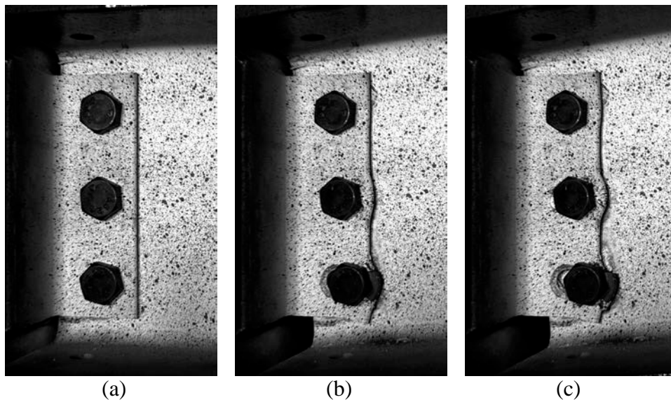
Figure 4.6. Specimen WA3A-2 at: (a) 0 radians (undeformed), (b) 0.089 radians (extreme bolt tear-out), and (c) 0.118 radians (bolt 2 tear-out, peak post-damage response).
