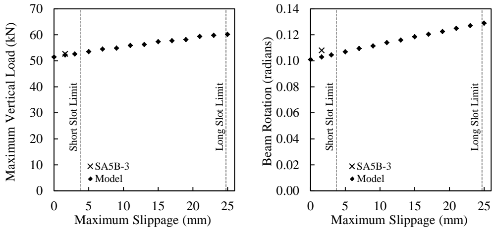
Figure 6.16. Parametric study: maximum bolt slippage.
