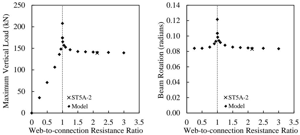
Figure 5.16. Parametric study: beam web tear-out resistance.
