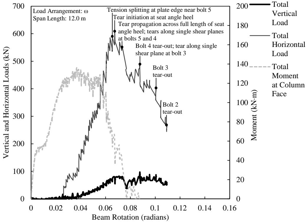
Figure D.39. Load versus rotation for ST5C-2.
