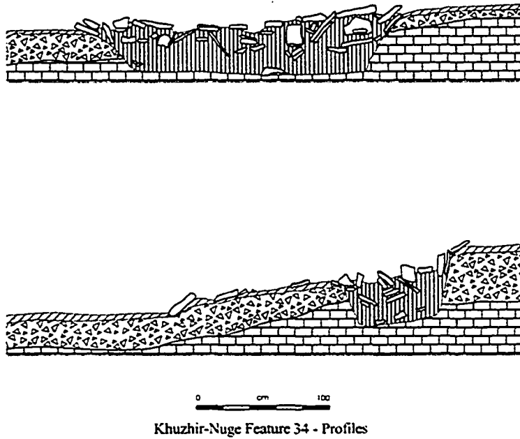
Figure 8. Cross and longitudinal section of Grave 34, Type B architecture.
