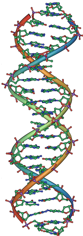
Figure 1.10 DNA structure
