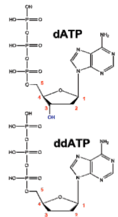
Figure 11.3 ddNTPs
