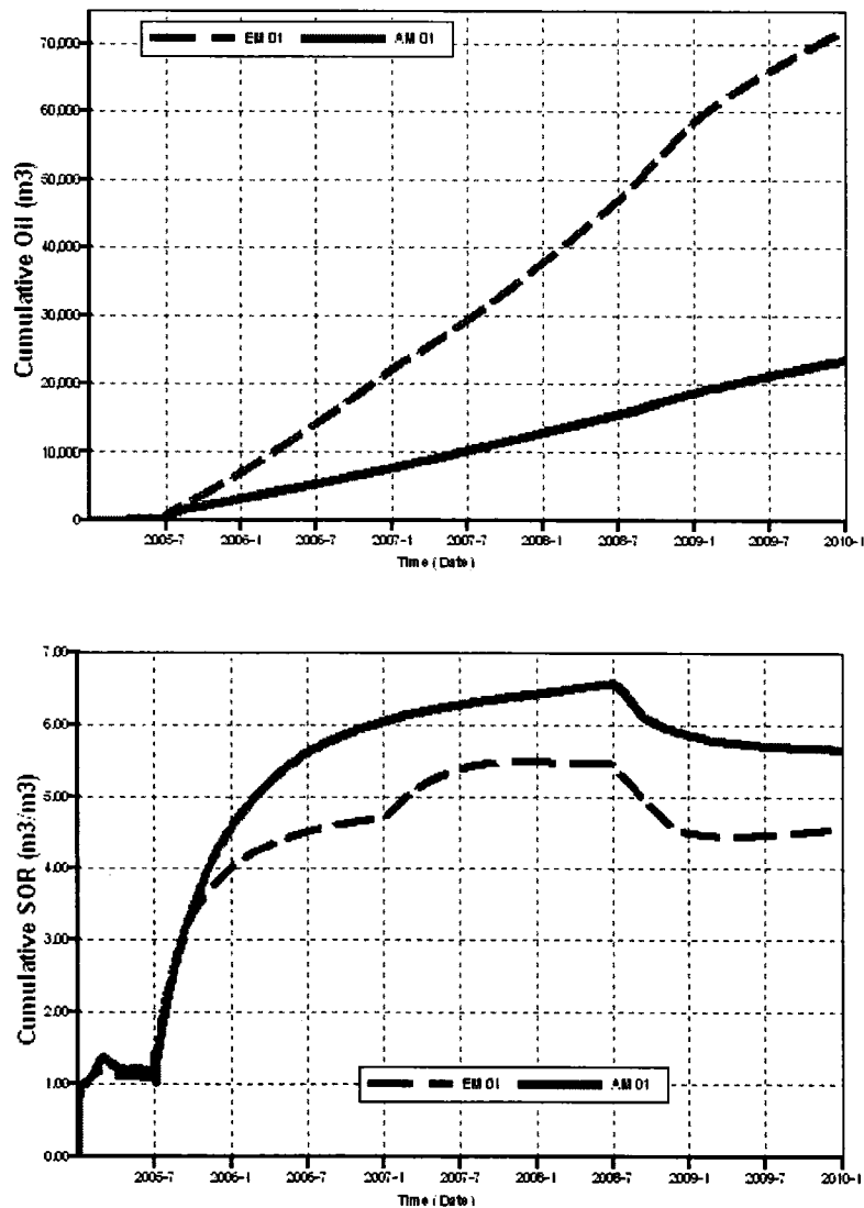
Figure 7-32: The results of flow simulation using the models generated by the two methods: the top plot is the cumulative oil production curves, and the bottom plot is the cumulative steam oil ratio (CSOR) curves. The gray solid line is for the approximate downscaling method, and the black dashed line is for the exact downscaling method.
