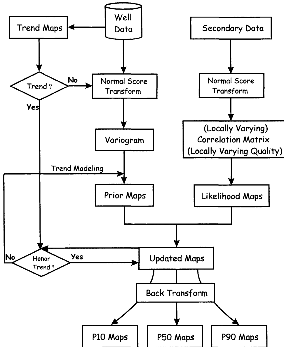
Figure 4-3: The work flow for Bayesian updating 2-D mapping techniques.
