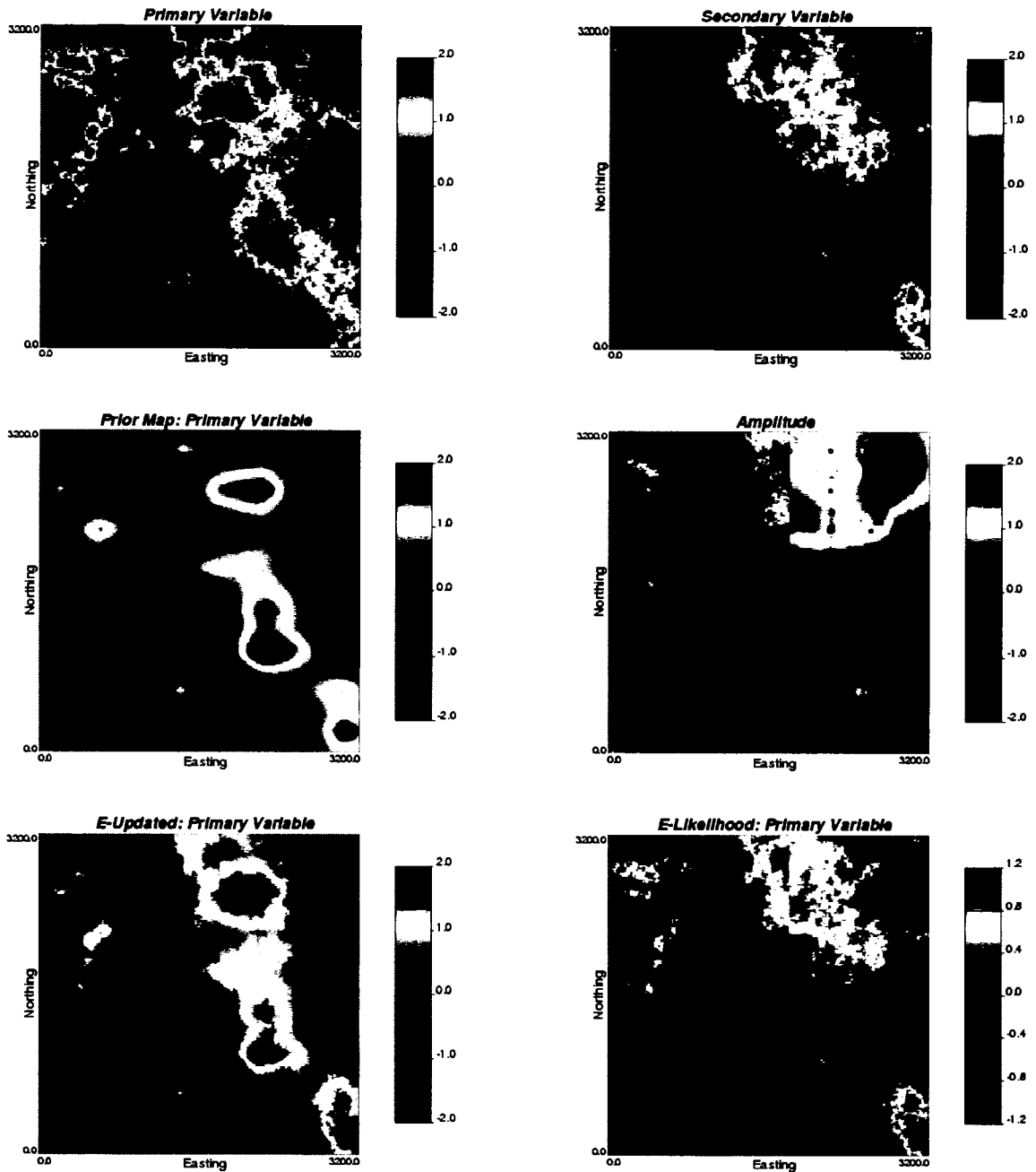
Figure 3-16: The results of enhanced Bayesian updating using LVC and LVQ.
