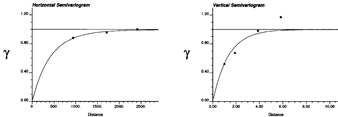
Figure 7-17: An omnidirectional horizontal variogram (left) and a vertical variogram (right).
