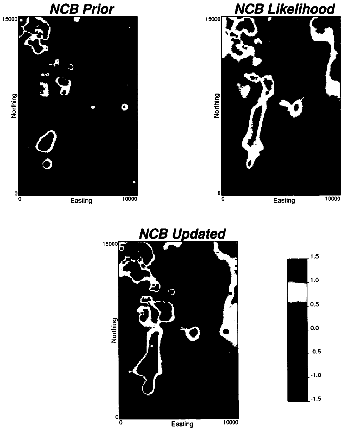
Figure 8-7: The prior (top left), likelihood (top right) and updated maps (bottom) of NCB in Gaussian units.
