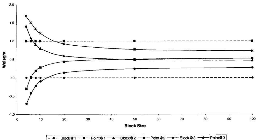
Figure 7-2: The weights of block and point data in the cells “1-3” with different block sizes. At the well location, the weights are constant (dash lines). Away from the well, the weights change with block size (solid lines).
