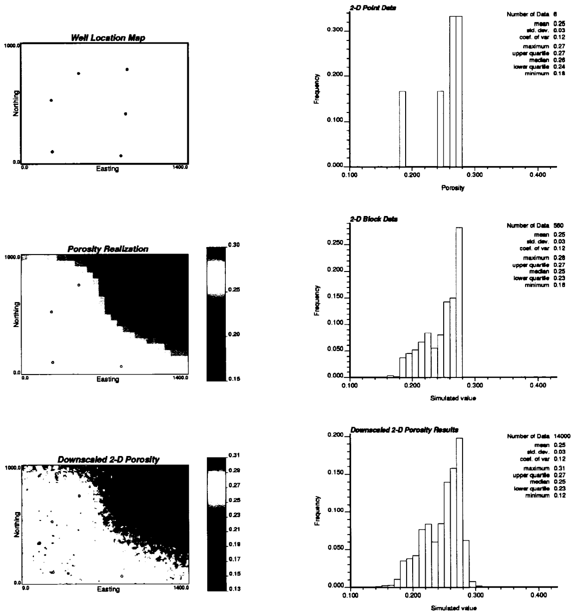
Figure 8-12: The Bayesian updating with P-Field simulation realization#1(middle left) is exact downscaled from 50m by 50m to 10m by 10m (bottom left). The histograms of point data (top right), block data (middle right), and downscaled values are shown on the right.
