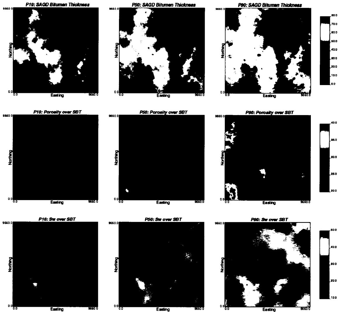
Figure 4-16: The P_{10}/P_{50}/P_{90} maps of SBT in meters (top), porosity (middle) and water saturation (bottom) are in percentage.
