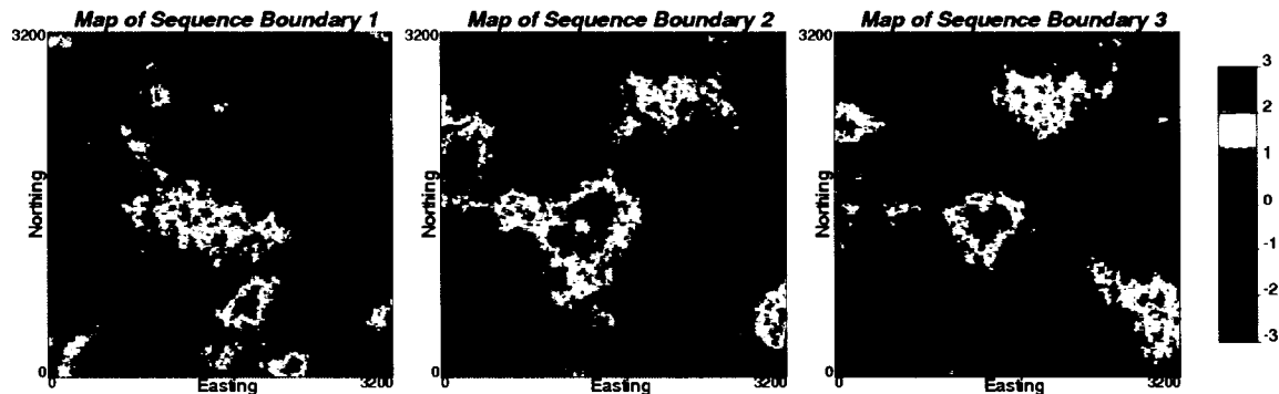
Figure 5-4: Maps of three secondary variables in Gaussian unit: sequence boundary 1 (left), sequence boundary 2 (centre) and sequence boundary 3 (right).
