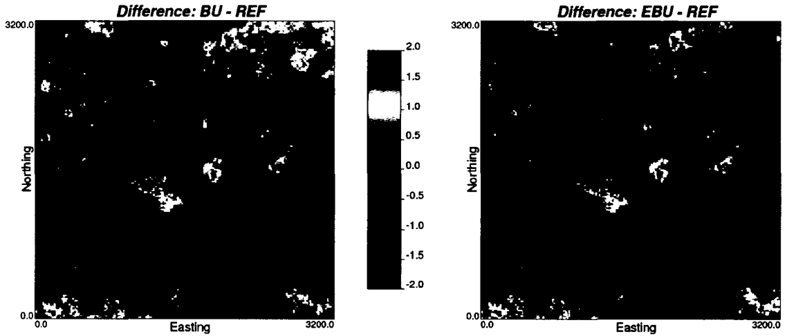
Figure 3-17: The maps of the difference between the Bayesian updating (BU) results and the reference (left) and the difference between the enhanced Bayesian updating (EBU) results and the reference (right).
