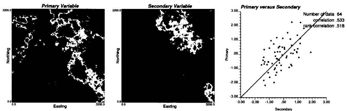
Figure 3-5: The maps of primary (left) and secondary (middle) variables and their cross plot (right) which indicates a global correlation coefficient of 0.533.
