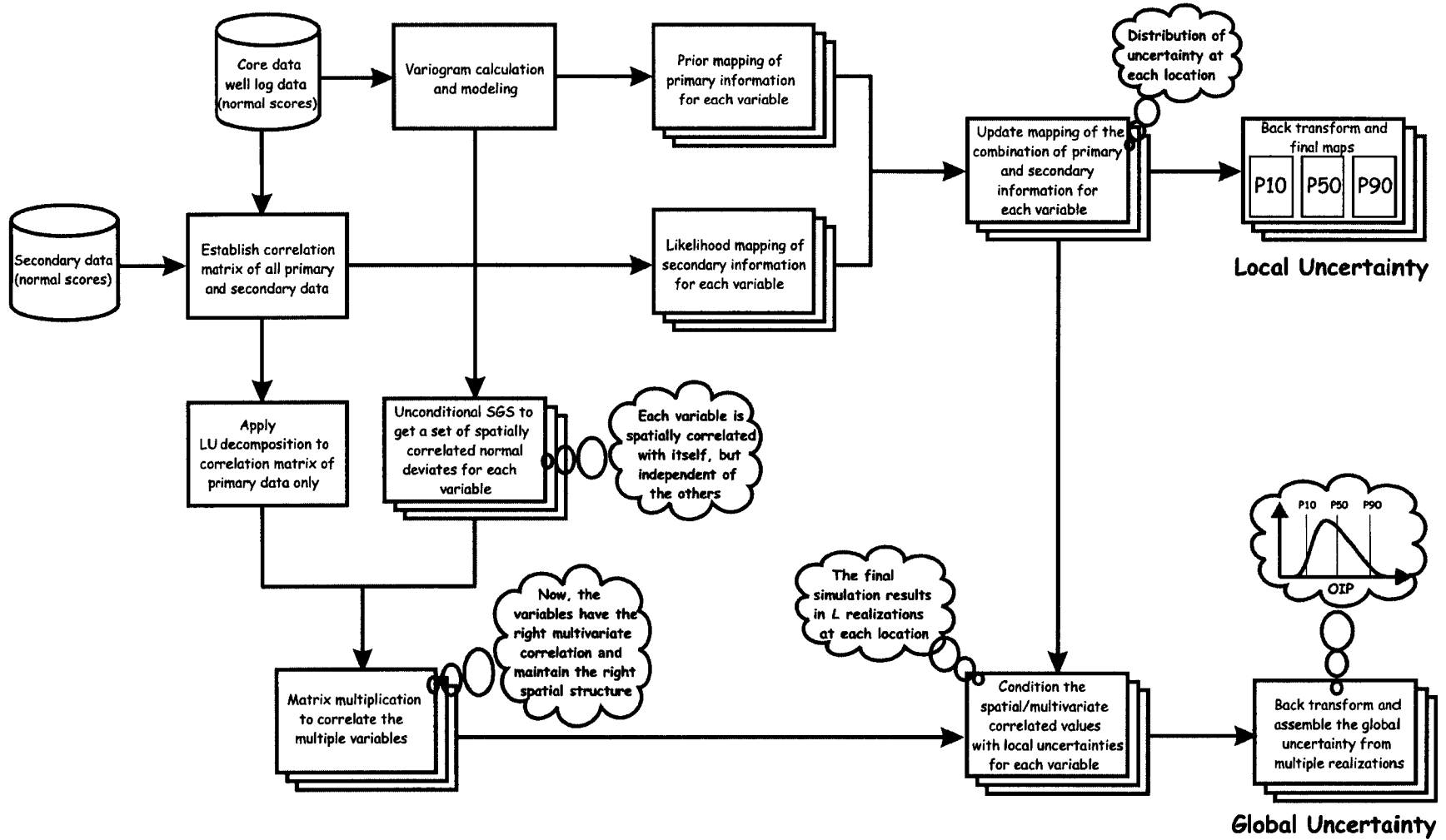
Figure 5-2: Work flow of the spatial/multivariate simulation approach for assessment of global uncertainty from local uncertainty.
