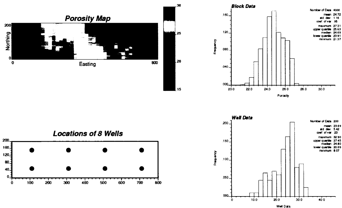
Figure 7-26: The porosity block data (top) and well data (bottom) used for downscaling. The porosity is in percentage.
