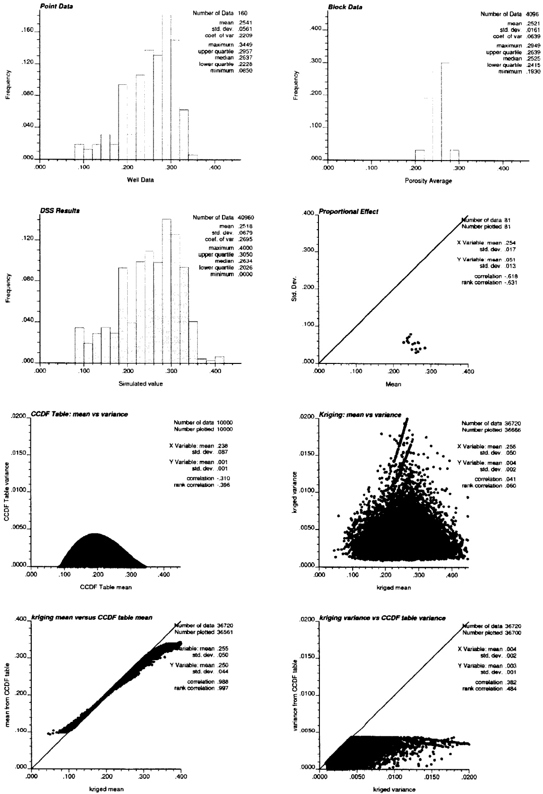
Figure 7-14: The CCDF lookup-table method results with a global distribution (top row). The proportional effect is not clear (second right). The CCDF table of means and variances does not cover all the kriging mean and variances (third row). The results of matching means and variances are shown in the bottom row.
