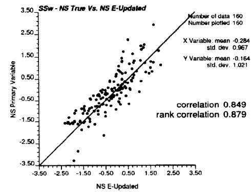
Figure 4-22: The cross validation of enhanced Bayesian updating results for water saturation in Gaussian units.
