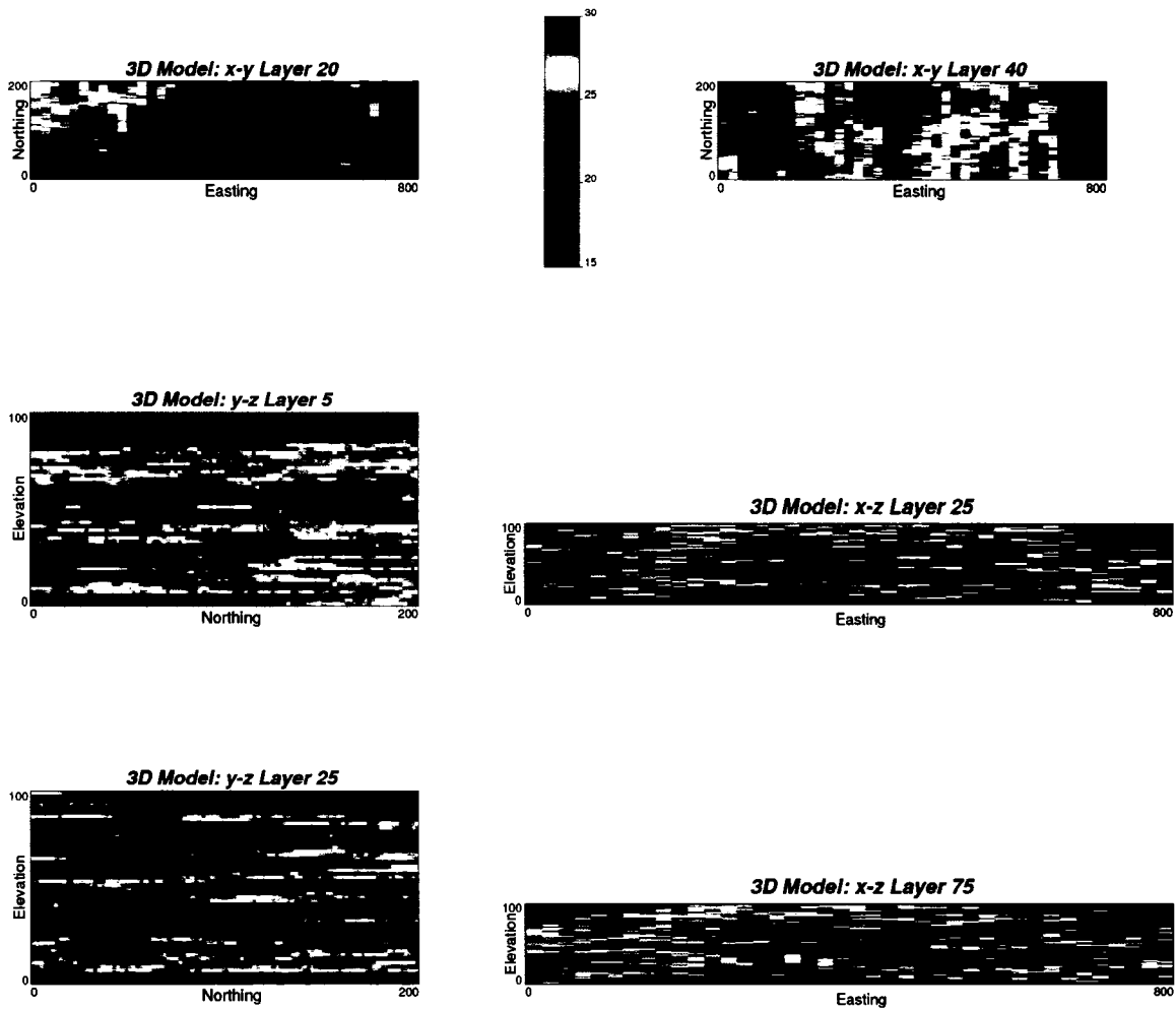
Figure 7-27: The exact downscaling results: 3-D porosity model in plane view (first row), y-z (left) and x-z (right) cross sections. The porosity is in percentage.
