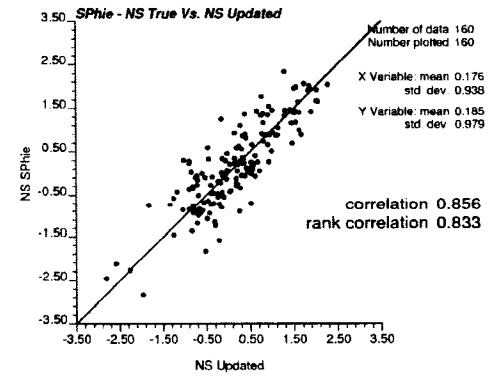
Figure 4-18: The cross validation of Bayesian updating results for porosity in Gaussian units.
