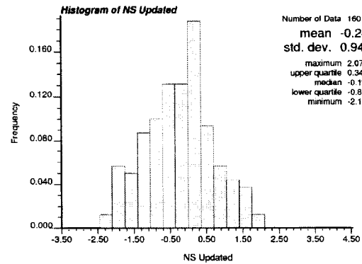
Figure 4-19: The cross validation of Bayesian updating results for water saturation in Gaussian units.
