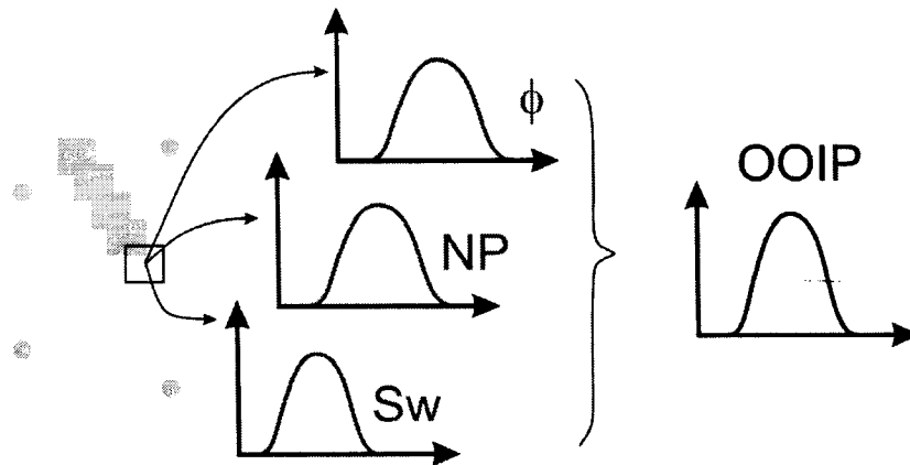
Figure 5-1: A schematic illustration of joint uncertainty of OOIP from local uncertainty models of constituent variables. The square with black line is the estimated location.
