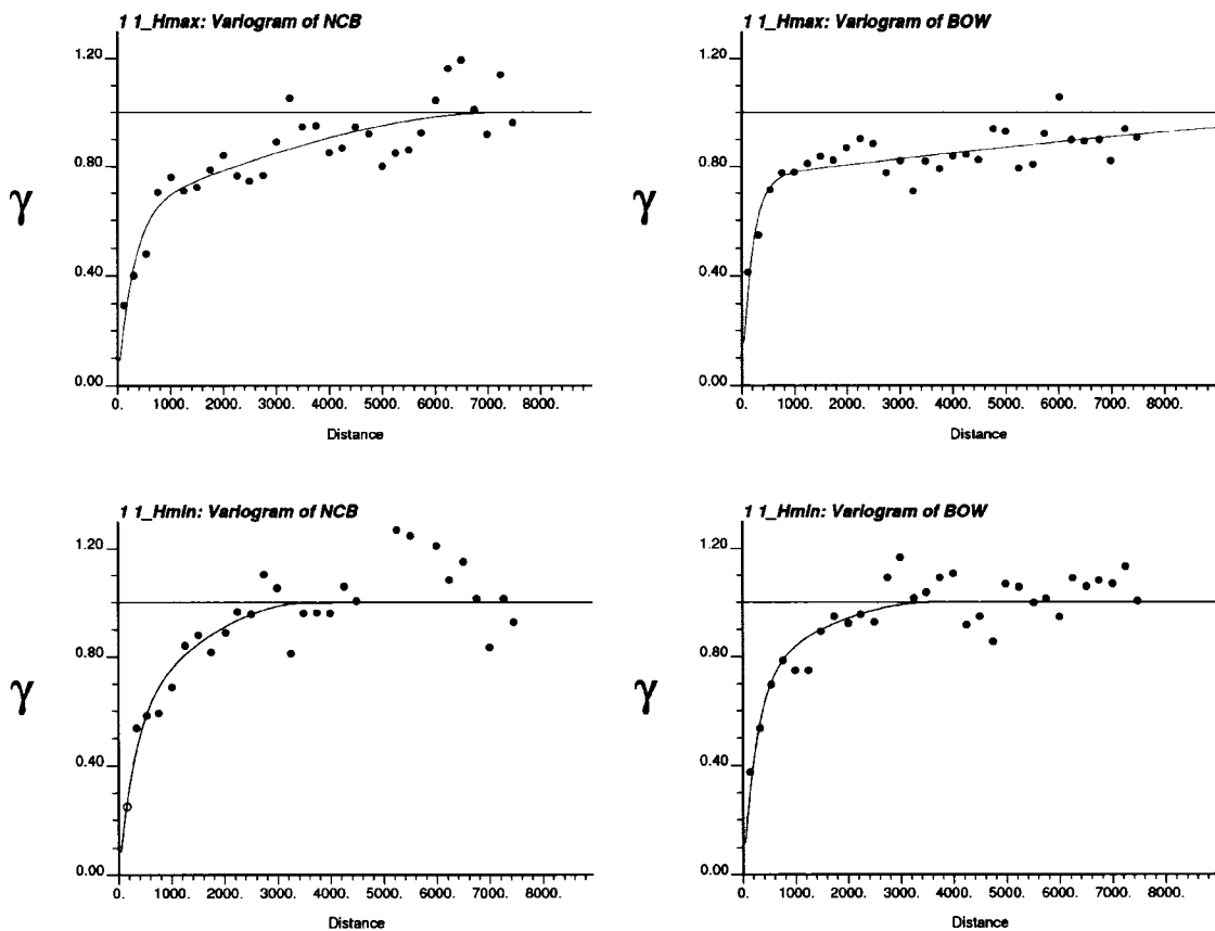
Figure 8-4: Directional variograms and fitted models for NCB (left) and BOW (right).
