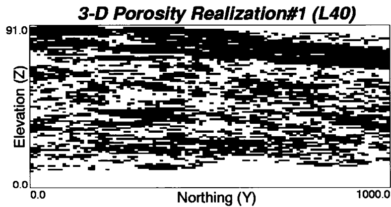
Figure 8-15: The 3-D porosity realization #1. The model has a grid resolution of 10 x 10m areally and 1m vertically. The field spans 1,400m, 1,000m and 91m in the Easting, Northing and Elevation directions, respectively. The vertical direction is exaggerated by 5 times.
