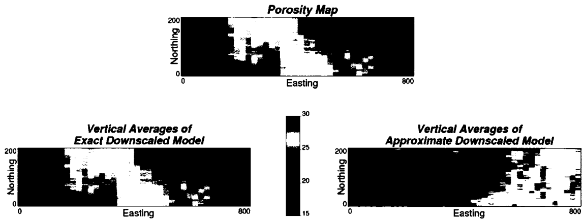
Figure 7-29: The map of original porosity block data (top), the map of vertically averaged porosity from the exact downscaled 3-D model (left) and the map of vertically averaged porosity from the approximate downscaled 3-D model (right). The porosity is in percentage.
