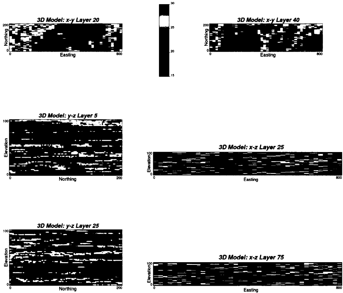
Figure 7-28: The approximate downscaling results in plane view (first row), y-z (left) and x-z (right) cross sections. The porosity is in percentage.
