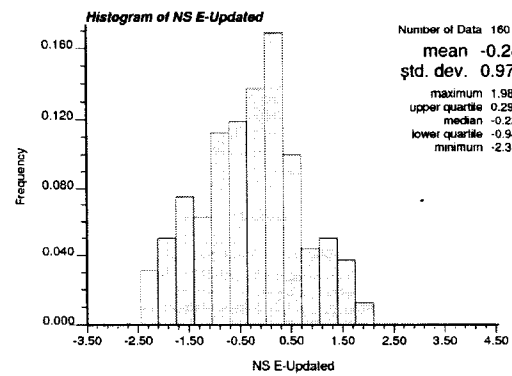
Figure 4-22: The cross validation of enhanced Bayesian updating results for water saturation in Gaussian units.
