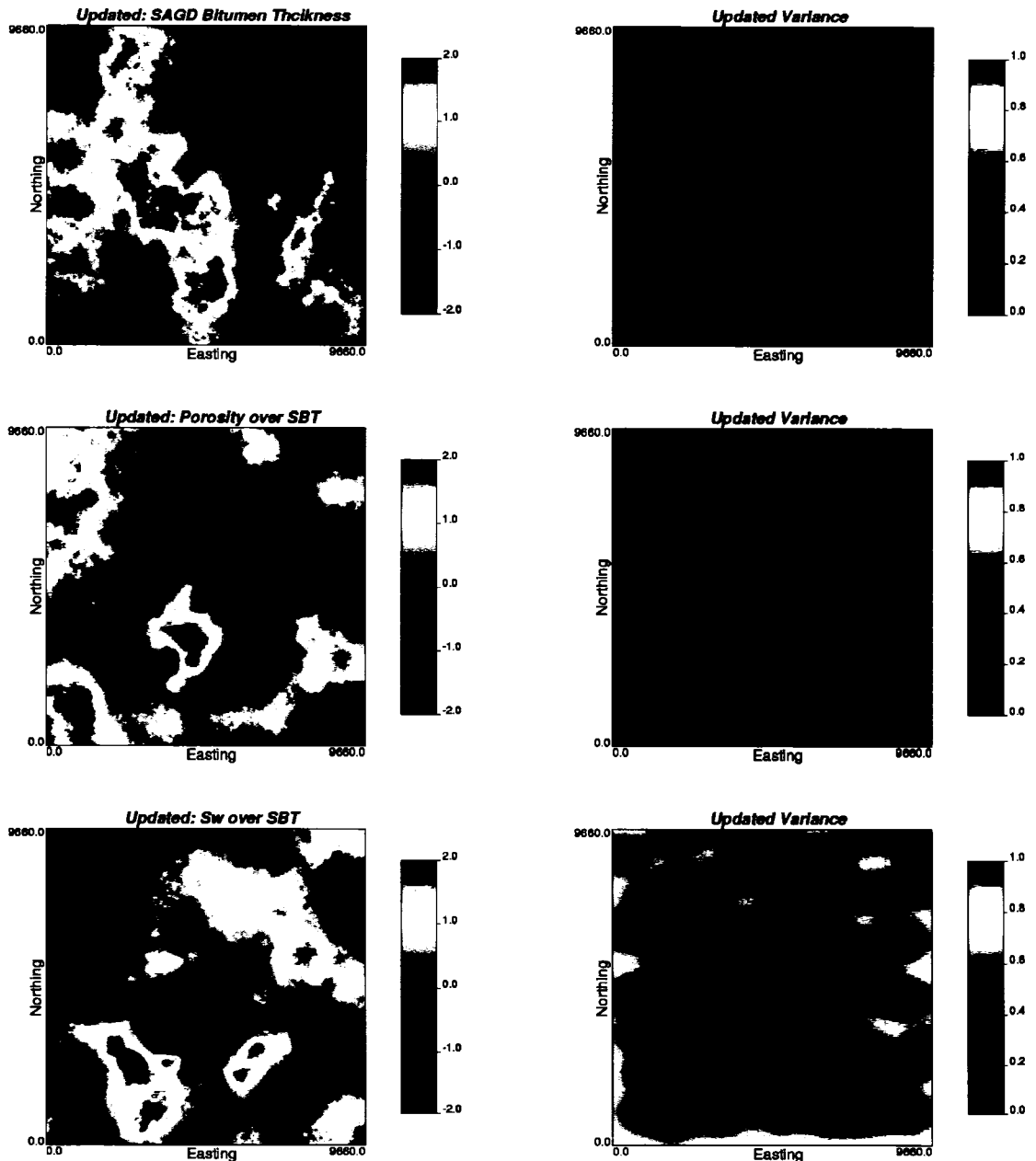
Figure 4-14: The updated maps of the primary variables from Bayesian updating method. The left column is updated mean in Gaussian units and the right column is updated variance.
