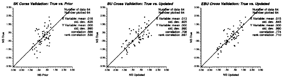
Figure 3-18: The cross validation of simple kriging (left), Bayesian updating (middle) and enhanced Bayesian updating (right).
