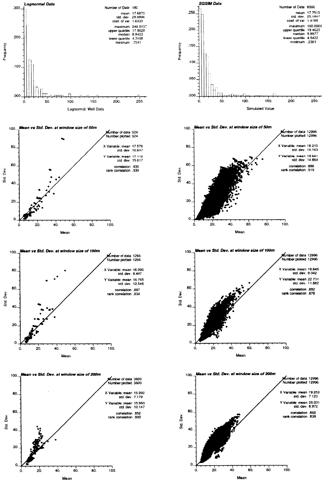
Figure 7-11: The proportional effect shown at different moving window sizes (50m, 100m and 200m). The two sets of data are used (the first row): a set of well data (left) and the sgsim realization using the well data (right). The correlations are different with different window sizes.
