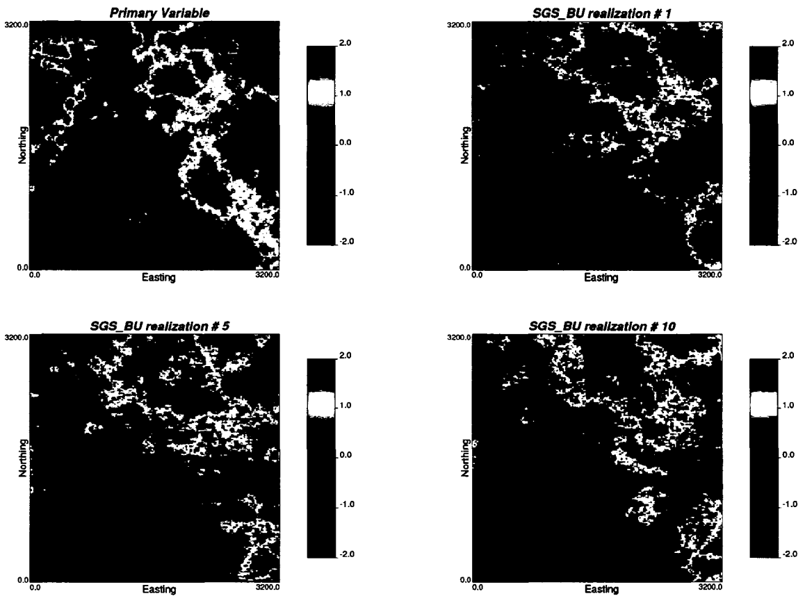
Figure 3-22: The primary variable (reference, up-left) and the SGS with Bayesian updating simulation realizations.
