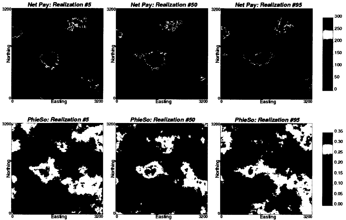
Figure 5-9: Realizations 5, 50 and 95 of the spatial/multivariate simulation. In each realization, all values are spatially correlated over the model area and the Net Pay thickness in meters (top row) and \phi S_o in fraction (bottom row) are also correlated.
