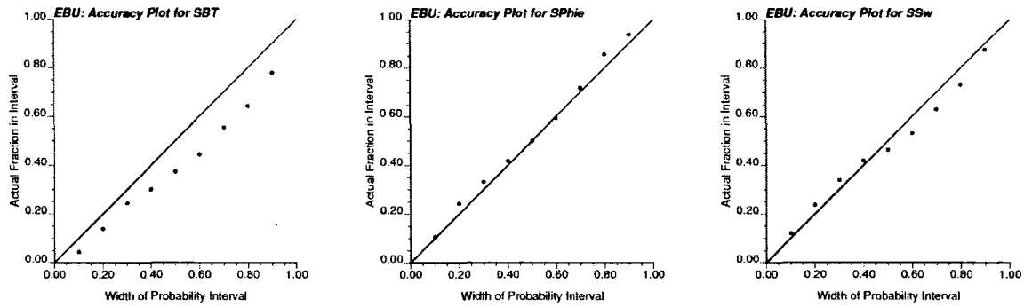
Figure 4-24: The accuracy plots of the SBT (left), porosity (middle) and water saturation (right) from enhanced Bayesian updating method.
