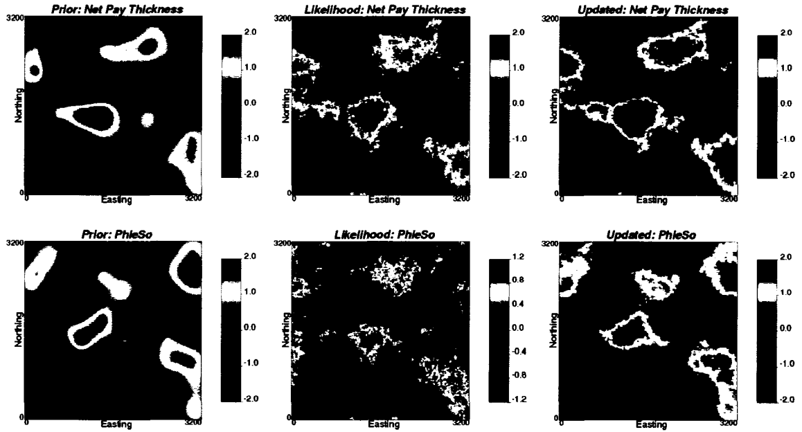
Figure 5-6: Prior (left), likelihood (centre) and updated (right) maps for NP (top) and \phi S_o (bottom) in Gaussian unit.
