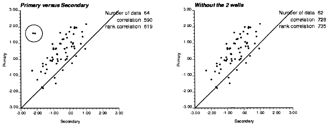
Figure 3-4: Cross plot of two variables with two outliers in the blue circle gives a correlation of 0.590 (left). And cross plot of two variables without the two outliers gives a correlation of 0.728 (right).
