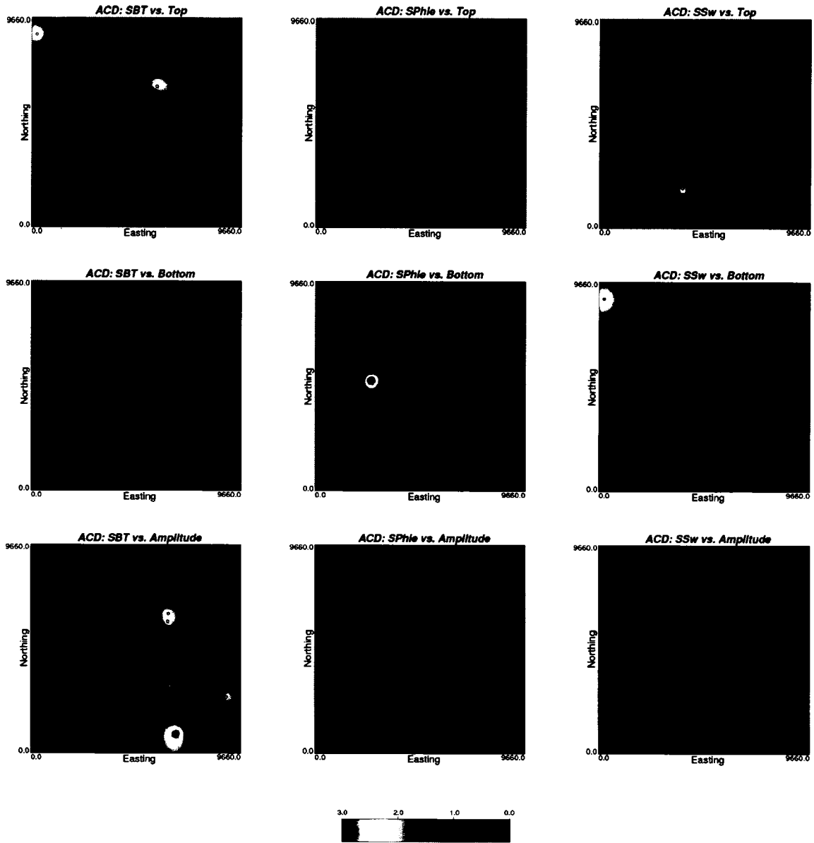
Figure 4-9: The ACD maps of each pair of variables.
