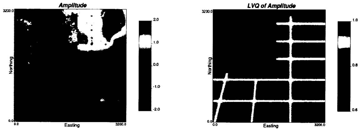
Figure 3-13: The map of amplitude and its local varying quality (LVQ). The upper-left area is the 3-D seismic area, and the rest of the area is modeled by kriging using 2-D seismic lines.
