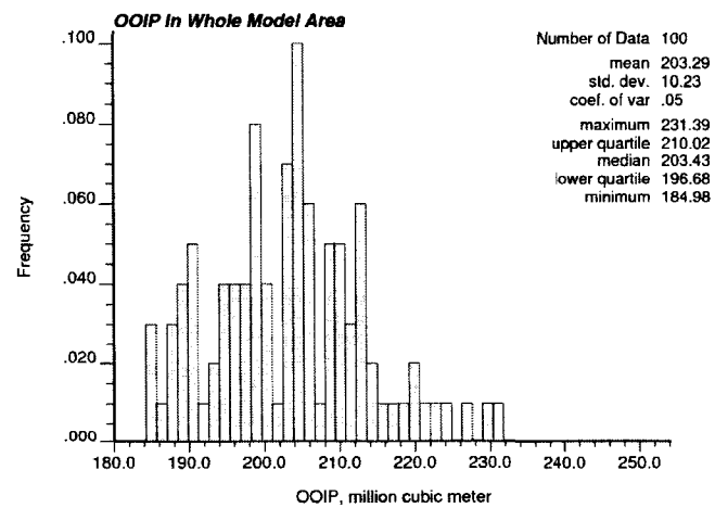
Figure 5-11: Global uncertainty distribution of the OOIP in the Area 1 (left), the Area 2 (centre), and the Whole Model Area (right).
