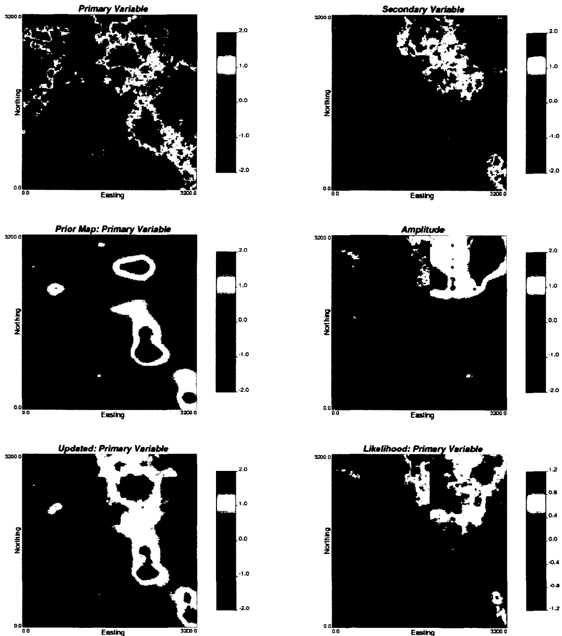
Figure 3-15: The results of Bayesian updating using global correlation coefficients.
