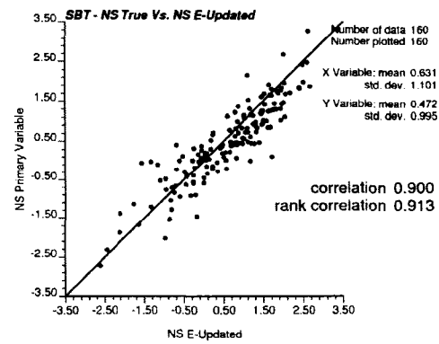
Figure 4-20: The cross validation of enhanced Bayesian updating results for SBT in Gaussian units.
