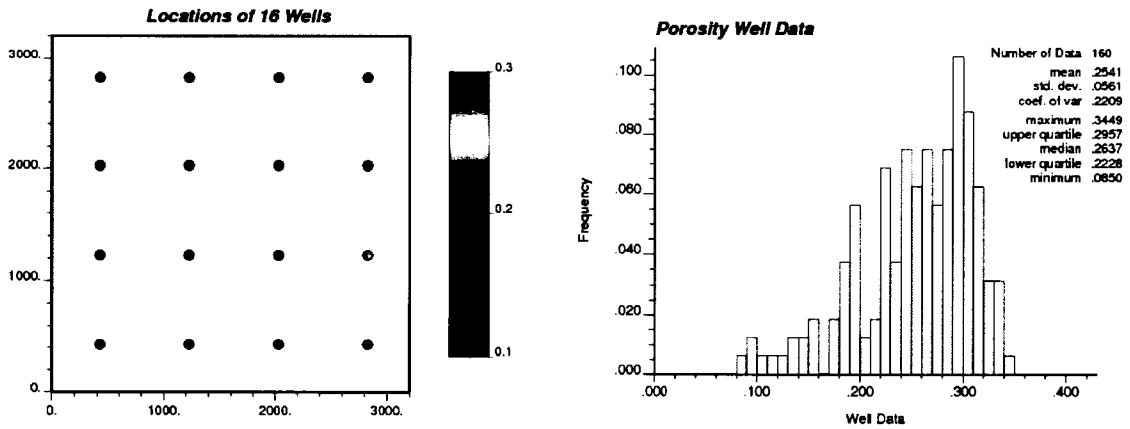
Figure 7-16: The location map of the 16 wells with the color scale showing porosity in fraction and the histogram of the well log porosity in the right.
