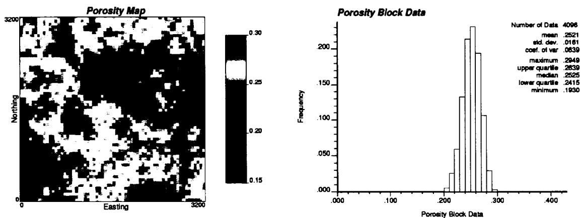
Figure 7-15: 2-D map of porosity block data at a scale of 50m x 50m x 10 m.
