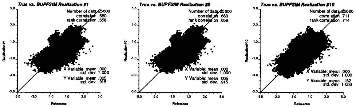
Figure 3-21: The cross plots of the reference versus the P-field simulation realizations #1, #5 and #10.
