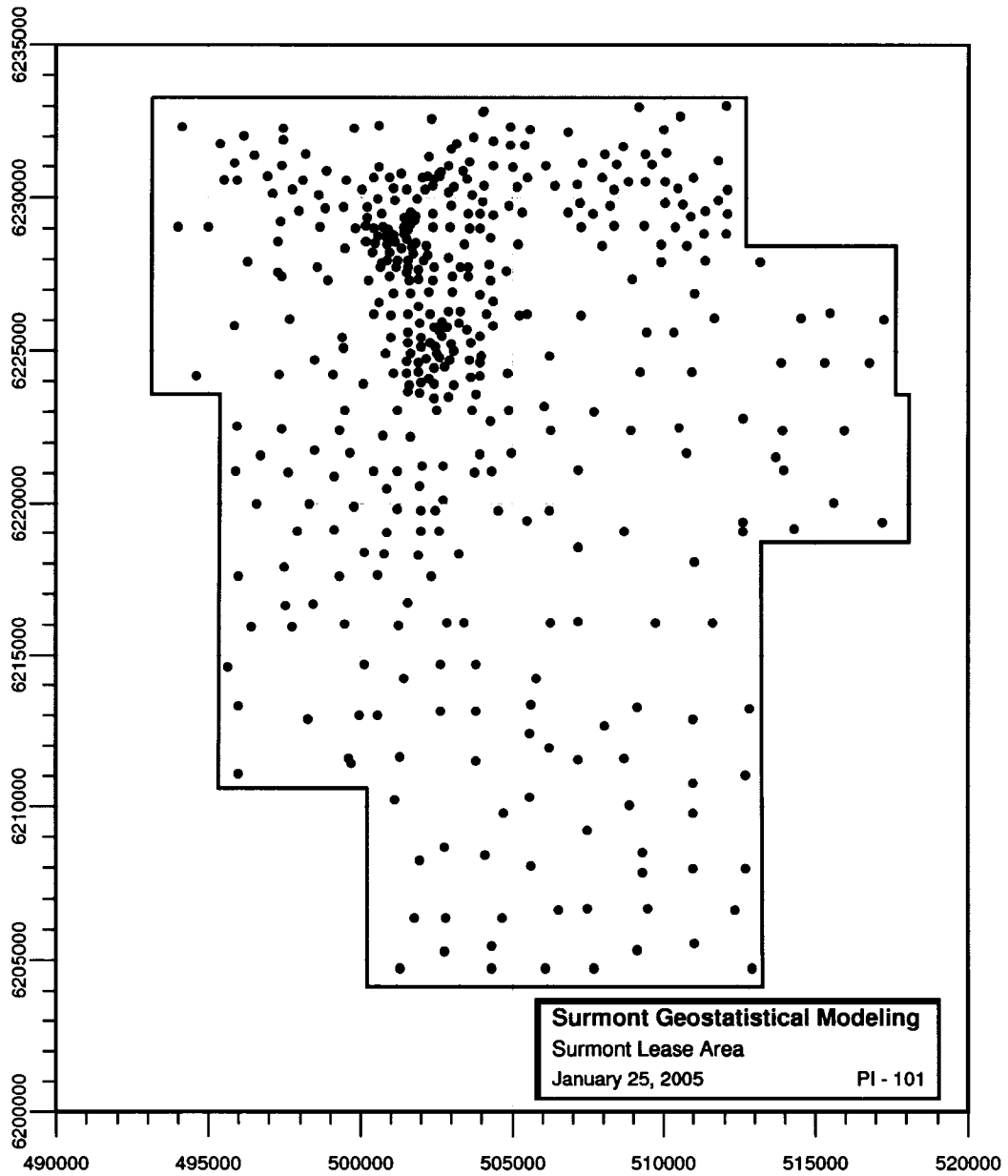
Figure 8-2: The Surmont lease map with delineation well locations, the map units are in meters.
