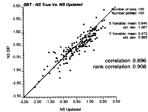
Figure 4-17: The cross validation of Bayesian updating results for SBT in Gaussian units.
