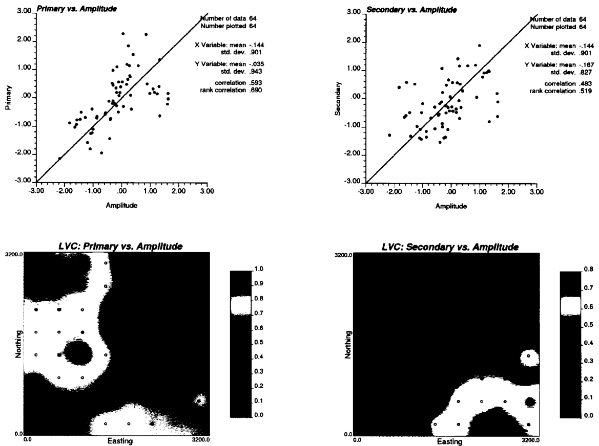
Figure 3-14: The global correlation and the map of locally varying correlation (LVC) between primary and amplitude (left column) and between secondary and amplitude (right column).
