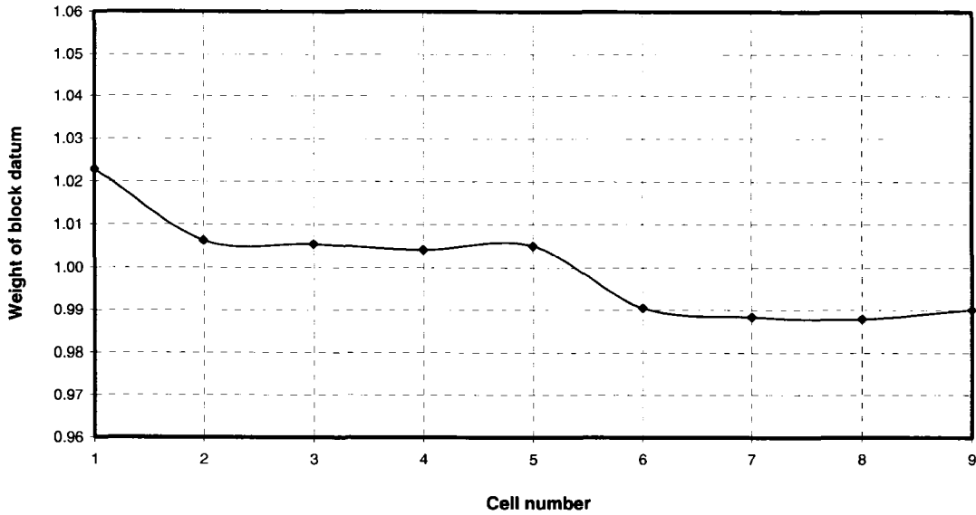
Figure 7-4: The weight of collocated block in each small cell in case 1.
