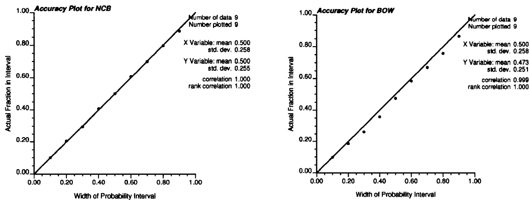
Figure 8-10: The accuracy plots of cross validation results for NCB and BOW.
