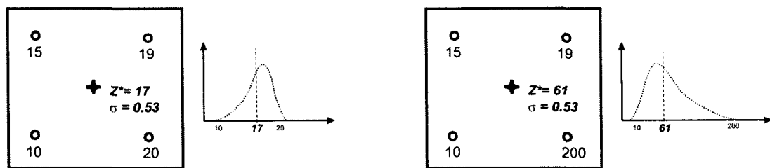
Figure 7-12: The local distribution and variance are affected by the data values.
