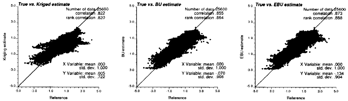
Figure 3-19: The cross plots of the estimates versus the reference for simple kriging (left), Bayesian updating (middle), and the enhanced Bayesian updating (right).
