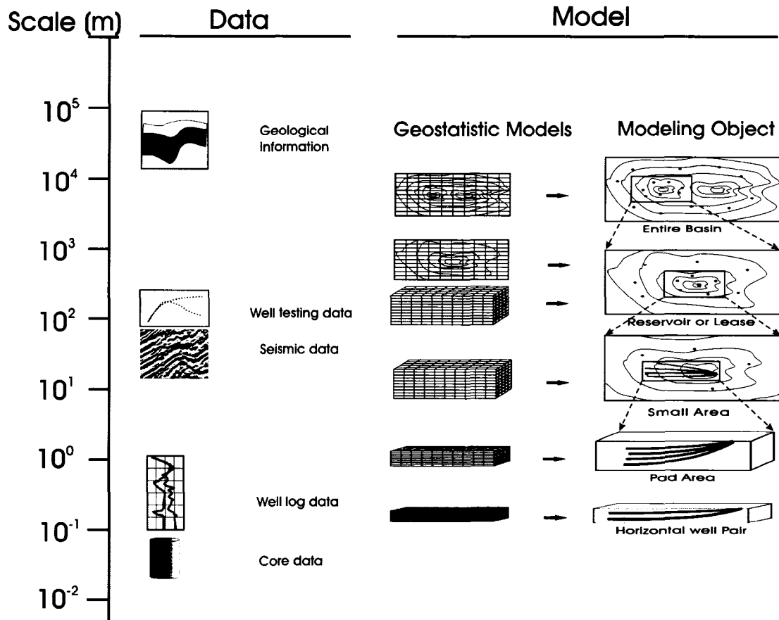
Figure 1-1: Schematic illustrations of the data and model scales for reservoir modeling. The modeling objects are taken from a heavy oil scenario in Northern Alberta.
