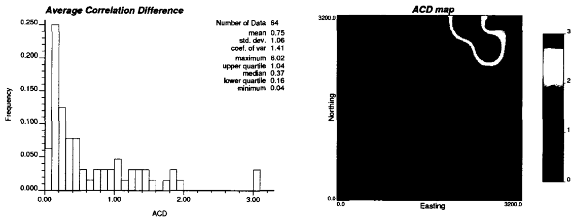
Figure 3-11: The histogram and kriged map of ACD for the two variables shown in Figure 3-8. The two wells are the two outliers shown in the cross plot in Figure 3-4.
