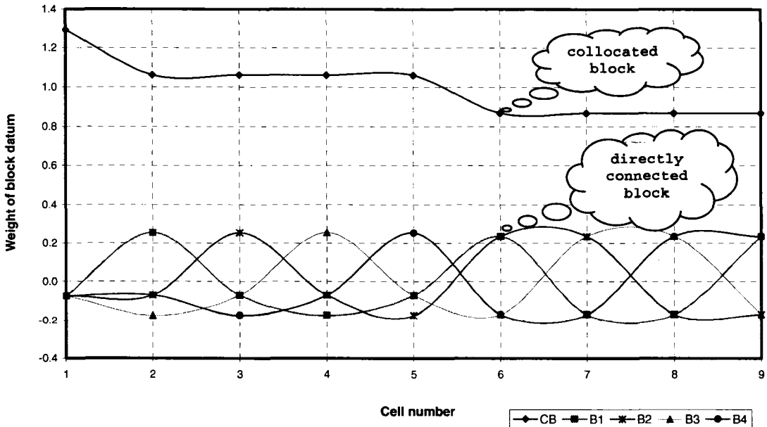
Figure 7-5: The weights of blocks in each small cell in case 2.
