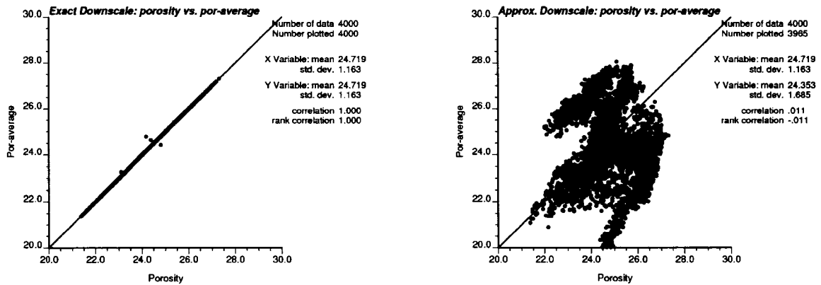
Figure 7-30: The cross plots of porosity block data vs. block average of fine scale model for the exact downscaling method (left) and the approximate downscaling method (right)
