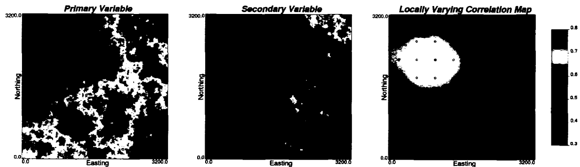
Figure 3-8: The maps of two variables (left and middle) and their locally varying correlation (right) for the case of two pairs of extreme values shown in Figure 3-4.
