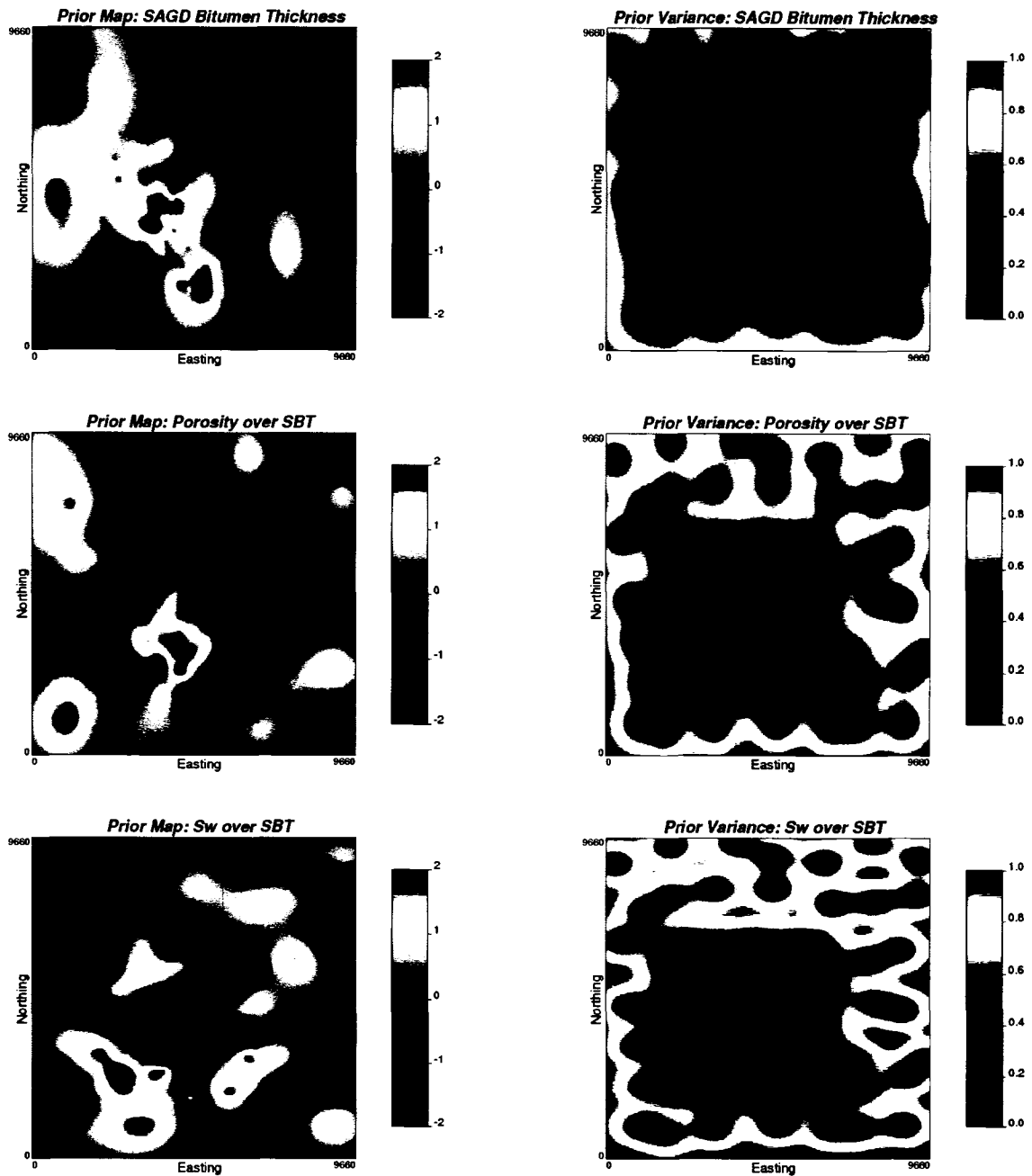
Figure 4-7: The prior maps of the primary variables. The left column is prior mean in Gaussian units and the right column is prior variance.
