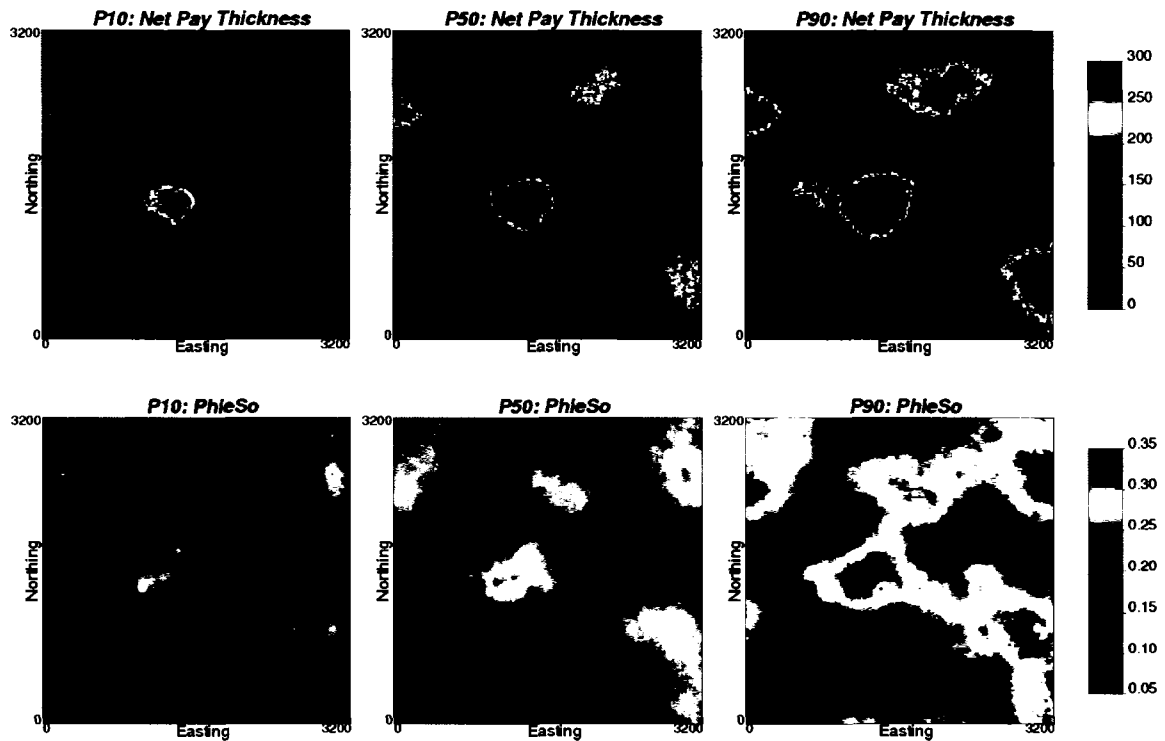
Figure 5-7: Final maps of uncertainty for Net Pay thickness in meters (top row) and \phi S_o in fraction (bottom row): P10 (left), P50 (centre) and P90 (right). Note the east-west section lines in the Net Pay thickness final maps are plotted in Figure 5-8, and the black circles represent well locations.
