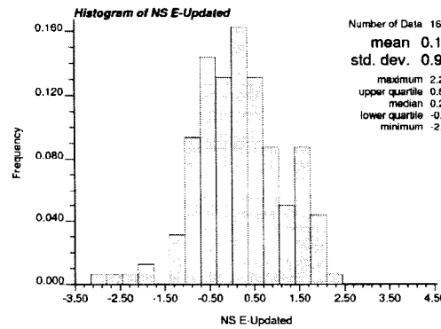
Figure 4-21: The cross validation of enhanced Bayesian updating results for porosity in Gaussian units.
