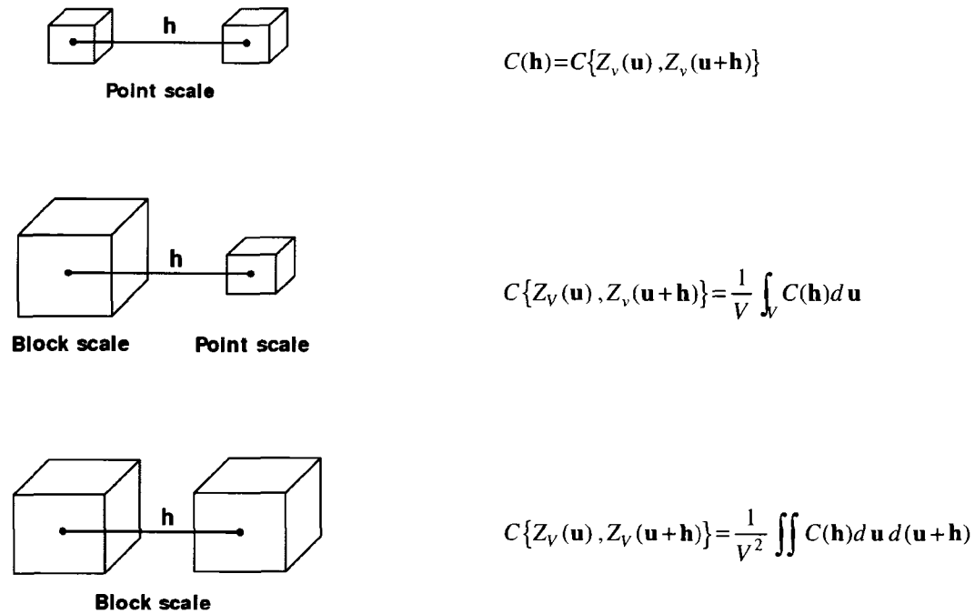
Figure 2-3: The volume averaged covariance models, where v is for the point scale volume and V is for the block scale volume.
