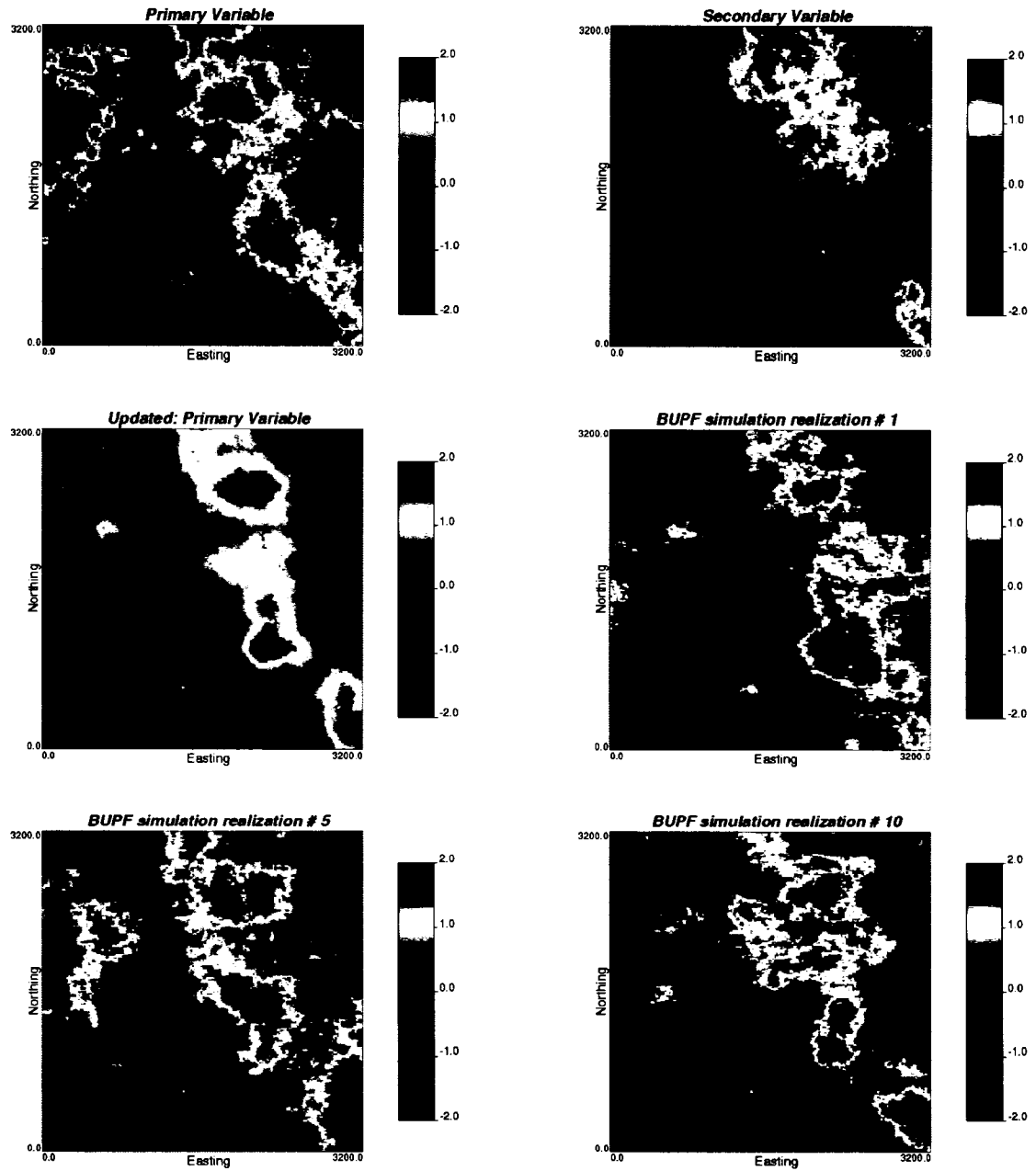
Figure 3-20: The primary variable (reference) and secondary variable used for Bayesian updating are in the top row. The Bayesian updated estimates and P-field simulation realizations are shown in the middle and bottom rows.
