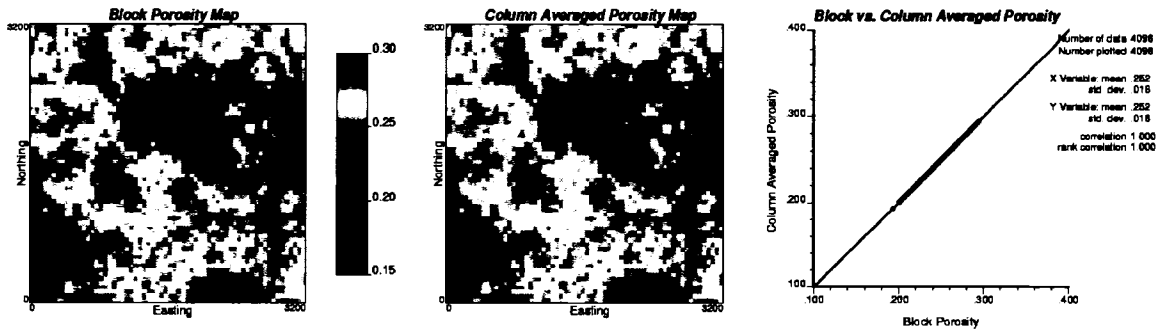
Figure 7-24: The block 2-D porosity map (left), the map of the column averaged porosity from the 3D model (middle), and the cross plot of the two grids (right) indicates the exactness. The porosity is in fraction.
