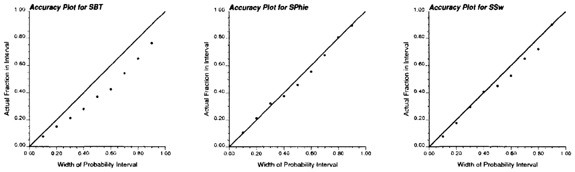
Figure 4-23: The accuracy plots of the SBT (left), porosity (middle) and water saturation (right) from Bayesian updating method.
