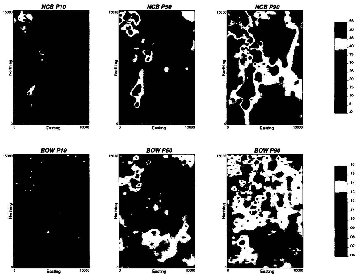
Figure 8-9: Maps summarizing uncertainty in NCB in meters (top row) and BOW in fraction (bottom row). The P10 low values are shown on the left, the P50 values are shown in the middle and the P90 high values are shown on the right.
