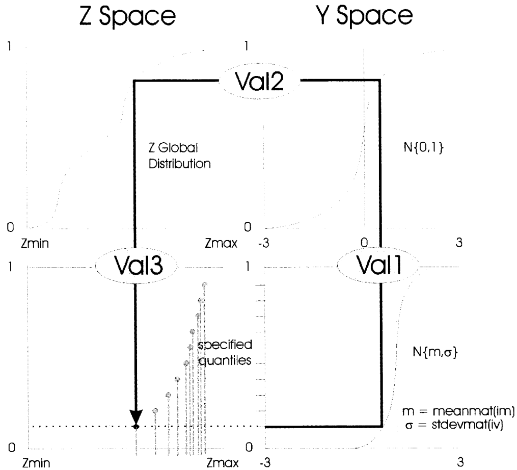
Figure 7-10: The graphical representation of the transformations applied to calculate the local distributions of uncertainty. The illustrated transformation is repeated for a sufficient number of quantiles to describe the local distribution (from Pyrcz and Deutsch, 2003).
