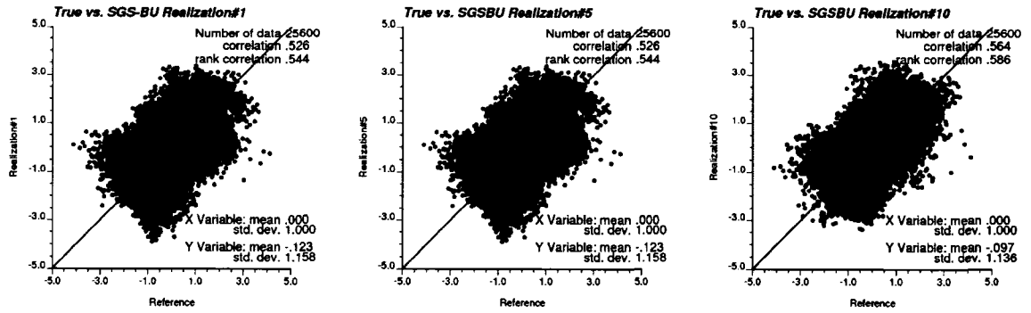
Figure 3-23: The cross plots of the reference versus the SGS with Bayesian updating simulation realizations #1, #5 and #10.
