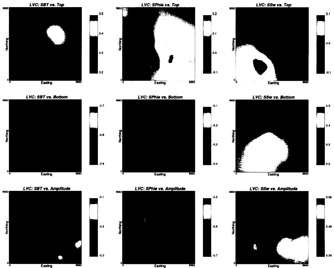
Figure 4-11: The locally varying correlations between primary variables and secondary variables.
