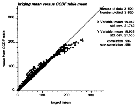
Figure 7-13: The CCDF lookup-table method results with a lognormal global distribution (top). The proportional effect is accounted in the DSS (second row). The CCDF table of means and variances does not cover all the kriging mean and variances (third row). The results of matching mean and variance are shown in bottom row.
