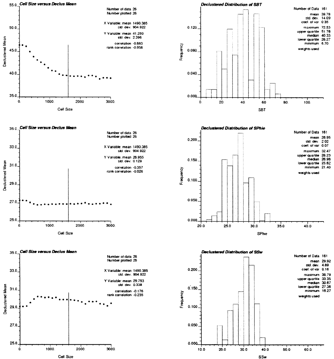
Figure 4-5: The declustering results of the three primary variables. The left column shows the declustered mean at different cell size range from 0 to 3000m. The red lines are the selected cell size at 1610m. The right column is the declustered distributions of the primary variables: the SAGD Bitumen Thickness (SBT) is in meters, and the porosity and Sw are in percentage.
