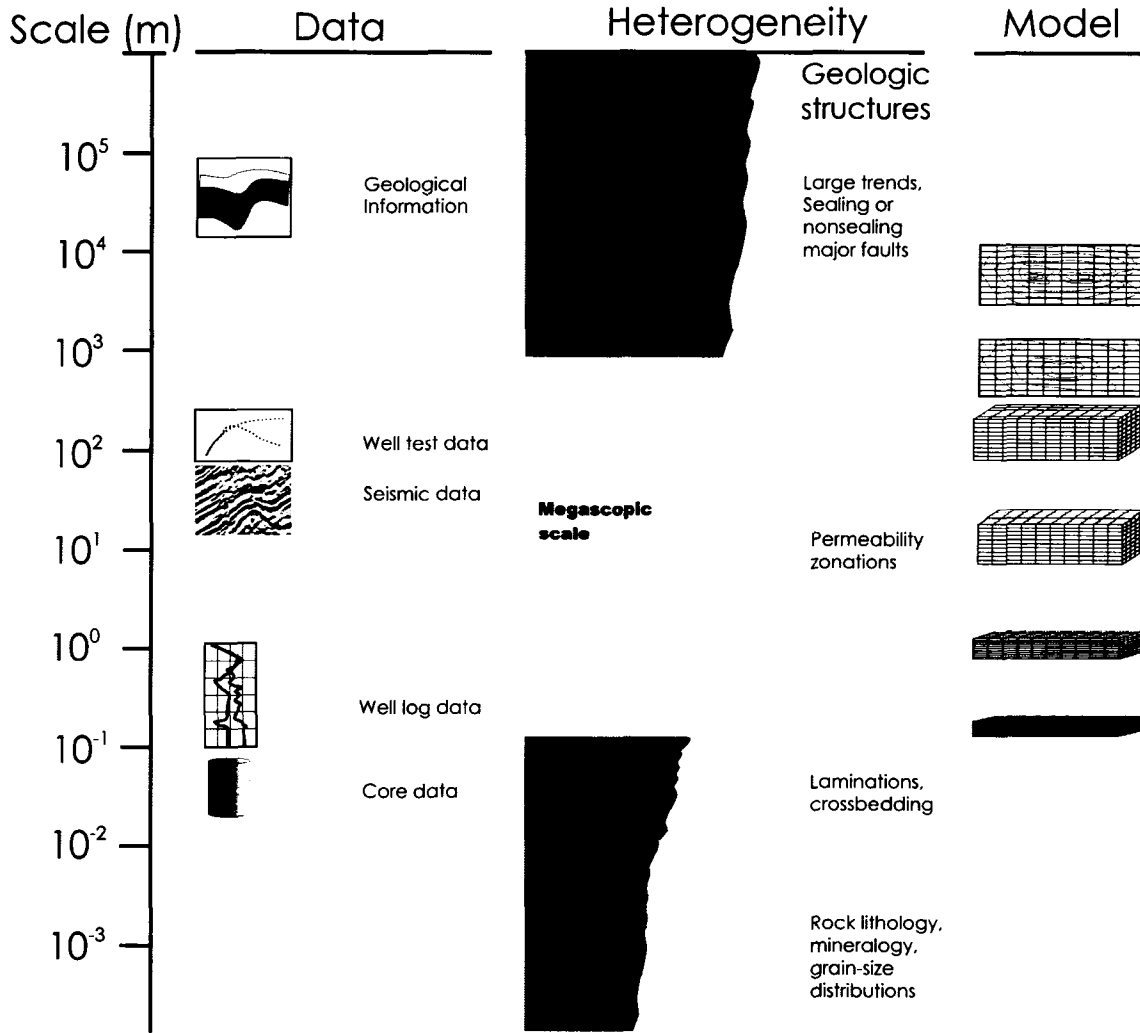
Figure 2-2: Schematic illustration of the scales of data, heterogeneity and model. The data and model scales are same as in Figure 1-1; they are related to the heterogeneity in the middle column.
