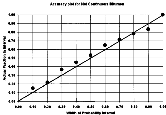
Figure 8-11: Accuracy plot of 2-D model validating with new wells of 2004.
