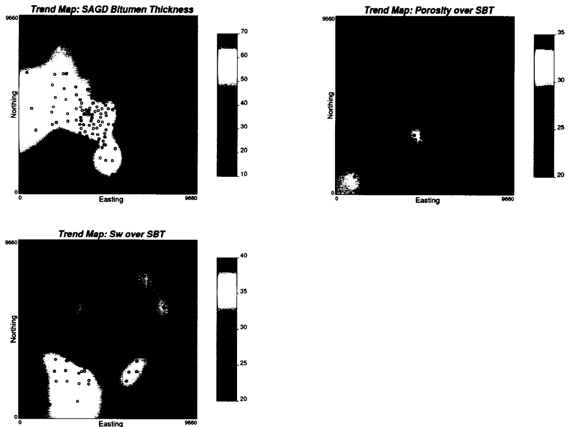
Figure 4-4: The trend maps of the primary variables: the SAGD Bitumen Thickness (SBT) is in meters, and the porosity and Sw are in percentage.
