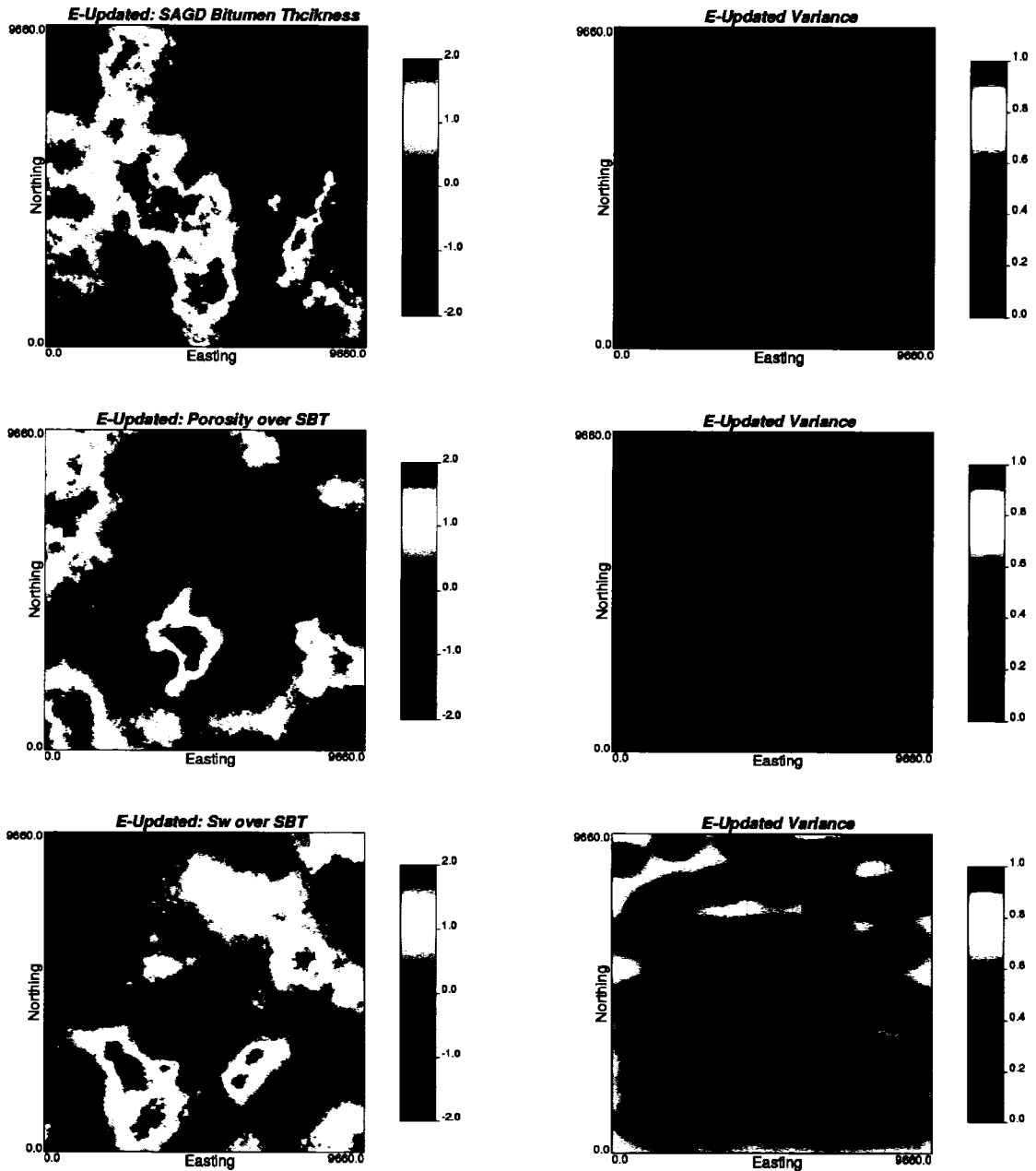
Figure 4-15: The updated maps of the primary variables from enhanced Bayesian updating method. The left column is updated mean in Gaussian units and the right column is updated variance.
