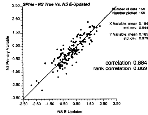
Figure 4-21: The cross validation of enhanced Bayesian updating results for porosity in Gaussian units.
