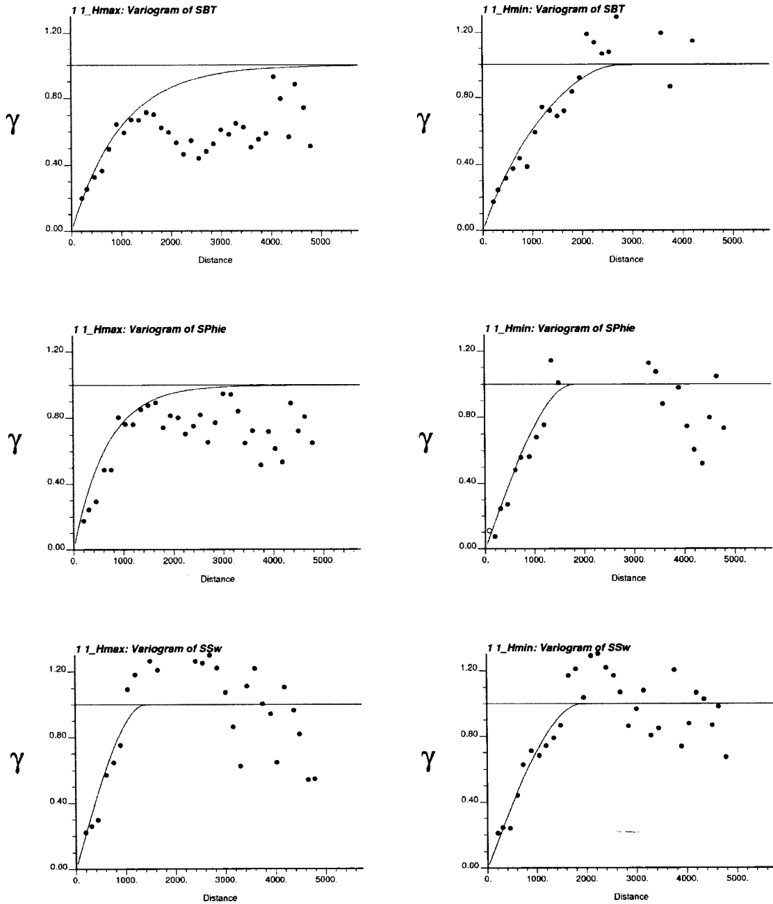
Figure 4-6: The major and minor principal directional variograms of SBT (top), porosity (middle) and water saturation (bottom).
