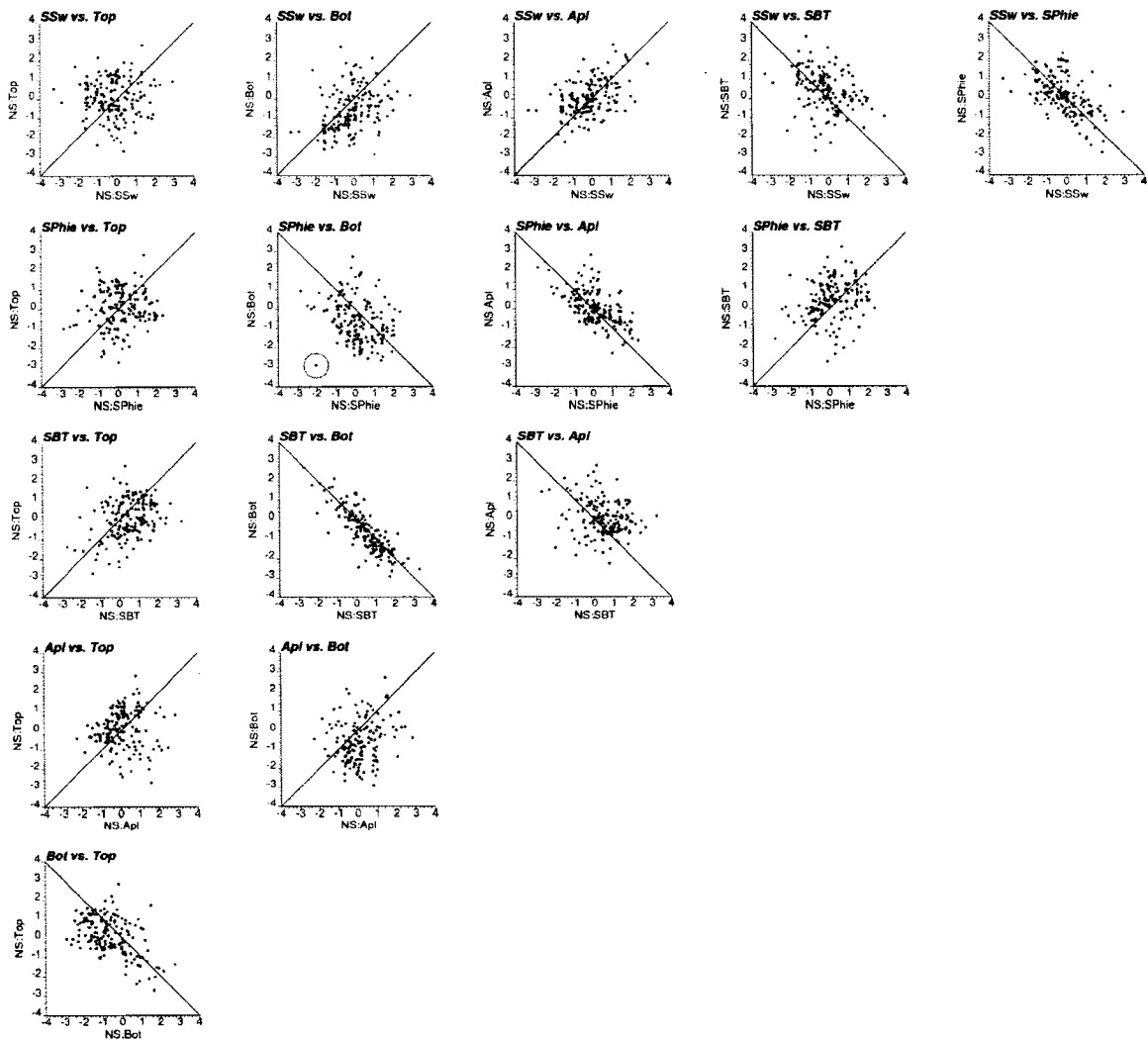
Figure 4-8: The cross plots of each pair of variables.
