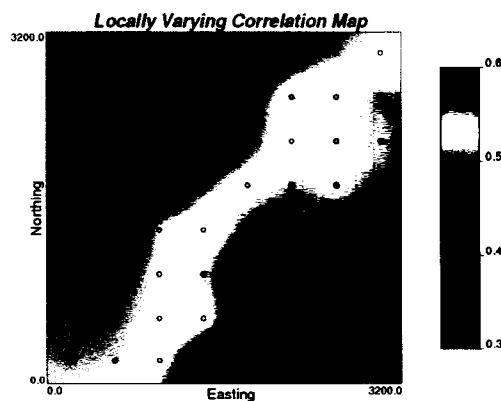
Figure 3-7: The locally varying correlation map of the two variables in Figure 3-5.
