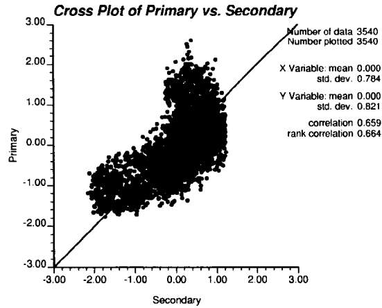
Figure 3-3: Cross plot of two variables that have a non-linear bivariate relationship.
