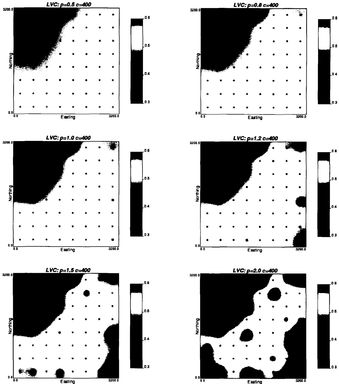
Figure 3-9: The locally varying correlation (LVC) maps with different powers.
