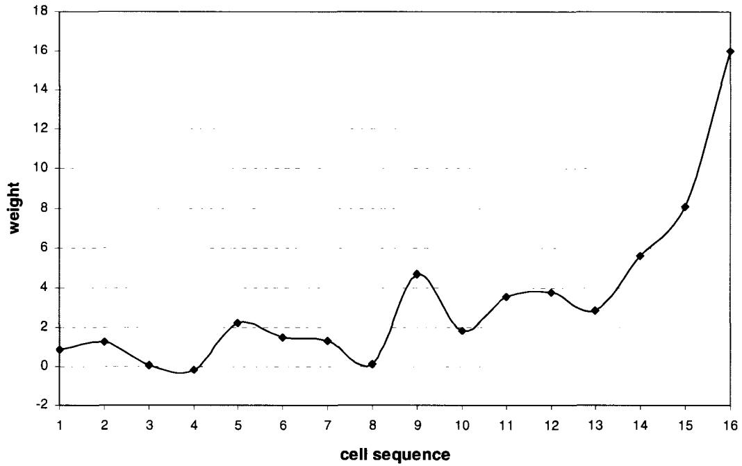
Figure 7-7: The kriging weight of block datum changes with simulation path
