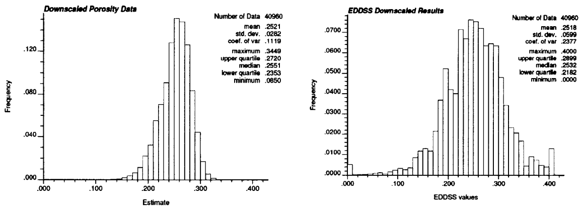
Figure 7-25: The histograms of the fine scale porosity estimated from EDDK (left) and simulated from EDDSS (right). The means are close to the input well data mean (Figure 7-16). The standard derivation of EDDK is small because of the kriging smoothness.
