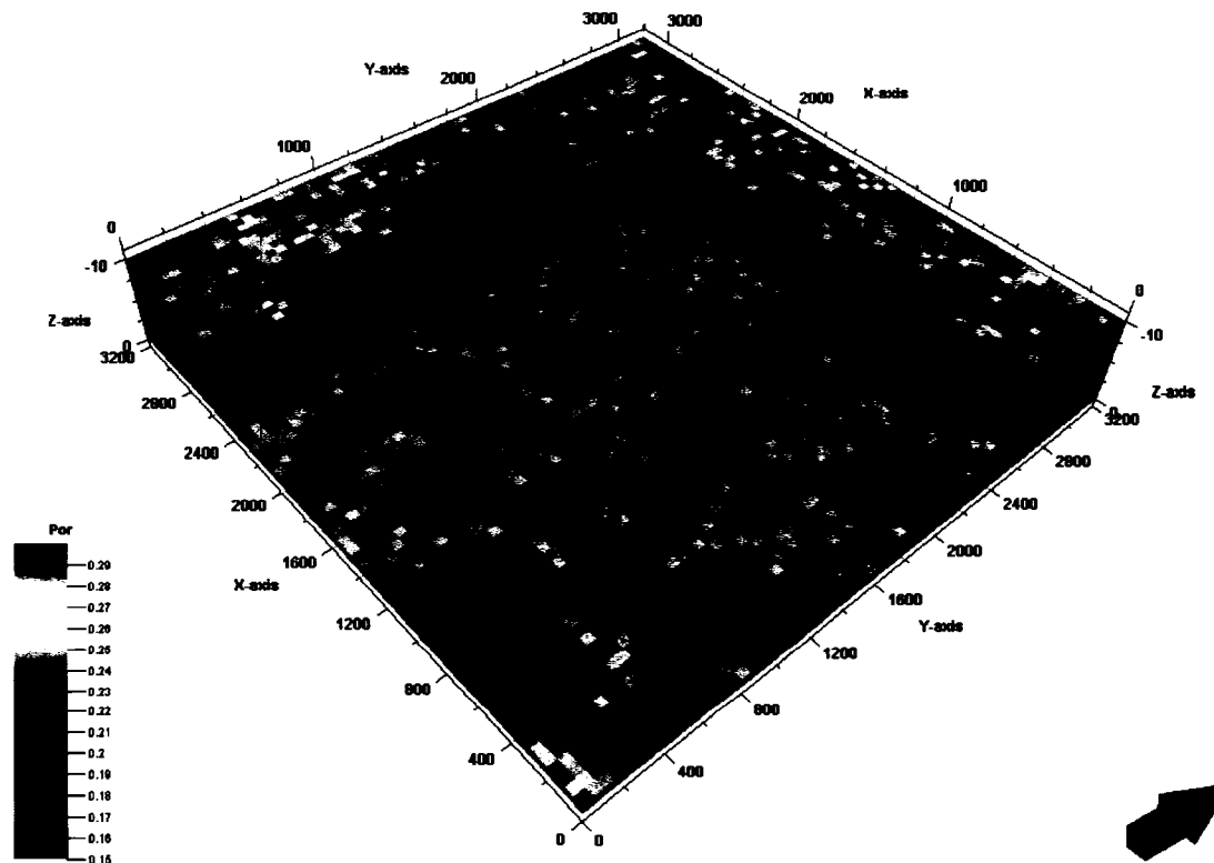
Figure 7-21: A 3-D porosity realization from EDDSS, the porosity is in fraction and the arrow is pointing to north.
