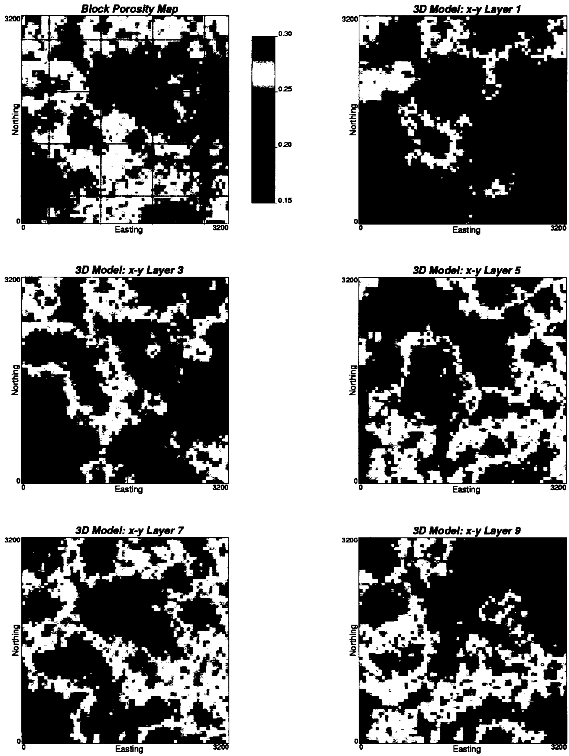
Figure 7-19: The 2-D porosity map and all odd numbered x-y view slices of the 3-D model from EDDK. The 3-D porosity is at the scale of 50 x 50 x 1m. The dashed lines in the porosity map (the top left) indicate the locations of the x-z and y-z cross sections, the porosity is in fraction.
