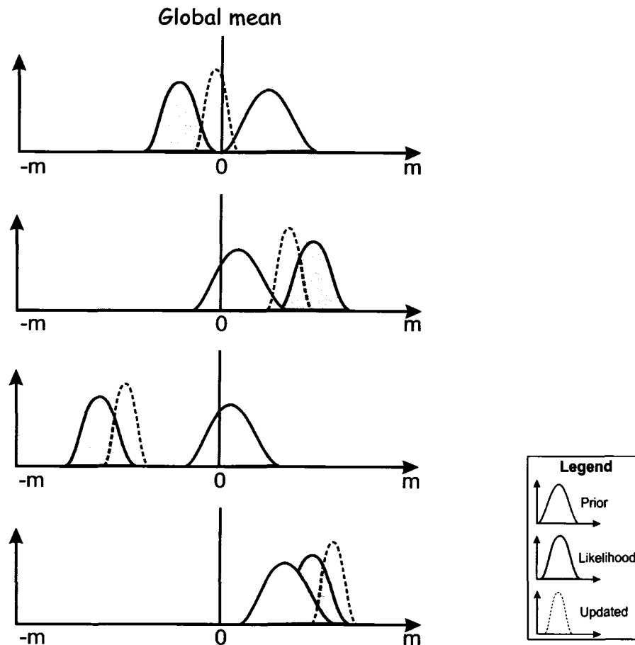
Figure 3-2: Schematic illustration of the location of updated distributions in Bayesian updating technique.
