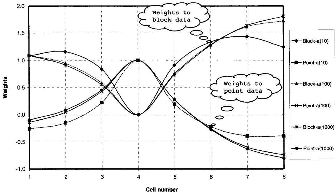
Figure 7-1: The kriging weights of block and point data with different variogram ranges.
