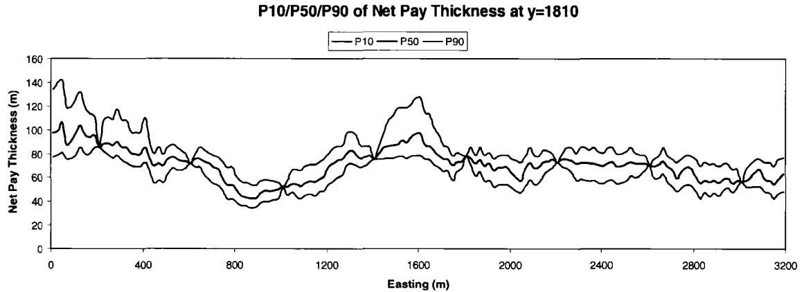
Figure 5-8: Uncertainty of Net Pay thickness in an east-west section: P10 (bottom line), P50 (middle line), and P90 (top line). The location of y=1810m is shown in the top row of Figure 5-7.
