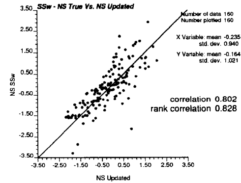
Figure 4-19: The cross validation of Bayesian updating results for water saturation in Gaussian units.
