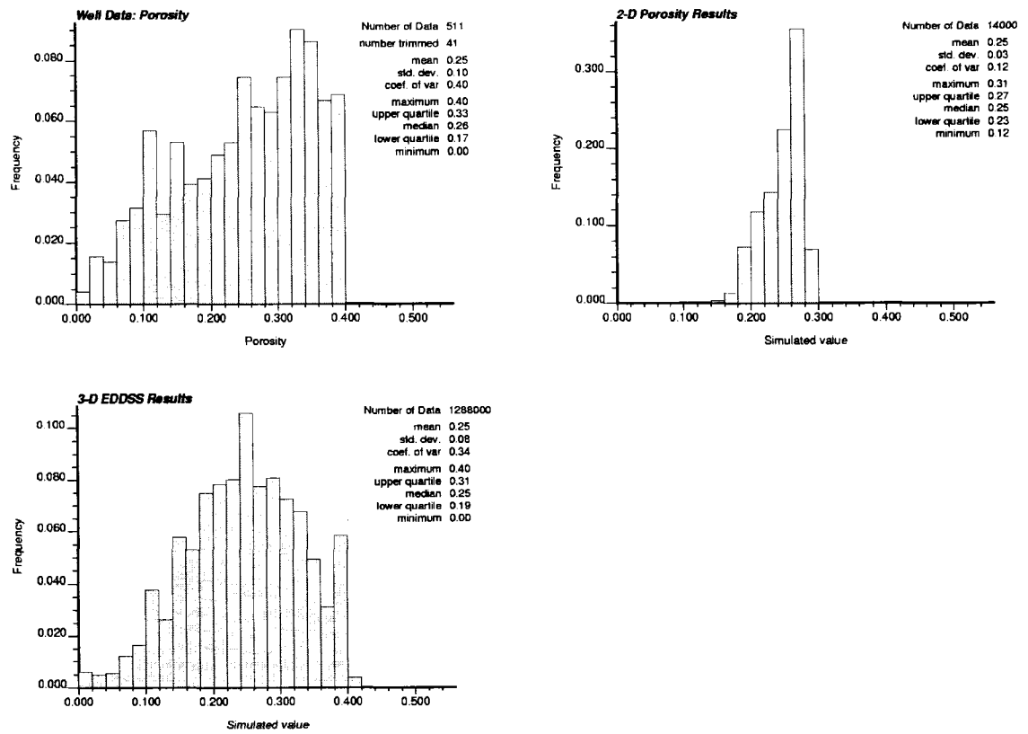
Figure 8-14: The histograms of point data (top left), block data (top right), and 3-D downscaled values (bottom).
