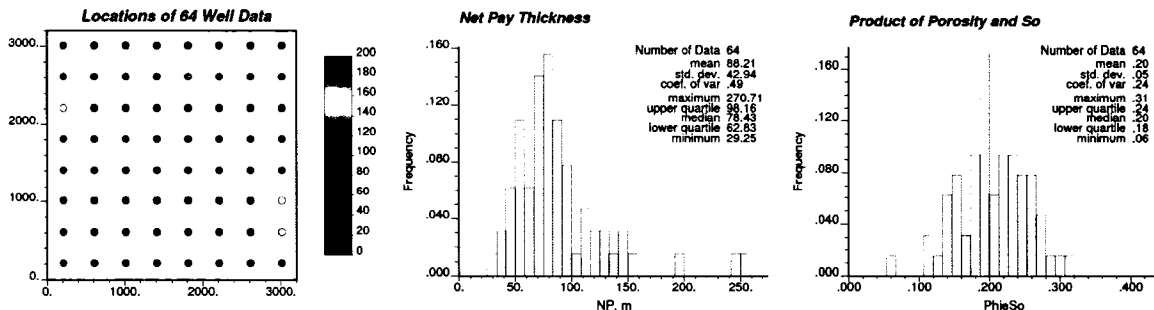
Figure 5-3: The location map of the 64 wells with the colour scale showing the net pay thickness in meters (left), and histograms of Net Pay thickness in meters (centre) and \phi S_o in fraction (right).
