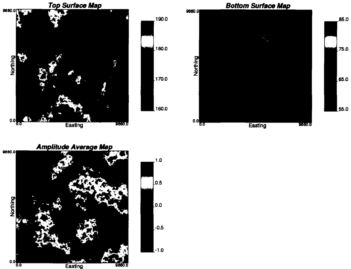
Figure 4-2: The maps of the secondary variables: top and bottom surfaces are depth in meters, and the vertical averaged amplitude is standardized to be values between 1 to -1.
