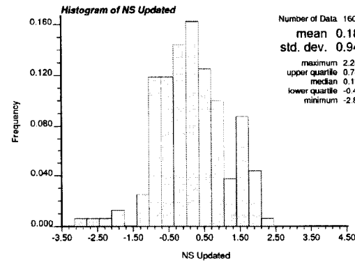
Figure 4-18: The cross validation of Bayesian updating results for porosity in Gaussian units.
