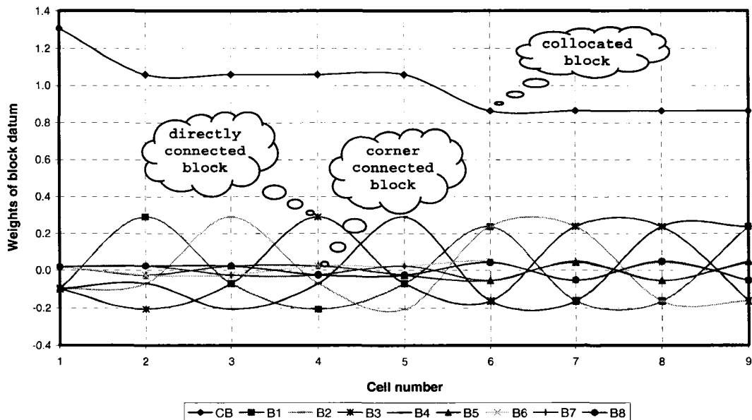
Figure 7-6: The weights of blocks in the small cell in case 3.
