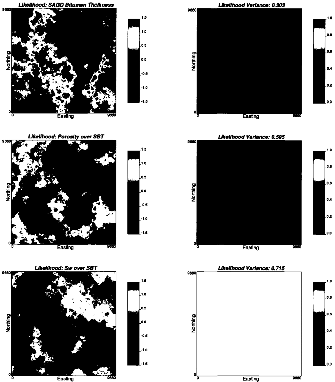
Figure 4-12: The likelihood maps of the primary variables from the global correlations. The left column is likelihood mean in Gaussian units and the right column is likelihood variance. The variances are constant over the model area.
