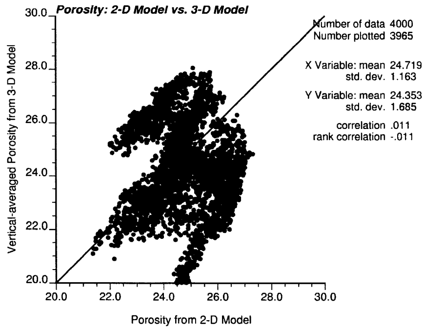
Figure 1-2: The cross plot of 2-D model versus the vertical averages of 3-D model of porosity in % (from Ren et al. , 2005c).
