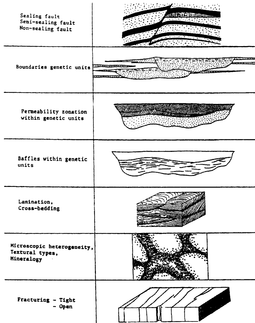
Figure 2-1: Classifications of reservoir heterogeneity types (from Weber, 1986).
