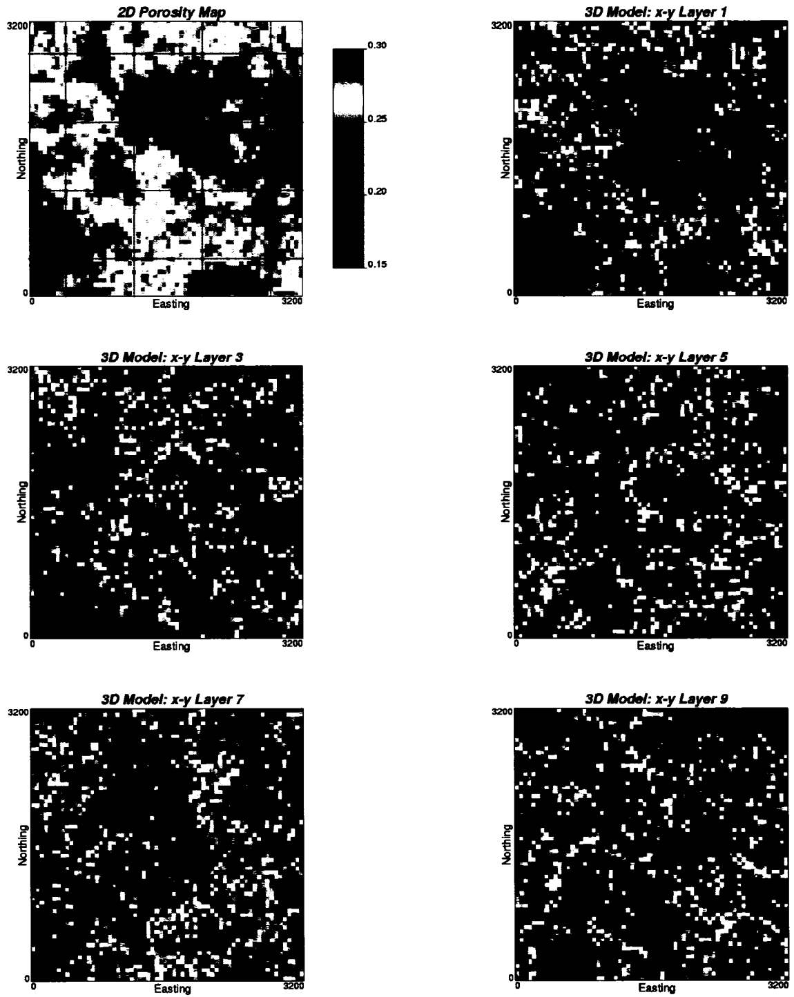
Figure 7-22: The 2-D porosity map and all odd numbered x-y view slices of the 3-D model from EDDSS. The 3-D porosity is at the scale of 50 x 50 x 1m. The dashed lines in the porosity map (the top left) indicate the locations of the x-z and y-z cross sections.
