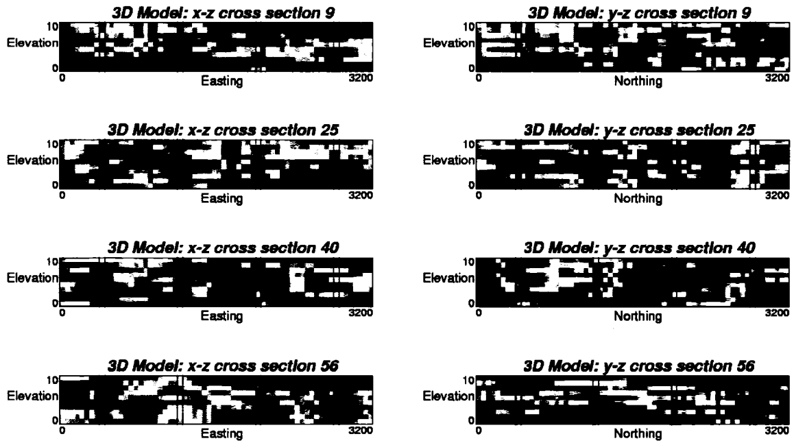
Figure 7-20: The x-z and y-z cross sections of the 3-D porosity model from EDDK. The 3-D porosity is at scale of 50x50x1m. The dashed lines in the x-z and y-z cross sections indicate the wells. The horizontal continuity matches the well data.
