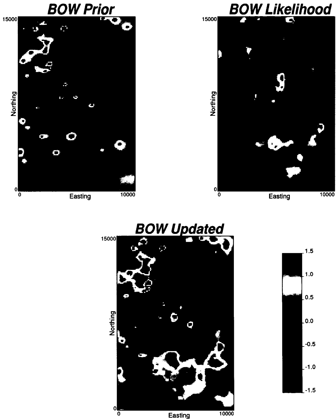
Figure 8-8: The prior (top left), likelihood (top right) and updated maps (bottom) of BOW in Gaussian units.
