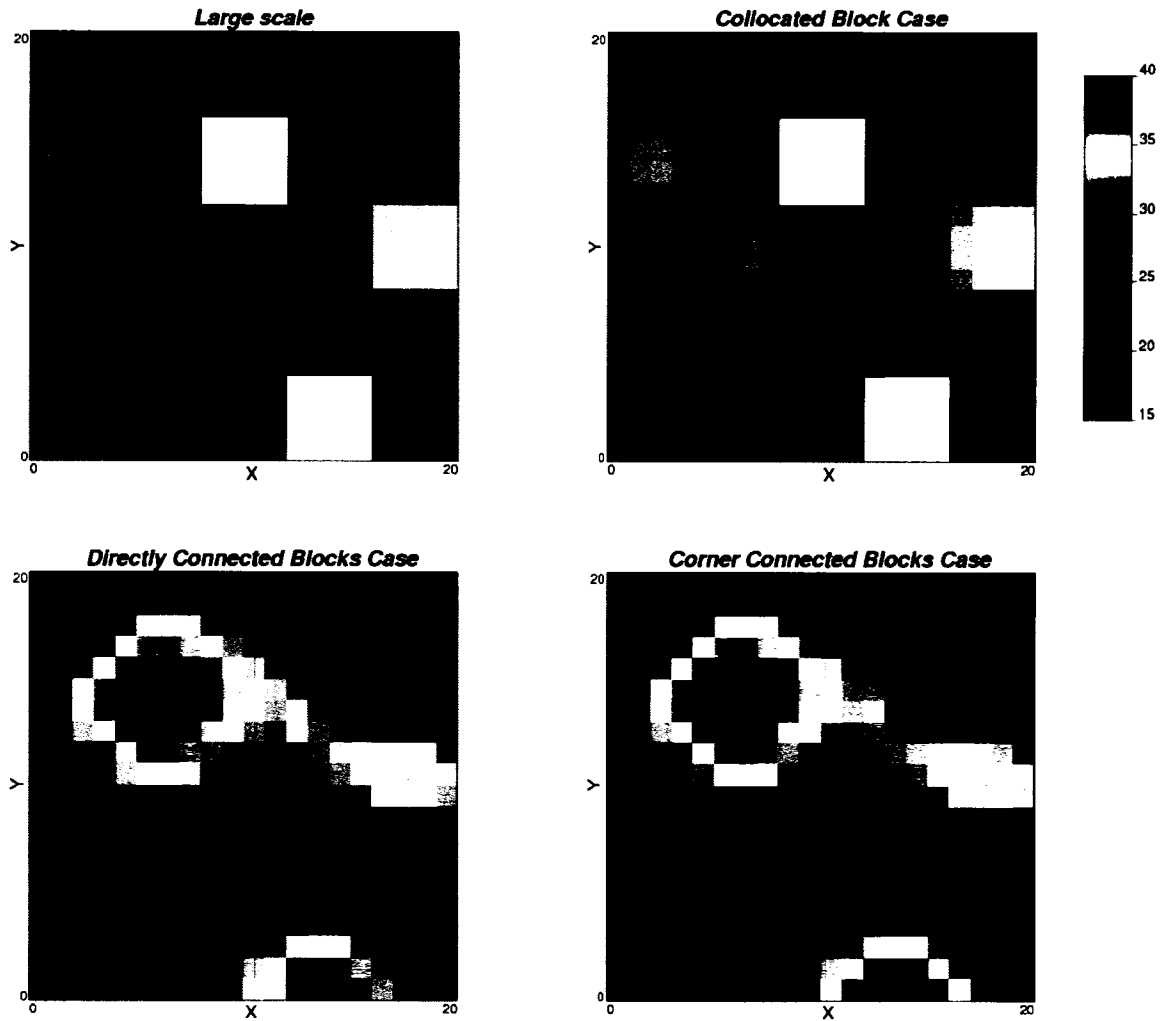
Figure 7-3: The large scale data (upper left) and the downscaled results in the three cases.
