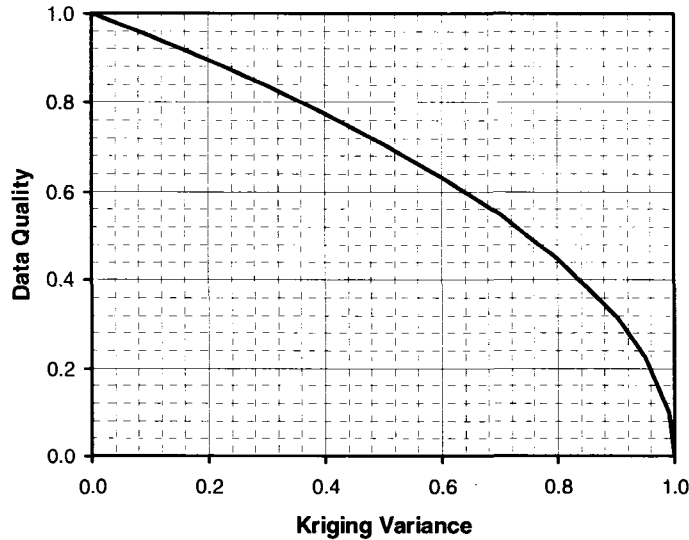
Figure 3-12: The curve of data quality versus kriging variance when the maximum quality C is 1.
