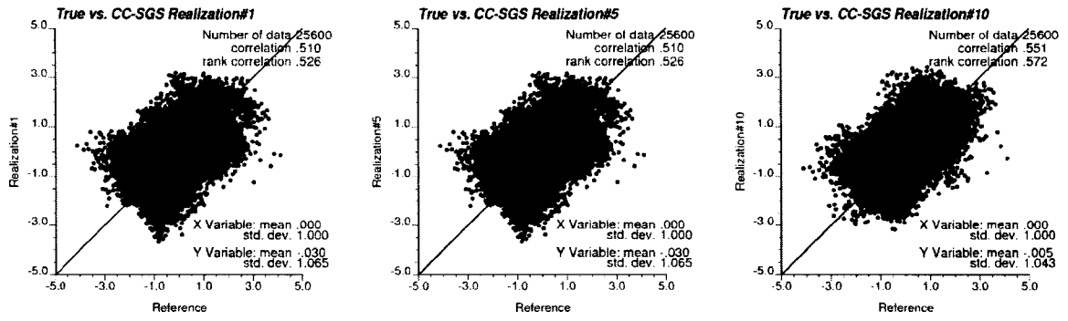
Figure 3-25: The cross plots of the reference versus the collocated co-simulation realizations #1, #5 and #10.
