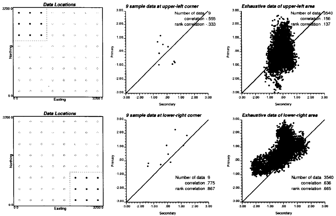
Figure 3-6: The data locations and the cross plots for the upper-left corner (upper row) and the lower-right corner (lower row). The middle column shows the cross plots of the nine data shown in the location map. The right column shows the cross plots of exhaustive data in these corners.
