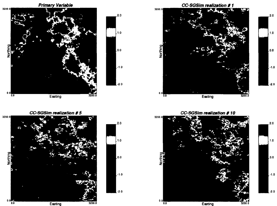
Figure 3-24: The primary variable (reference, up-left) and the collocated co-simulation realizations.
