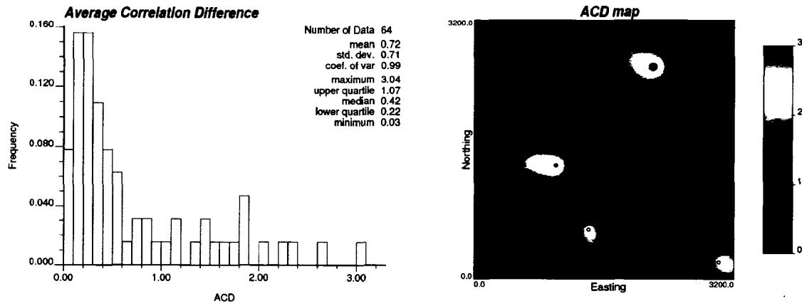
Figure 3-10: The histogram and kriged map of ACD for the two variables shown in Figure 3-5.
