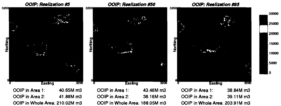
Figure 5-10: Calculated OOIP from the two variables shown in Figure 5-9. The colour scale shows the OOIP in cubic meters. Two areas of interest (in black box) and the whole model area were selected to estimate the global OOIP. The global OOIP in the three areas in million cubic meters are shown below the maps for each realization.
