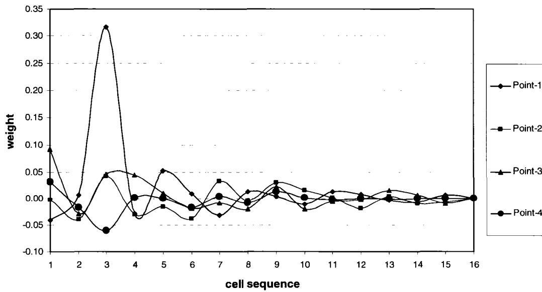
Figure 7-8: The kriging weights of point data changes with simulation path.
