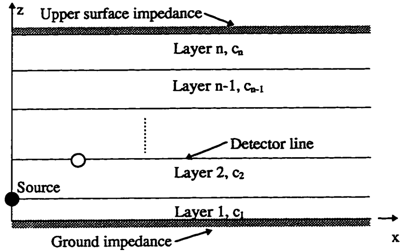
Figure D.1: Layered atmosphere for FFP implementations.
