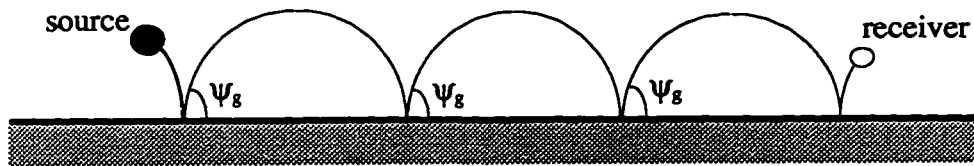
Figure C.2: Multiple ground reflections for any sound ray under strong positive gradients.
