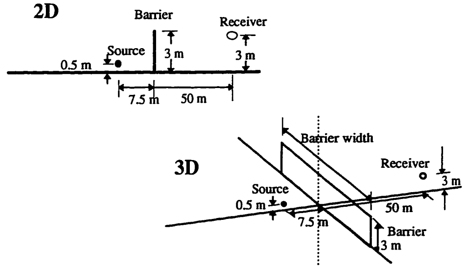
Figure 2.25: Comparisons between 2D and 3D barrier geometry by varying 3D barrier width.
