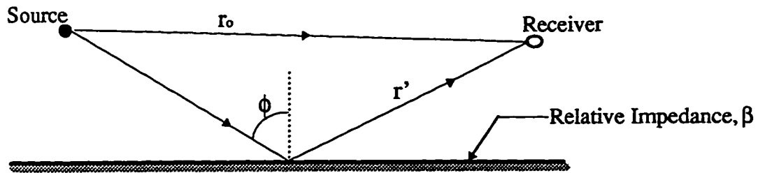
Figure 2.6: Source and receiver above ground with finite impedance.
