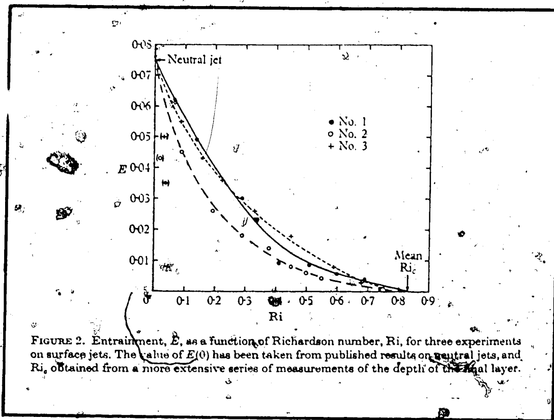
FIG. 5.01 ENTRAINMENT ( E ) AS A FUNCTION OF THE GRADIENT RICHARDSON NUMBER ( R_i ) FROM ELLISON AND TURNER (II)
