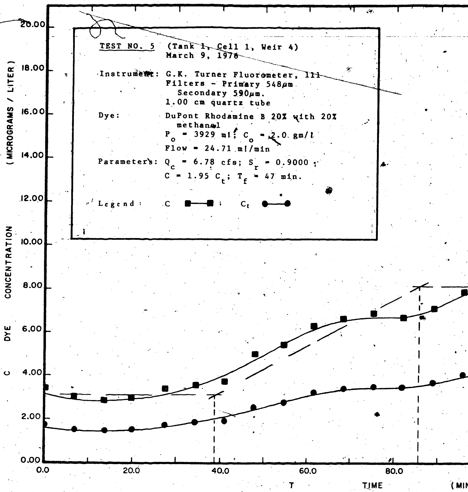
FIG. 4.05 A TIME - CONCENTRATION CURVES
