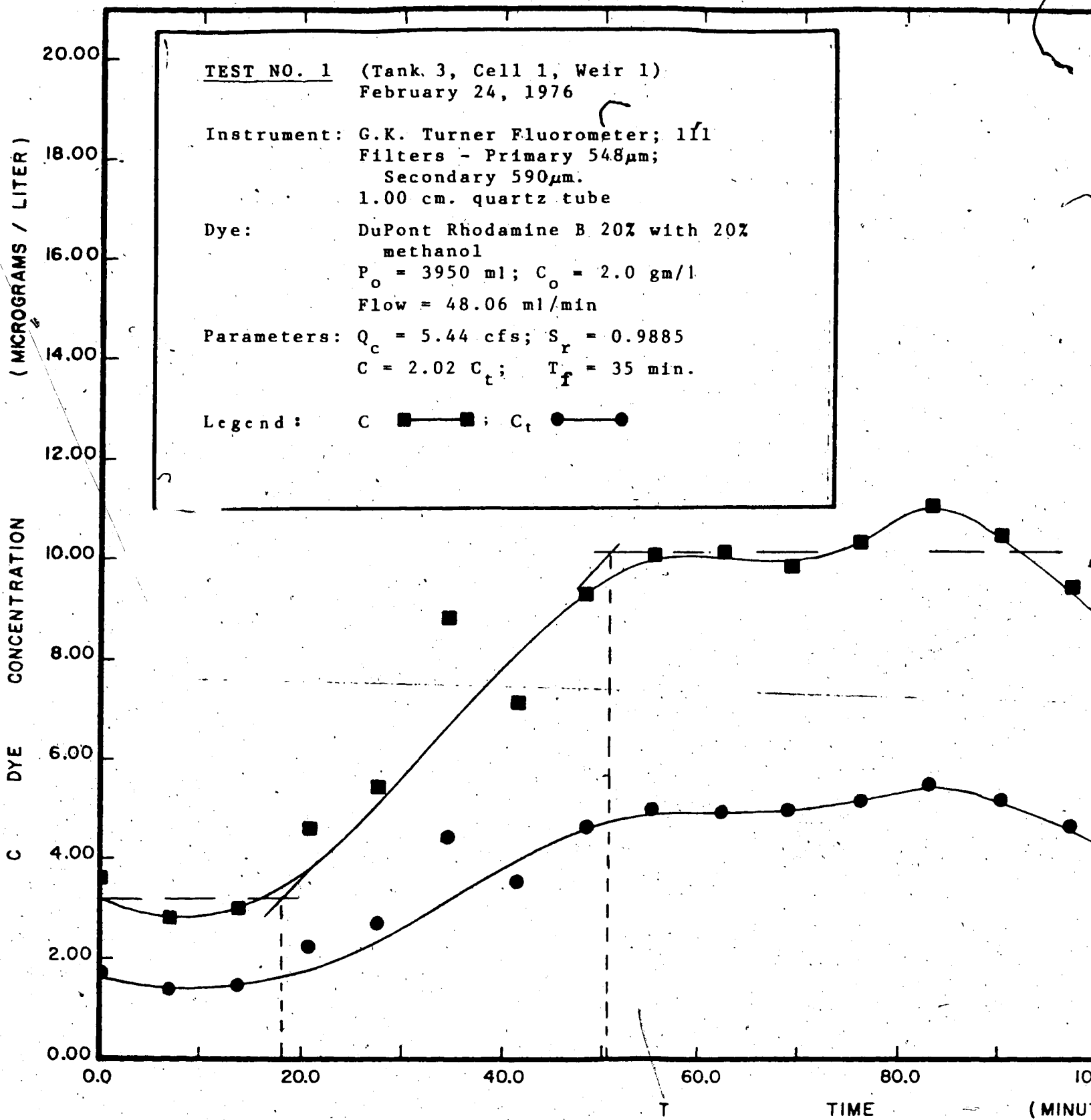
FIG. 4.01A TIME - CONCENTRATION CURVES
