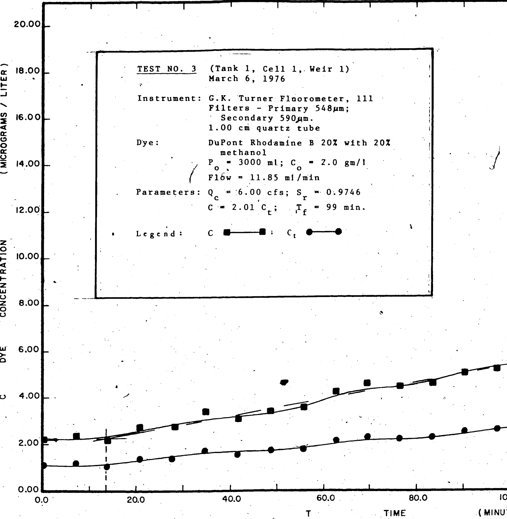
G. 4.03A TIME - CONCENTRATION CURVES
