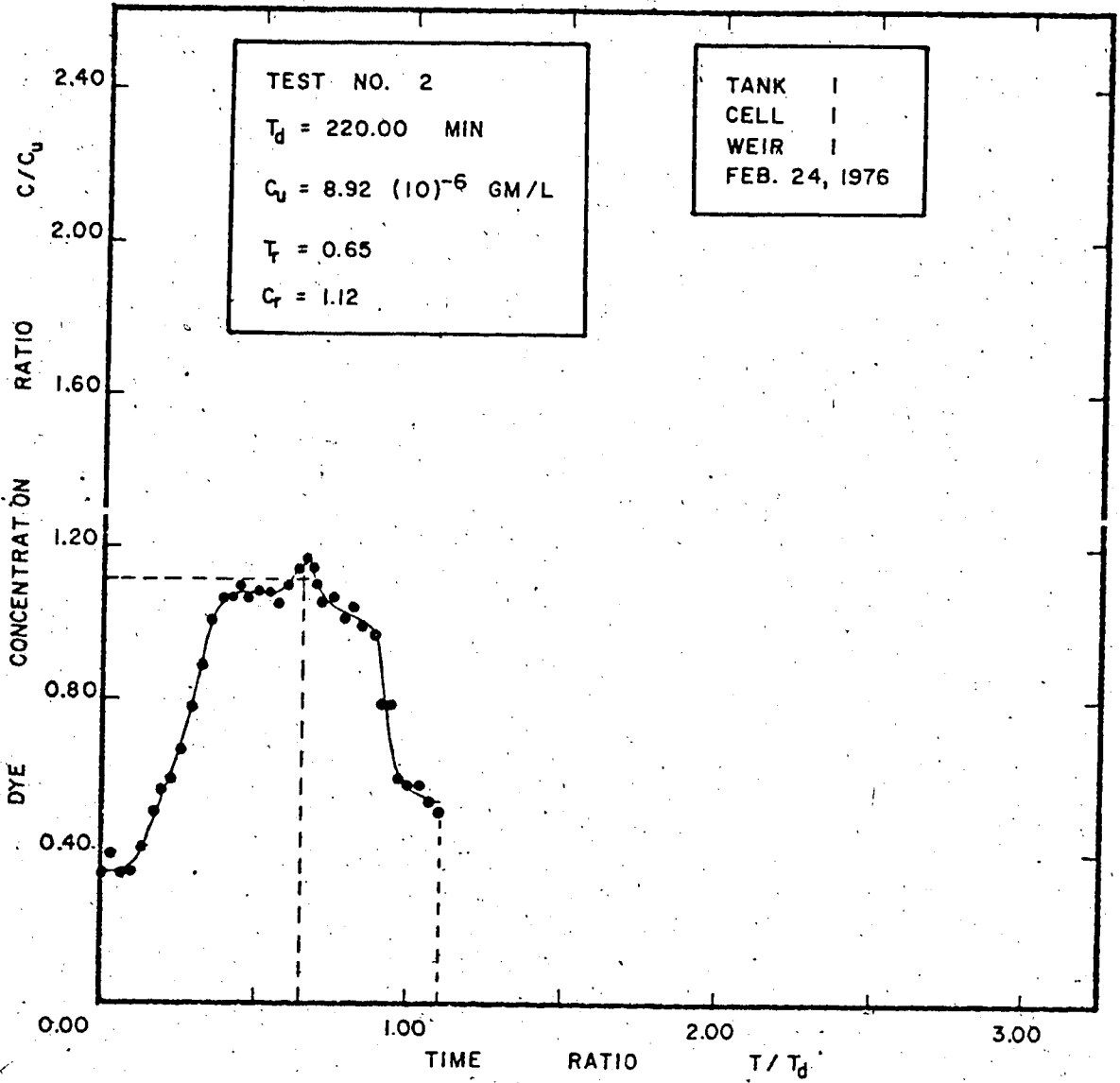
FIG. 5.02 A DIMENSIONLESS ANALYSIS OF TIME - CONCENTRATION CURVES
