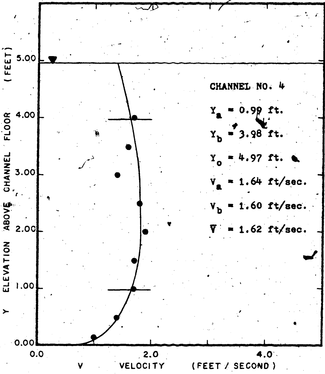
FIG. I.13A CROSS CHANNEL VELOCITY PROFILE
