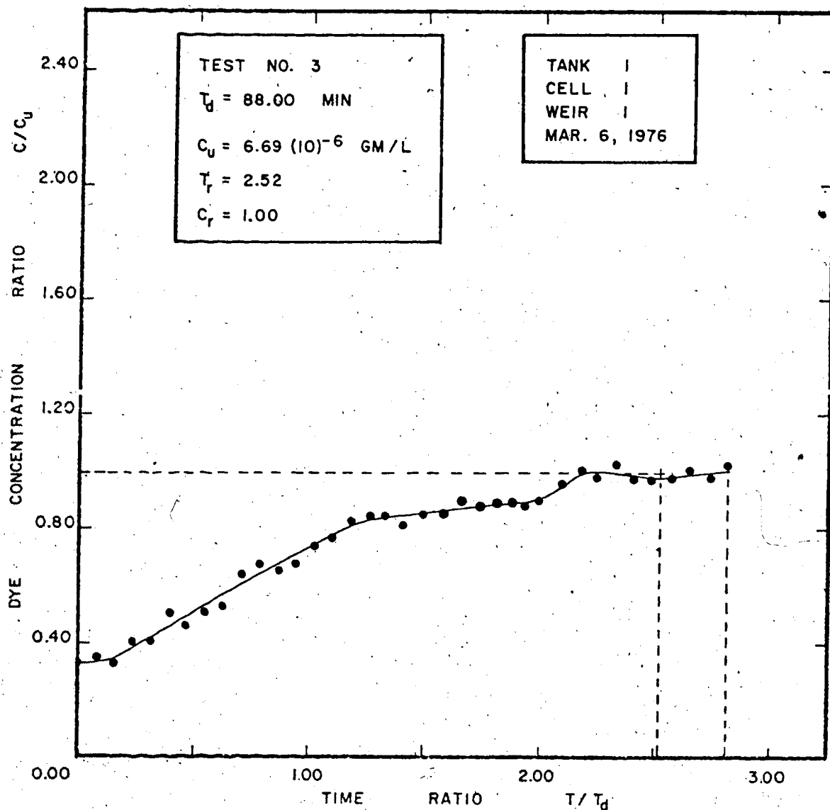
FIG. 5.03A DIMENSIONLESS ANALYSIS OF TIME - CONCENTRATION CURVES.
