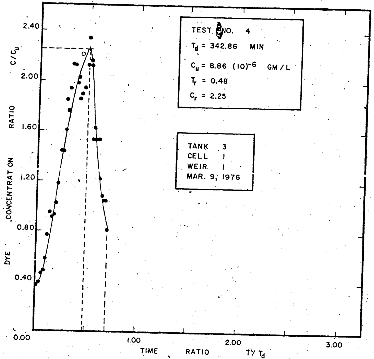
FIG. 5.04 A DIMENSIONLESS ANALYSIS OF TIME - CONCENTRATION CURVES
