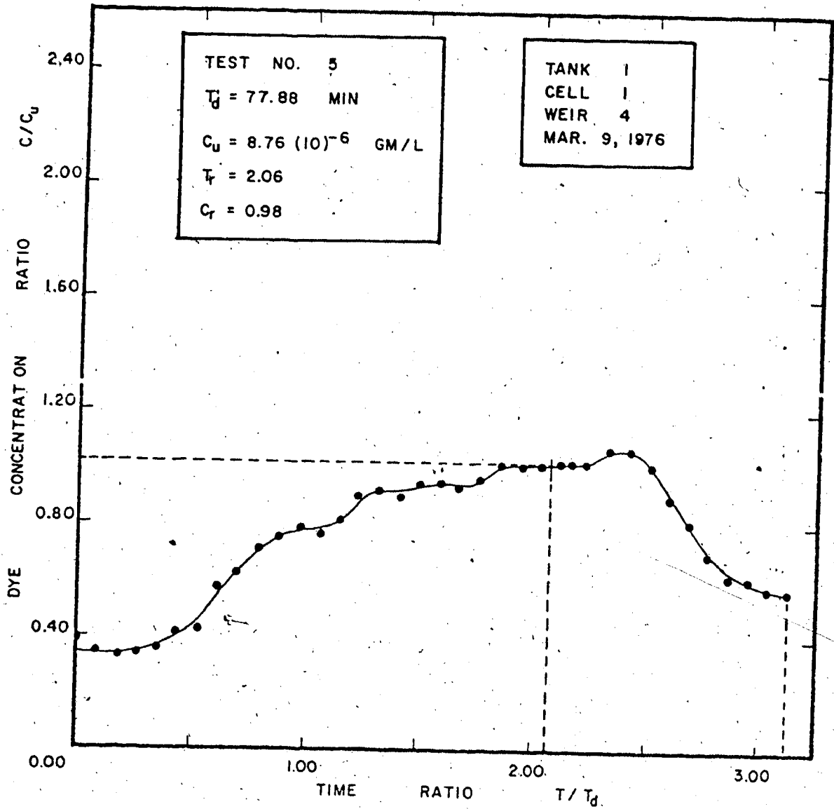
FIG. 5.05A DIMENSIONLESS ANALYSIS OF TIME - CONCENTRATION CURVES
