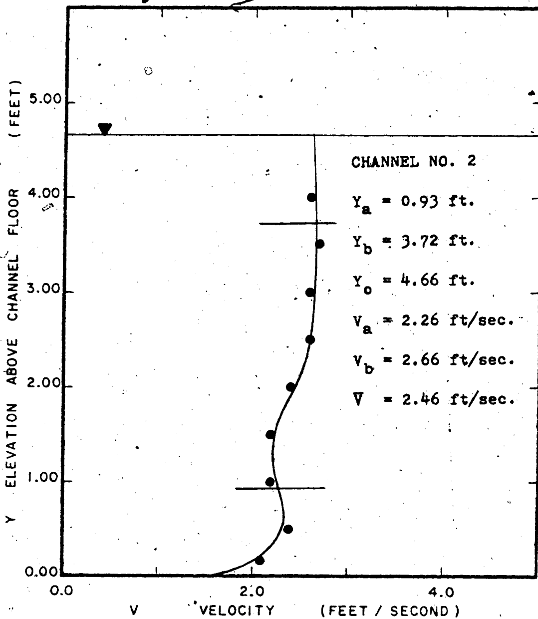
FIG. I.07A CROSS CHANNEL VELOCITY PROFILE
