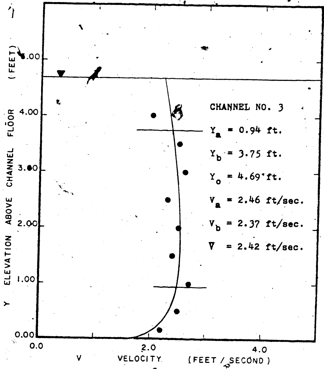
FIG. 1.11 A CROSS CHANNEL VELOCITY PROFILE
