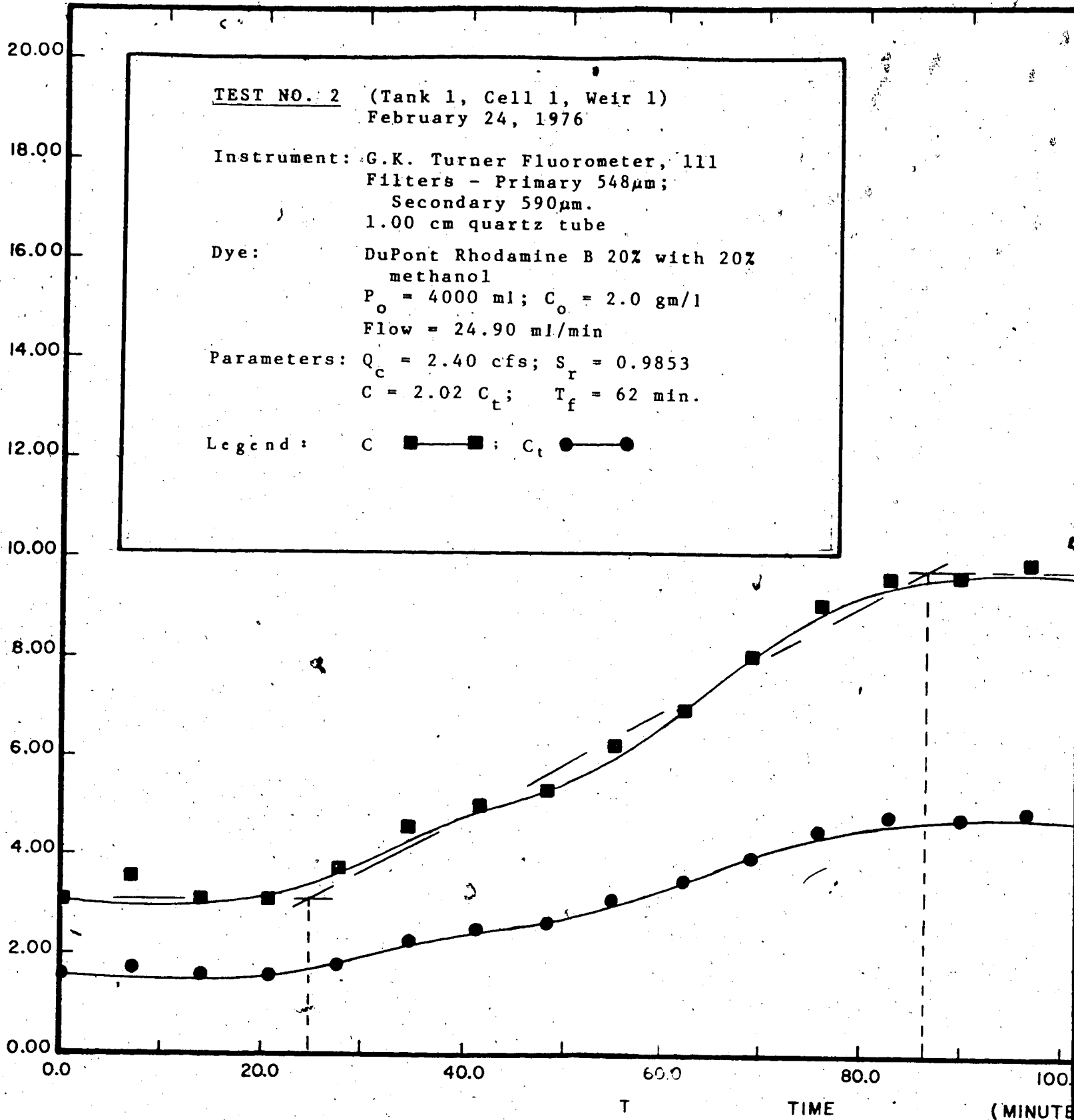
4.02 A TIME - CONCENTRATION CURVES
