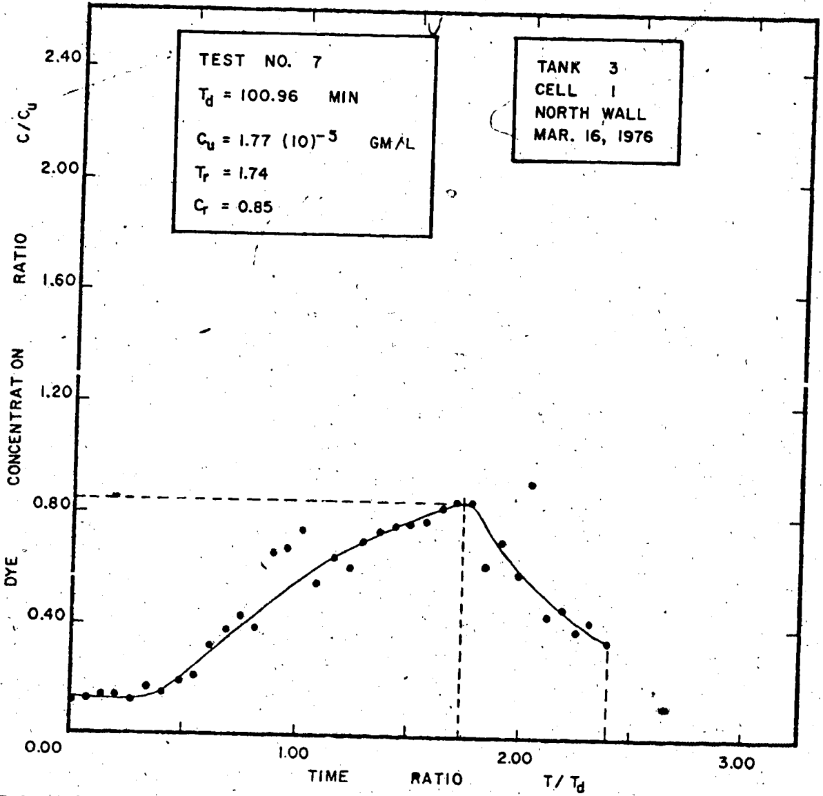
FIG. 5.07A DIMENSIONLESS ANALYSIS OF TIME - CONCENTRATION CURVES
