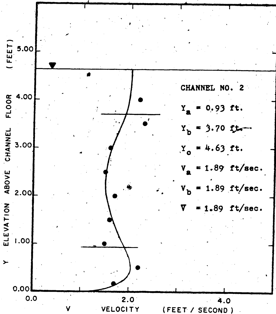
FIG. 1.06A CROSS CHANNEL VELOCITY PROFILE
