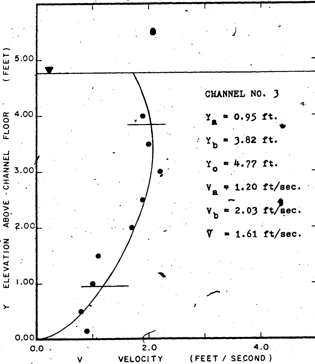
FIG. 1.09A. CROSS CHANNEL VELOCITY PROFILE
