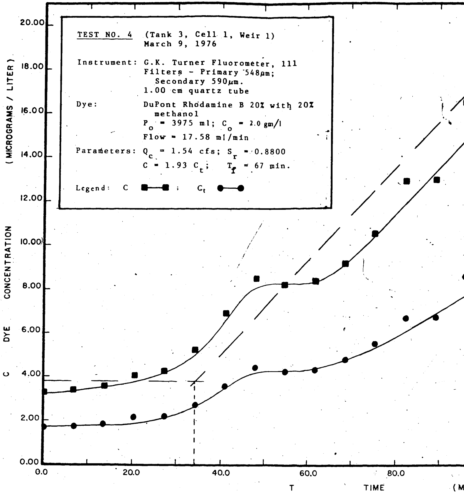
FIG. 4.04 A TIME - CONCENTRATION CURVES
