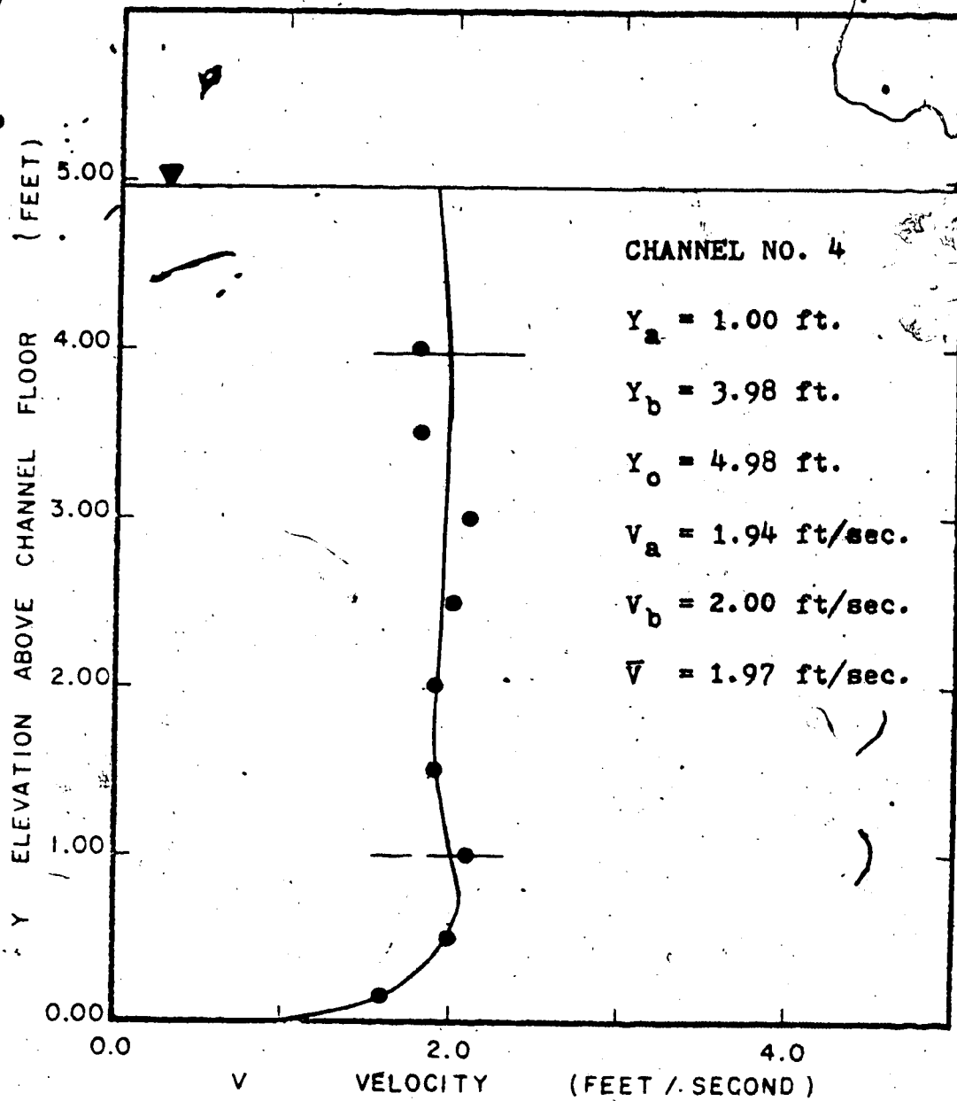
FIG. I.12A CROSS CHANNEL VELOCITY PROFILE
