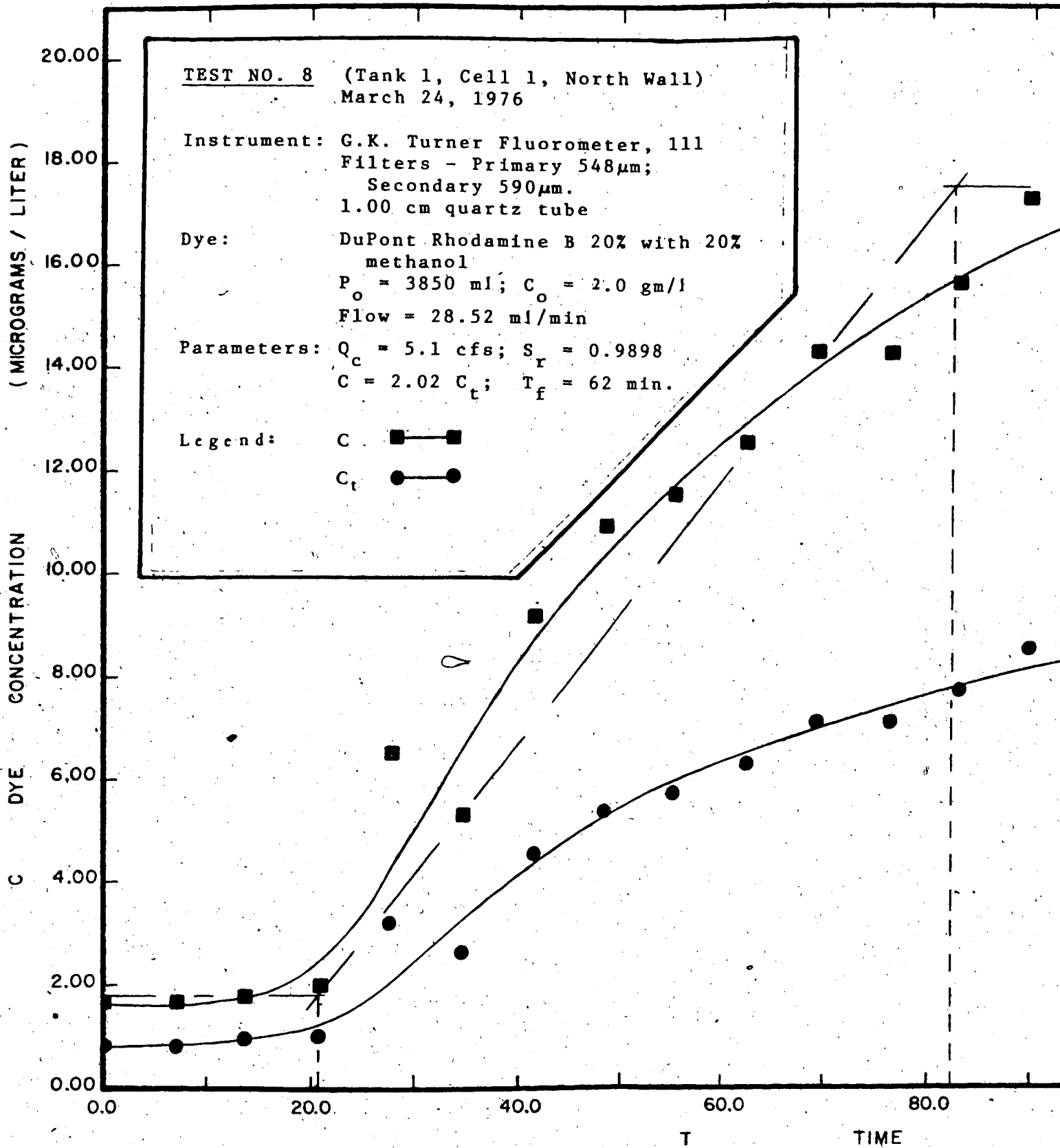
FIG. 4.08 A TIME - CONCENTRATION CURVES
