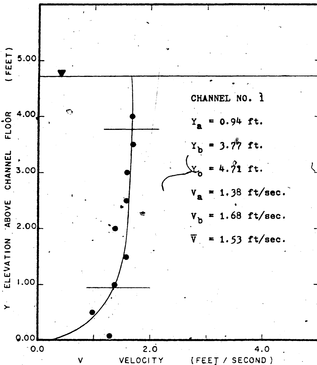
FIG. 1.02A CROSS CHANNEL VELOCITY PROFILE
