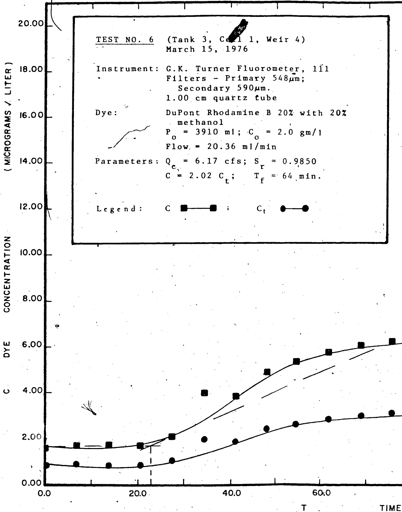
FIG. 4.06 A TIME - CONCENTRATION CURVES
