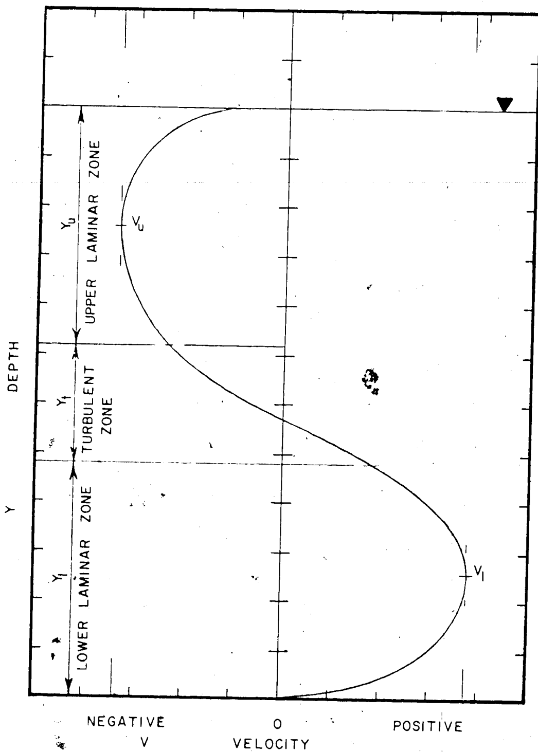
FIG. 4.06 CHARACTERISTIC VELOCITY PROFILE WITHIN THE MODEL TANK
