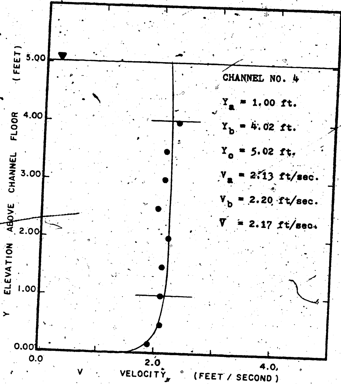
FIG. 1.14 A CROSS CHANNEL VELOCITY PROFILE
