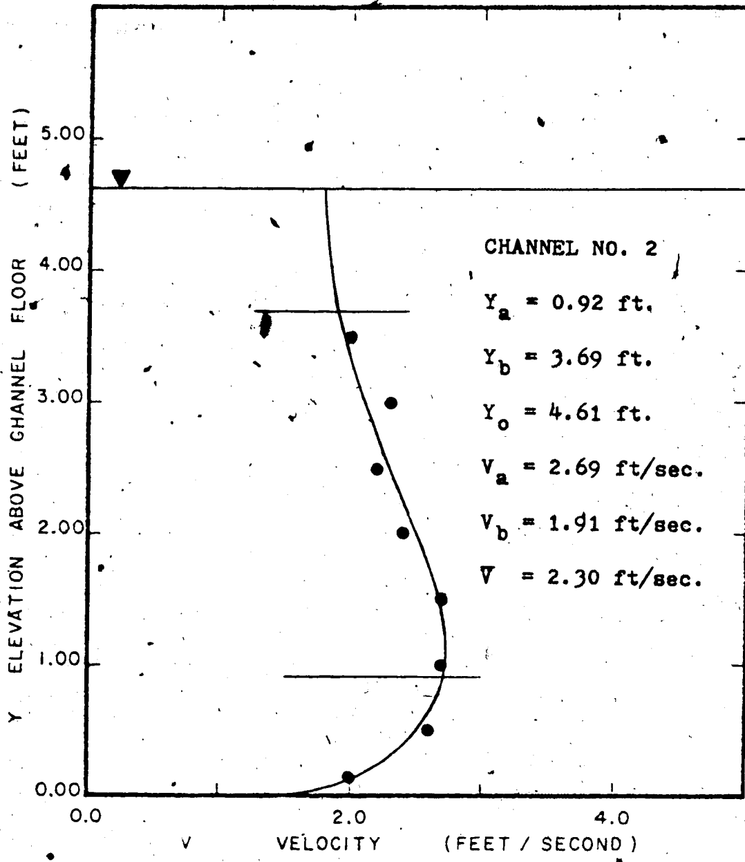
FIG. I.04A CROSS CHANNEL VELOCITY PROFILE
