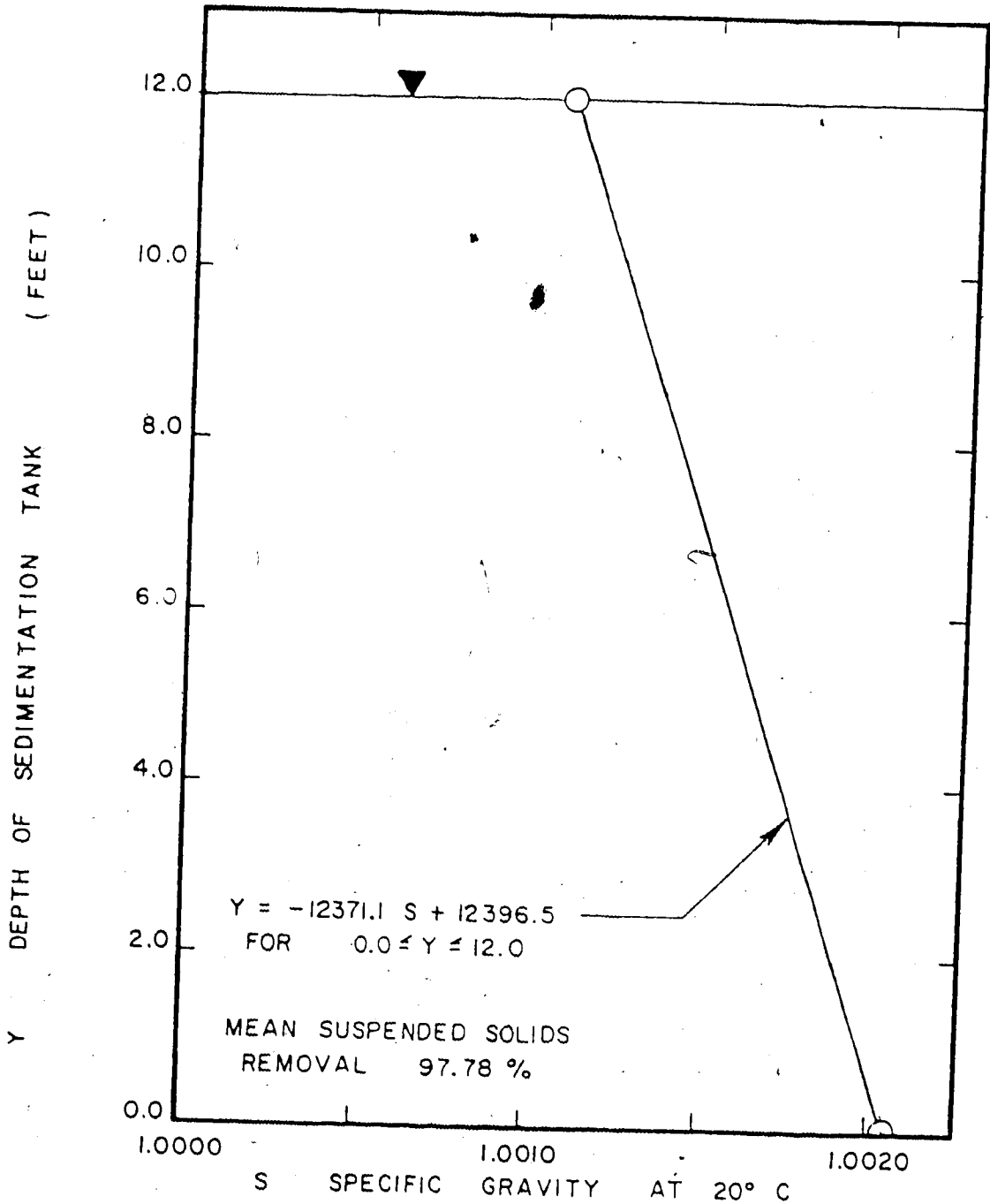
FIG. 4.04 MEAN SPECIFIC GRAVITY AS A FUNCTION OF DEPTH IN THE SECONDARY SEDIMENTATION TANK
