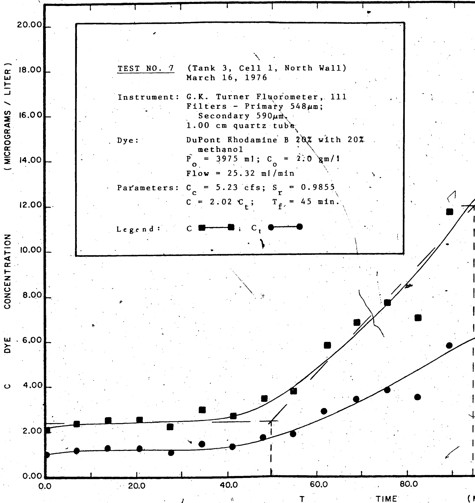
FIG. 4.07 A TIME - CONCENTRATION CURVES
