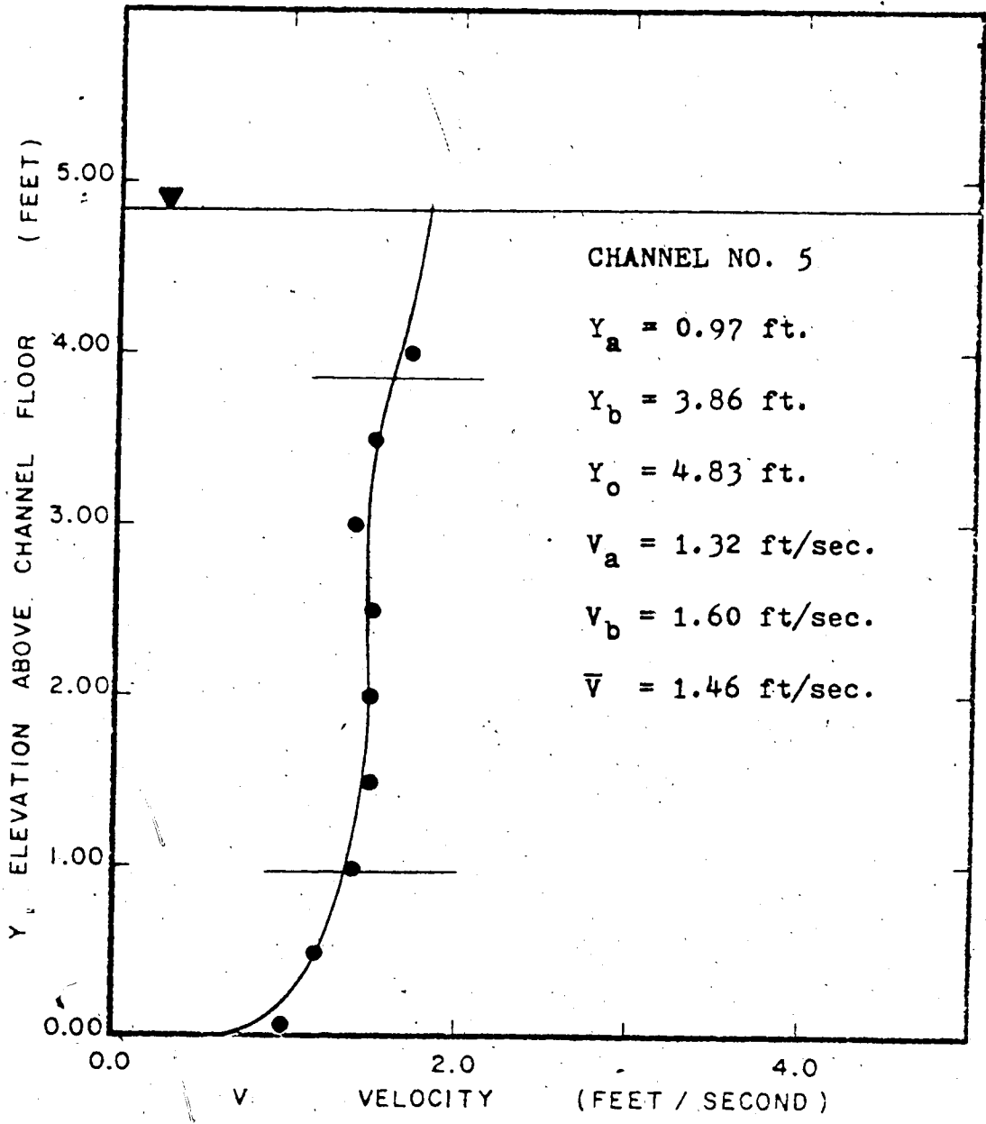
FIG. 1.17A CROSS CHANNEL VELOCITY PROFILE
