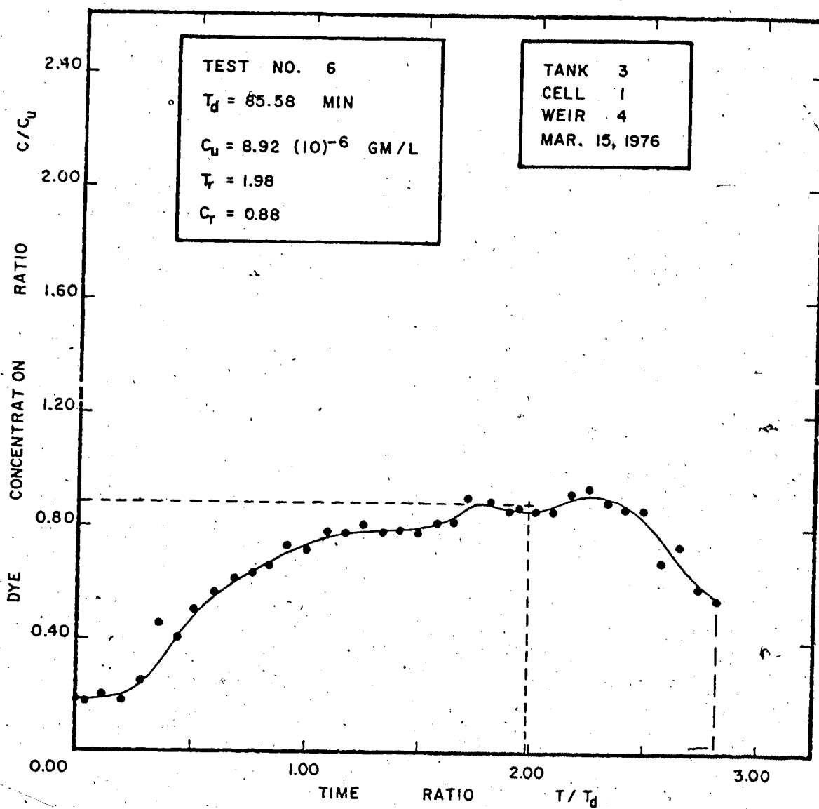
FIG. 5.06 A DIMENSIONLESS ANALYSIS OF TIME - CONCENTRATION CURVES
