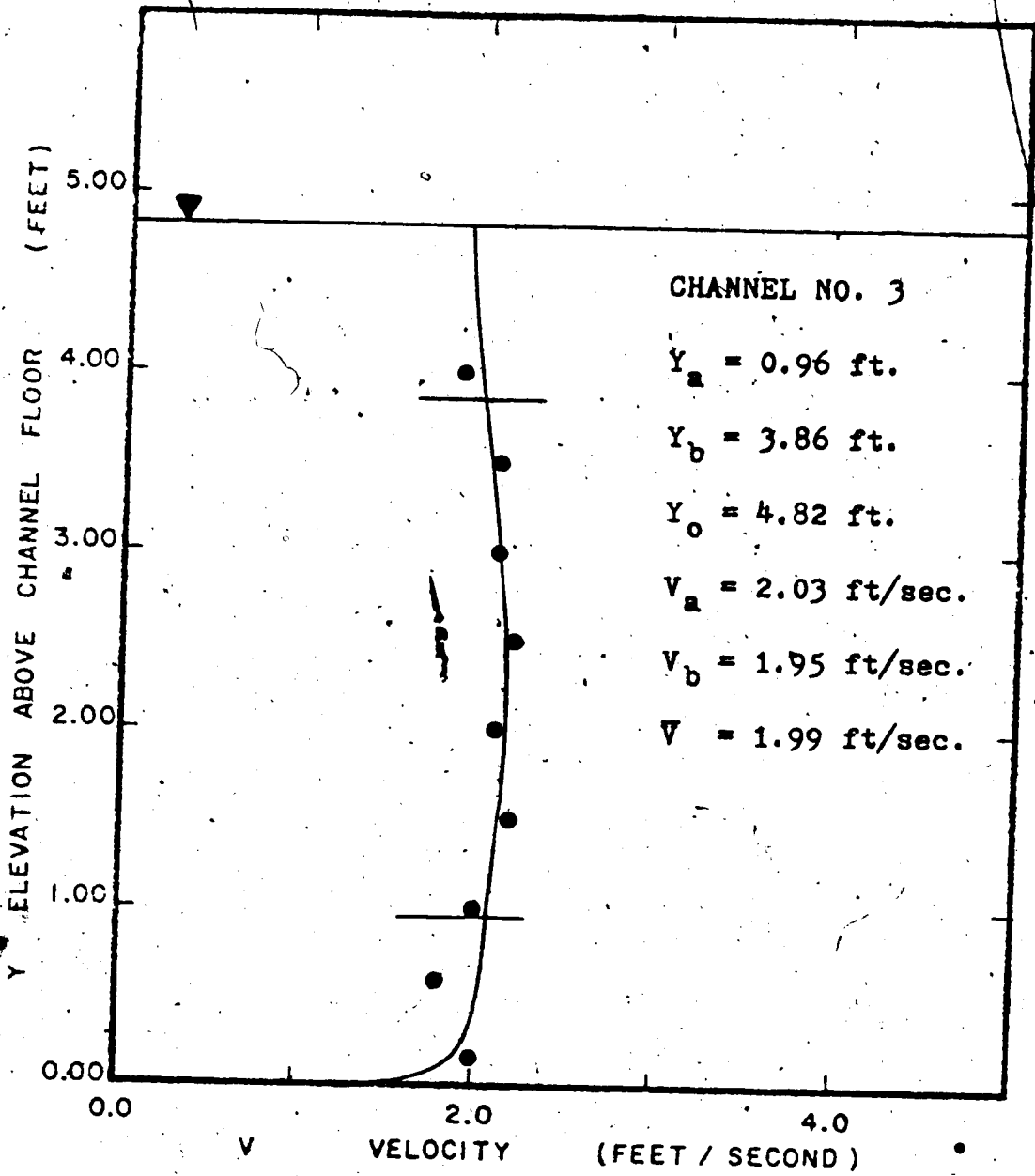
FIG. 1.08A CROSS CHANNEL VELOCITY PROFILE
