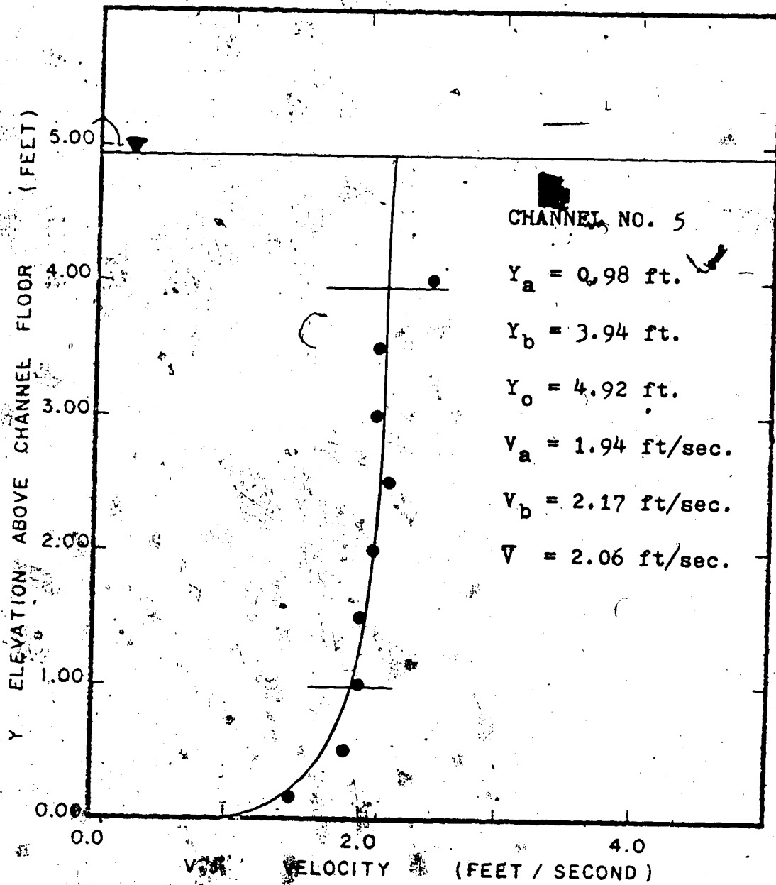
FIG. 1.15 A CROSS CHANNEL VELOCITY PROFILE
