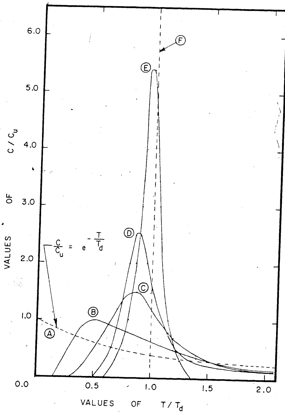
FIG. 3.04 TYPICAL DISPERSION CURVES FOR TANKS — REPRINTED WITH MODIFICATIONS FROM T.R. CAMP (6)
