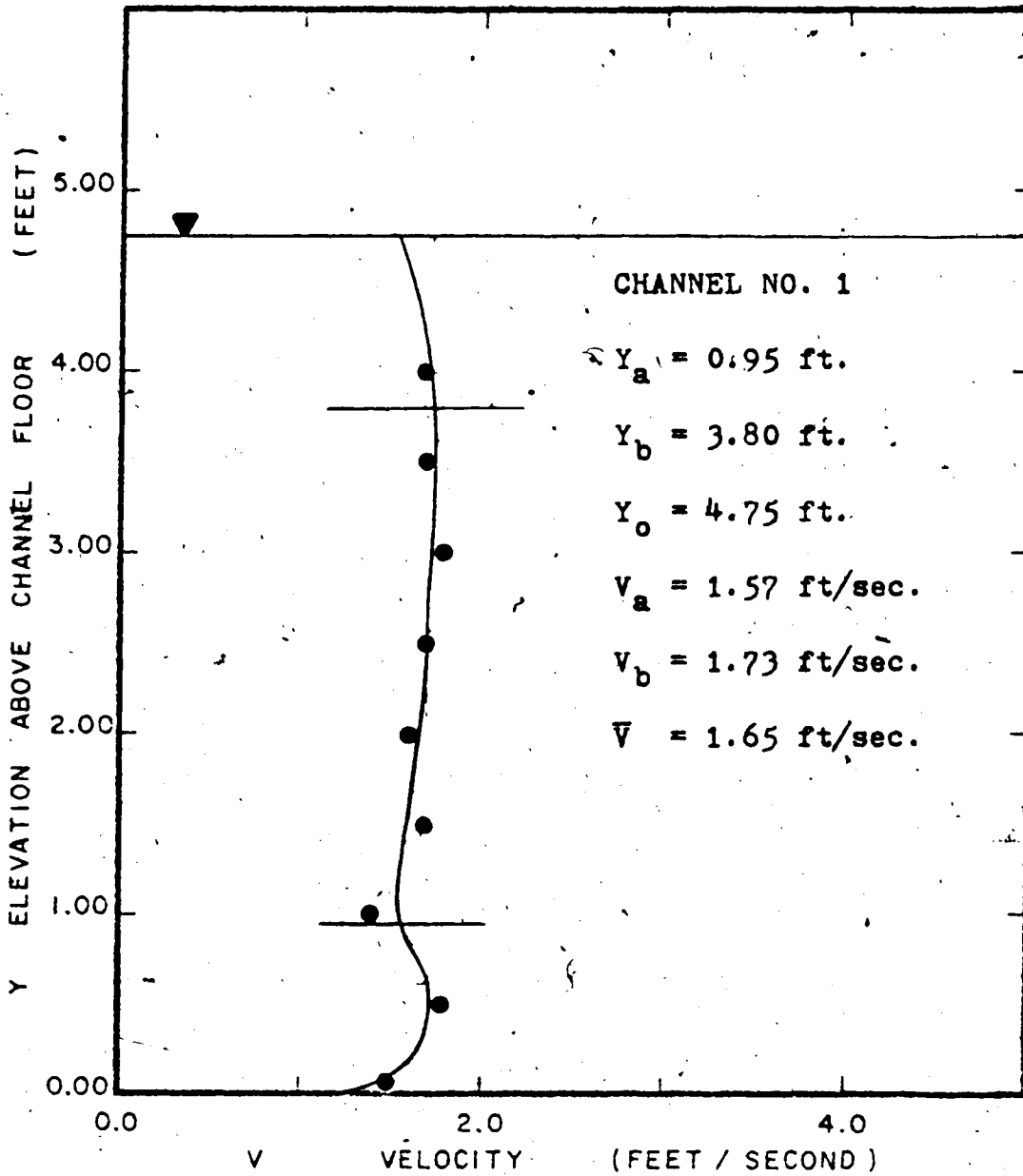
FIG. 1.03 A CROSS CHANNEL VELOCITY PROFILE
