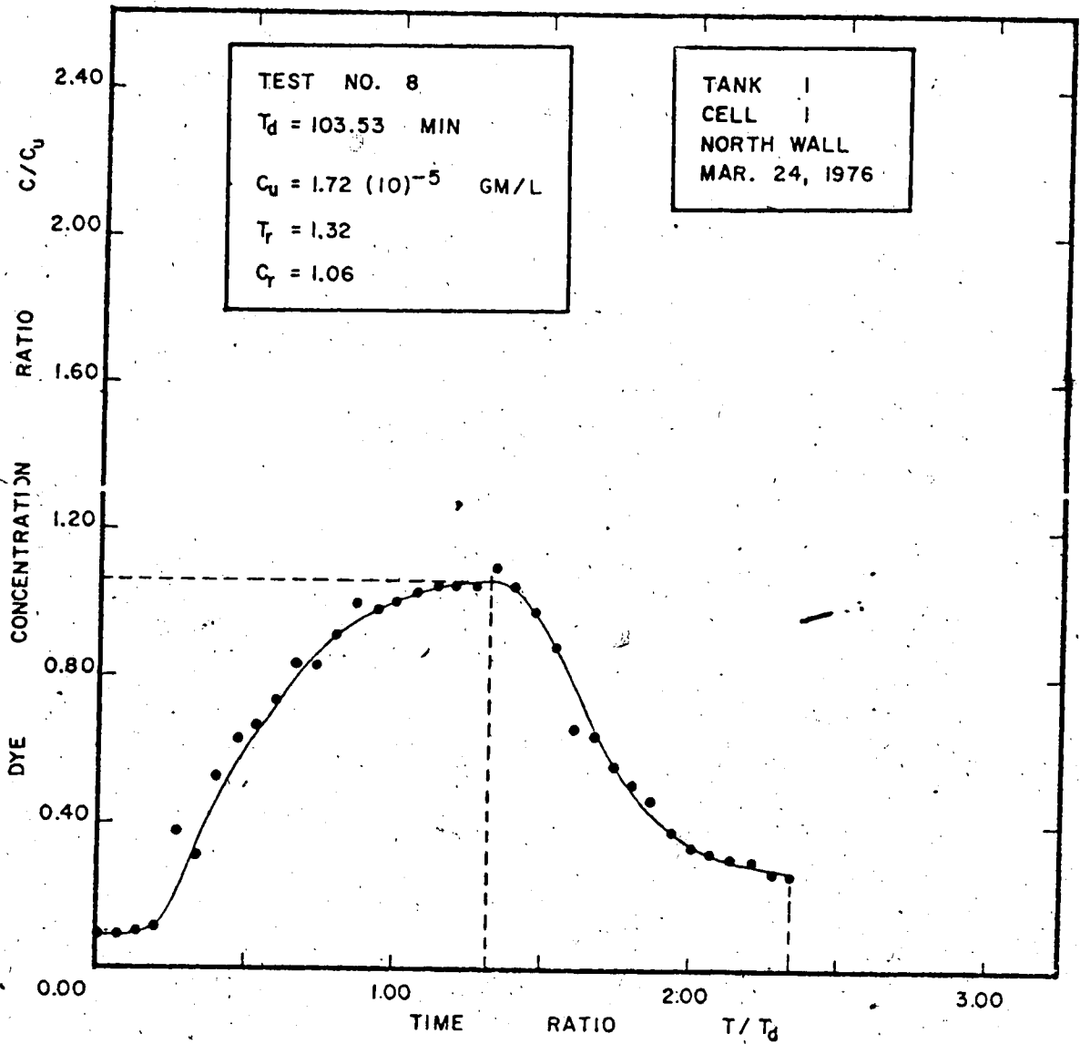
FIG. 5.08 A DIMENSIONLESS ANALYSIS OF TIME - CONCENTRATION CURVES
