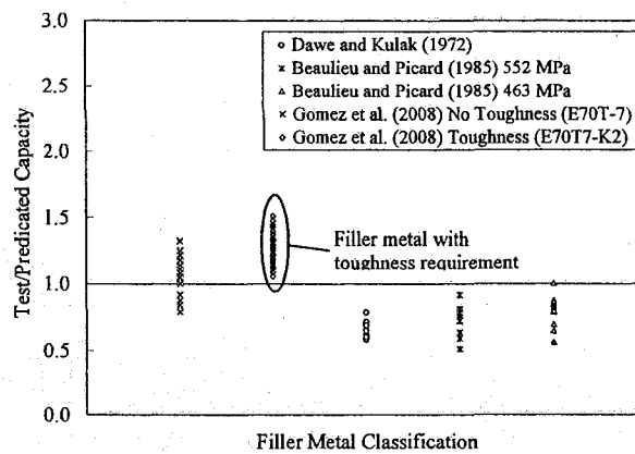
f) Test-to-predicted ratio versus filler metal classification
