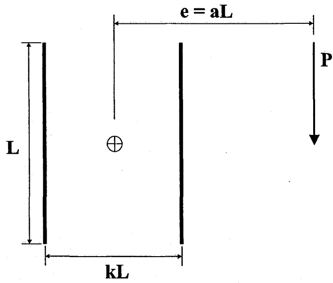
Figure 4.3 – In-plane eccentricity
