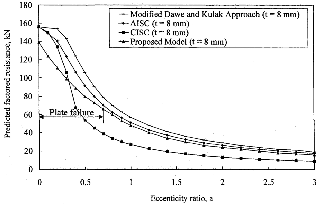
Figure D.2 Predicted capacity versus eccentricity ratio for t = 8 mm and D = 5 mm
