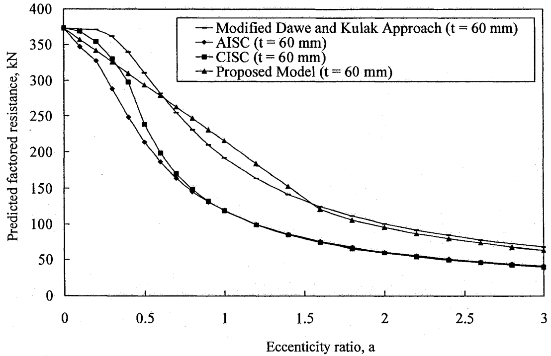
Figure D.4 Predicted capacity versus eccentricity ratio for t = 60 mm and D = 12 mm
