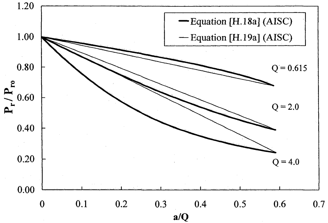
Figure C.3 – Comparison between Equations [C.18a] and [C.19a]
