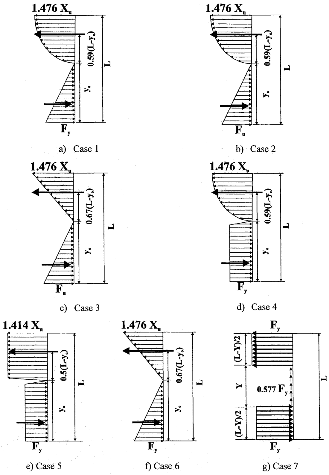
Figure 4.5 – Stress distributions proposed by Neis (1980)
