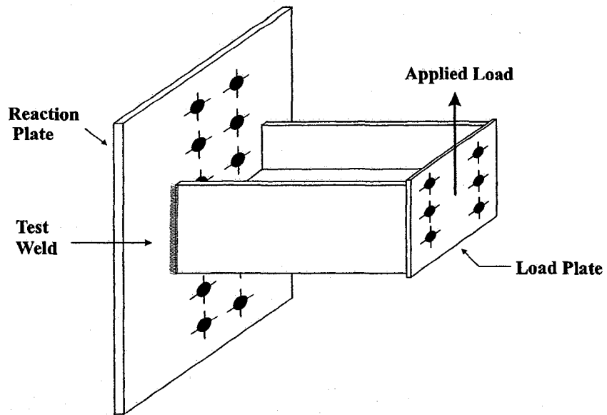
Figure 3.1 – Typical test specimen used in Dawe and Kulak (1972) test program
