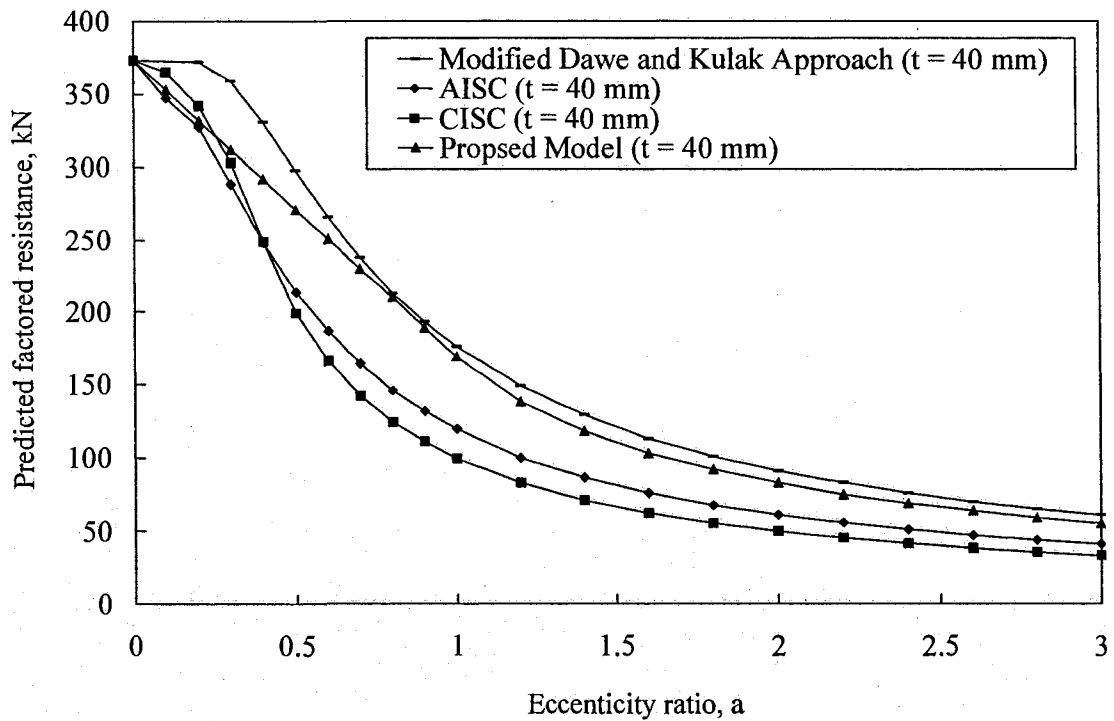
Figure D.3 Predicted capacity versus eccentricity ratio for t = 40 mm and D = 12 mm
