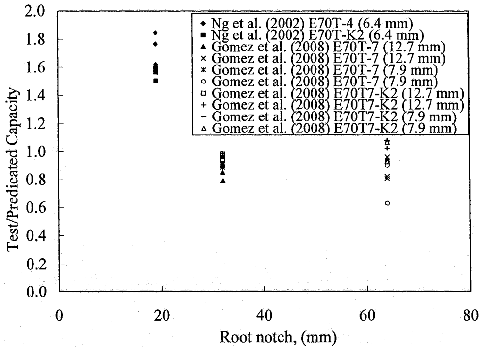
Figure 3.9 – Test-to-predicted ratio versus root notch of cruciform specimens
