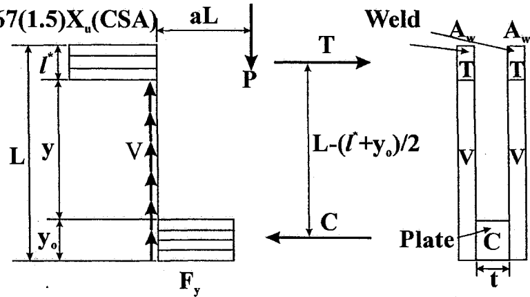
Figure C.2 – Flexure Model for Small Load Eccentricity
