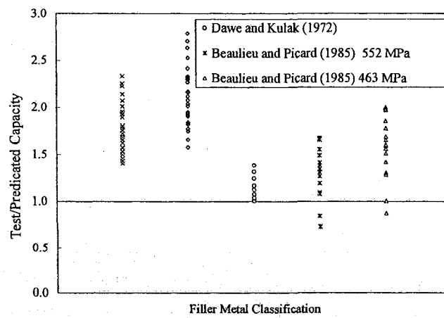
f) Test-to-predicted ratio versus filler metal classification
