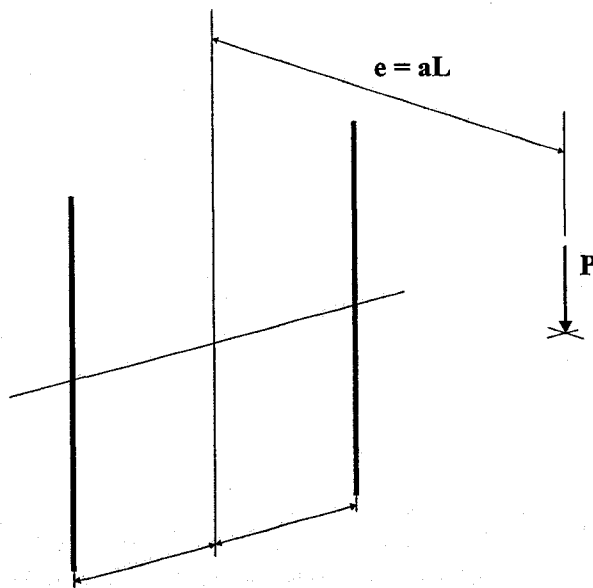
Figure 4.4 – Out-of-plane eccentricity
