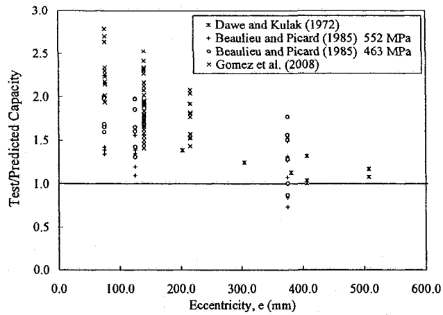
d) Test-to-predicted ratio versus eccentricity
