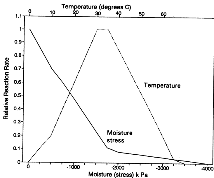
Figure 2. Relative reaction rates for organic matter decomposition at various stresses and temperatures (1 kPa = 0.01 bar).
