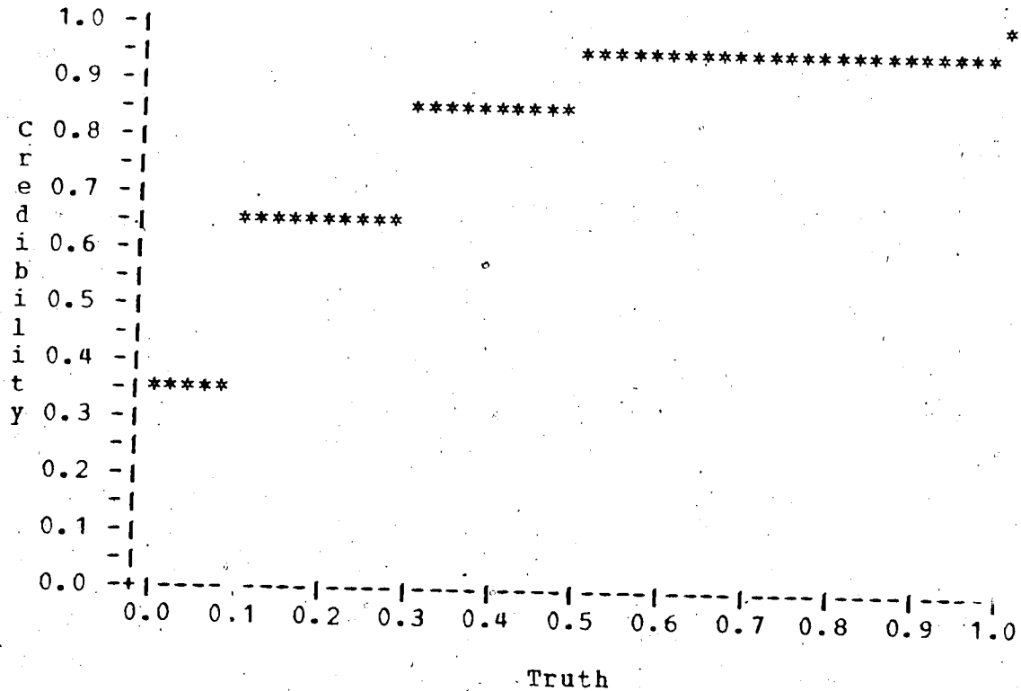
Figure 2.8 A discrete cumulative credibility distribution
