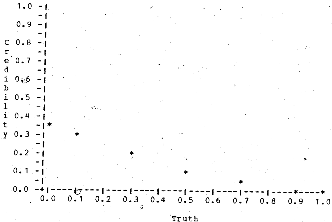
Figure 2.7. A discrete credibility distribution
