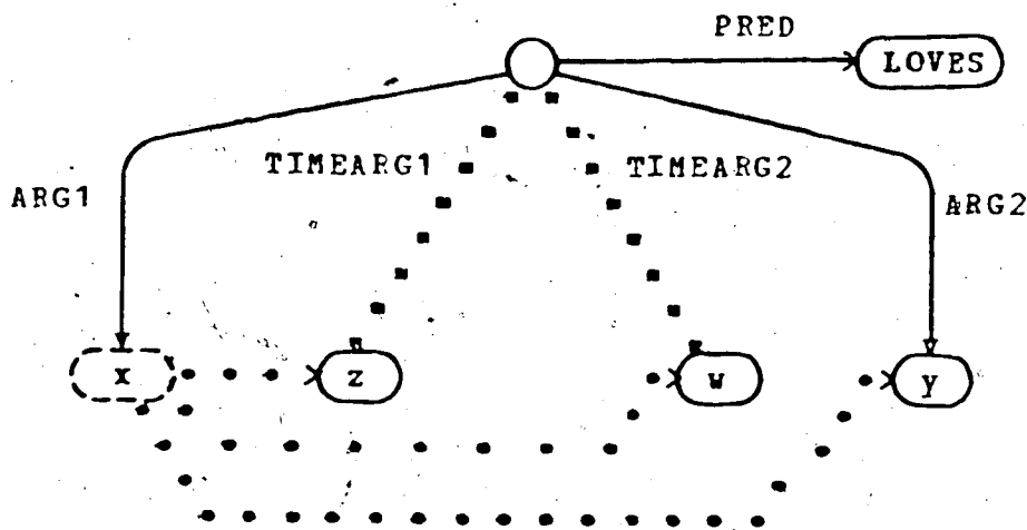
Figure 2.6. \forall x \exists y \exists z \exists w [x \text{ LOVES} \langle z, w \rangle y]
