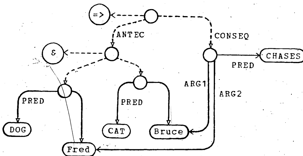
Figure 2.3 [[[Fred\ DOG] \ \& \ [Bruce\ CAT]] \Rightarrow [Fred\ CHASES\ Bruce]]
