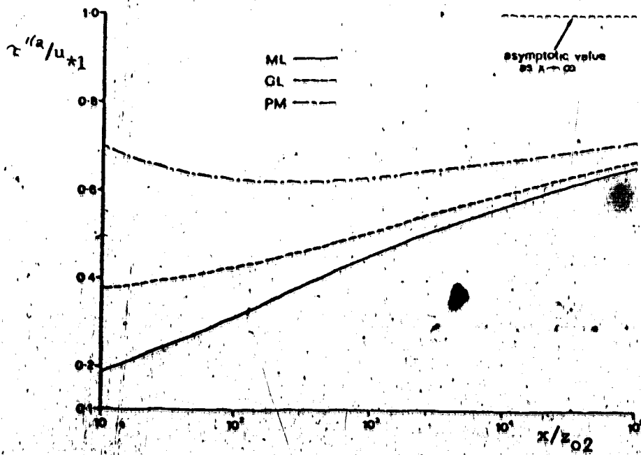
(b) Rough-to-smooth flow, M=3
