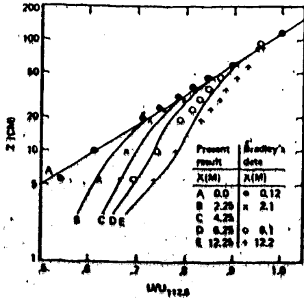
(c) Wind profiles for rough-to-smooth flow
