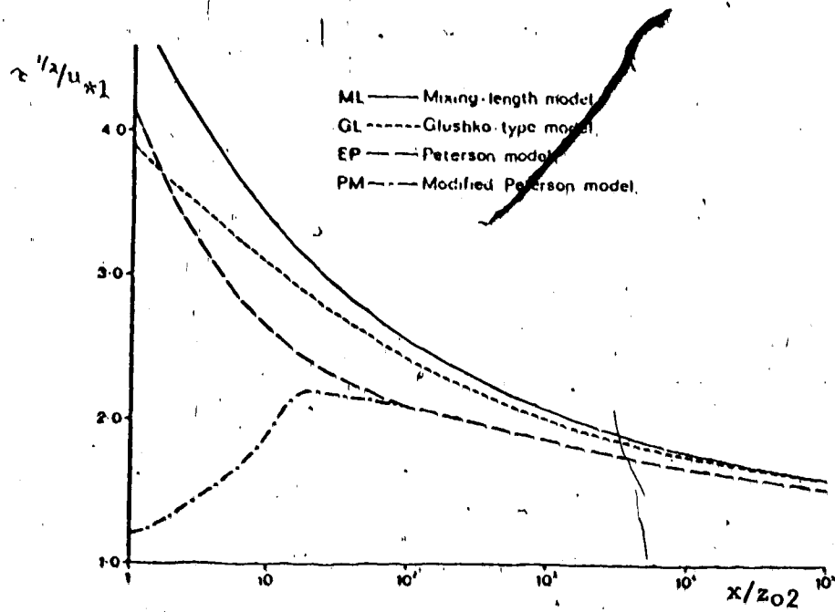
(a) Smooth-to-rough flow, M=5
