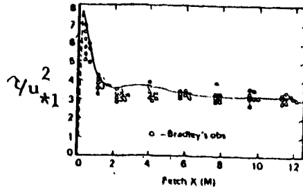
(b) Variation of surface shear stress for smooth-to-rough flow
