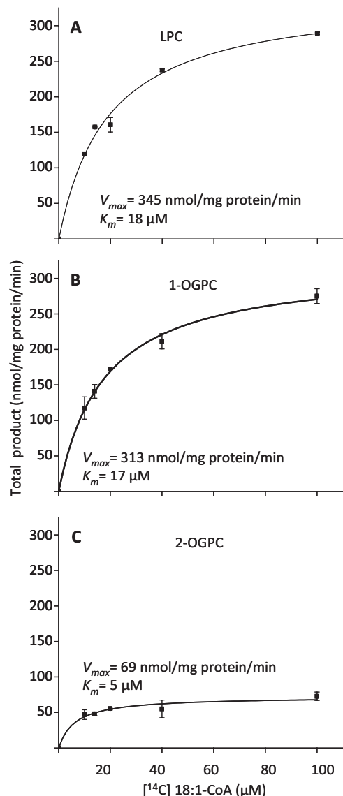
FIGURE 4. Kinetics of acylation of different acyl acceptors using [ ^{14}\text{C} ]18:1-CoA as an acyl donor, catalyzed by AtLPCAT1. LPC, sn -1-18:1-LPC; 1-OGPC, sn -1-O-(9- cis -octadecenyl)- sn -glycero-3-phosphocholine; 2-OGPC, sn -2-O-(9- cis -octadecenyl)- sn -glycero-3-phosphocholine. Assays were performed as described for the forward reaction under "Experimental Procedures" with acyl-CoA concentrations as indicated in the figure. The results presented are from duplicate assays \pm S.D.
