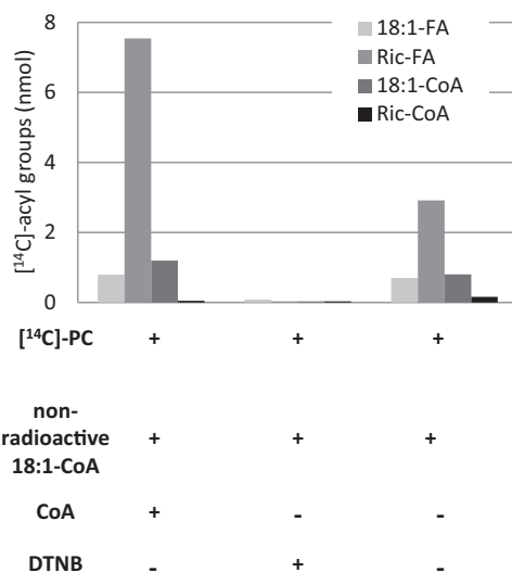
FIGURE 6. Quantification of products of the reverse reactions of AtLPCAT2 with an equimolar mixture of sn -1-16:0- sn -2- ^{14}\text{C} ]18:1-PC and sn -1-16:0- sn -2- ^{14}\text{C} ]ricinoleoyl-PC. Assays were performed as described for LPCAT reverse reaction conditions (see "Experimental Procedures") with the additions and omissions indicated in the figure. DTNB was used at a concentration of 0.5 mM. Incubation time was 1 h. Four assays were pooled for extraction and separation of lipids. Ric, ricinoleoyl; FA, free fatty acids.
