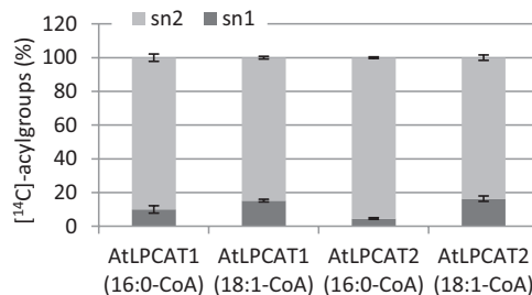
FIGURE 5. Relative incorporation of [ ^{14}\text{C} ]16:0 and [ ^{14}\text{C} ]18:1 from acyl-CoA into the different sn positions of PC by AtLPCAT1 and AtLPCAT2 in absence of LPC. Incubations were performed as assays for the reverse reaction (see "Experimental Procedures") but in the absence of added nonradioactive acyl-CoA during 30 min with 22 \mu\text{g} of yeast microsomal protein. The total amounts of radioactive acyl groups incorporated into PC per assay were for LPCAT1, 1.1 and 4.3 nmol for [ ^{14}\text{C} ]16:0-CoA and [ ^{14}\text{C} ]18:1-CoA substrates, respectively, and 2.8 and 5.4 nmol for LPCAT2, respectively. PC from six assays was pooled before lipase treatment, and the data presented were from duplicates of such pooled samples \pm S.D.
