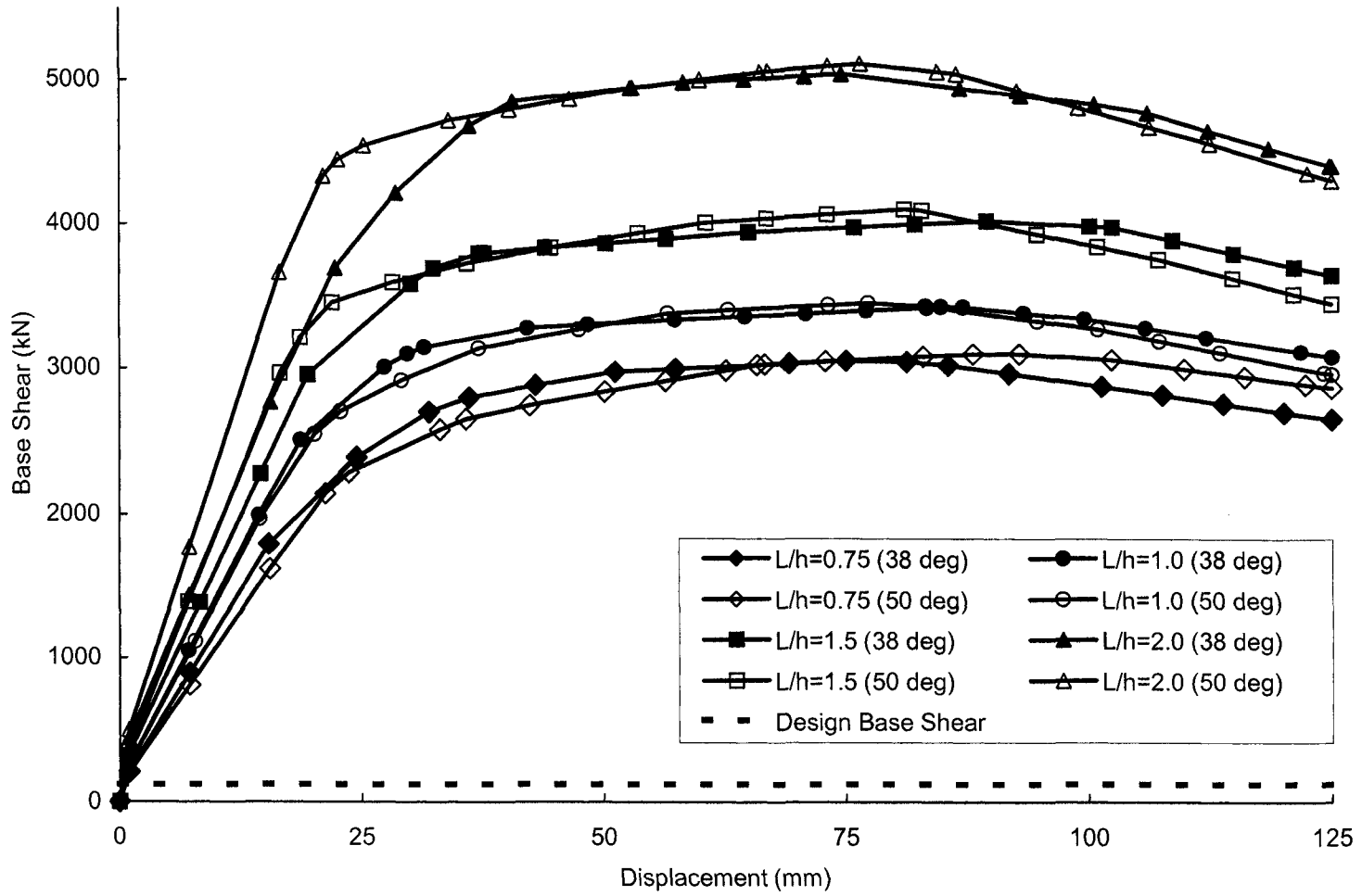
Figure 6.2 - Response Curves for Group 1-A Models
