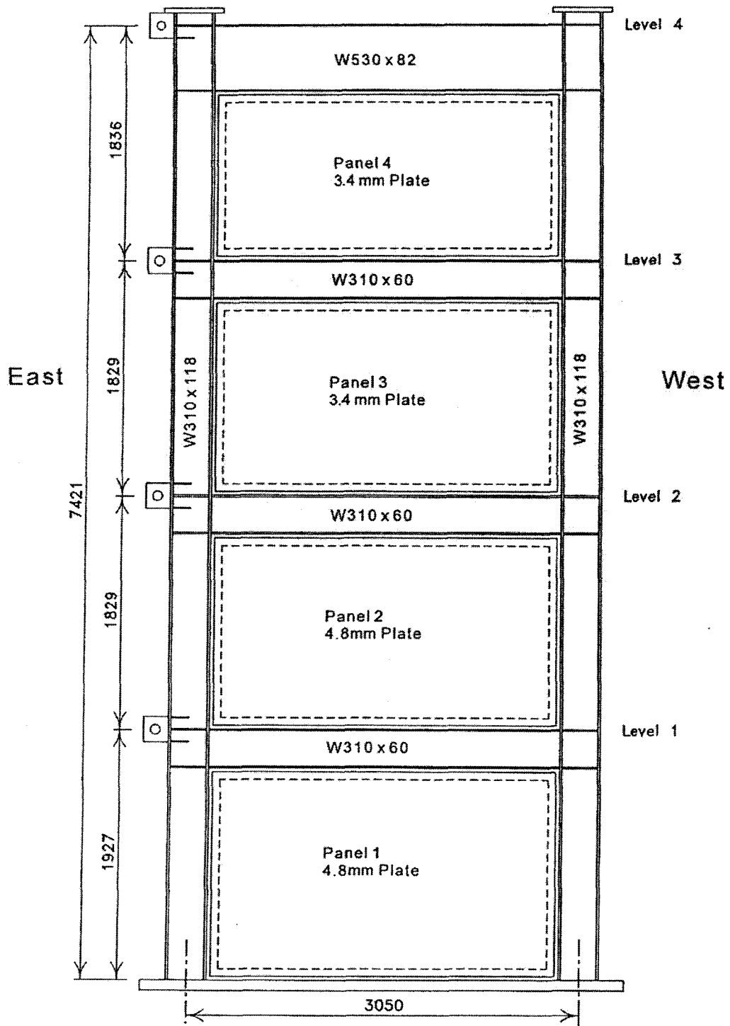
Figure 2.6 - Four-Storey Test Specimen (Driver et al. 1997; 1998a)
