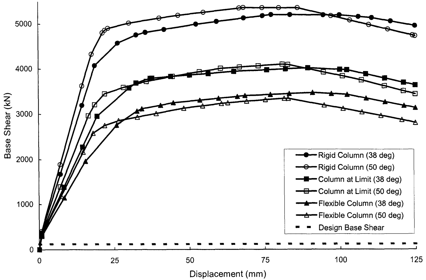
Figure 6.3 - Response Curves for Group 1-B Models
