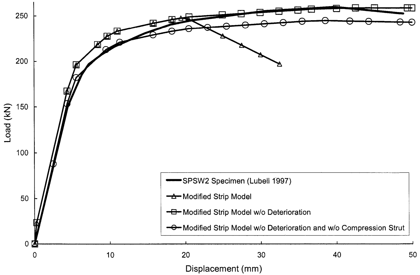
Figure 5.4 - Response Curves for SPSW2 (Lubell 1997) Specimen and Various Modified Strip Models
