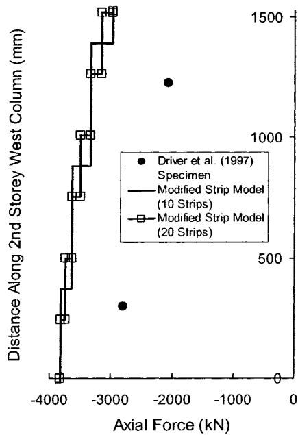
Figure A.11 - Second-Storey West Column Axial Forces
