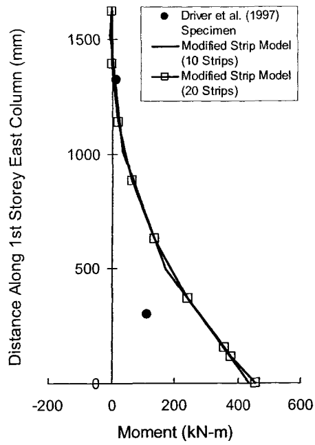
Figure A.2 - First-Storey East Column Moments
