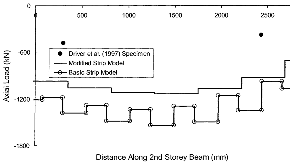
Figure 4.19 - Second-Storey Beam Axial Forces
