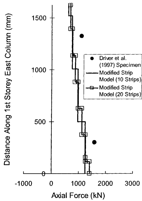
Figure A.8 - First-Storey East Column Axial Forces
