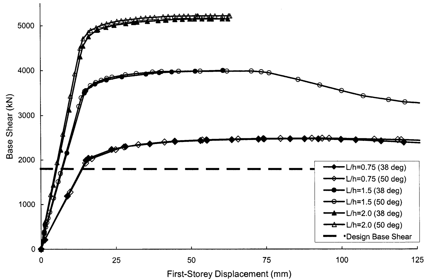
Figure 6.10 - Response Curves for Fifteen-Storey Models
