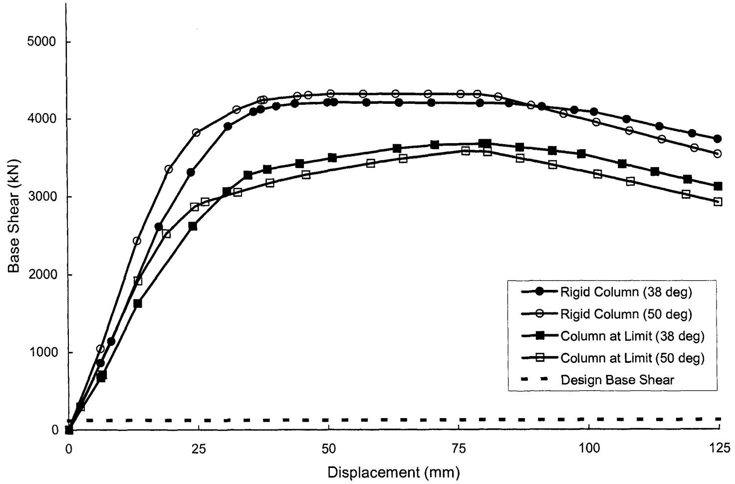
Figure 6.5 - Response Curves for Group 1-D Models
