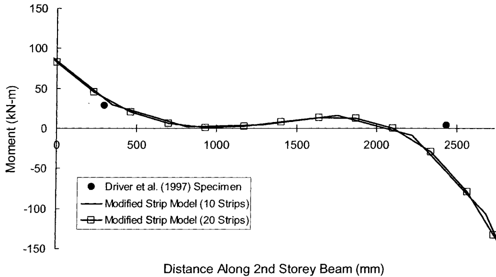
Figure A.7 - Second-Storey Beam Moments
