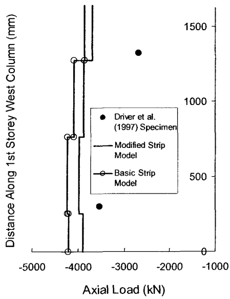
Figure 4.15 - First-Storey West Column Axial Forces
