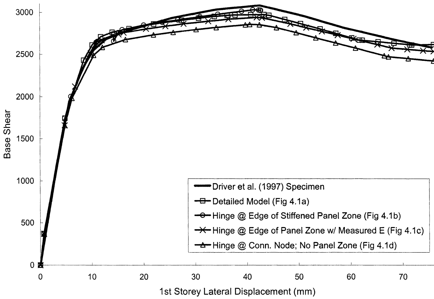
Figure 4.2 - First-Storey Response Curves for Alternative Frame-Joint Arrangements, Detailed Model, and Driver et al. (1998a) Specimen
