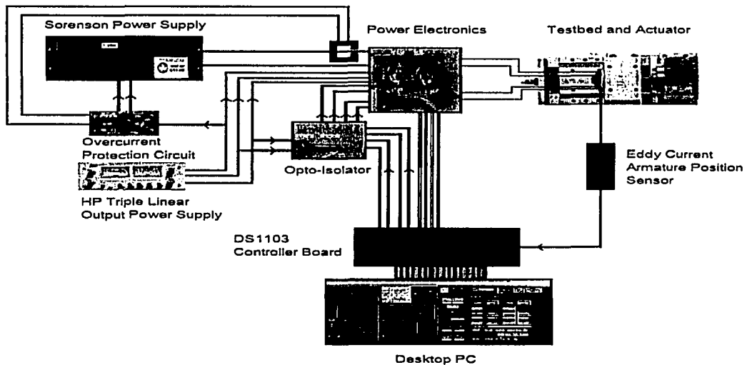
Figure 4.15: Experimental testbed setup schematic
