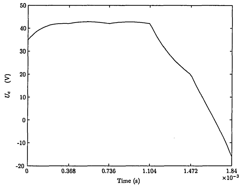
Figure 3.16: Reference coil voltage ( U_c )
