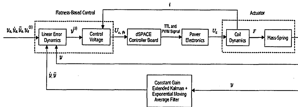
Figure 5.1: Scheme of flatness-based voltage end-control with estimation of state variables
