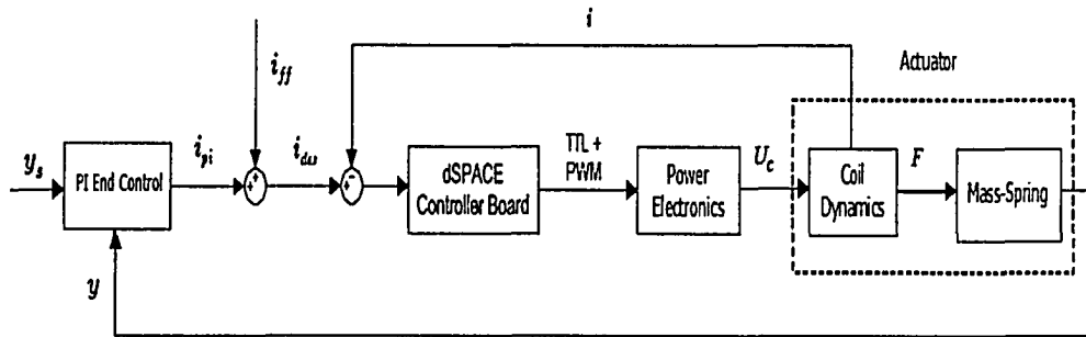
Figure 5.18: Scheme of proportion-integral current end-control for real-time implementation
