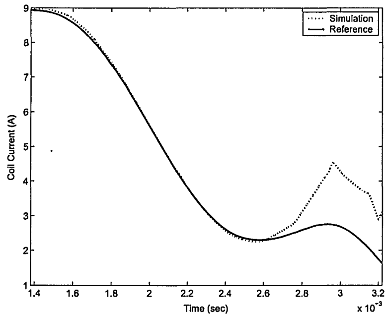
Figure 5.7: Desired and simulated coil current
