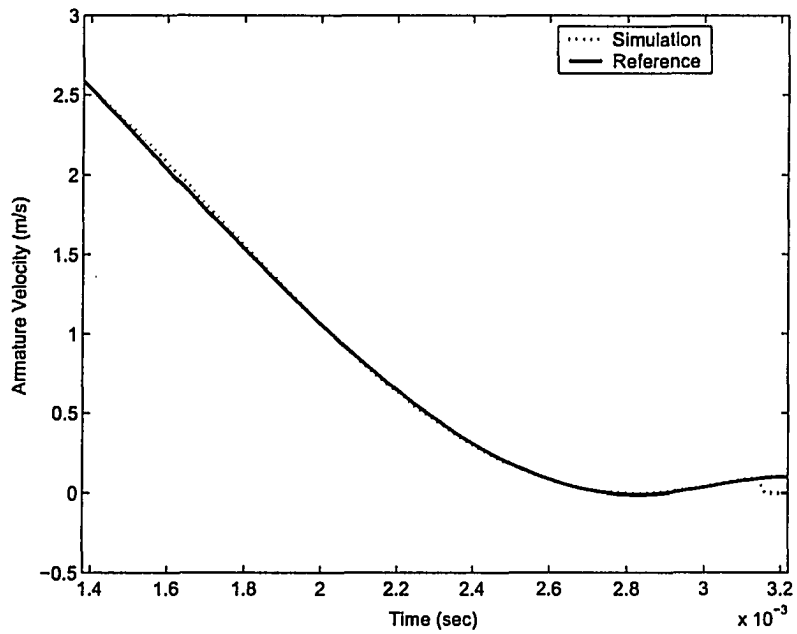
Figure 5.5: Desired and simulated armature velocity
