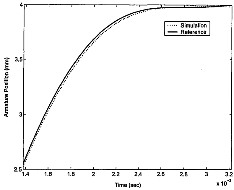
Figure 5.4: Desired and simulated armature position
