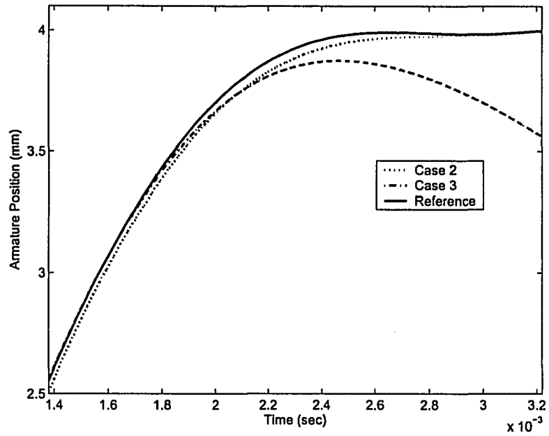
Figure 5.10: Desired and simulated armature position (Case 2 and 3)
