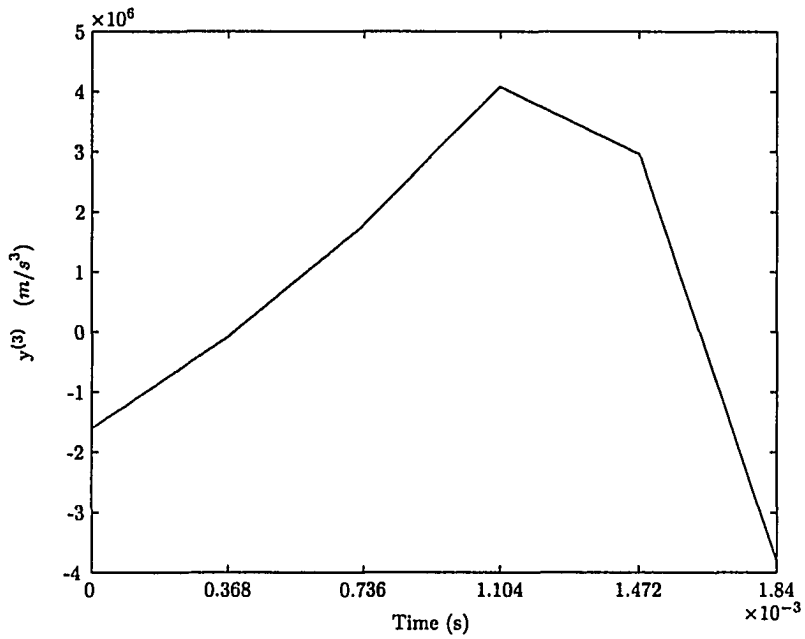
Figure 3.14: Reference armature jerk ( y_d^{(3)} )
