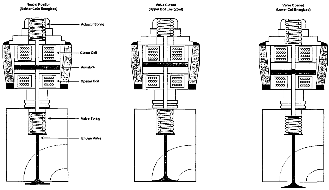
Figure 2.3: Typical operation of a two spring solenoid actuator valve
