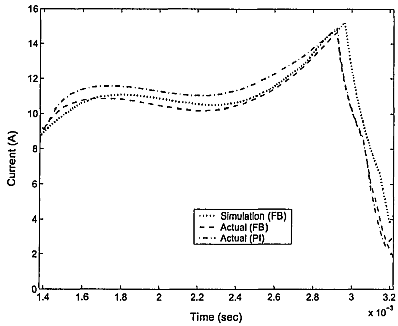
Figure 5.23: Simulated and experimental results for current
