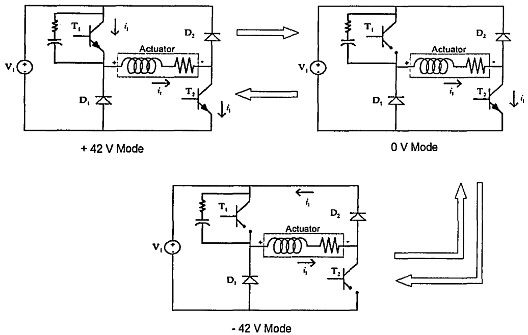
Figure 4.14: Power electronics output modes
