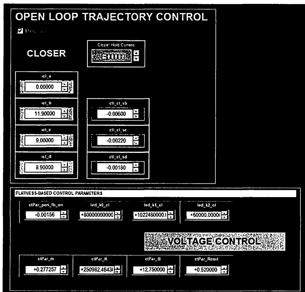
Figure 5.17: Approach control and flatness-based end-control parameter inputs in ControlDesk
