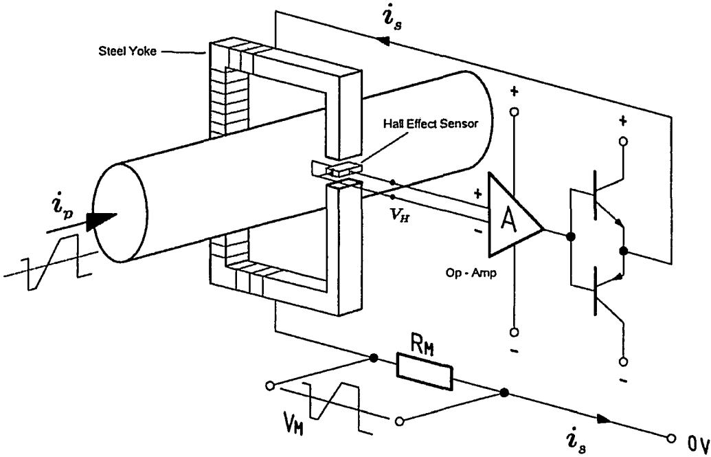
Figure 4.11: Schematic of hall-effect current sensor
