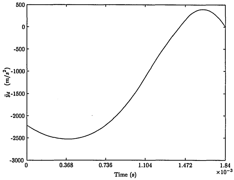
Figure 3.13: Reference armature acceleration ( \ddot{y}_d )
