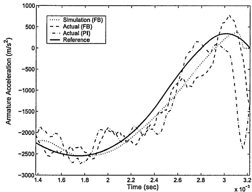
Figure 5.22: Desired, simulated and experimental results for armature acceleration
