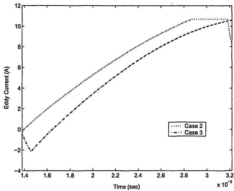
Figure 5.14: Simulated eddy currents (Case 2 and 3)
