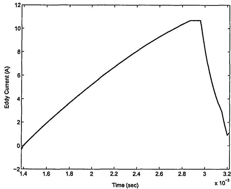
Figure 5.8: Simulated eddy currents
