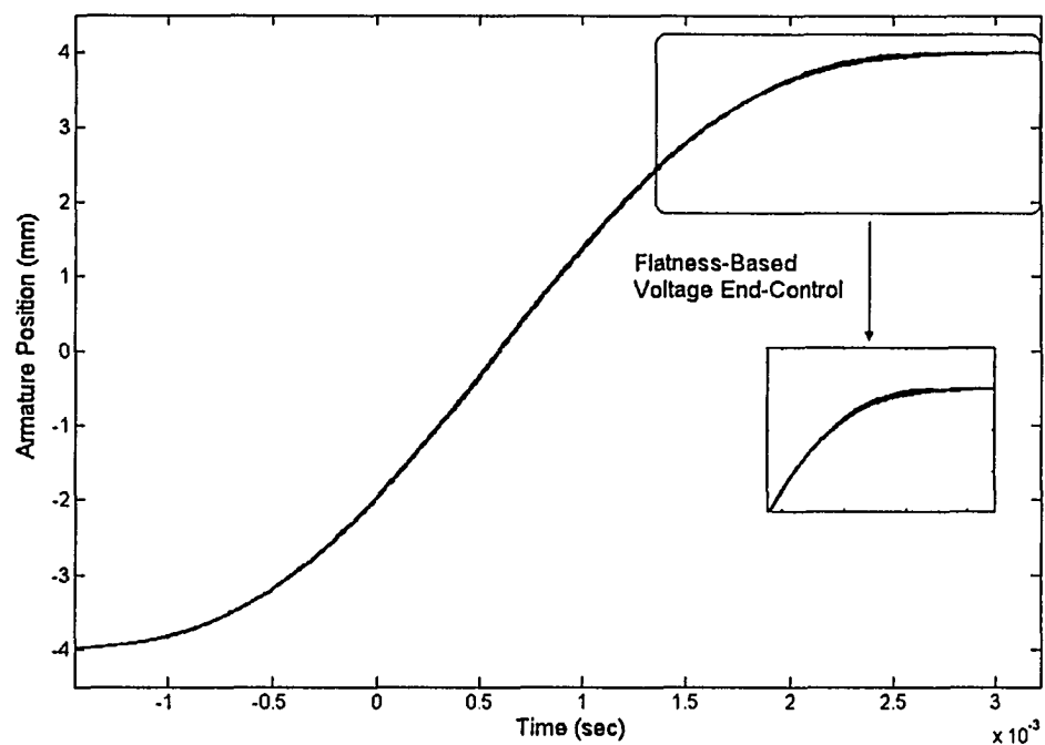
Figure 5.25: 50 cycles of experimental armature position data for flatness-based voltage end-control
