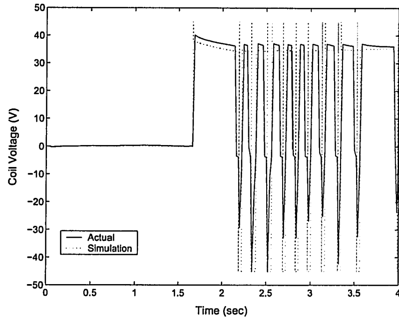
Figure 5.3: Actual and simulated power electronics output voltages
