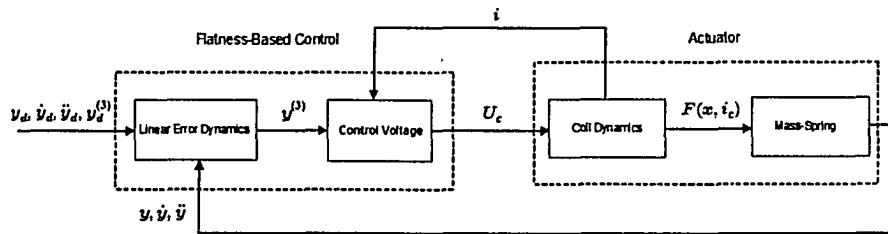
Figure 3.7: Scheme of the flatness-based end-control loop for the actuator
