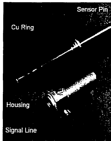
Figure 4.12: Eddy current type lift sensor
