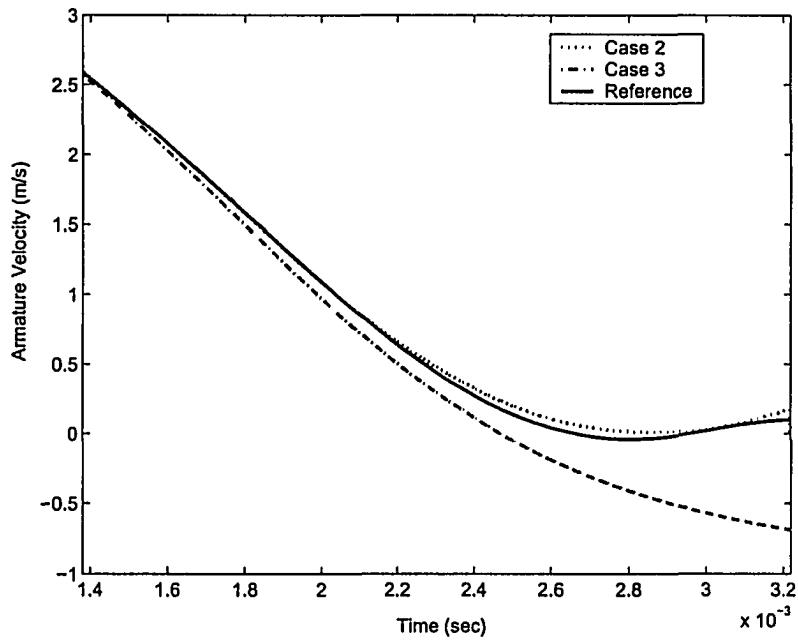
Figure 5.11: Desired and simulated armature velocity (Case 2 and 3)
