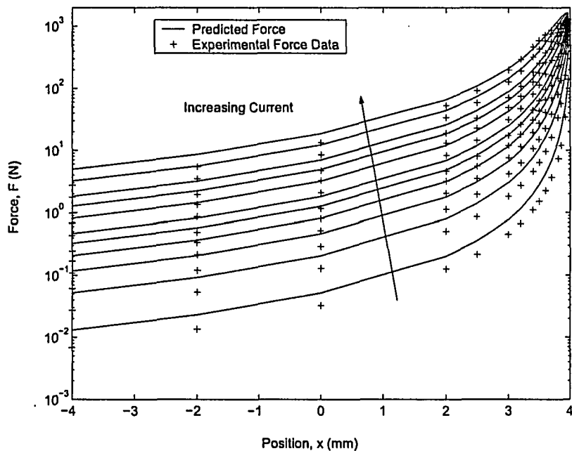
Figure 3.3: Comparison of (3.6) with experimental force
