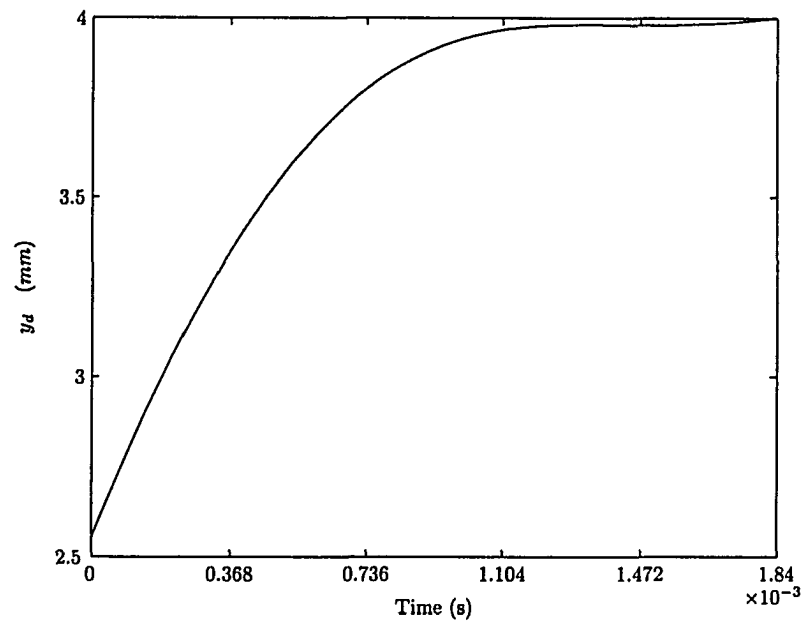
Figure 3.11: Reference armature position ( y_d )
