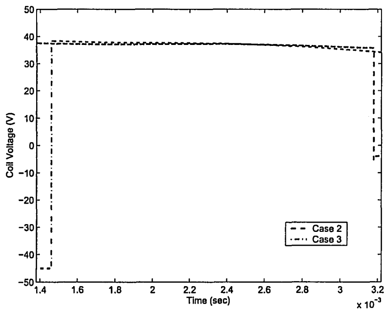
Figure 5.15: Simulated coil voltage input (Case 2 and 3)
