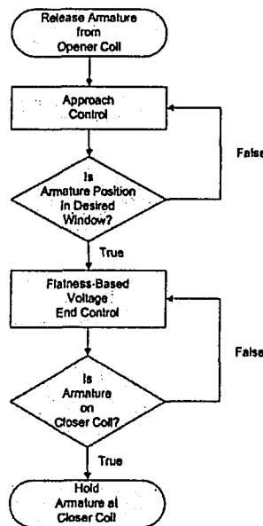
Figure 5.16: Control algorithm for flatness-based voltage end-control
