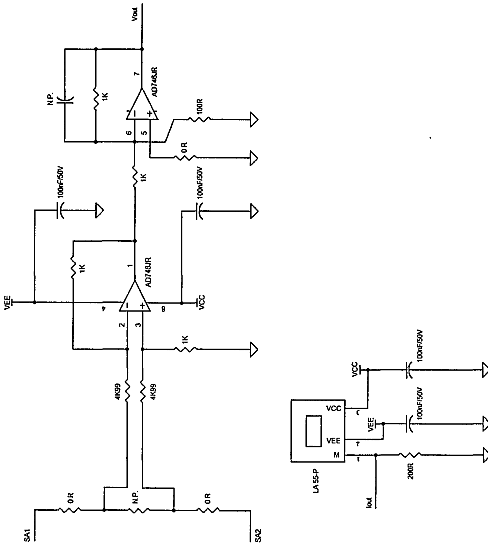
Figure B.3: Onboard power electronics current-voltage sensing
