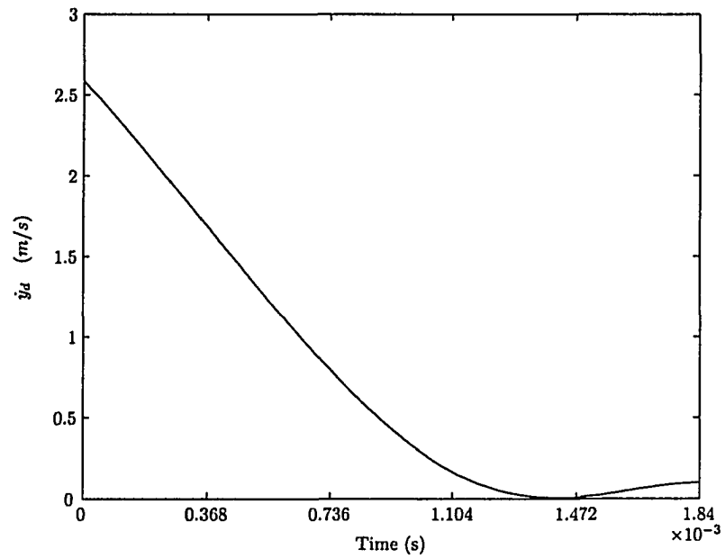
Figure 3.12: Reference armature velocity ( \dot{y}_d )
