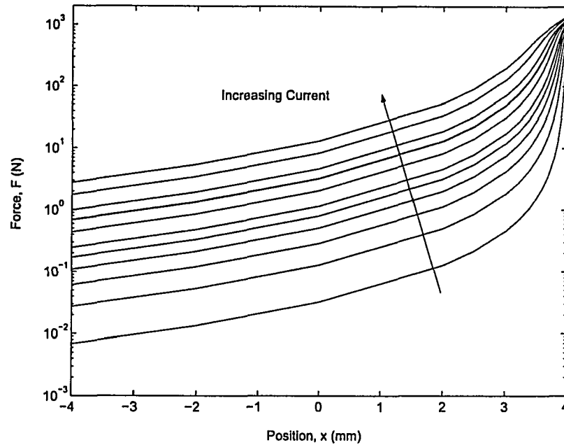
Figure 3.2: Experimental force versus position for varying current
