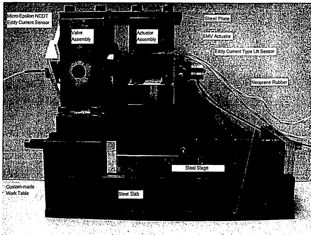
Figure 4.6: Testbed setup
