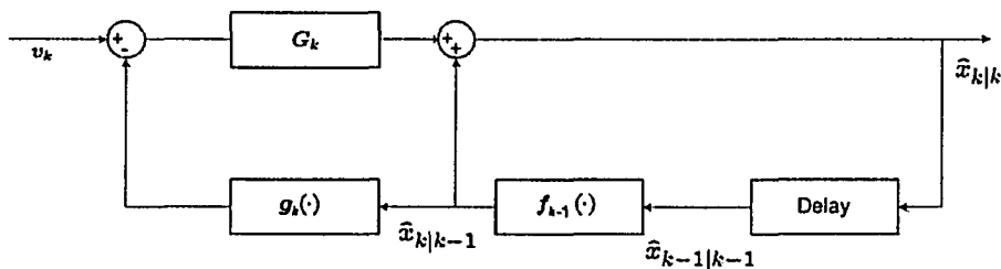
Figure A.1: Block diagram of Kalman filter algorithm
