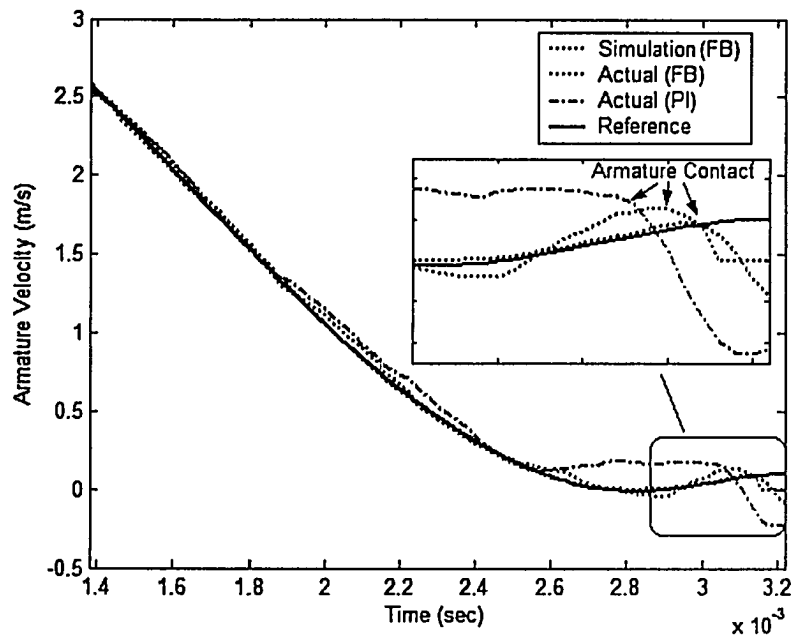
Figure 5.21: Desired, simulated and experimental results for armature velocity
