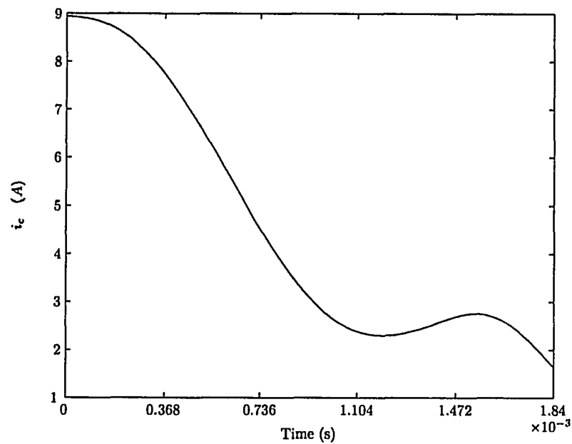
Figure 3.15: Reference coil current ( i_c )
