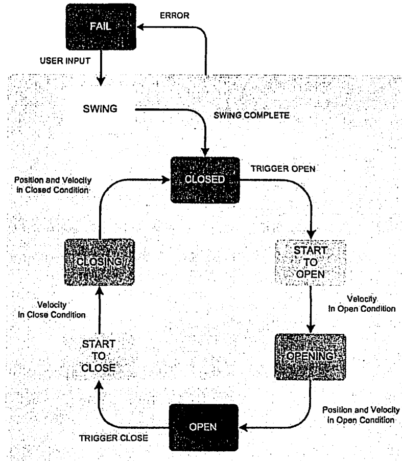
Figure C.2: Control state machine
