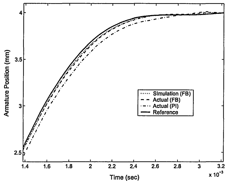
Figure 5.20: Desired, simulated and experimental results for armature position
