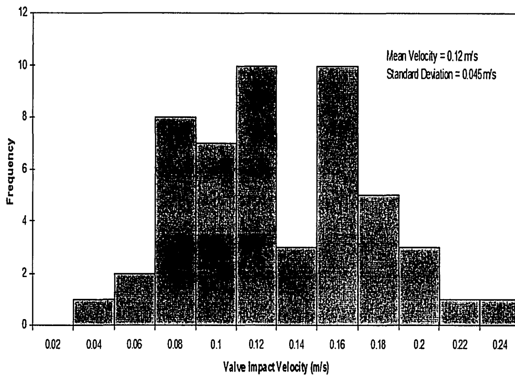
Figure 5.27: Distribution of armature impact velocity for 50 cycles using proportional-integral current end-control
