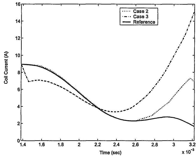
Figure 5.13: Desired and simulated coil current (Case 2 and 3)
