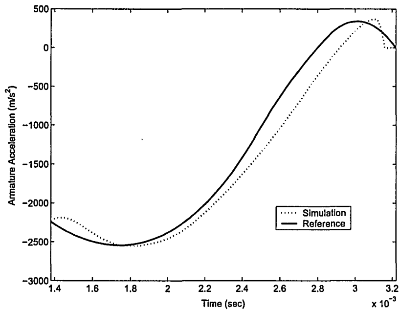
Figure 5.6: Desired and simulated armature acceleration
