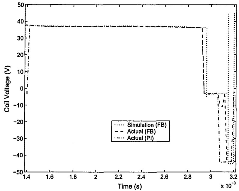
Figure 5.24: Simulated and experimental results for coil voltage
