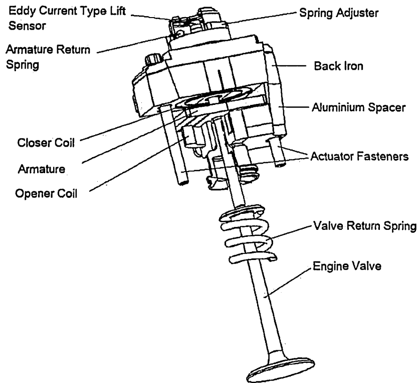
Figure 4.2: TEMIC actuator and valve sectional view [Chladny, 2003]
