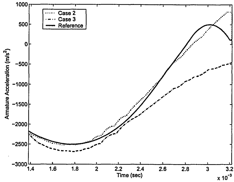
Figure 5.12: Desired and simulated armature acceleration (Case 2 and 3)
