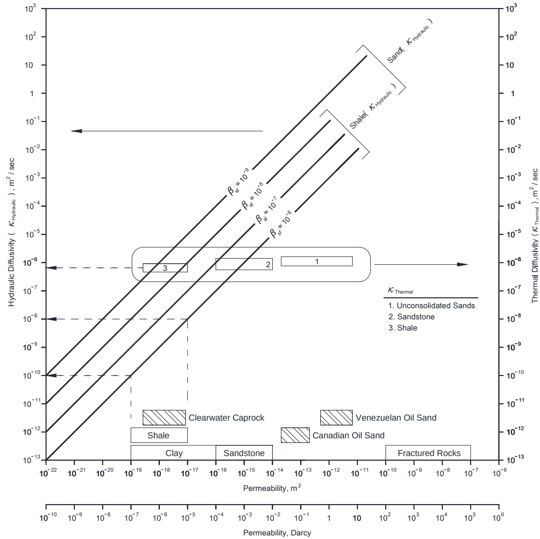
Figure 4.47. Variation of hydraulic diffusivity ( \kappa_{Hydraulic} ) and thermal diffusivity ( \kappa_{Thermal} ) versus formation permeability ( k ) for different compressibility of porous medium ( \beta_{sf} ), and their comparison for shale formations.
