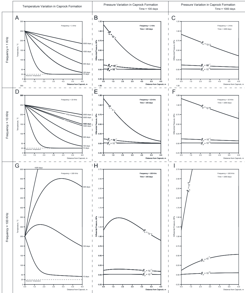
Figure 4.48. Variation of temperature in caprock for different applied frequencies (Section A, D, and G) and induced thermal pressure for different compressibility of porous medium ( \beta_{st} ) (Sections B and C for 1 kHz; Sections E and F for 10 kHz; Sections H and I for 100 kHz). See Table 2.2 for caprock and coil properties.
