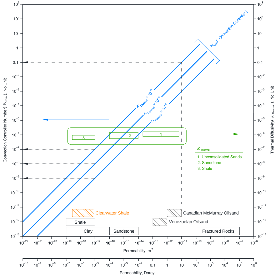
Figure 4.46. Variation of convection controller number ( N_{\text{conv}} ) versus formation permeability ( k ) for different thermal diffusivities ( \kappa_{\text{Thermal}} )
