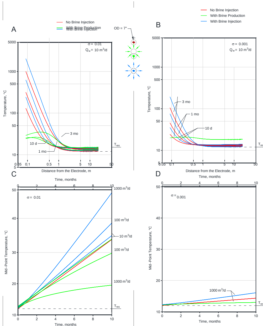
Figure 2.15. Temperature profile versus distance from the electrode for electro-thermal in convective and non-convective heating in lean zones (Section A) and in bitumen rich zones (Section B); and mid-point temperature variation (wells spaced 5 m apart) in lean zones (Section C) and in bitumen rich zones (Section D). See Table 2.1 for electrode and reservoir properties.
