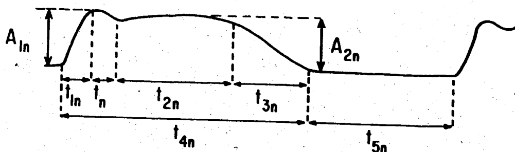
Figure 21: The parameters of the notched control potential used in the analysis of its temperature dependence.
