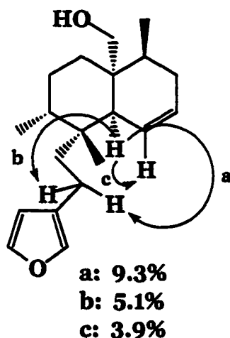
Figure 4. Selected nOe Data of Furyl Alcohol 114
