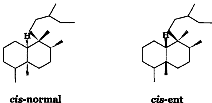
Figure 2. Conformational Structures of cis -Clerodanes
