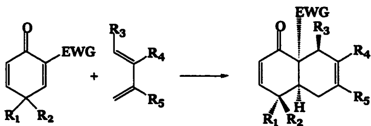
Figure 3. Conceptual Intermolecular Diels-Alder Approach to cis -Normal Clerodanes
