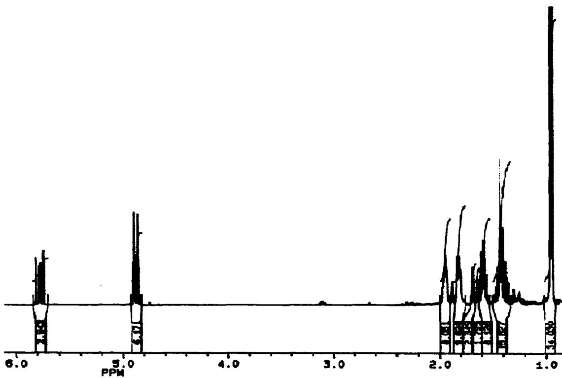
Figure 5. Proton NMR Spectrum of Synthetic 42
