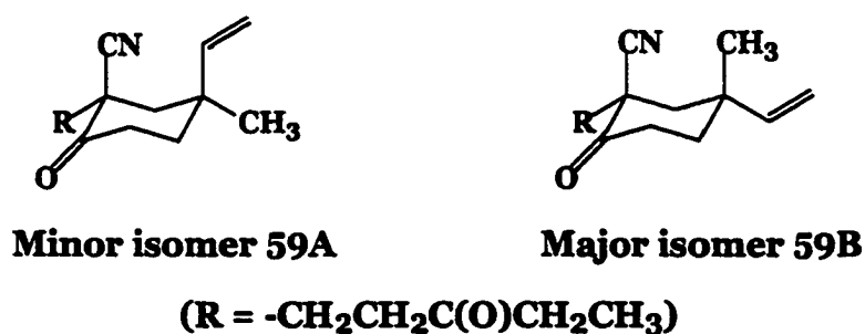
Figure 2. Dominating Conformations of the Isomeric Diketone 59
