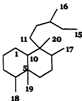
Figure 1. Clerodane Carbon Skeleton
