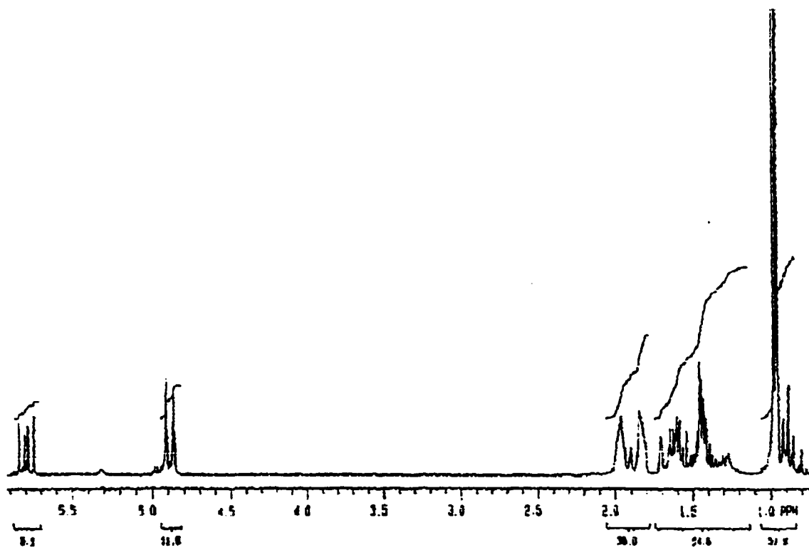
Figure 6. Reported Proton NMR Spectrum of 42
