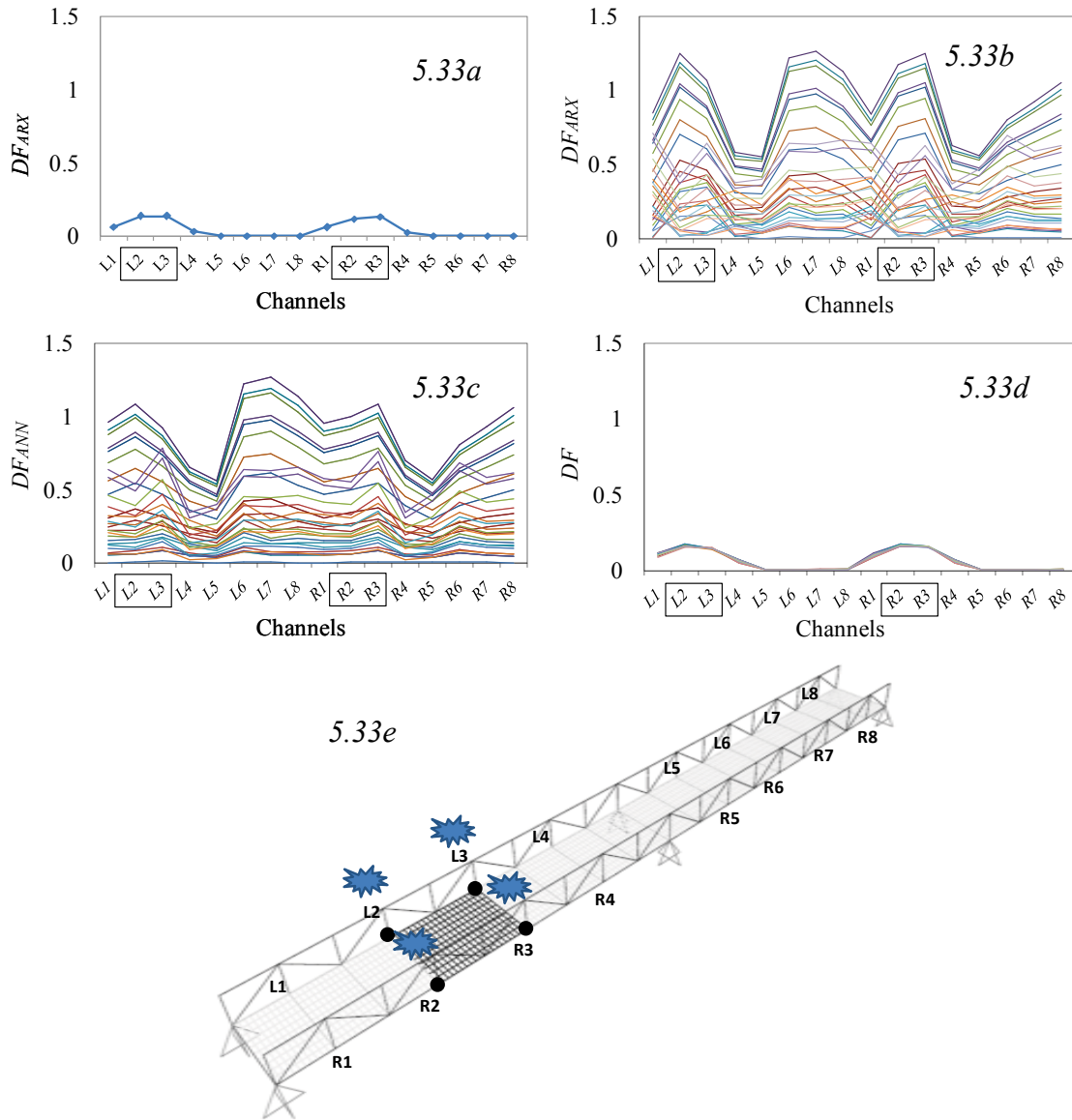
Figure 5.33. DC5 with 0% noise diagrams – (a) DF_{ARX} with damage only; (b) DF_{ARX} with damage and temperature effects; (c) Neural network output ( DF_{ANN} ); (d) Final values of DFs after correction using DF_{ANN} ; (e) Damage location
