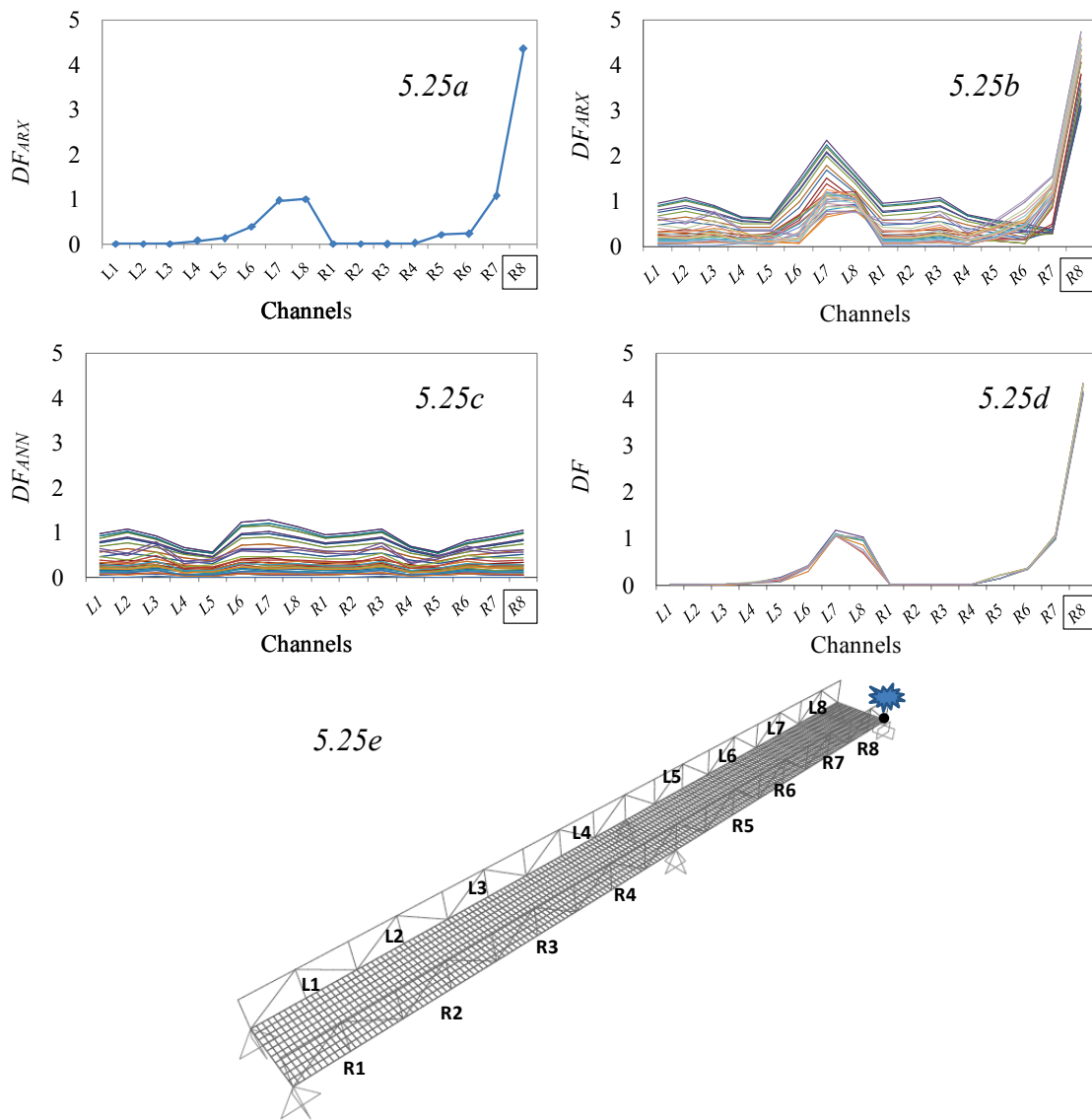
Figure 5.25. DC3 with 0% noise diagrams – (a) DF_{ARX} with damage only; (b) DF_{ARX} with damage and temperature effects; (c) Neural network output ( DF_{ANN} ); (d) Final values of DF s after correction using DF_{ANN} ; (e) Damage location
