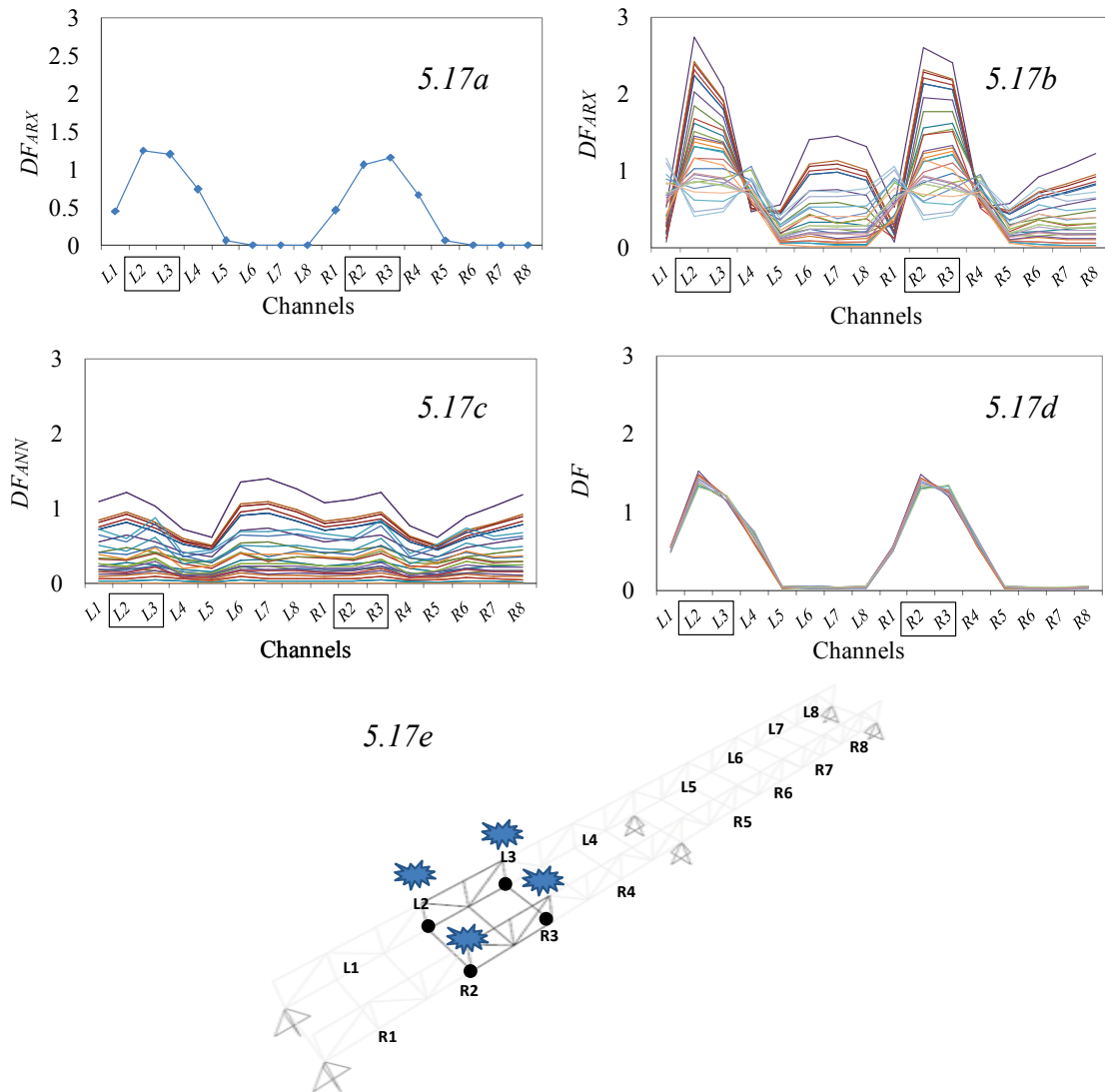
Figure 5.17. DC1 with 0% noise diagrams – (a) DF_{ARX} with damage only; (b) DF_{ARX} with damage and temperature effects; (c) Neural network output ( DF_{ANN} ); (d) Final values of DF s after correction using DF_{ANN} ; (e) Damage location
