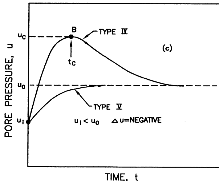
Fig. 5 Idealized pore pressure dissipation response in OC fine grained soil for different measurement locations
