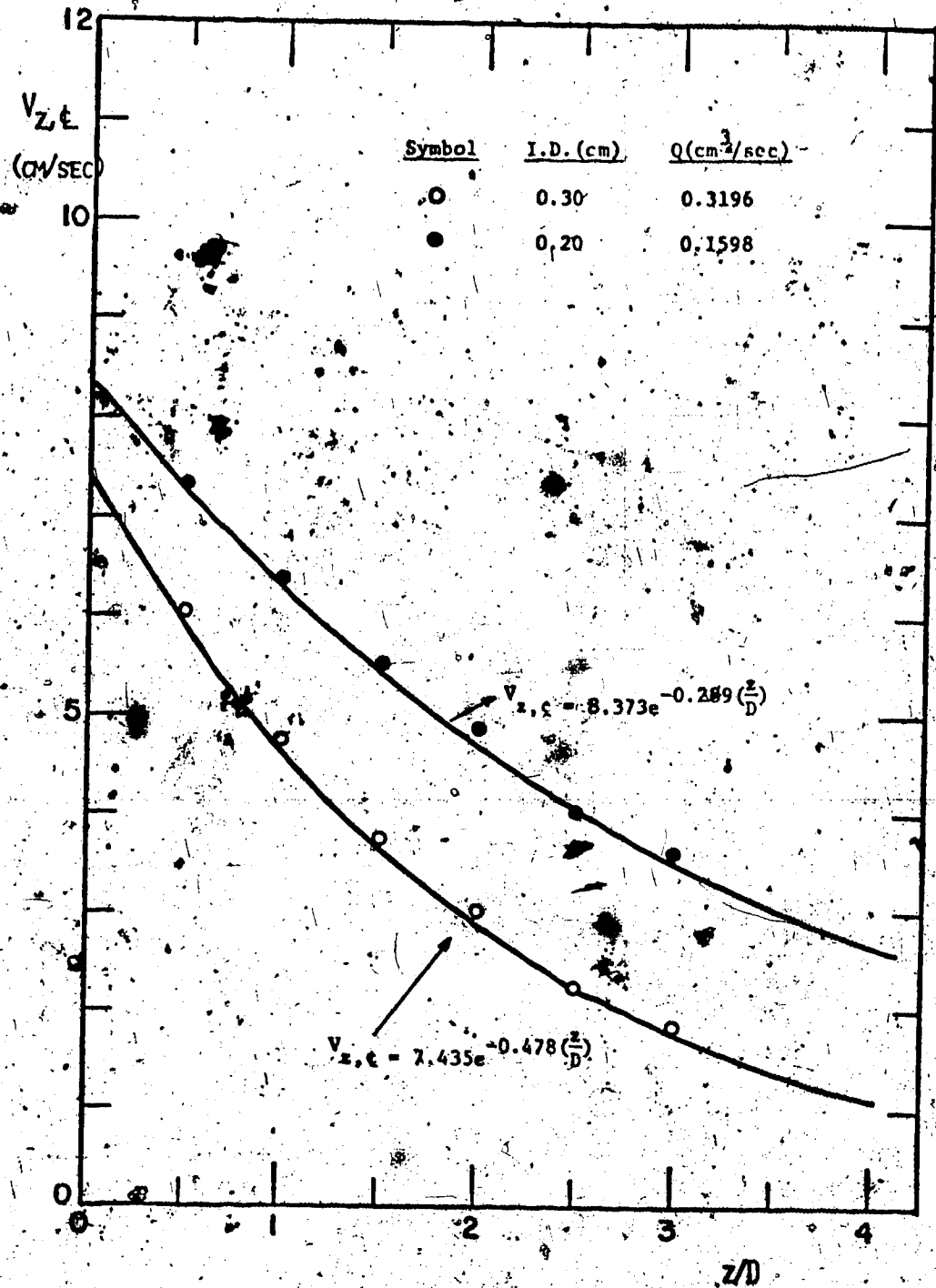
FIGURE IV-23 COMPARISON OF CENTERLINE AXIAL VELOCITY WITH EXPONENTIAL DECAY MODEL
