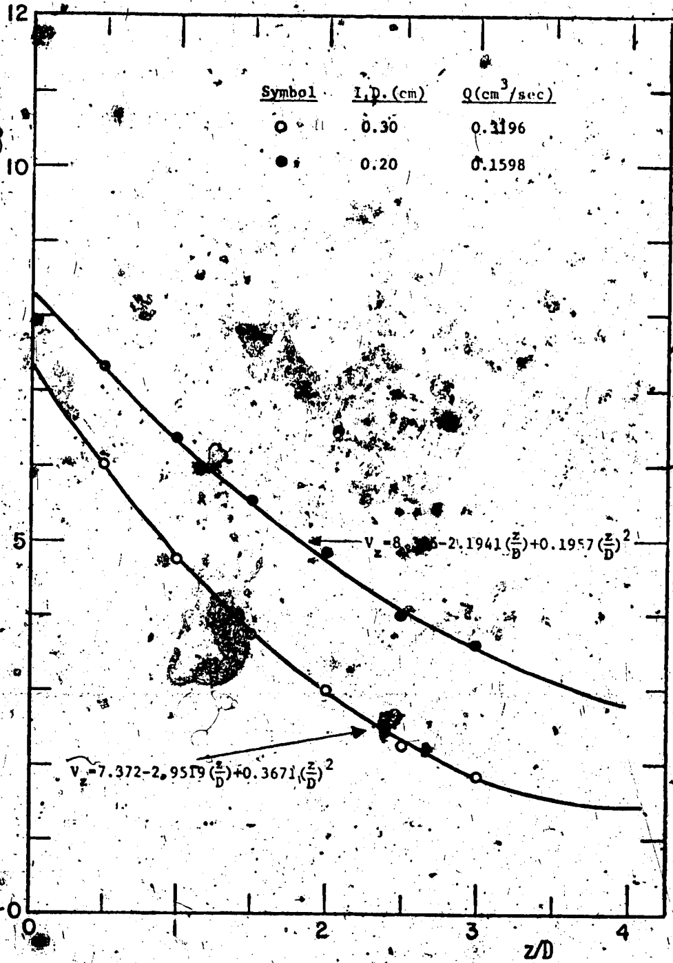
FIGURE IV-15 TYPICAL CENTERLINE AXIAL VELOCITY; K-1 MODEL
