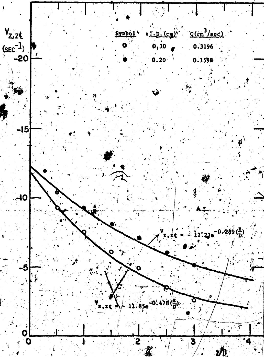
FIGURE IV-24 COMPARISON OF CENTERLINE STRETCH RATE WITH EXPONENTIAL DECAY MODEL
