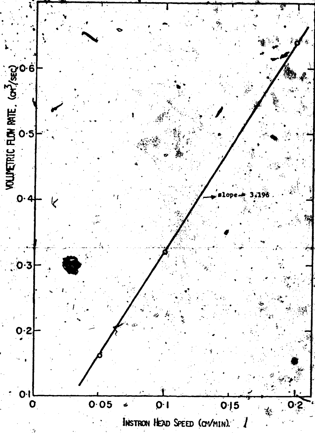
FIGURE A-1 CALIBRATION OF INSTRON HEADSPEED
