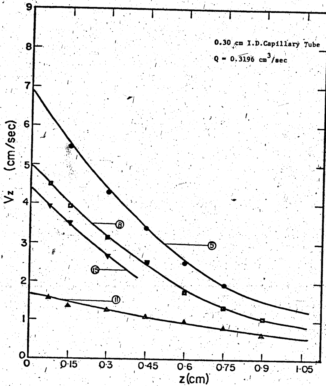
FIGURE III-7 TYPICAL AXIAL VELOCITY - POSITION DATA
