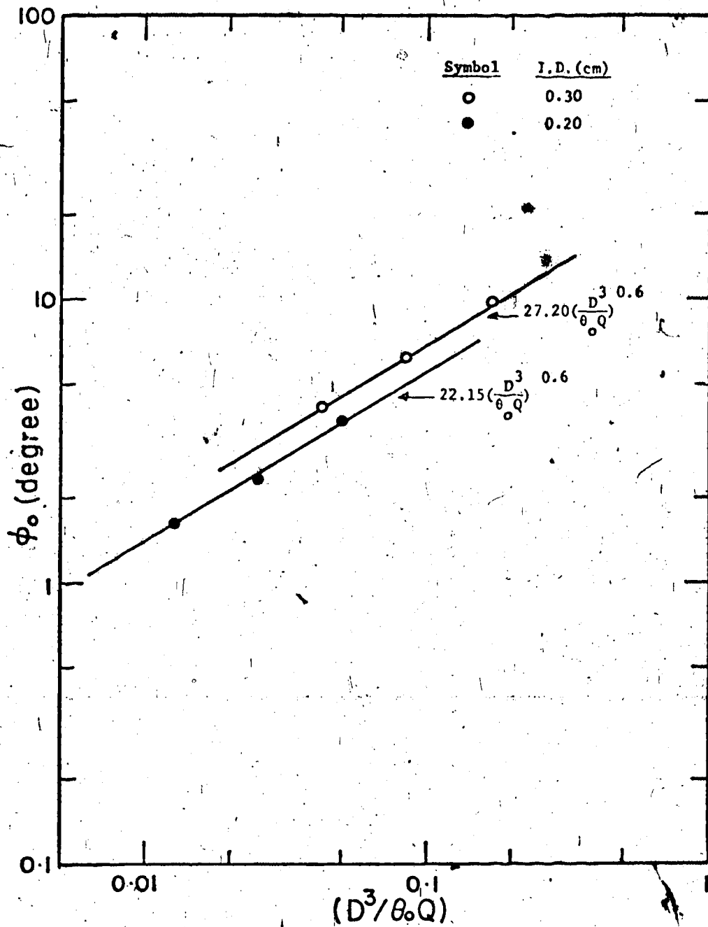
FIGURE IV-5 INITIAL CONE SEMI-ANGLE VERSUS (\frac{D^3}{\theta_0 Q})
