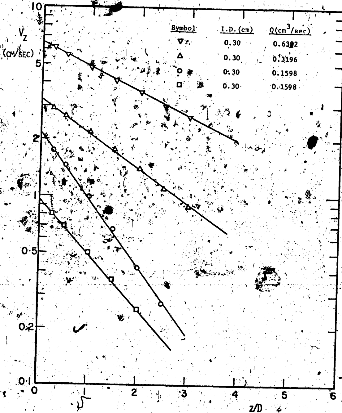
FIGURE IV-19 TYPICAL AXIAL VELOCITY; EXPONENTIAL DECAY MODEL
