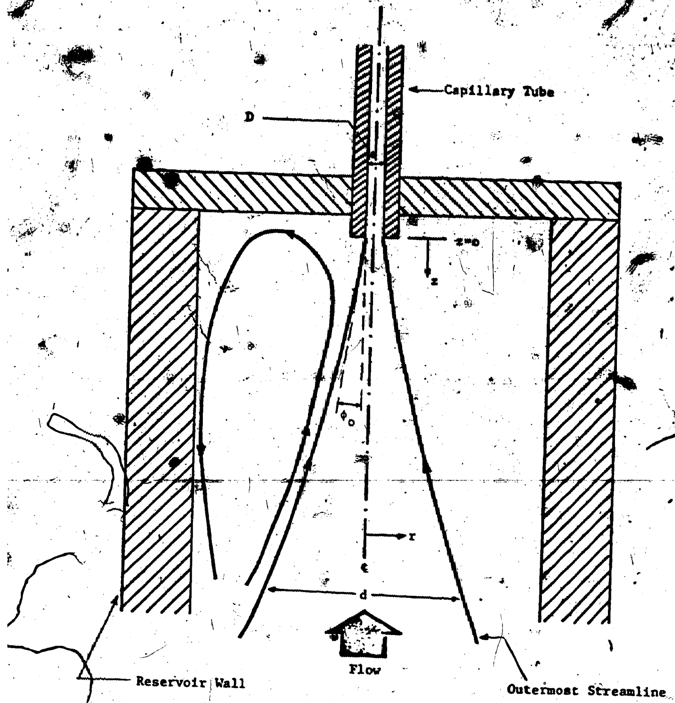
FIGURE 11-2 COORDINATE SYSTEM USED IN ANALYSIS: K-I MODEL
