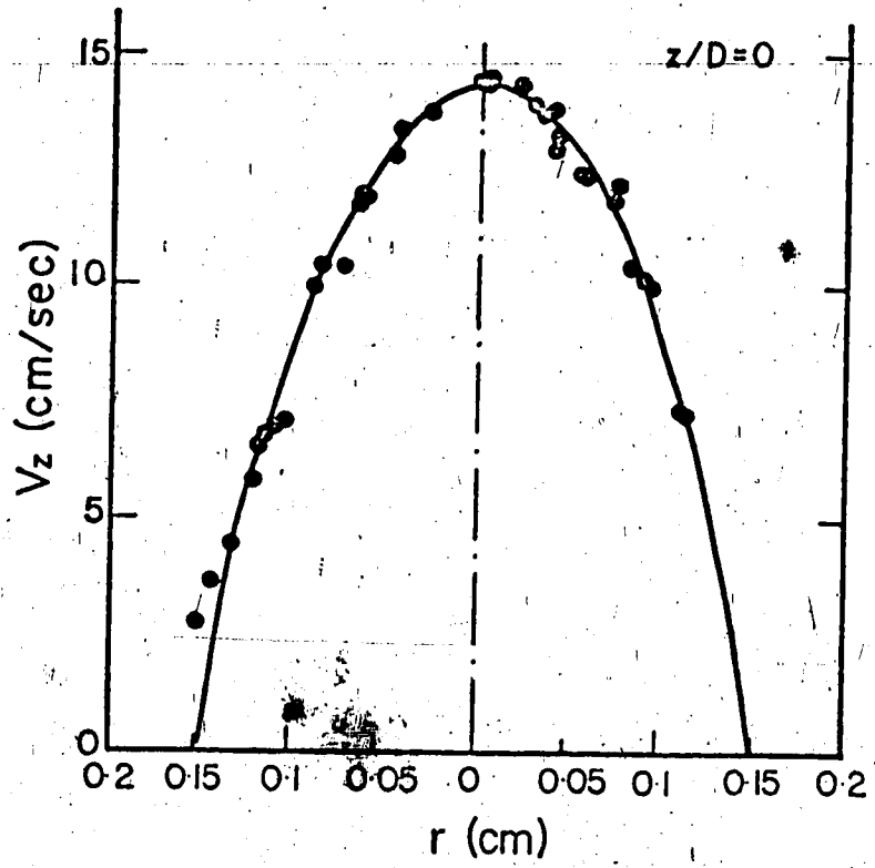
FIGURE IV-2 AXIAL VELOCITY PROFILES, 0.30 CM I.D. CAPILLARY TUBE, Q = 0.6392 \text{ cm}^3/\text{SEC}
