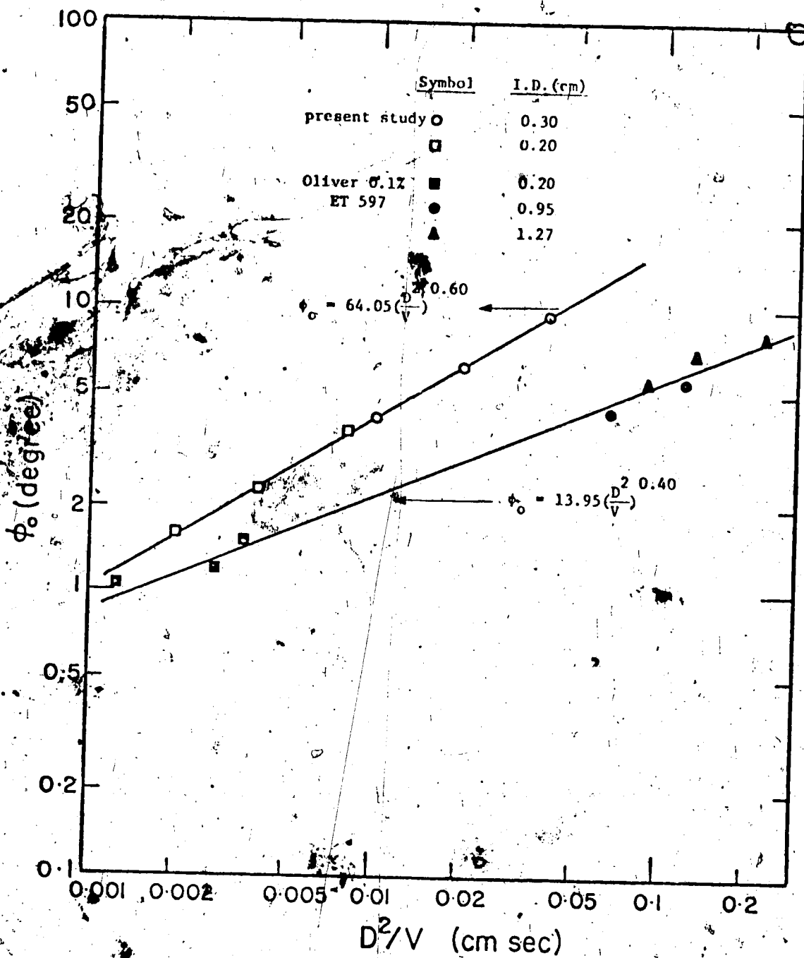
FIGURE IV-7 INITIAL CONE SEMI-ANGLE VERSUS (D^2/V)
