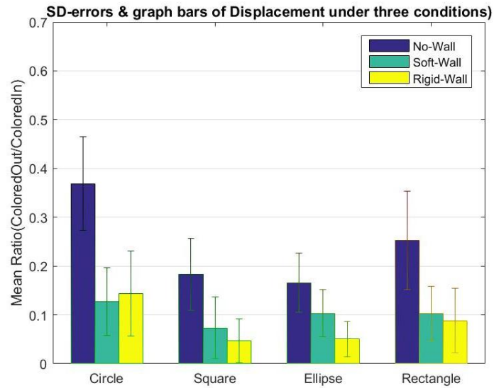
Fig. 4 Illustration of mean variances of the Ratio of the ColoredAreaOut to the ColoredAreaIn under different assistance conditions. The Ratio has significantly decreased by altering from No-walls to either Soft- or Rigid-walls conditions
