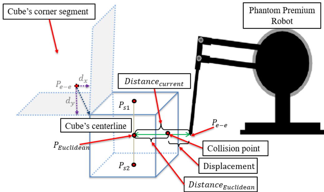
Fig. 3 Illustration of the implementation of the cubical-shaped VF forces when the robot crosses over the ROIs. Two samples points, P_{s1} and P_{s2} , and a sample P_{Euclidean} are shown
