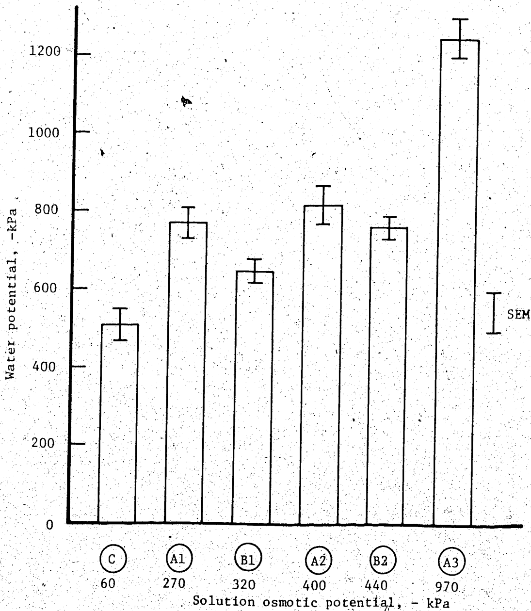
Figure 33. Mean water potential of saltgrass shoots grown at various Mg/Ca ratios and salt concentrations (Experiment 2). C = control (no added sodium), A = Mg/Ca = 5/1, B = Mg/Ca = 1/1, 1 = 50me/l Na, 2 = 100me/l Na, 3 = 300me/l Na.
