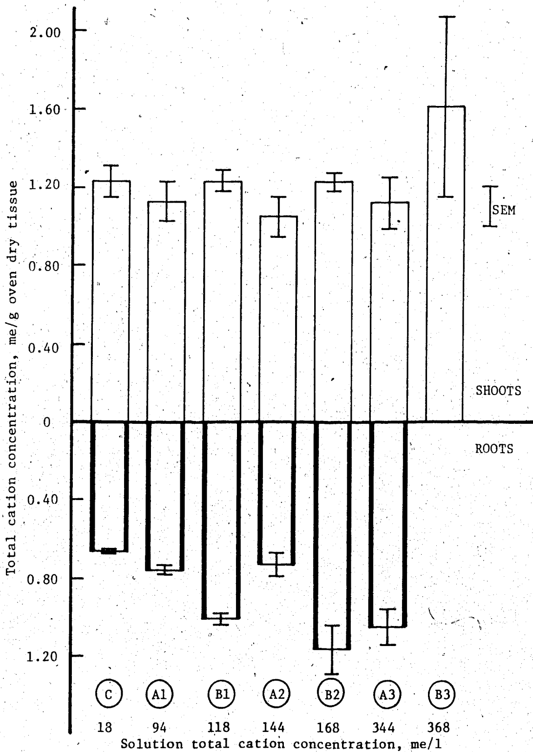
Figure 38. Mean total cation concentration in saltgrass grown at various Mg/Ca ratios and salt concentrations (Experiment 2). See Figure 33 for explanation.
