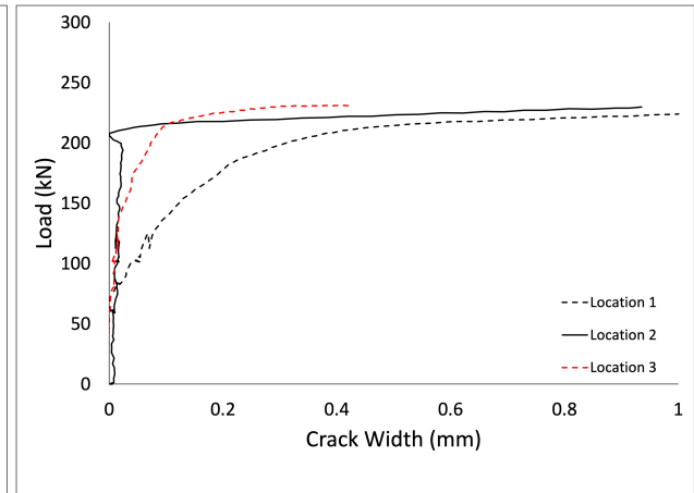
Figure B.4 – DA-250 crack widths
