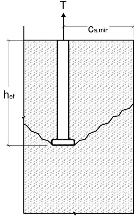
Figure 3.2 – Tension breakout cone truncated by a free edge.
