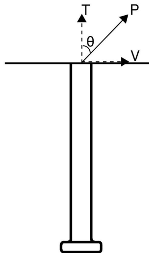
Figure 3.5 – Combined shear ( V ) and tension ( T ) load applied to a single anchor resulting from an inclined force ( P ).
