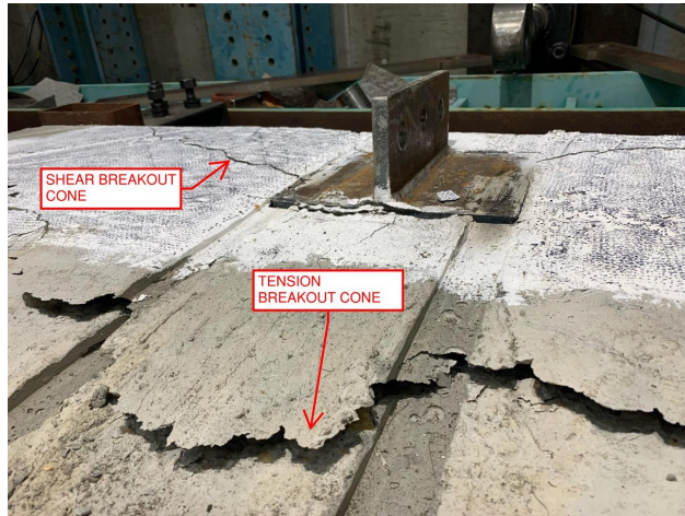
Figure 6.10 – ST-250 P breakout cone. Note the shear breakout cone forming from the embed, while the tension breakout cone extends past the back of the embed.
