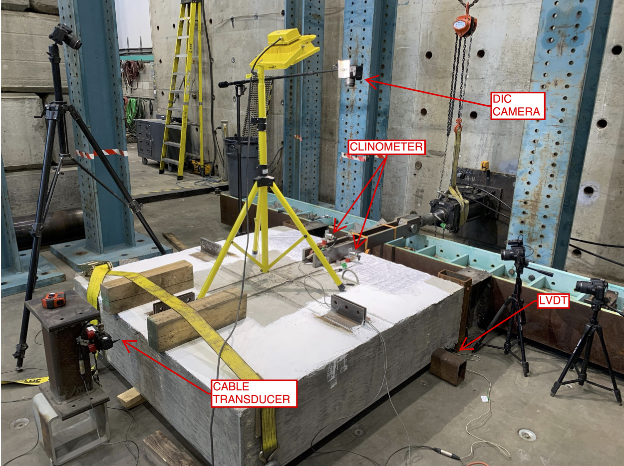
Figure 5.5 – Test instrumentation
