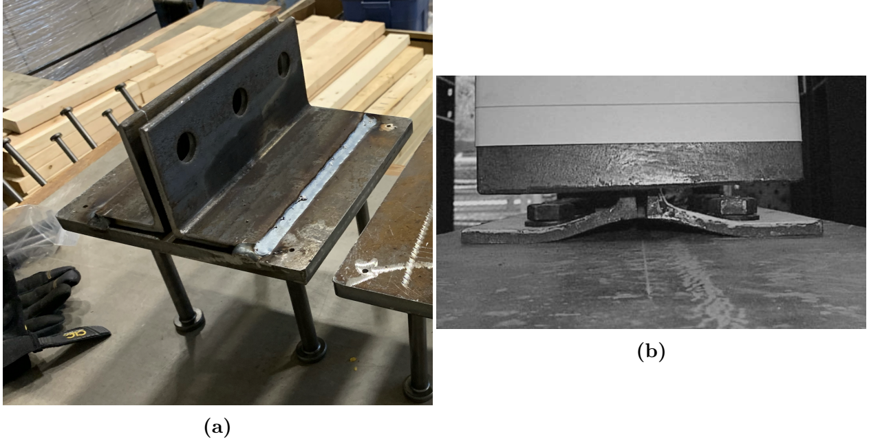
Figure 4.12 – (a) Embed with angles welded to the baseplate along their toes, and (b) bolted double angle connection prying away from baseplate (adapted from Hong et al. (2002))
