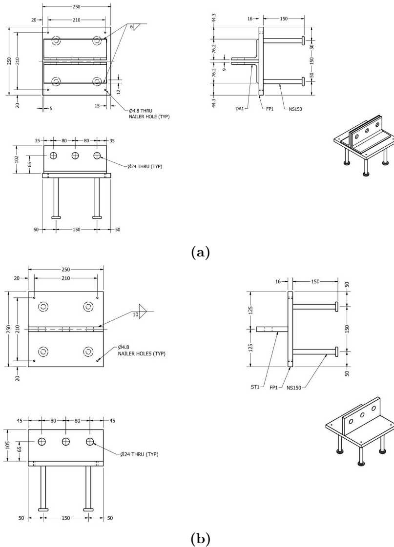
Figure 5.2 – Shop drawings for embedded plates with (a) double angles and (b) shear tabs. ST1, DA1, FP1, and NS150 are item marks for fabrication purposes.
