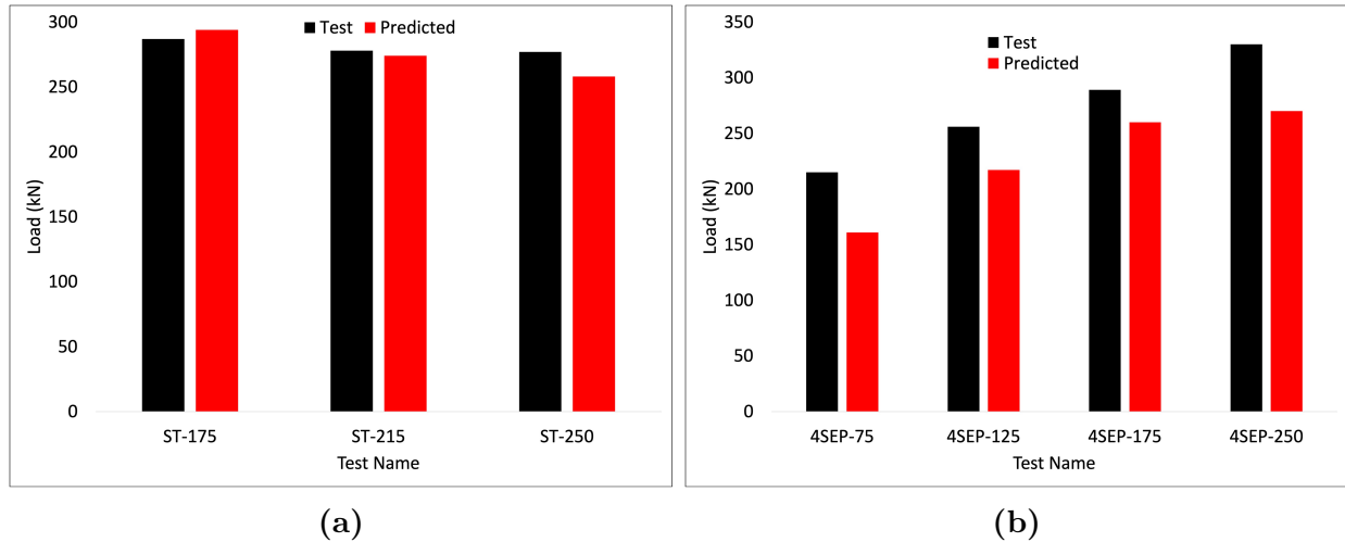
Figure 6.20 – Comparisons predictions from Sharma et al. (2018) with test results from (a) this thesis and (b) Chin (2021)
