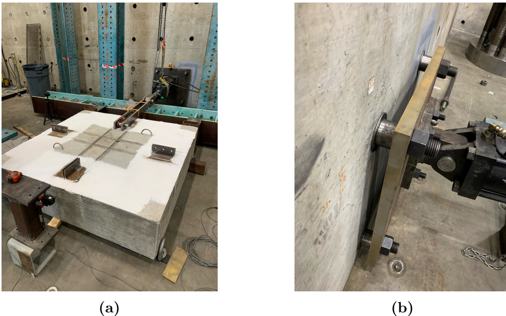
Figure 5.4 – (a) Test setup prior to instrumentation installation and (b) pin connection between the jack and the strong wall
