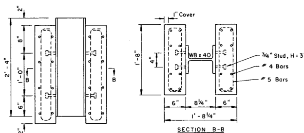
Figure 2.11 – Pushout test setup for examining shear behaviour of headed studs (Ollgaard et al. (1971))
