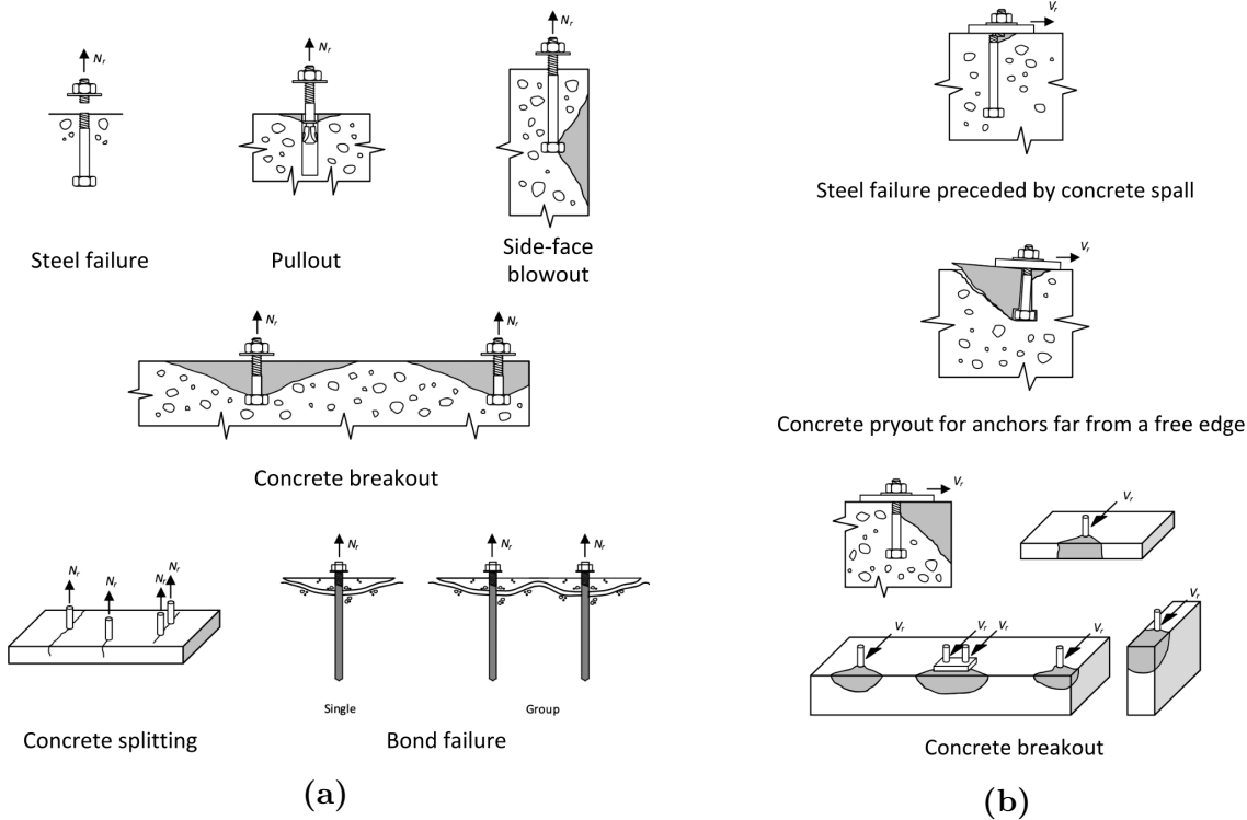
Figure 1.2 – Failure modes of anchors embedded in concrete loaded in (a) tension, and (b) shear (adapted from CSA (2019))
